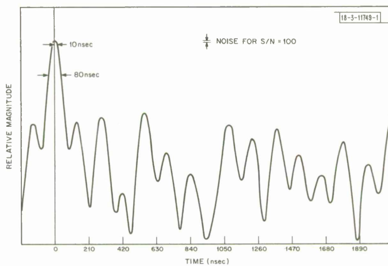
Fig. 8. Sidelobe structure of function shown in Fig. 7.
