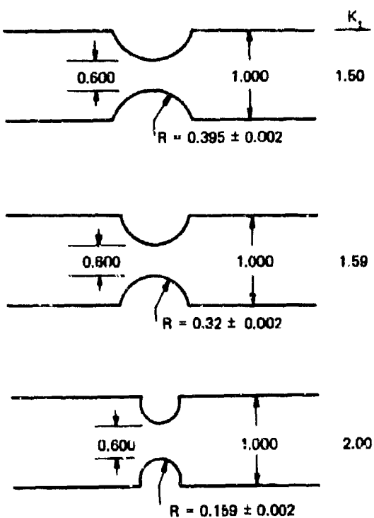
Figure 3. Notch configurations and notch dimensions of 0.1-inch thick flat notched specimens.
