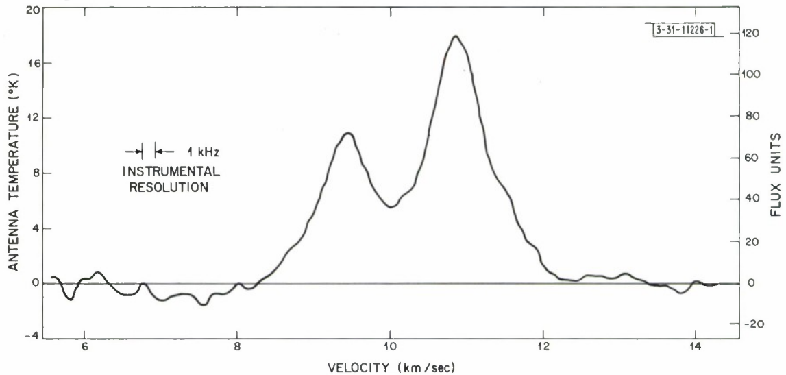
Fig. 18. W28 spectrum at 1720 MHz ( S_O ).
