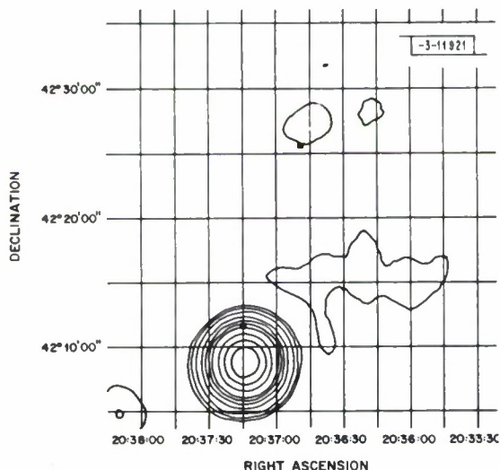
Fig. 46. W75 map at 7.795 GHz at Haystack.
