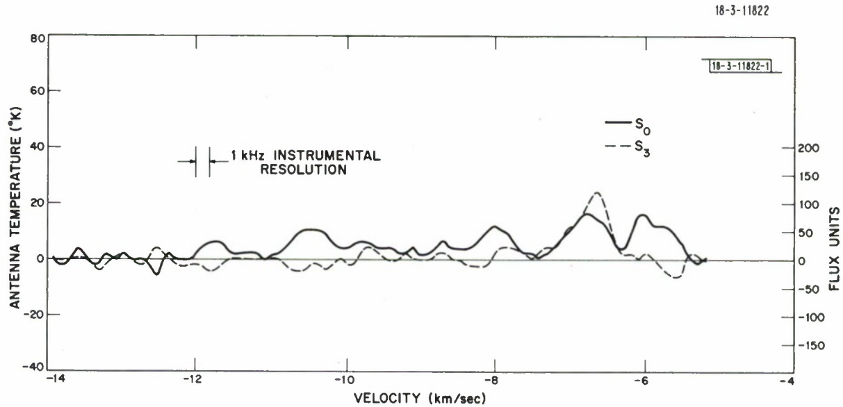
Fig. 29. NGC 6334S restored spectrum at 1665 MHz; Haystack data of September and October 1966.
