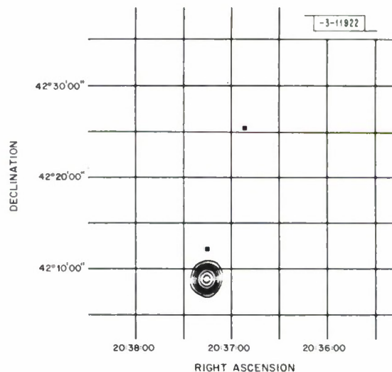
Fig. 47. W75 map at 15.5 GHz at Haystack.
