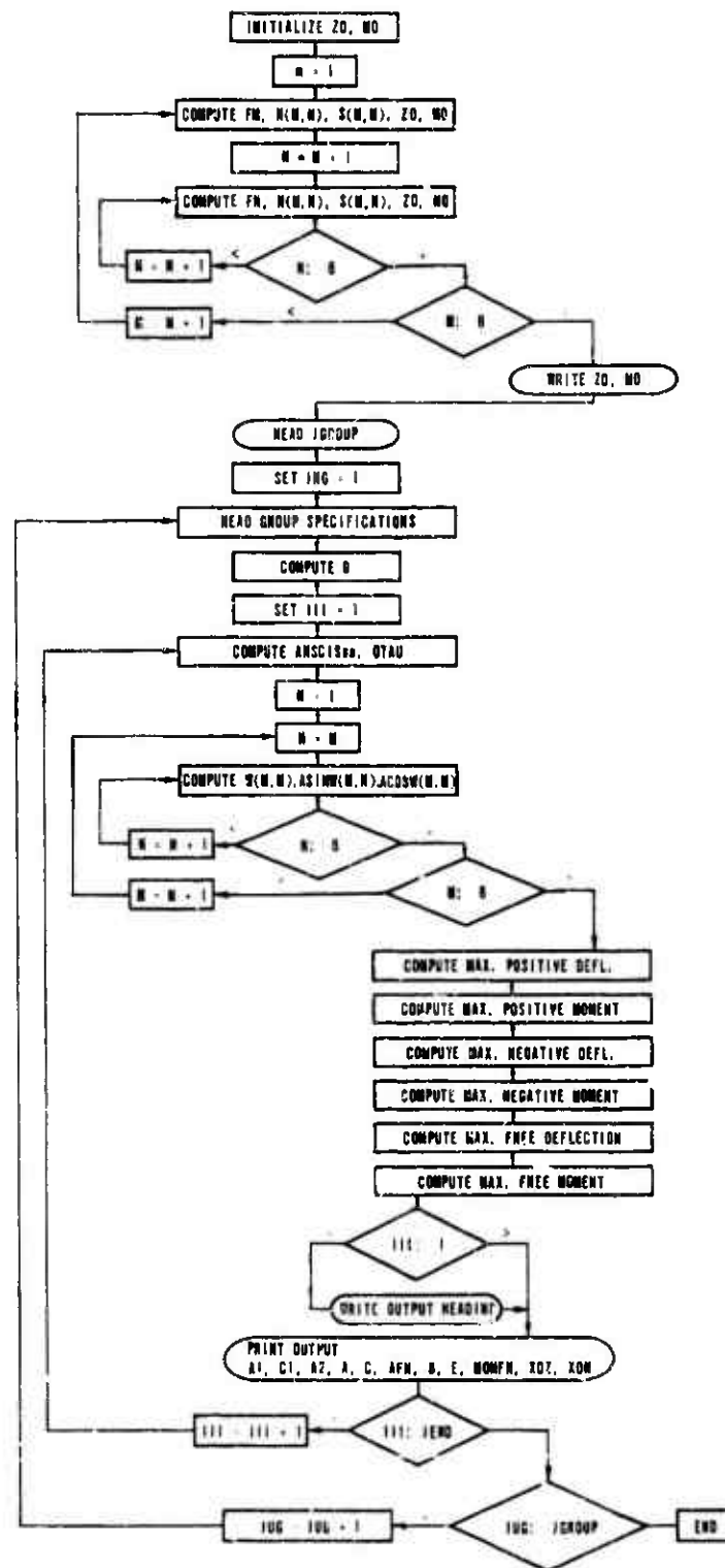
FIG. A.1 FLOW CHART FOR MULTIPLATE PROGRAM TO COMPUTE MULTIMODAL DYNAMIC AMPLIFICATION FACTORS
