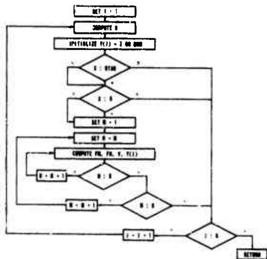
SUBROUTINE FORCZM
