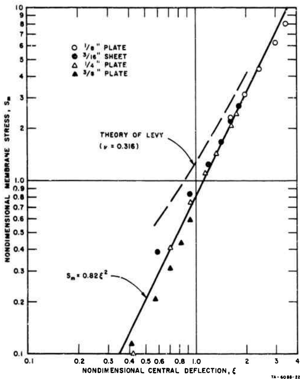
FIG. D.8 MEMBRANE STRESS AS A FUNCTION OF CENTRAL DEFLECTION
