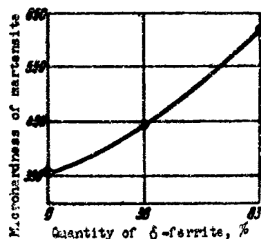
Fig. 4. The effect of the quantity of \delta -ferrite on the microhardness of martensite after quenching from 1100°C in water.
