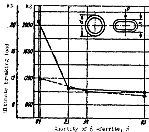
Fig. 6. The effect of the quantity of \delta -ferrite on maximum breaking load of rings during testing for collapse (designation the same as that in Fig. 5).
