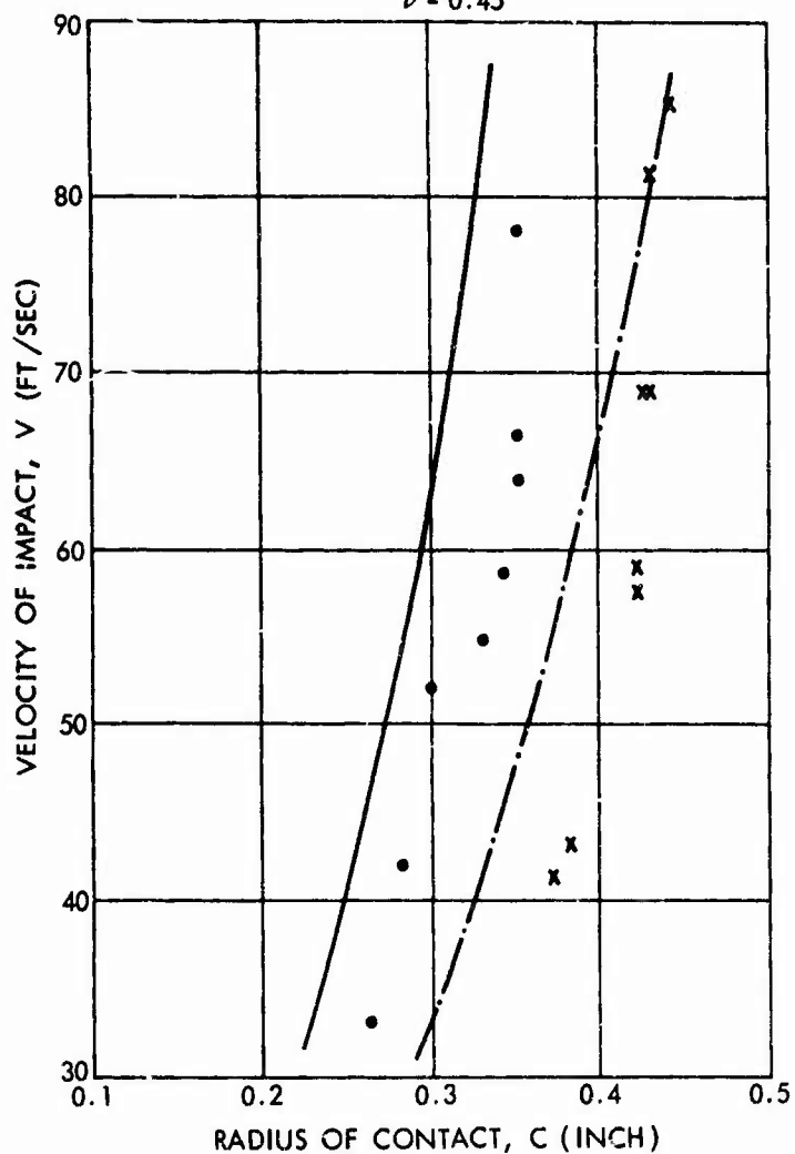
FIG. 9 VELOCITY OF IMPACT VS RADIUS OF CONTACT (ADIPRENE COVERING)
