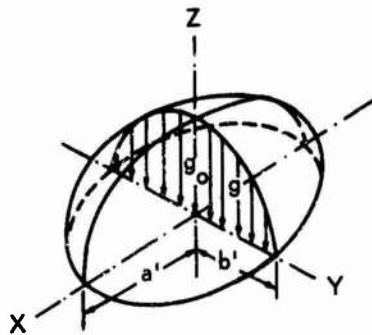
FIG. 1 CONTACT PRESSURE DISTRIBUTION, TWO GENERAL CURVED SURFACES
