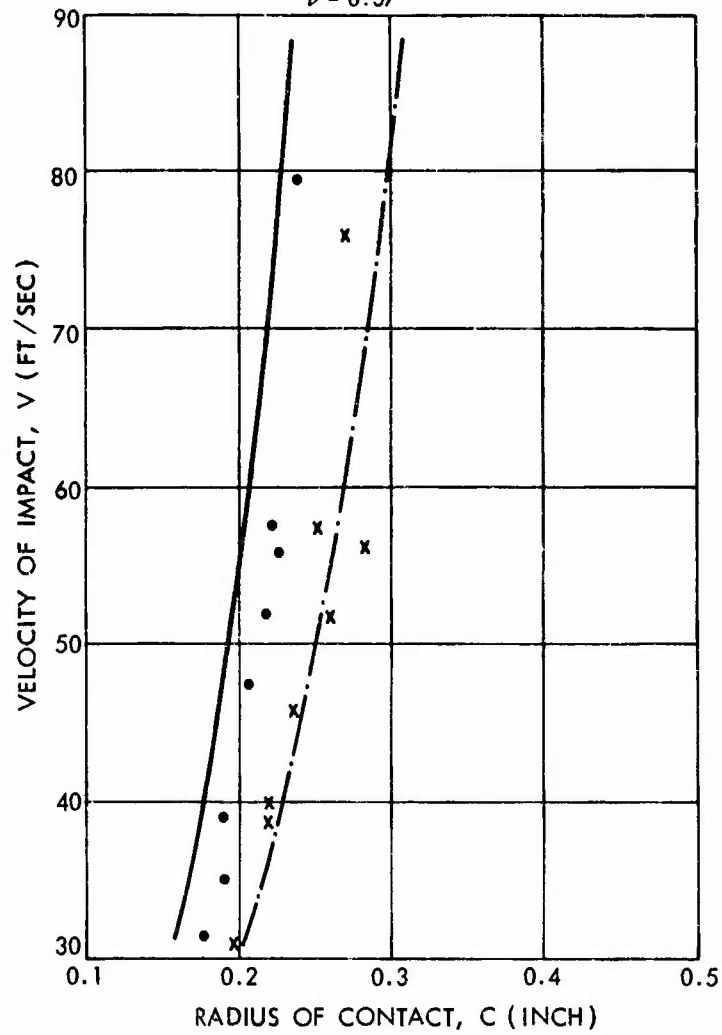
FIG. 8 VELOCITY OF IMPACT VS RADIUS OF CONTACT (LEXAN COVERING)
