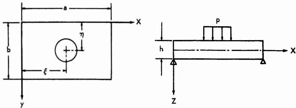
FIG. 5 UNIFORMLY DISTRIBUTED CONTACT PRESSURE
