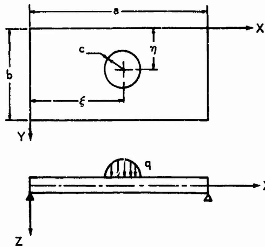
FIG. 4 HEMISPHERICALLY DISTRIBUTED CONTACT PRESSURE
