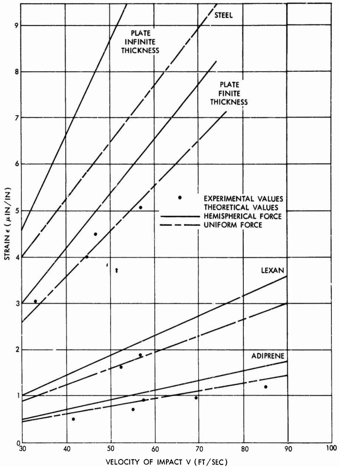
FIG. 10 STRAIN VS VELOCITY OF IMPACT (1"-R PROJECT)
