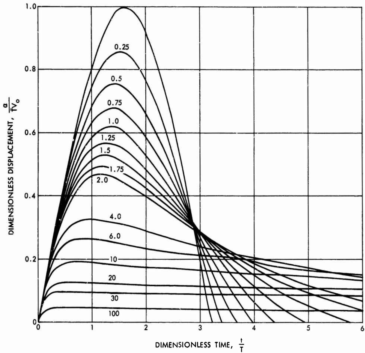
FIG. 3 DIMENSIONLESS DISPLACEMENT AS A FUNCTION OF DIMENSIONLESS TIME
