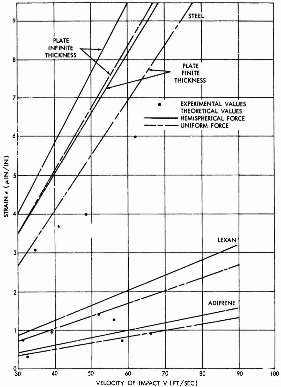
FIG. 11 STRAIN VS VELOCITY OF IMPACT (0.5"-R PROJECT)
