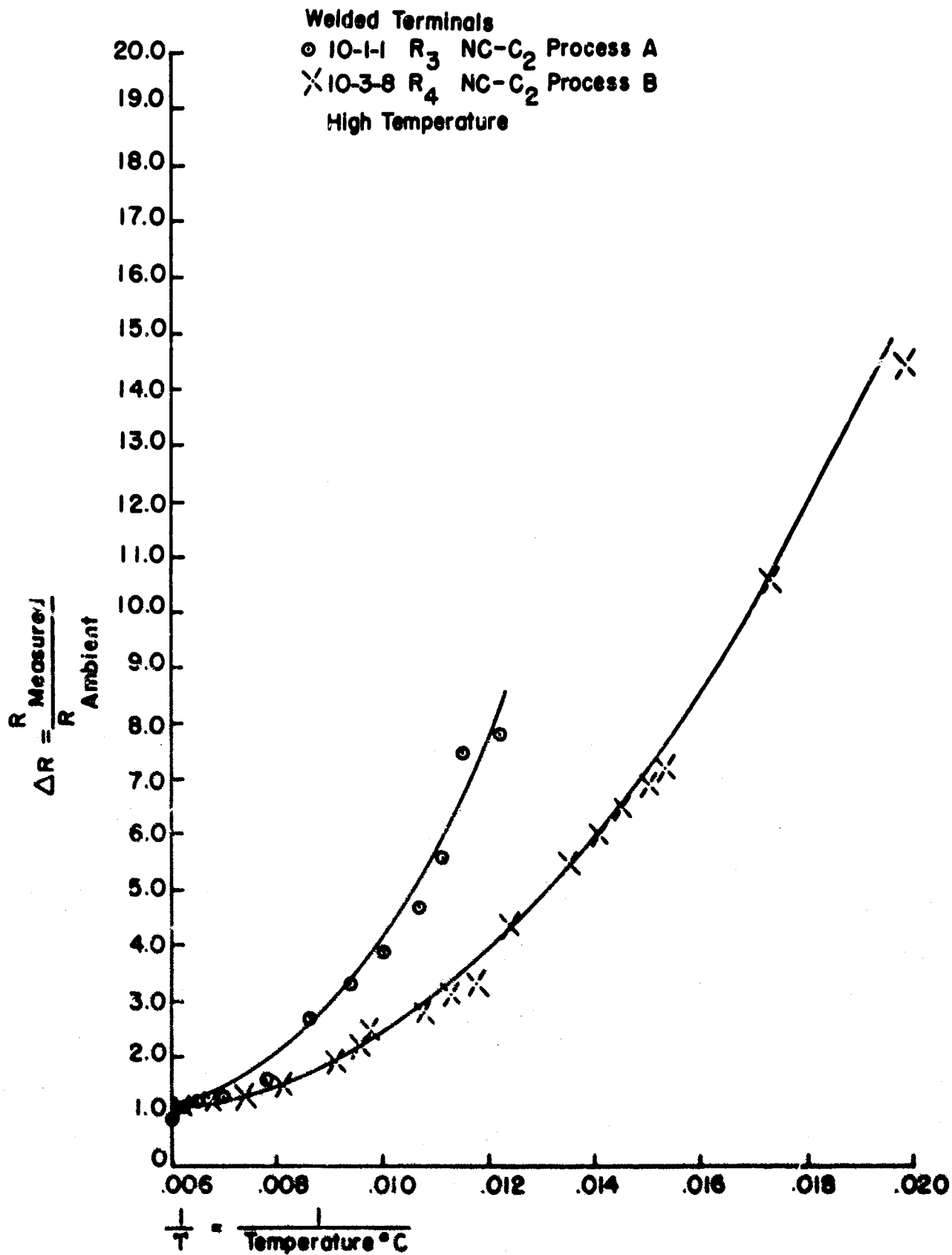
Fig A13 Cooling Curve \Delta R vs \frac{1}{T}
