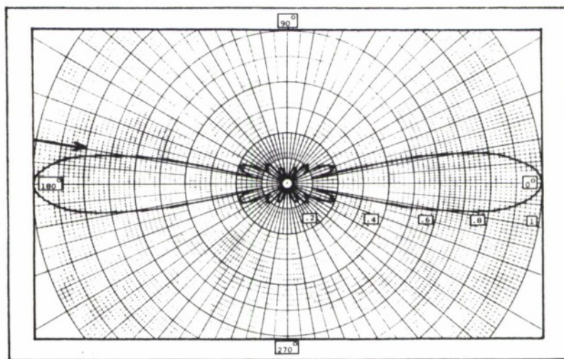
Figure 2-1. Vertical Field Strength Pattern of Communications Products Type 200-509 Antenna (Extracted from Reference 1)
