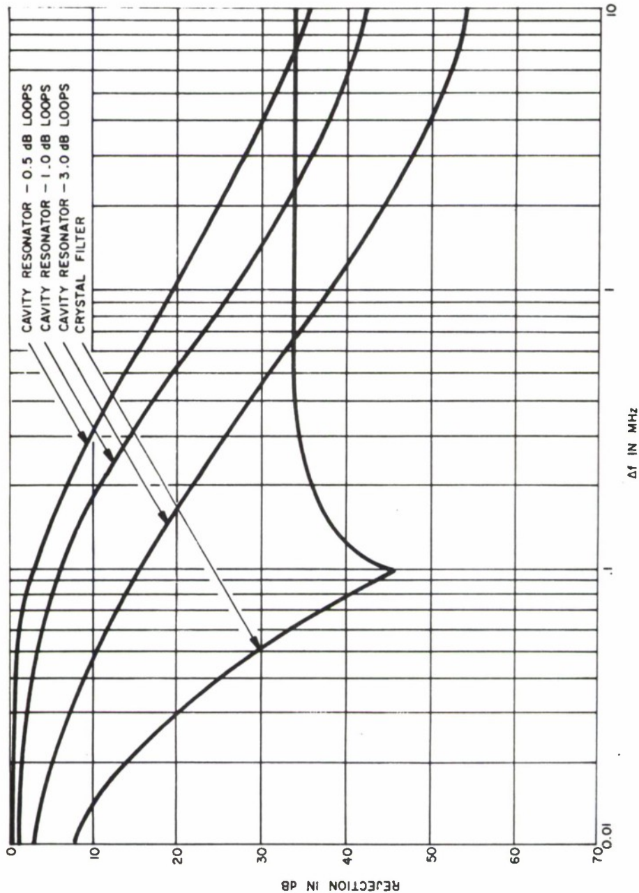
Figure 2-5. Selectivity Characteristics of RF Filtering Devices
