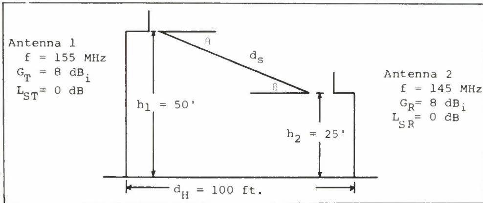
Figure 2-3. Sample Antenna Installation
