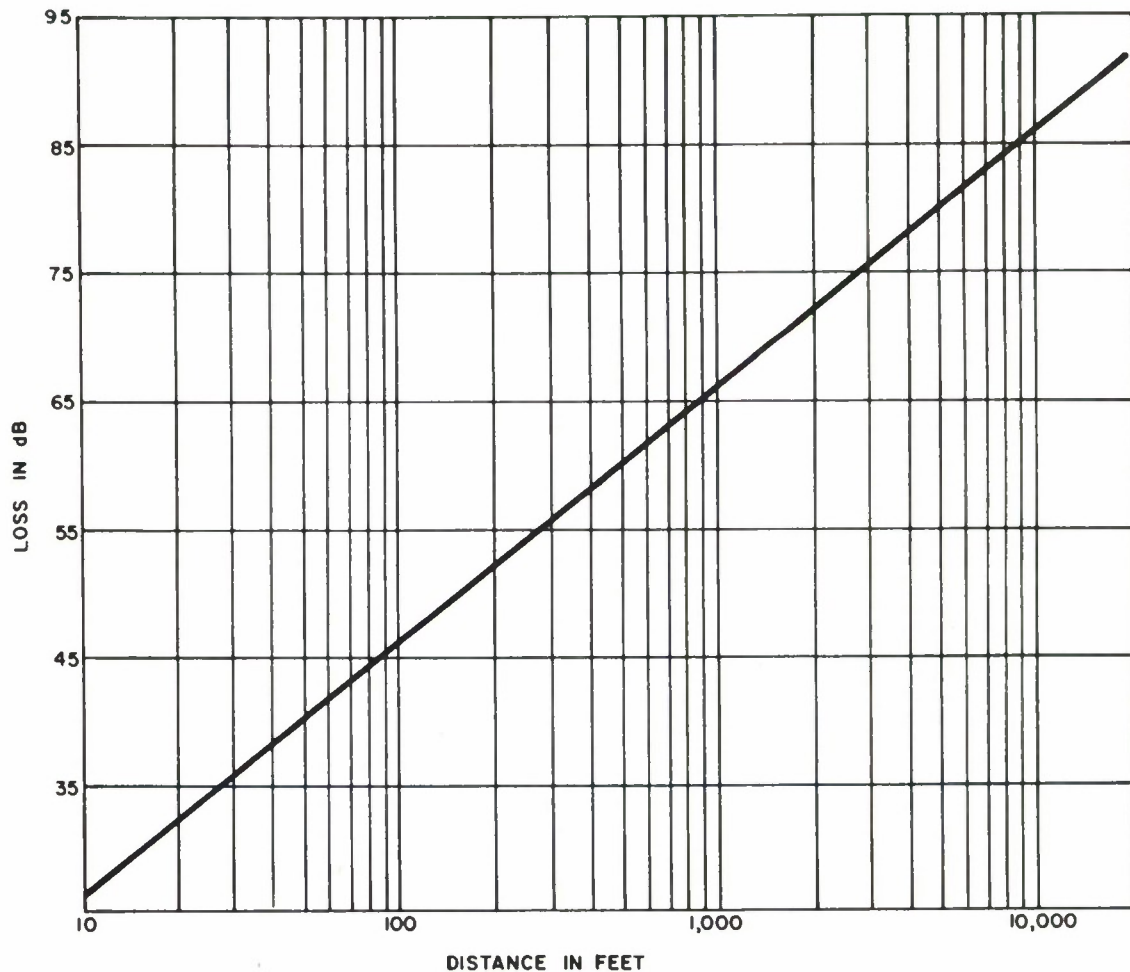
Figure 2-2. Free-Space Loss Versus Distance at 150 MHz
