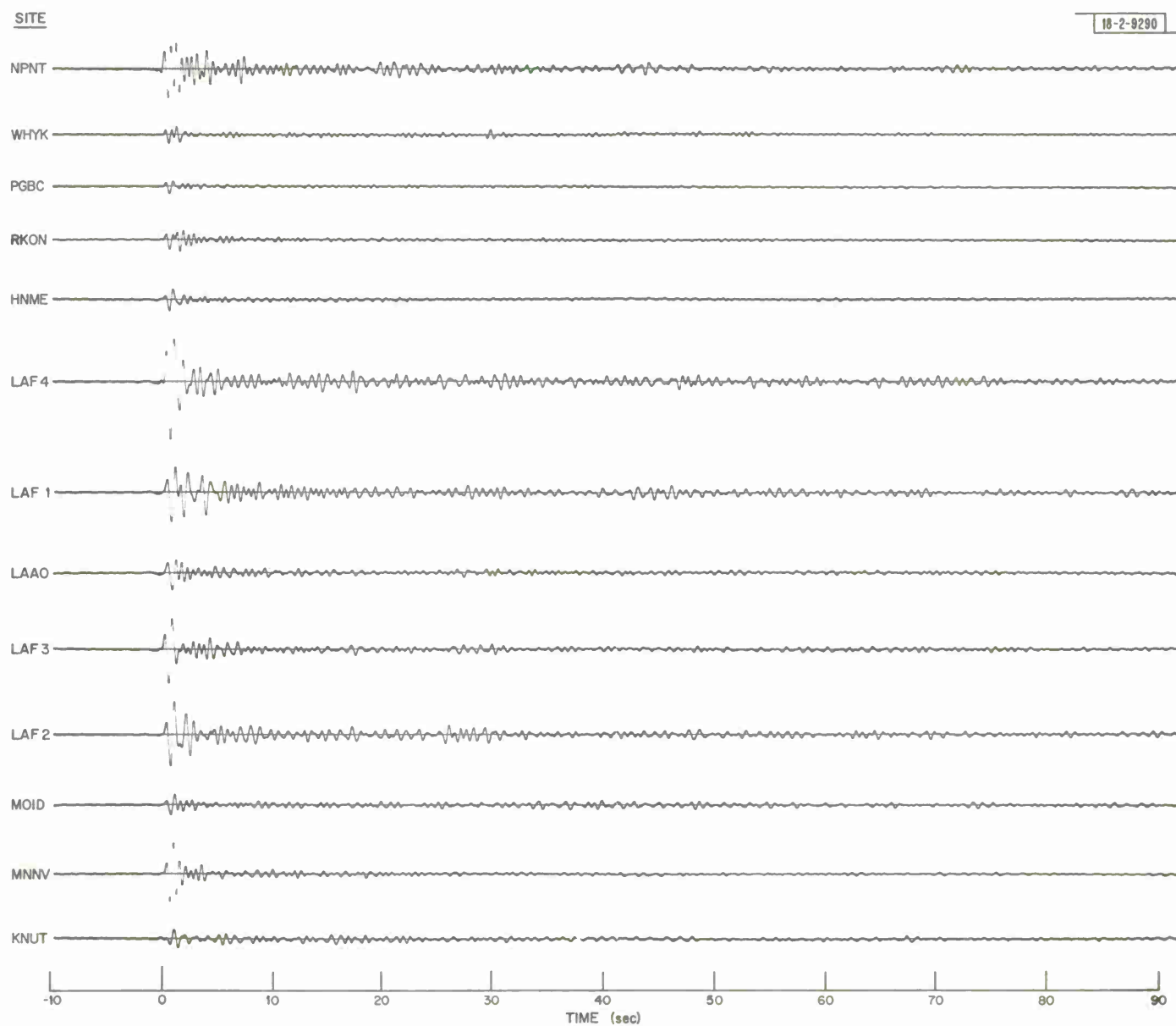
Fig. 7. Waveforms for 18 December 1966 Eastern Kazakh event.
