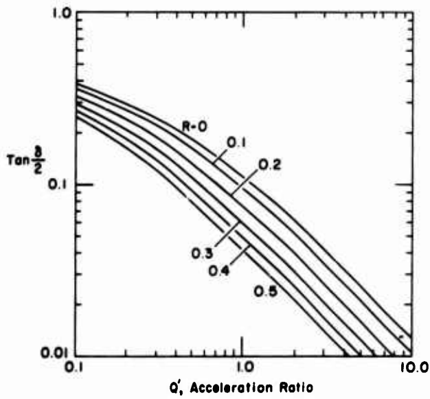
Figure 8. \tan \delta/2 vs acceleration ratio Q' , third mode.
