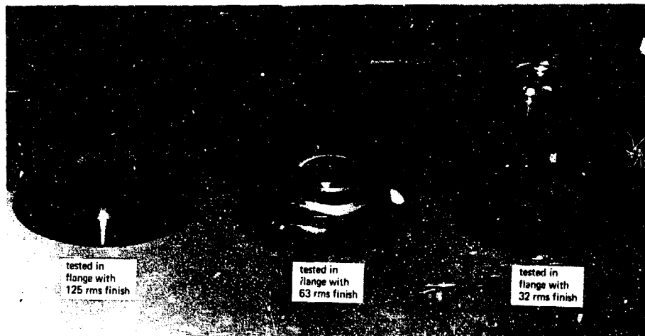
Figure E-3. Model viewports after test, set 1.
