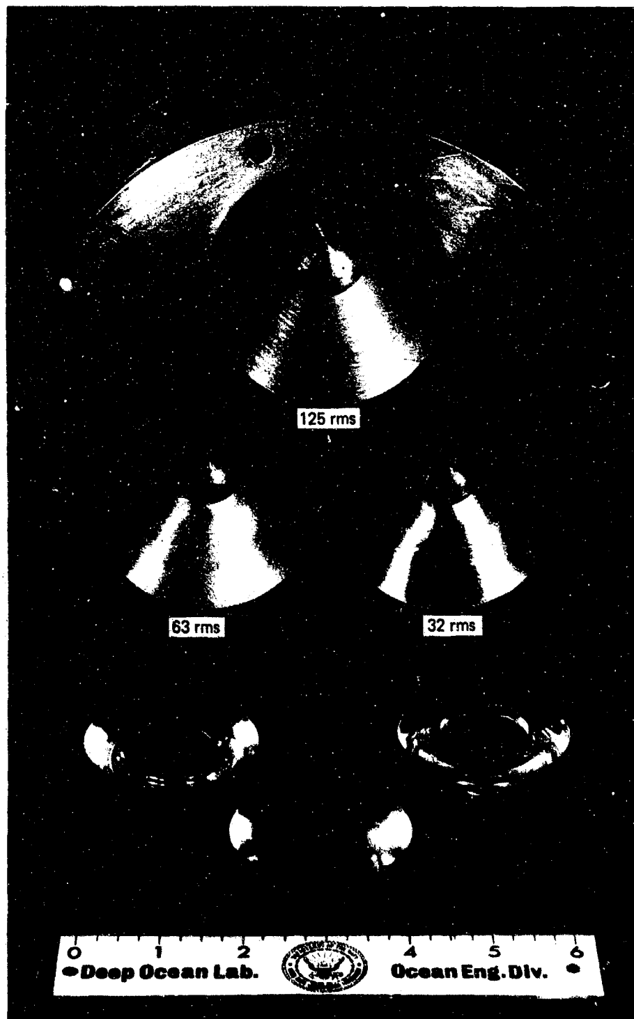
Figure E-2. Flange for surface finish tests.
