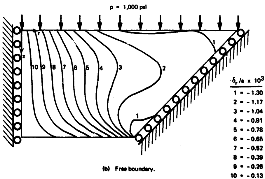
Figure 6. Radial displacement contour plots.
