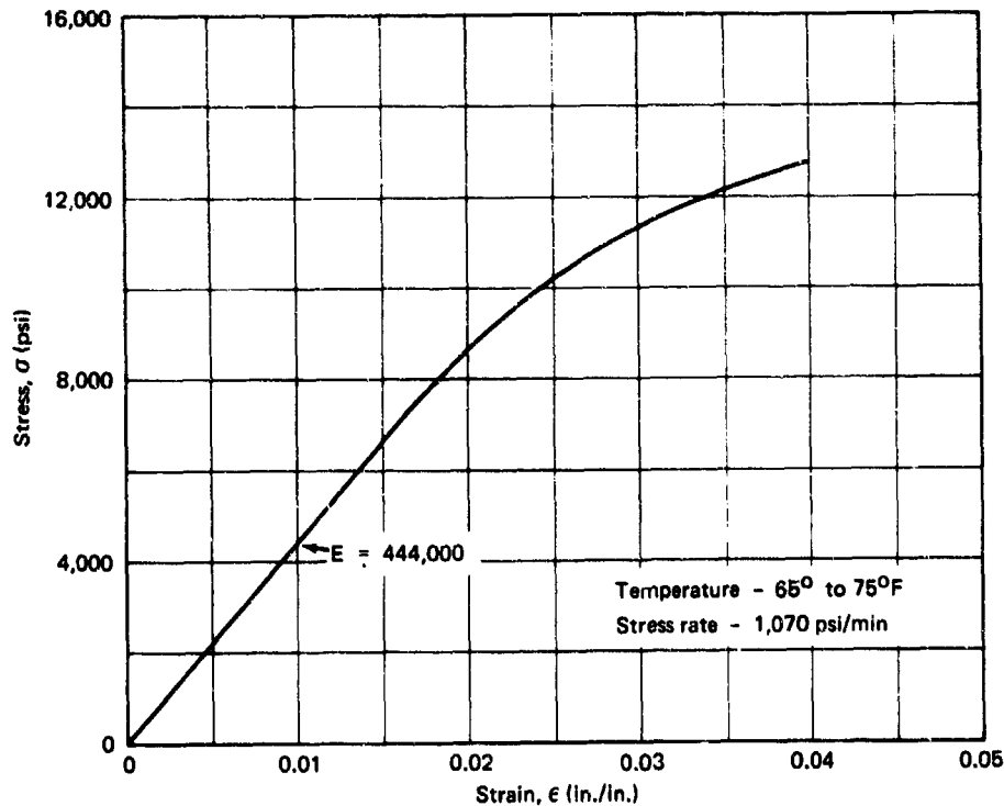
Figure C-2. Compressive stress-strain diagram for acrylic plastic.
