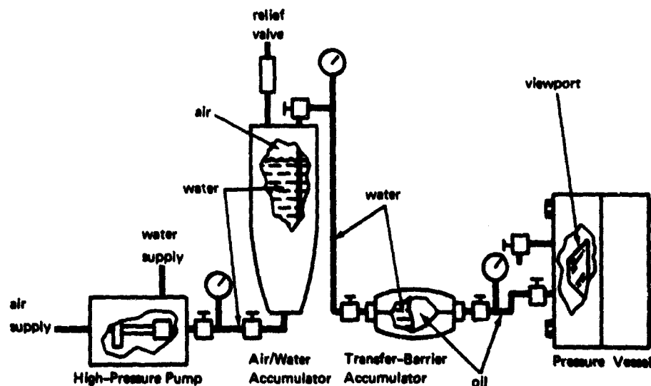
Figure B-1. Schematic of high-pressure equipment.
