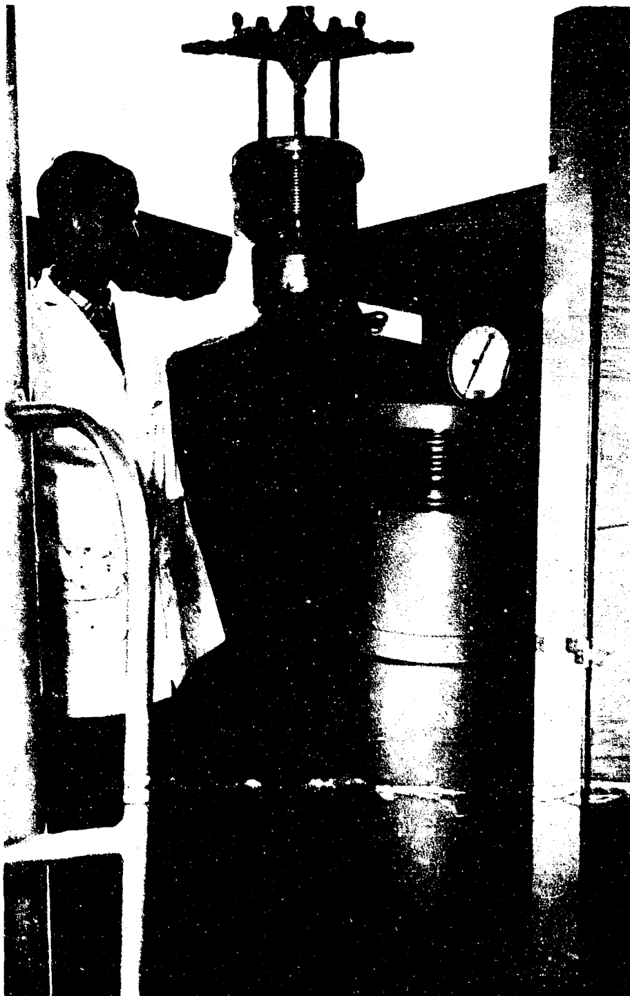
Figure E-1. Pressure vessel converted from 16-inch Naval gun shell.
