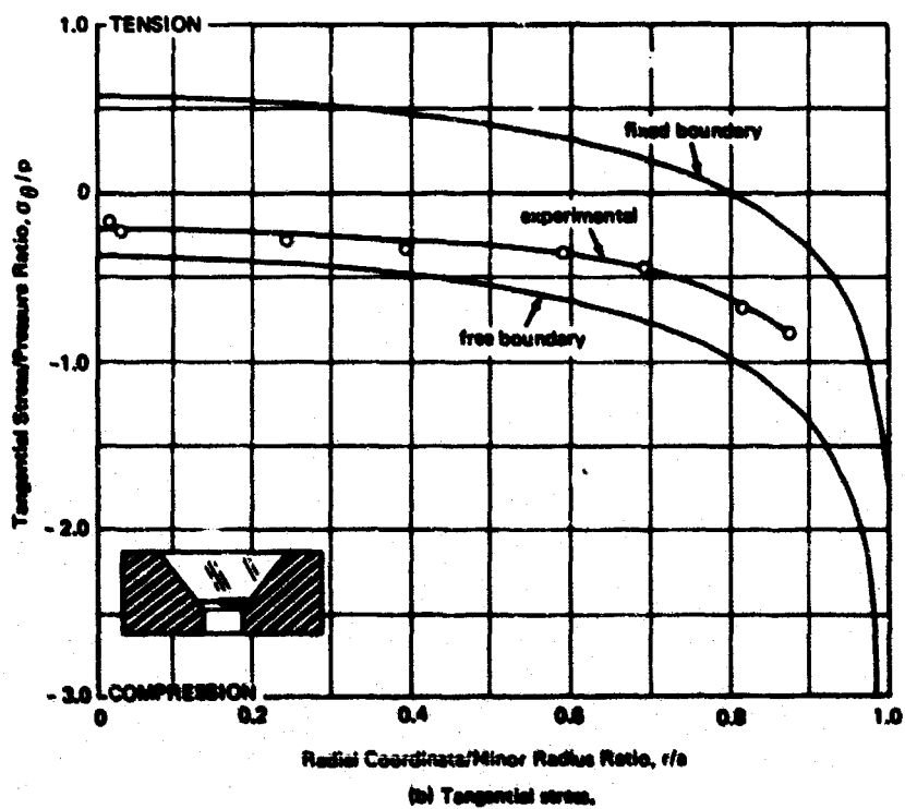
Figure 8. Stress distribution on low-pressure face.
