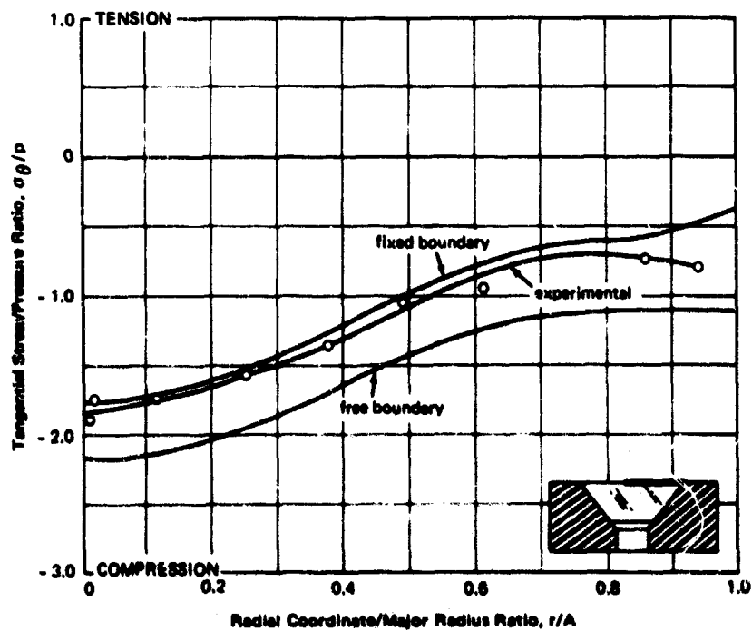
(b) Tangential stress.
