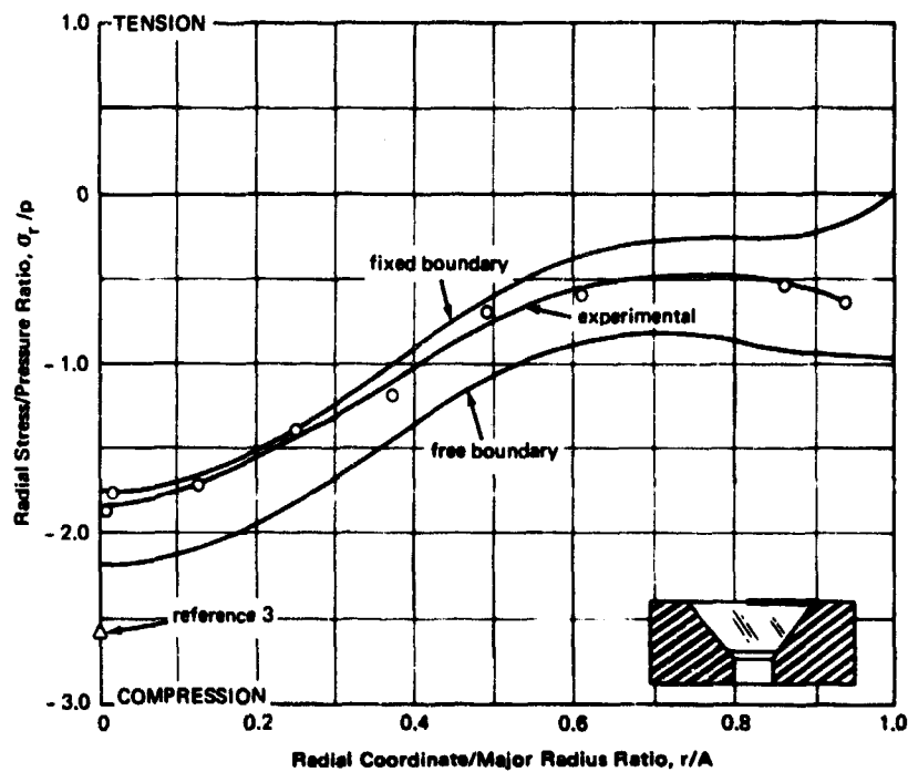
(a) Radial stress.
