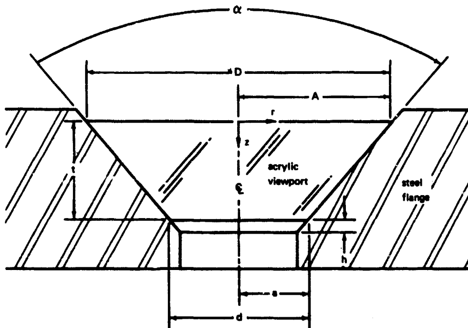
Figure 2. Cross section of a typical viewport.
