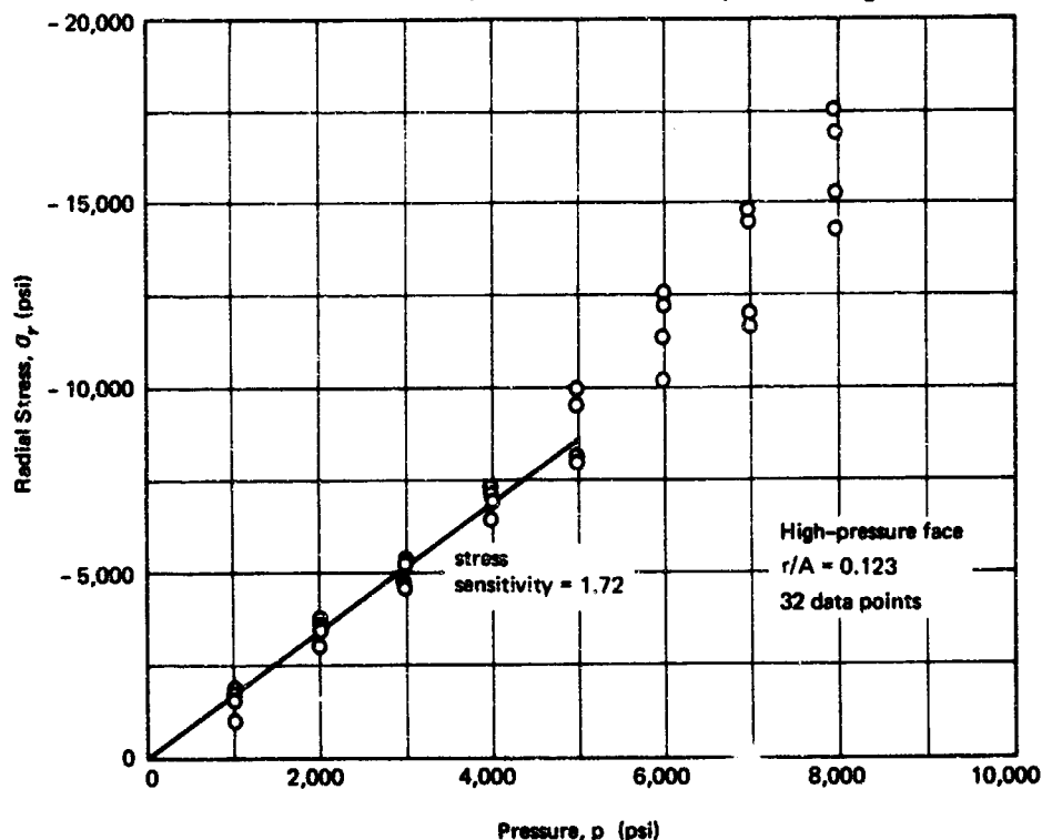
Figure A-6. Typical experimental stress versus pressure plot.
