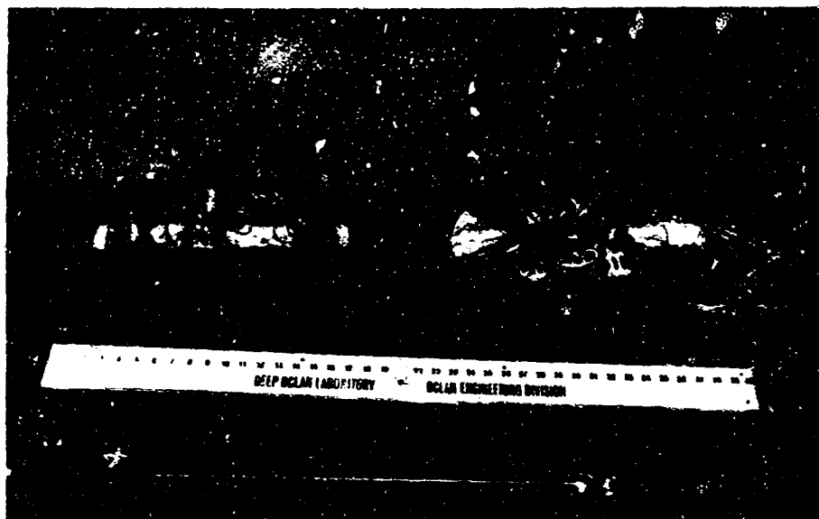
Figure A-5. High-pressure electrical penetrators shown with 8-inch minor diameter viewports.
