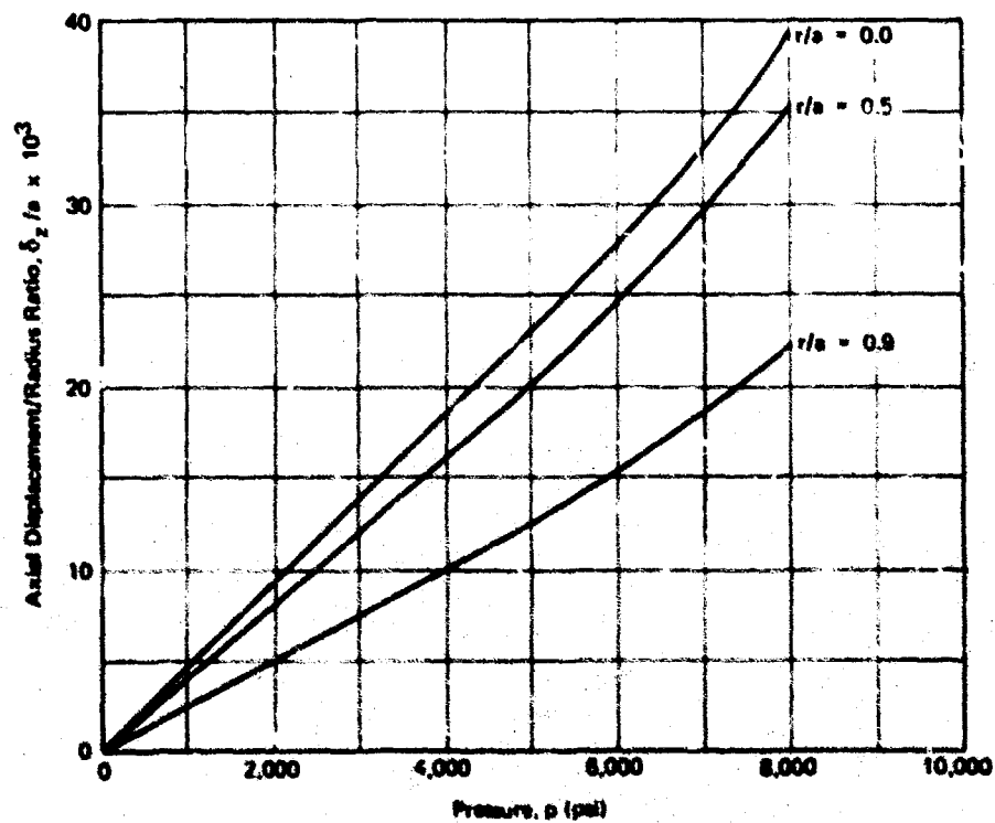
Figure A-3. Experimental displacements for low-pressure face.
