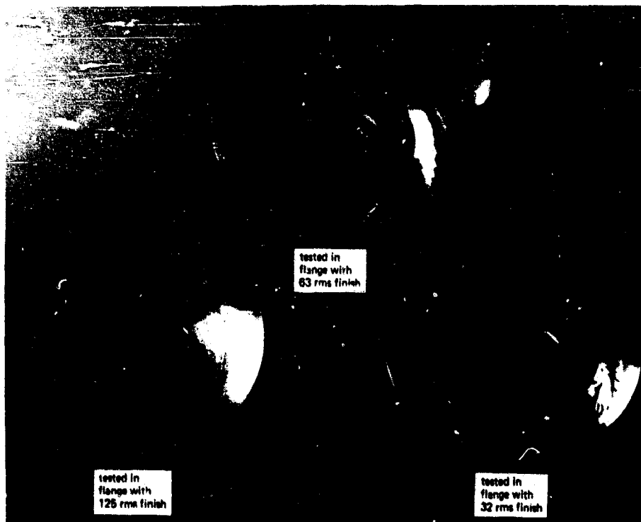
Figure E-4. Model viewports after test, set 3.
