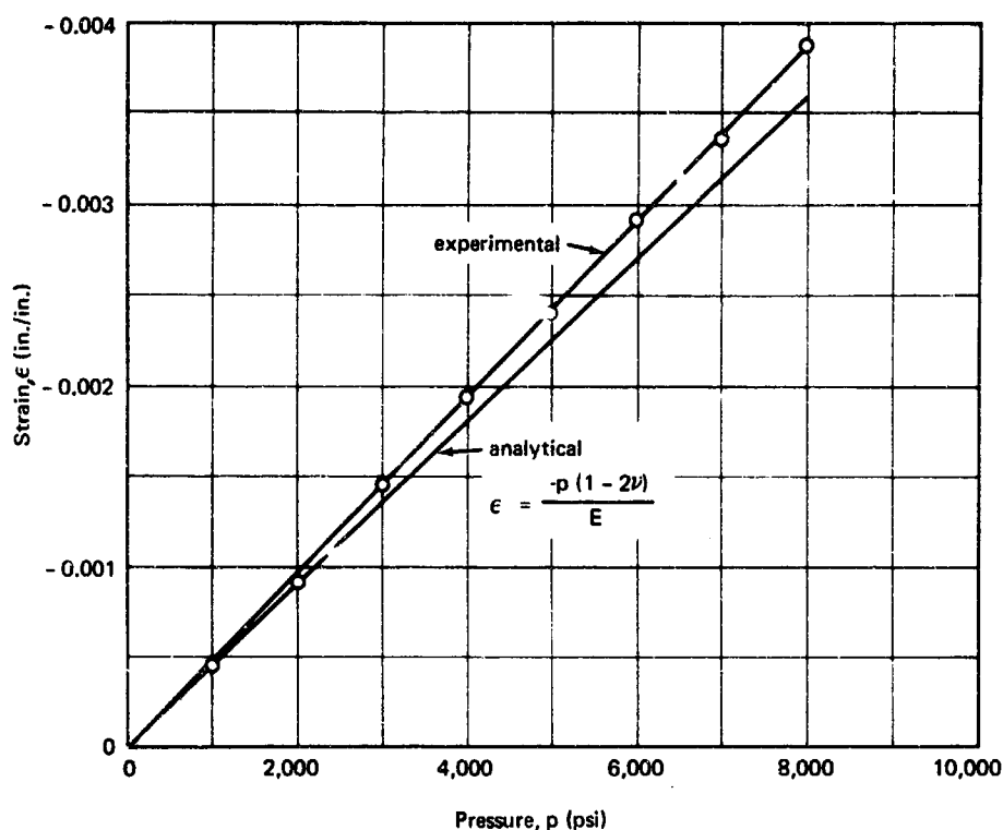
Figure C-3. Hydrostatic verification of material properties.
