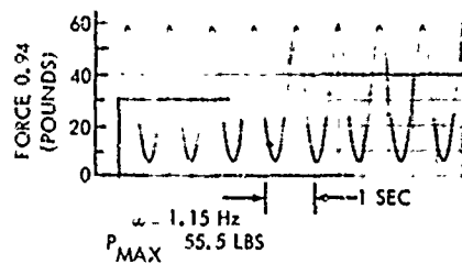
(c) FORCE RESPONSE AT RESONANCE
