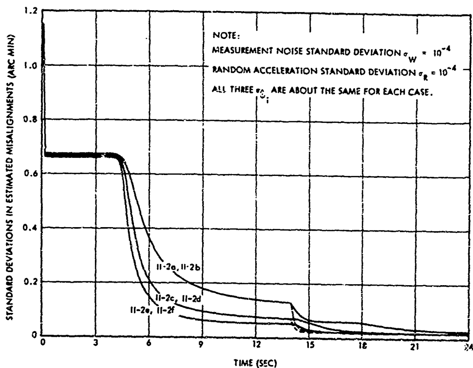
Figure 4.12a Standard Deviations in the Estimated Misalignments, \hat{\sigma}_{\psi_i} , for Nominal Trajectories II-2a through II-2f
