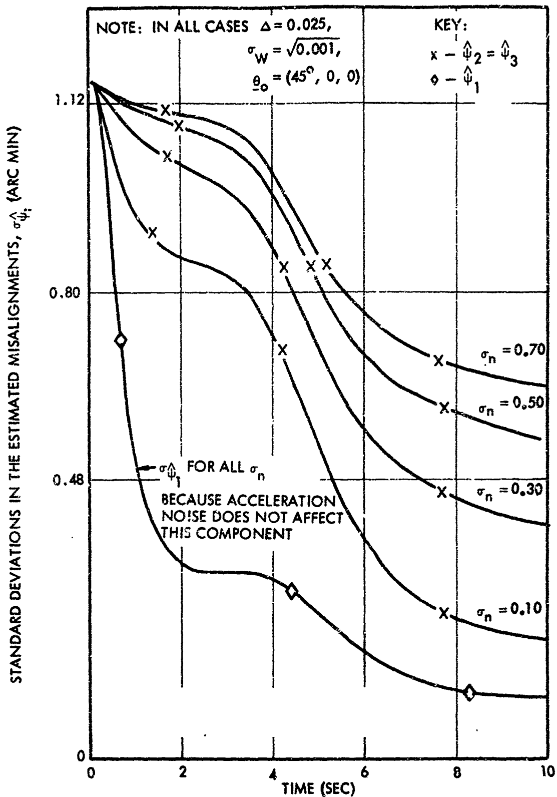
Figure 4.3b \sigma_{\hat{\phi}_i} for various \sigma_n using the Nominal shown in Fig 4.1
