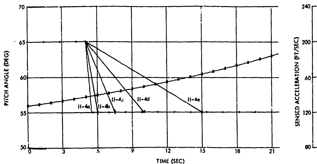
Figure 4.14a Nominal Trajectories II-4a Through II-4e
