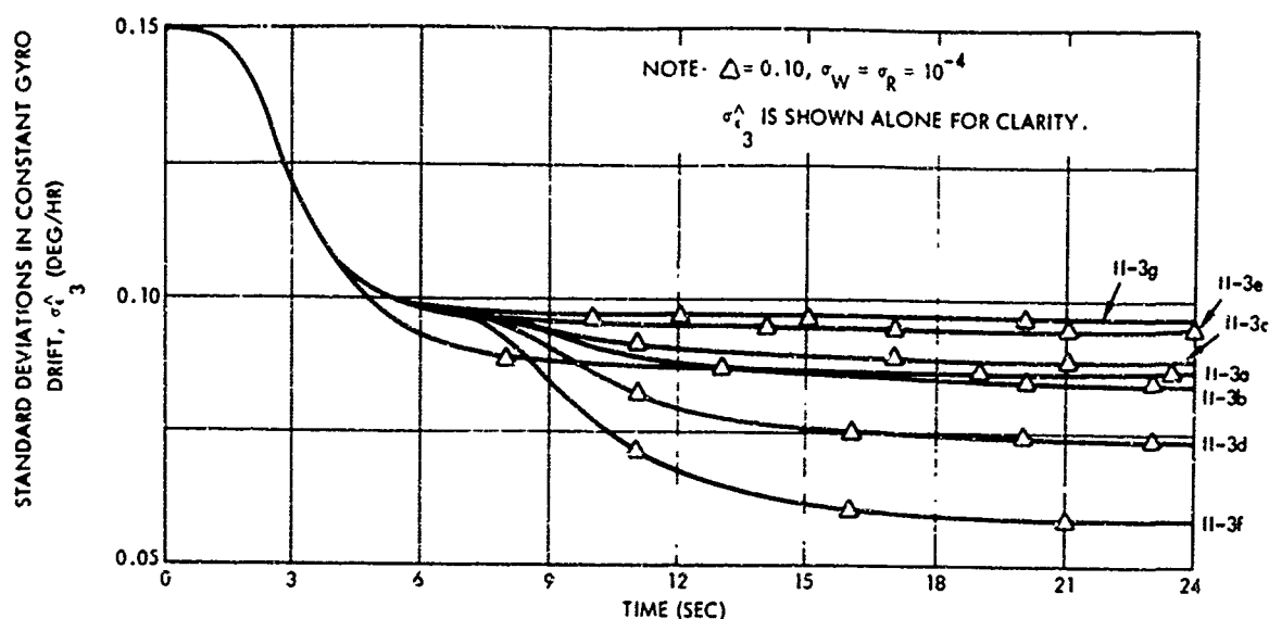
Figure 4.13d Standard Deviations in the Estimated Constant Gyro Drifts, \sigma_{\hat{e}_3}^{\wedge} , for Nominals II-3a Through II-3g
