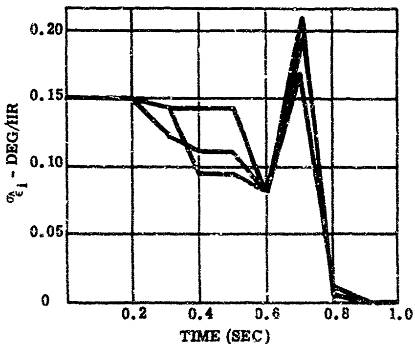
Figure 5.2b Constant Gyro Drift Sigmas, \sigma_{\epsilon_i} , for \sigma_R = \sigma_W = 0 .
