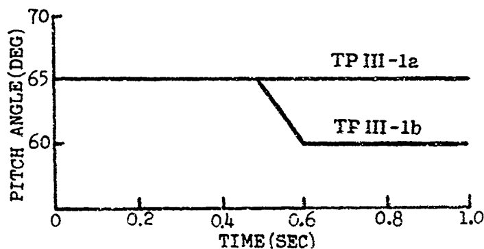
Figure 5.3 Nominal Pitch Profiles III-1a and III-1b
