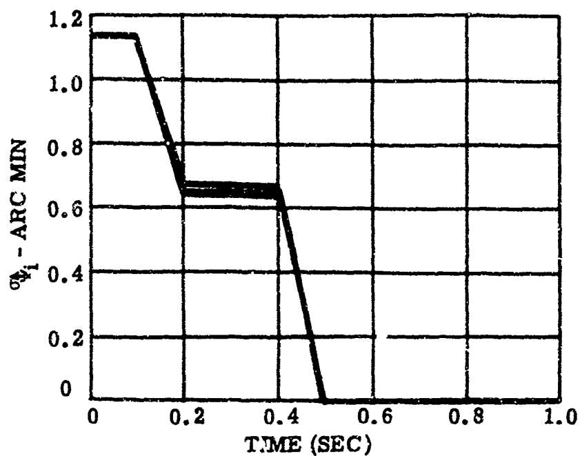
Figure 5.2a Misalignment Sigmas, \sigma_{\psi_i} , for \sigma_R = \sigma_W = 0 .
