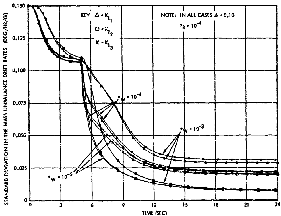
Figure 4.20a Effect of \sigma_W on the Estimation of k_{S_i}
