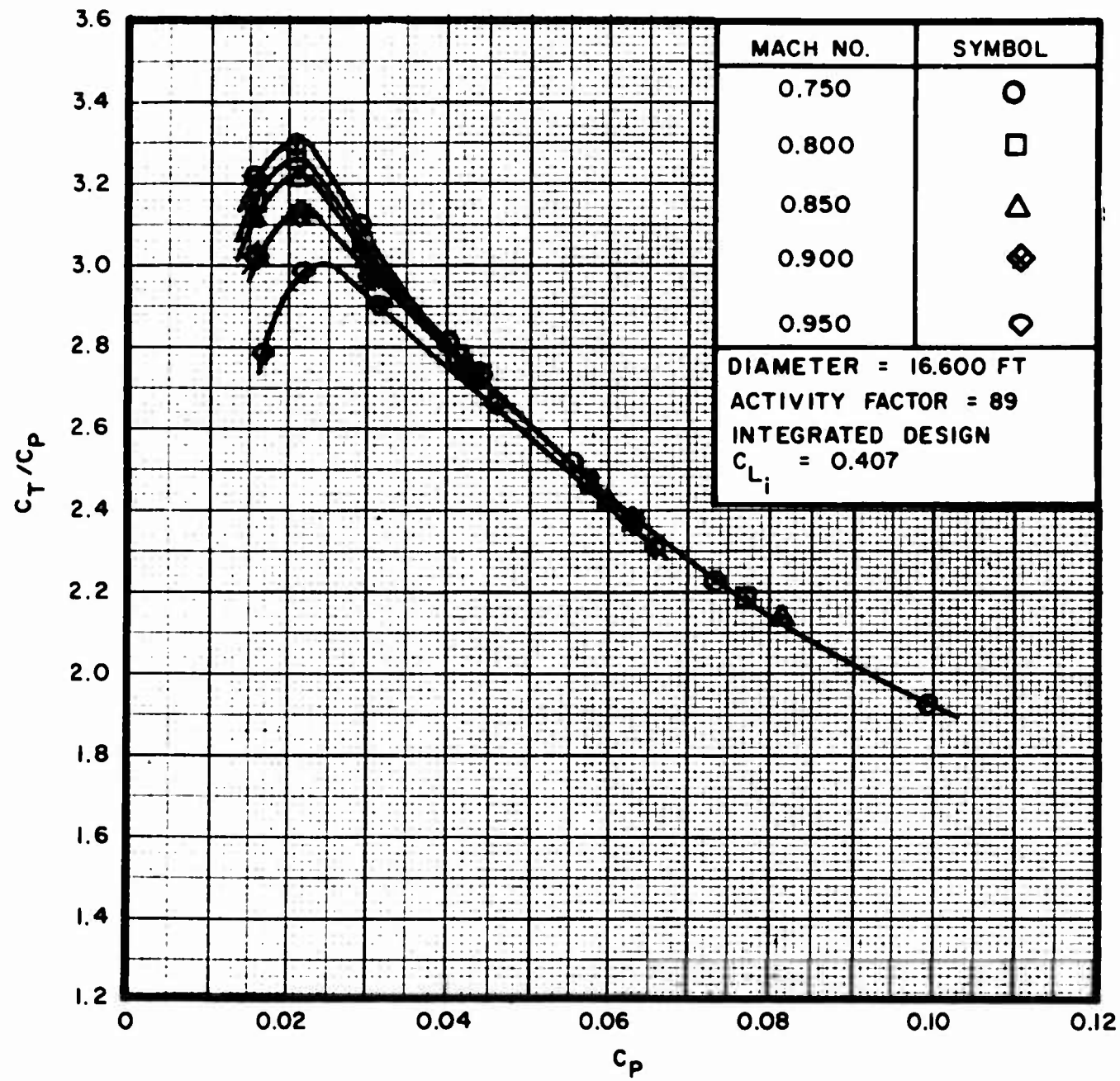
Figure 33. SK59868-0R (Round Tip), Walls Down, Performance at Different Tip Mach Numbers a. C_T/C_P vs C_P plot
