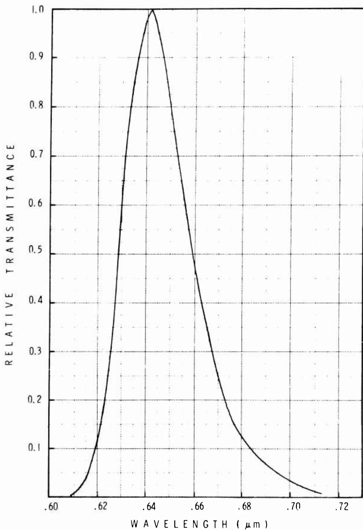
Fig. 23 - Pyrometer Filter Band-Pass Characteristic
