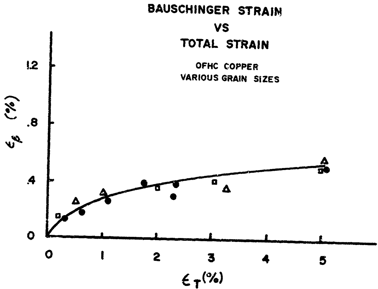
Figure 7a. \epsilon_B vs. \epsilon_{total} OFHC Cu - 3 Different Grain Sizes
