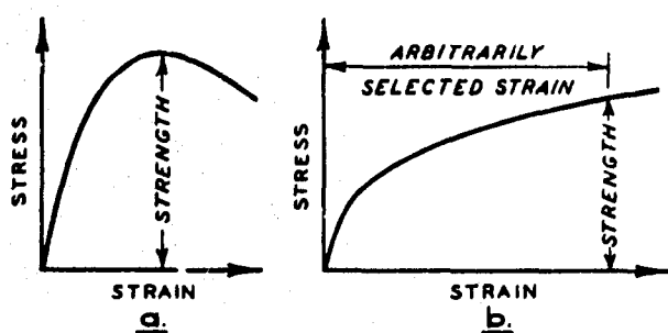
Fig. 3.1 Stress-strain curves from controlled-strain tests
