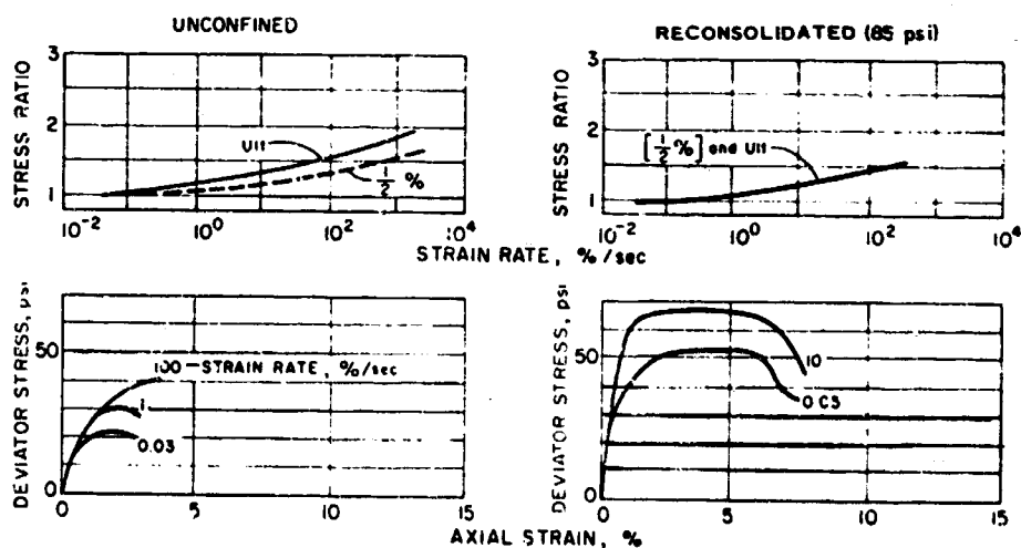
Fig. 3.20 Effect of strain rate on behavior of a saturated clay with and without confining pressure
