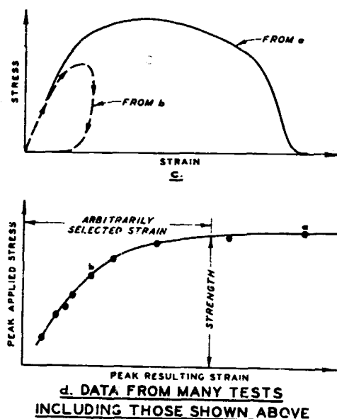
Fig. 3.3 Results from controlled-stress tests with pulse loading
