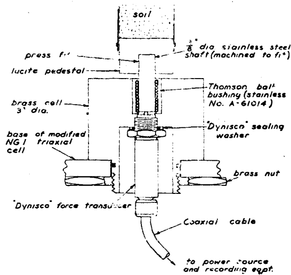
Fig. 3.12 Force transducer for recent tests at MIT
