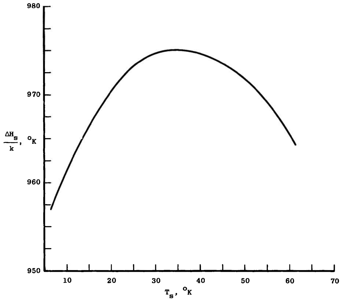
Fig. 12 Heat of Sublimation for Solid Argon at Equilibrium
