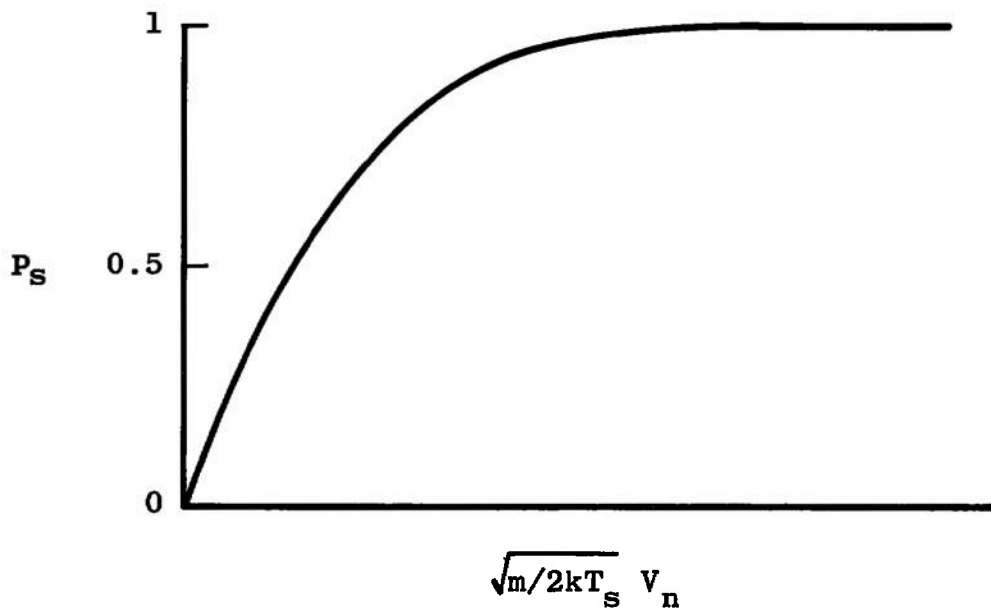
b. P_s for Surface Velocities with an Incident Beam Fig. 15 Probability for a Surface Velocity
