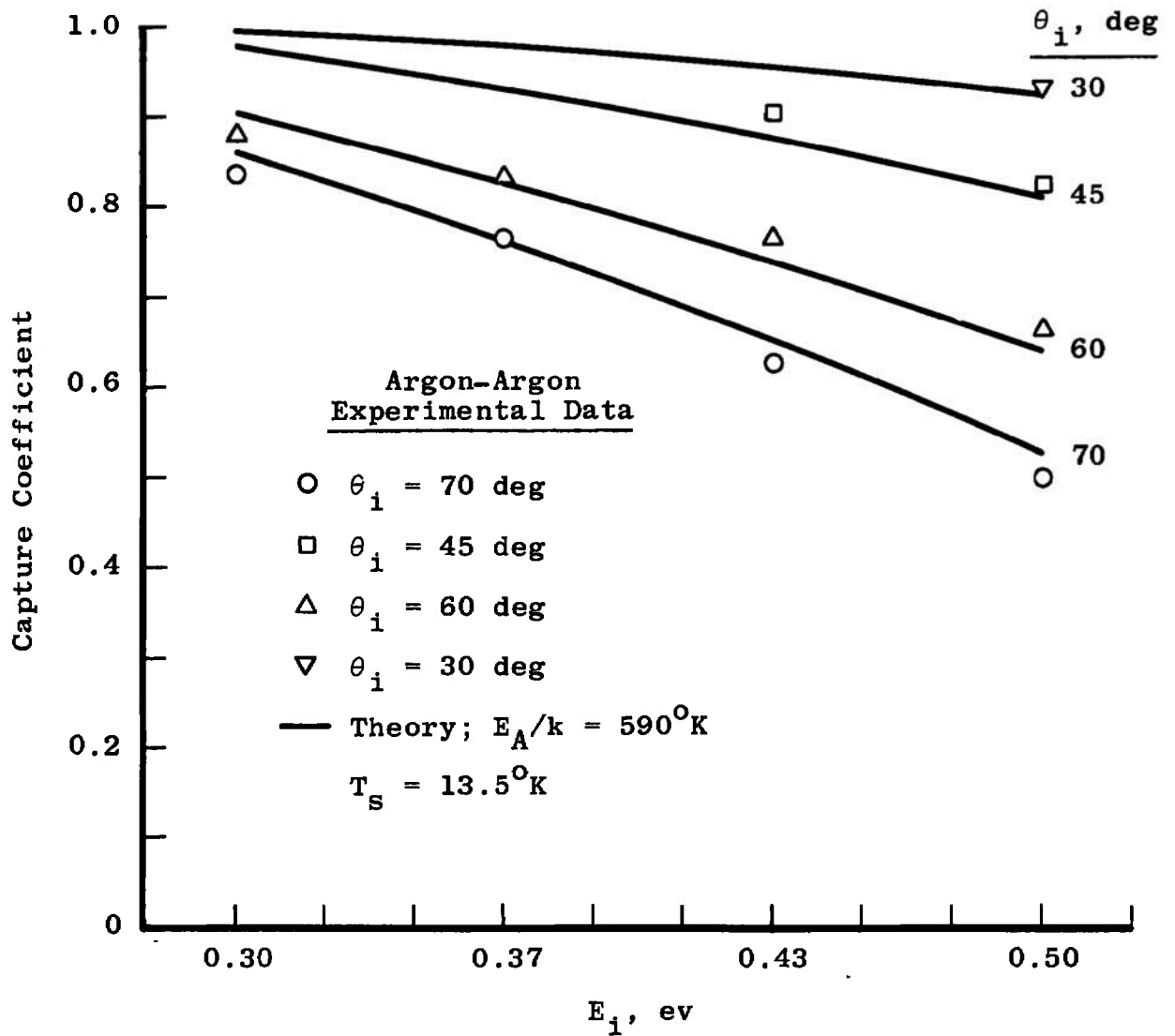
Fig. 20 Beam Capture Coefficient for Various Beam Energies—Comparison of Theory and Experiment
