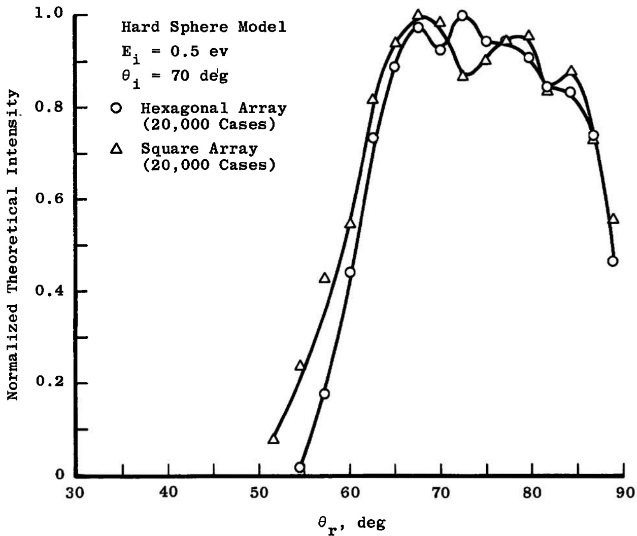
Fig. 8 Comparison of the In-Plane Normalized Spatial Distributions of the Hexagonal and Square Surface Arrays
