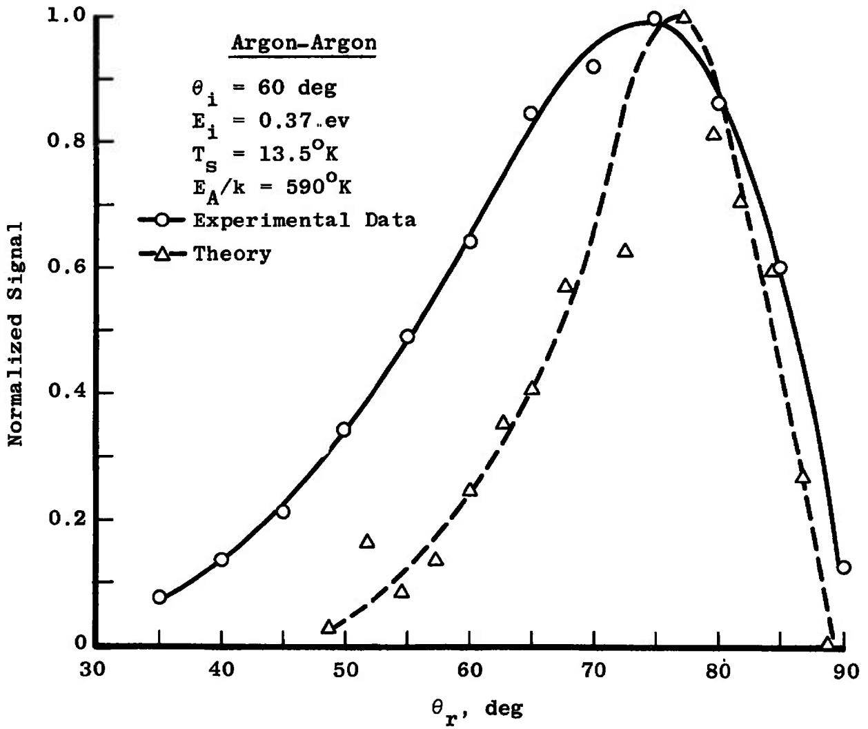
Fig. 27 Normalized In-Plane Spatial Distribution for \theta_i = 60 \text{ deg} and E_i = 0.37 \text{ ev}
