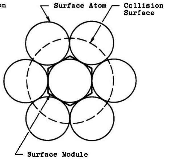
b. Hexagonal Surface Array
