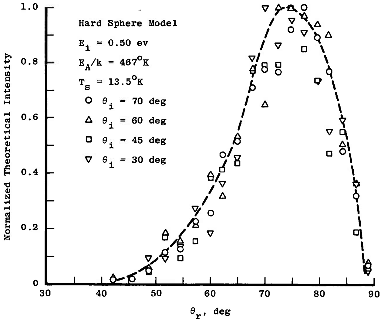
Fig. 17 In-Plane Normalized Spatial Distributions for Various Angles of Incidence
