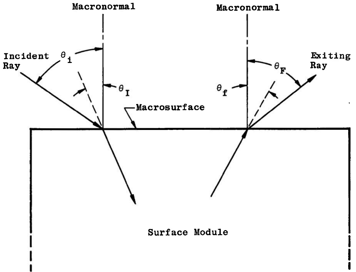
Fig. 10 Trajectory Alterations Due to a Square-Well Potential
