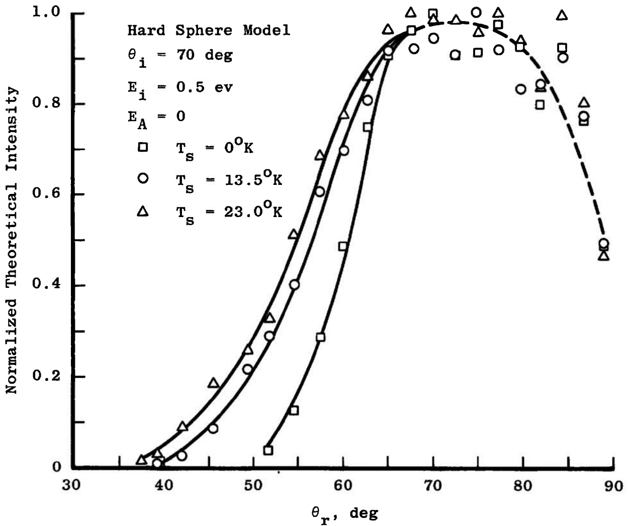
Fig. 16 In-Plane Normalized Spatial Distributions for Various Surface Temperatures
