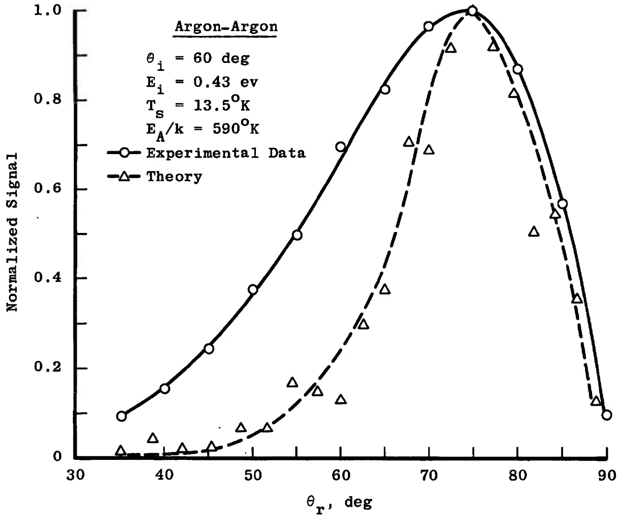
Fig. 26 Normalized In-Plane Spatial Distribution for \theta_i = 60 deg and E_i = 0.43 ev
