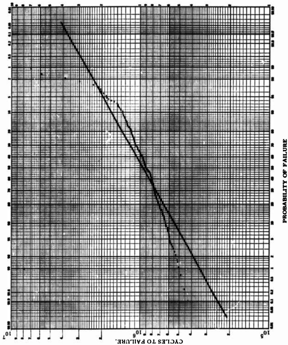
FIG. 25 LOG-NORMAL PROBABILITY PLOT. SINGLE DISTRIBUTION. BLOOMER & ROYLANCE, MACHINE-3; 245 SPECIMENS, r=0.88778 .
