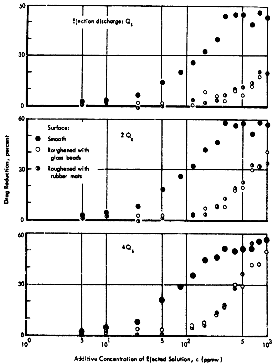
FIGURE 10 - DRAG REDUCTION BY EJECTING ADDITIVE SOLUTIONS OVER A ROUGH BOUNDARY
