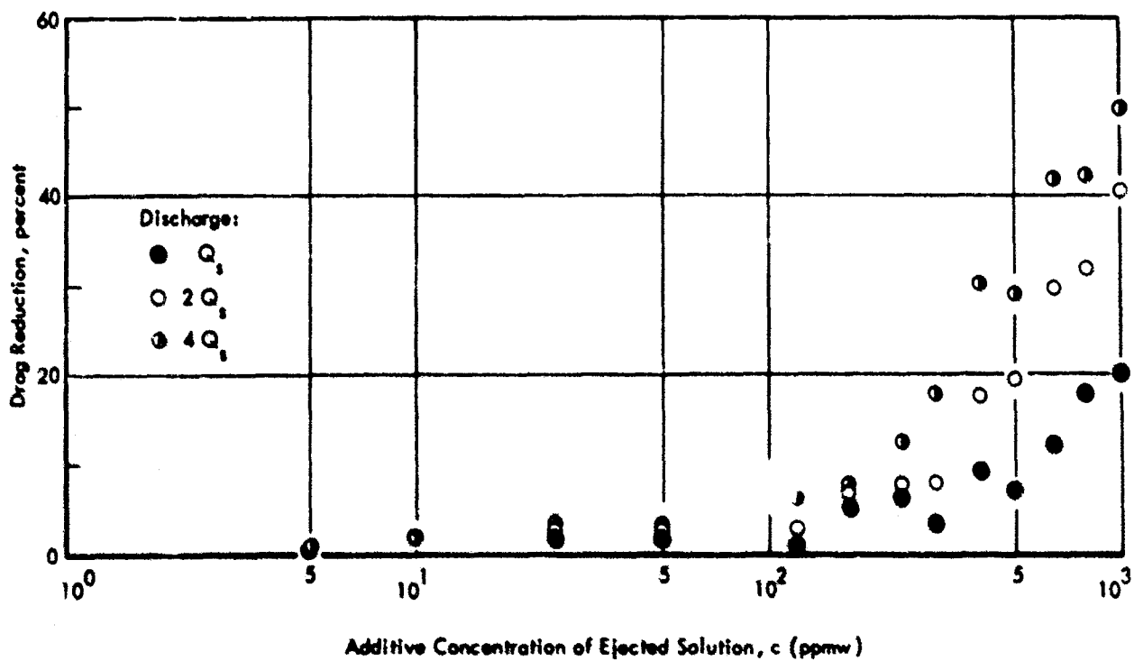
FIGURE 6 - DRAG REDUCTION BY EJECTING ADDITIVE SOLUTIONS INTO A PURE-WATER BOUNDARY LAYER OF A ROUGH SURFACE (GLASS BEADS, SLOT OPENING 0.022 INCHES)
