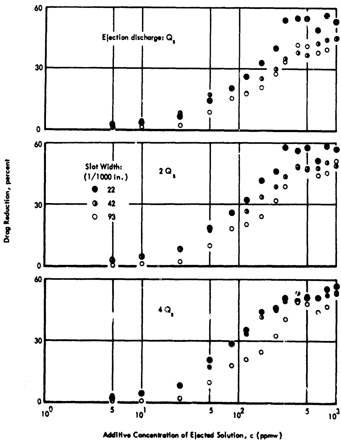
FIGURE 8 - DRAG REDUCTION BY EJECTED ADDITIVE SOLUTIONS OVER A SMOOTH BOUNDARY
