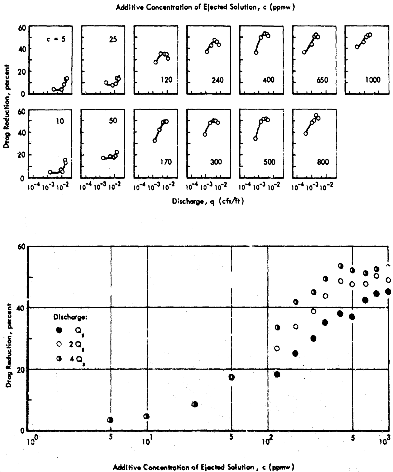
FIGURE 4 - DRAG REDUCTION BY EJECTING ADDITIVE SOLUTIONS INTO A PURE-WATER BOUNDARY LAYER OF A SMOOTH SURFACE ( SLOT OPENING 0.042 INCHES )
