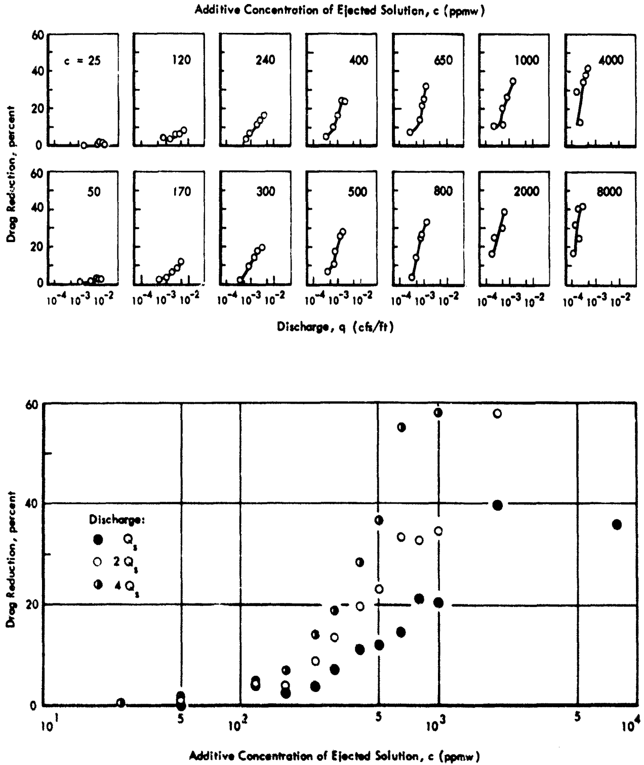
FIGURE 7 - DRAG REDUCTION BY EJECTING ADDITIVE SOLUTIONS INTO A PURE-WATER BOUNDARY LAYER OF A ROUGH SURFACE ( RUBBER MATS, SLOT OPENING 0.022 INCHES )
