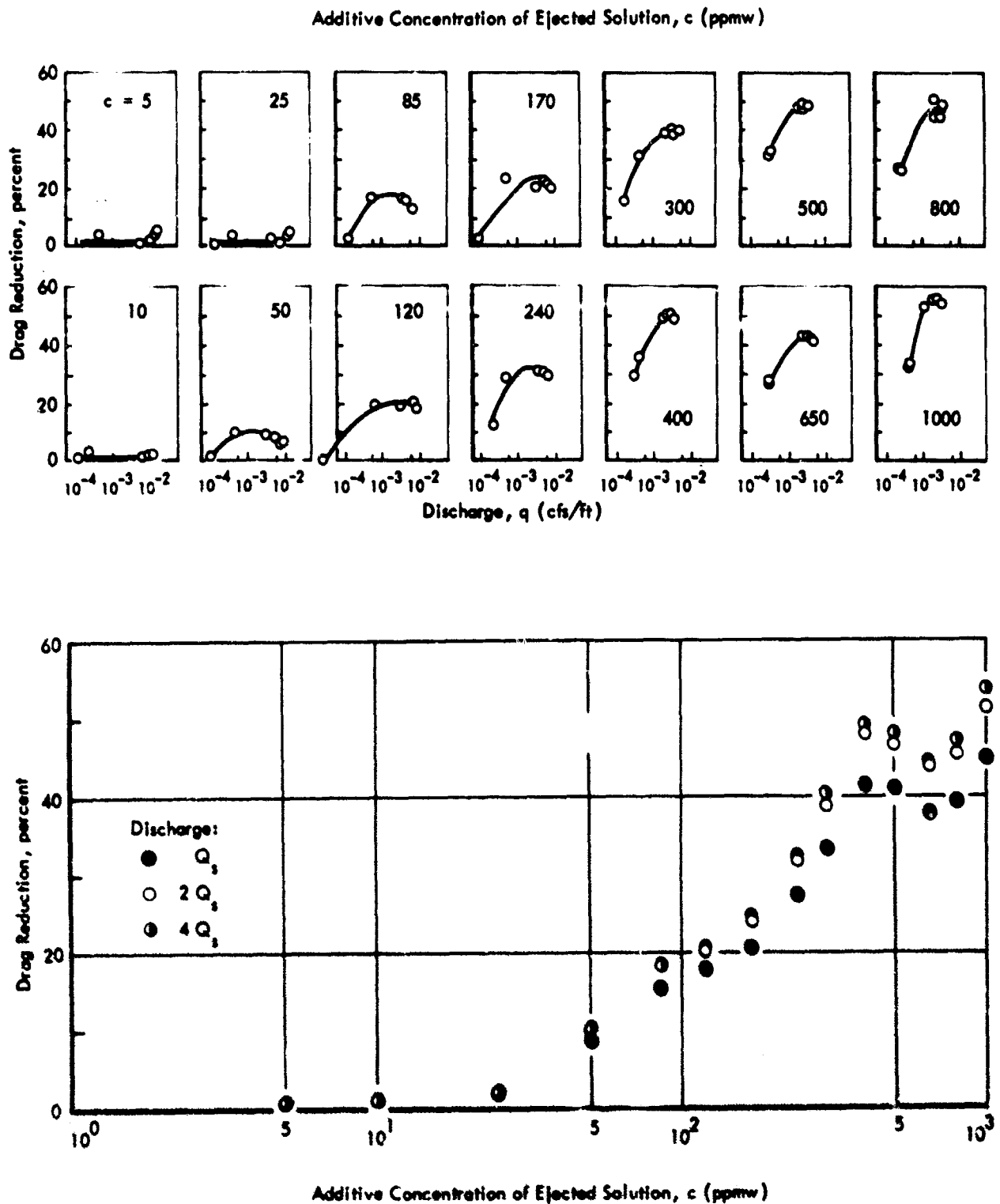
FIGURE 5 - DRAG REDUCTION BY EJECTING ADDITIVE SOLUTIONS INTO A PURE-WATER BOUNDARY LAYER OF A SMOOTH SURFACE (SLOT OPENING 0.093 INCHES)
