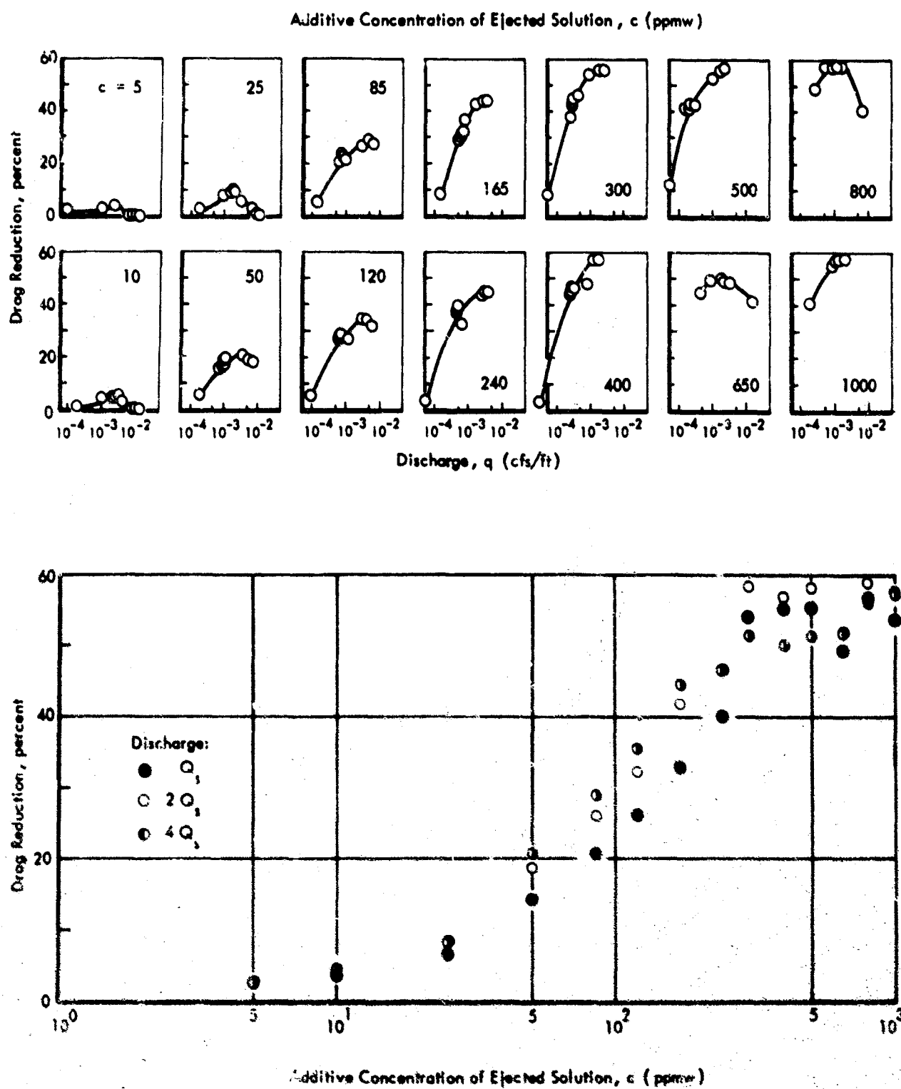
FIGURE 3 - DRAG REDUCTION BY EJECTING ADDITIVE SOLUTIONS INTO A PURE-WATER BOUNDARY LAYER OF A SMOOTH SURFACE (SLOT OPENING 0.022 INCHES)
