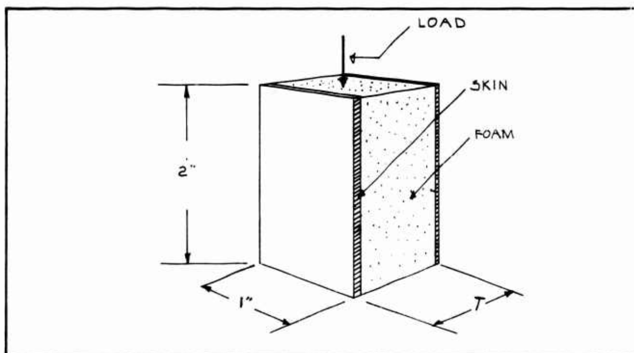
Figure 152. Typical Compression Test Specimen
