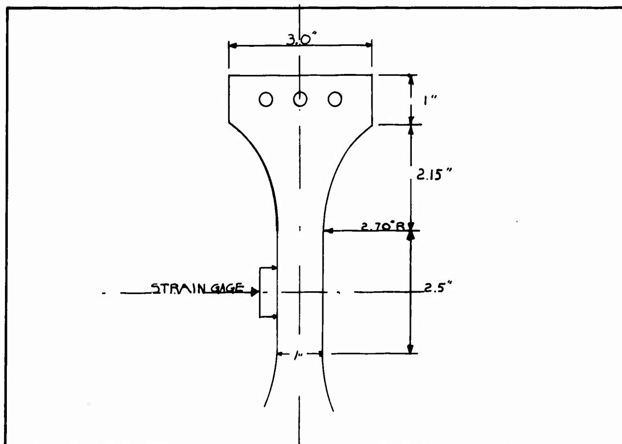
Figure 151. Typical Tension Test Specimen
