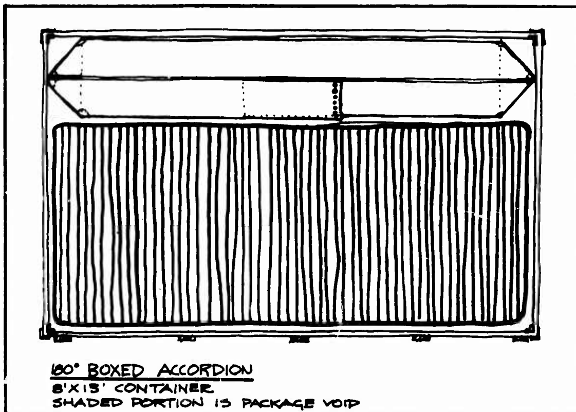
Figure 2. Shelter Folding Configuration (180°)
