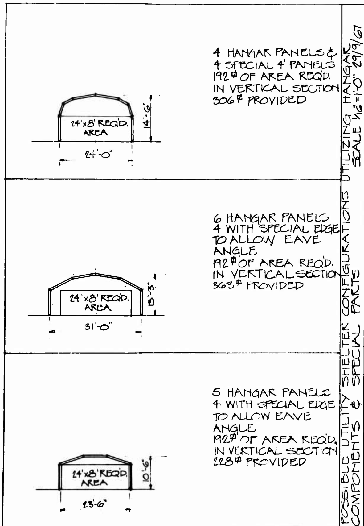
Figure 105. Possible Shelter Configurations - Special Components
