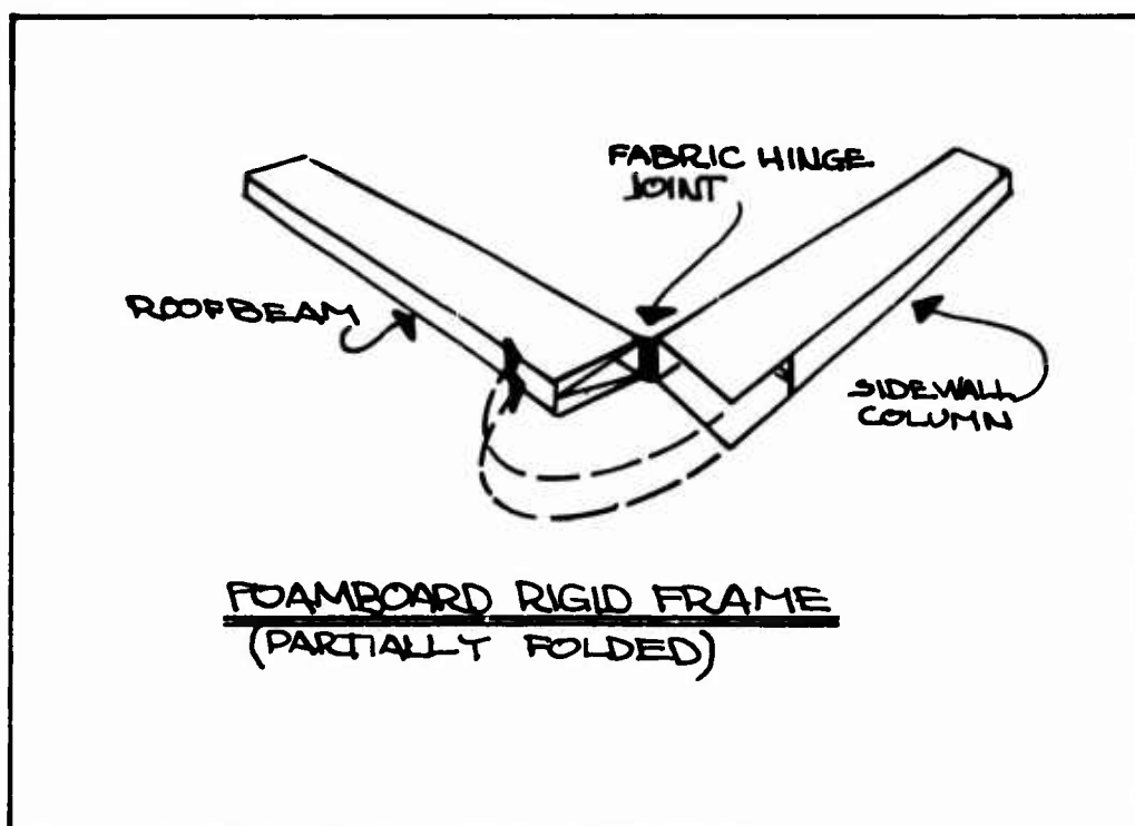
Figure 92. Rigid Frame Elements
