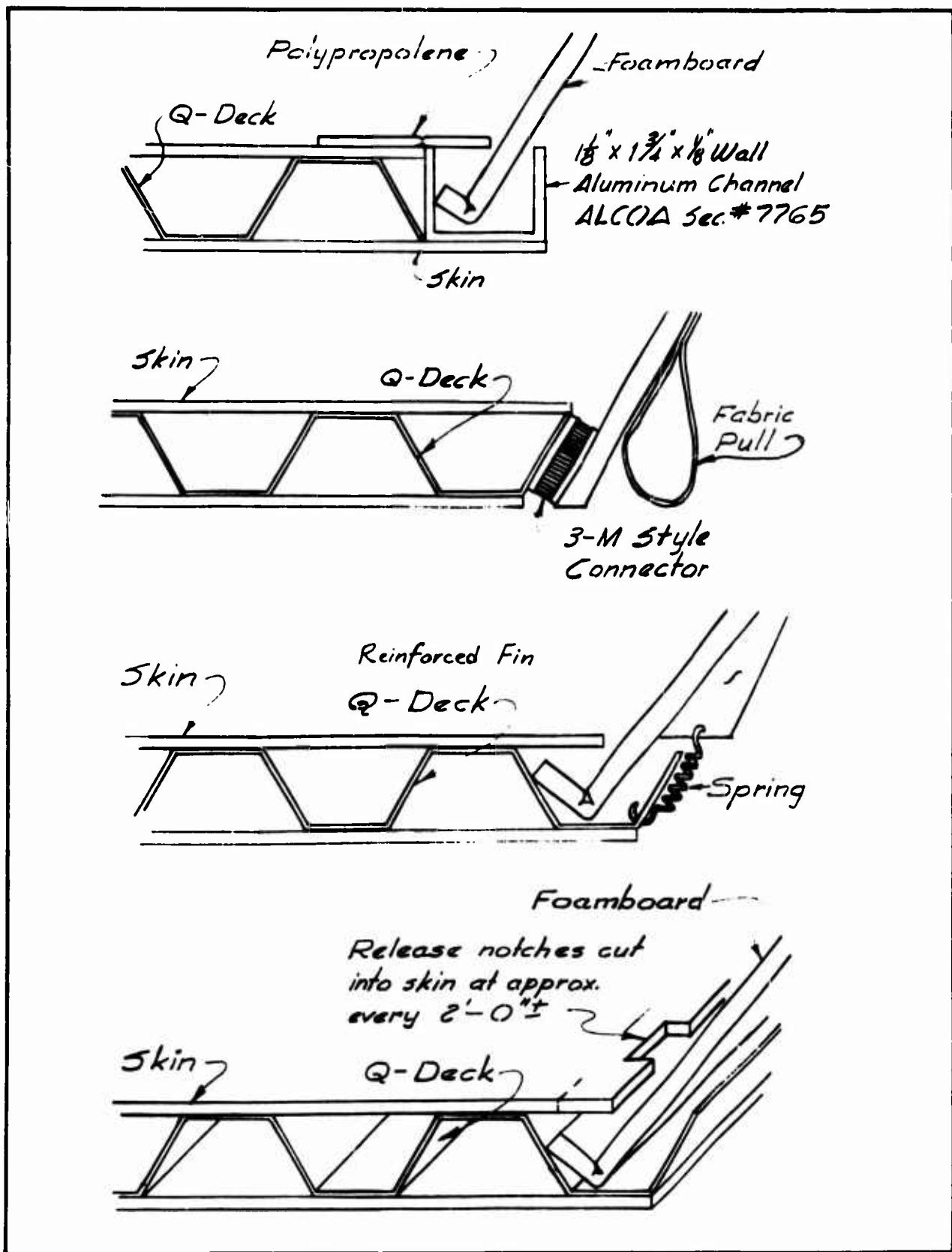
Figure 39. Foamboard Shell-to-Floor Edge; Attachment Variations
