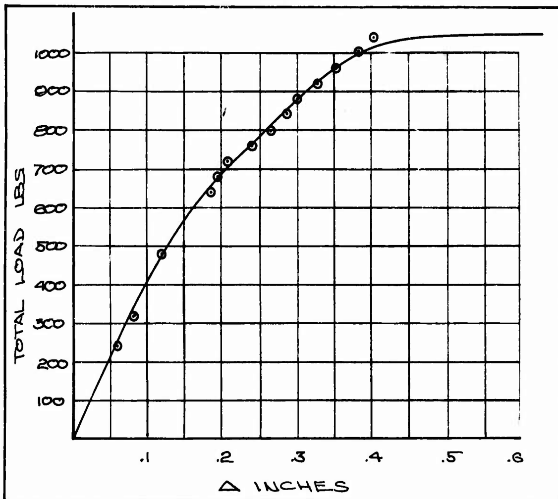
Figure 118. Load-Deflection Curve for 48" Span (Unstrapped)
