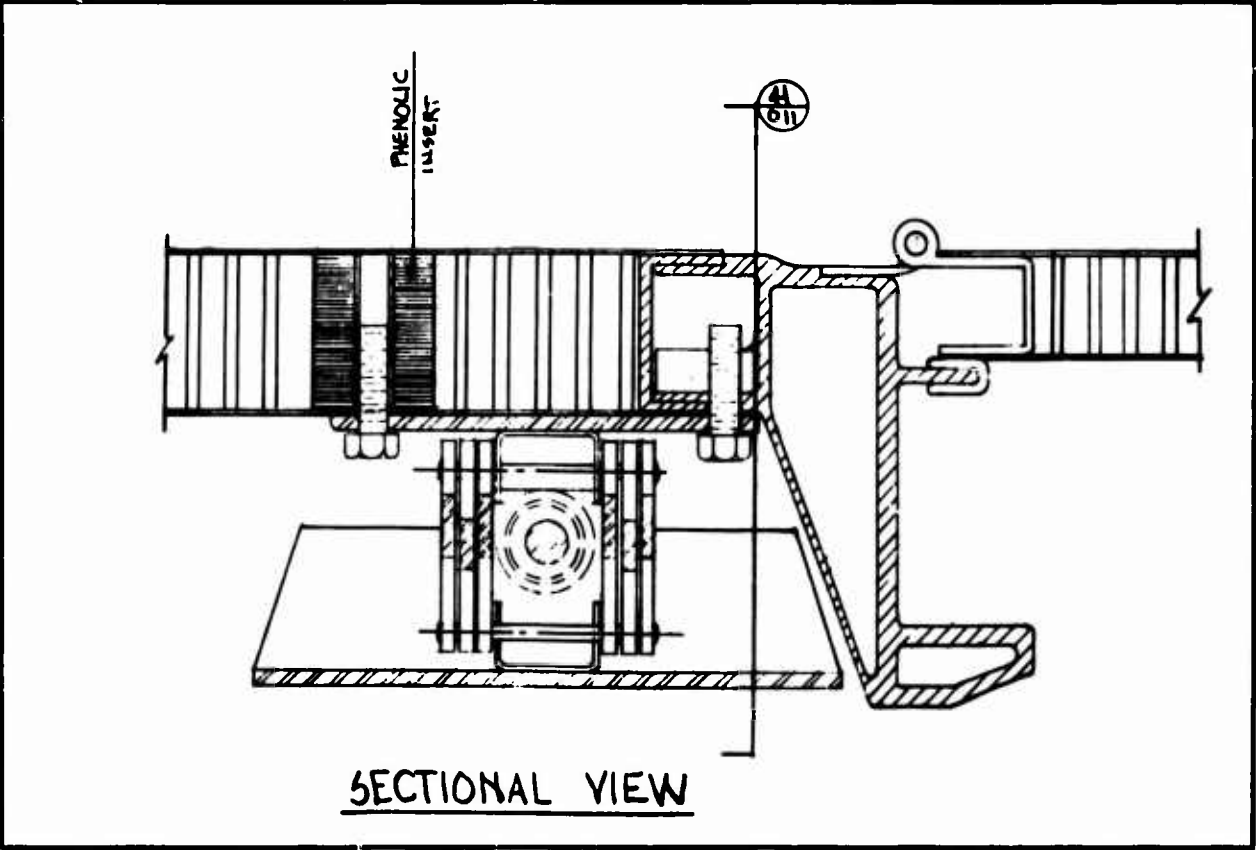
Figure 80. Support Jack at Center Section
