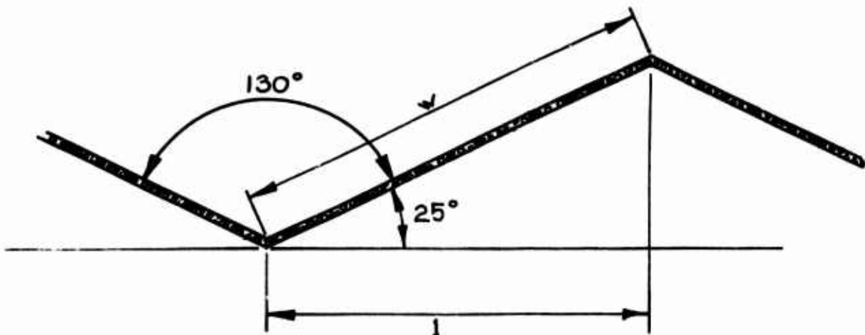
Figure 37. Basic Foamboard Geometry
