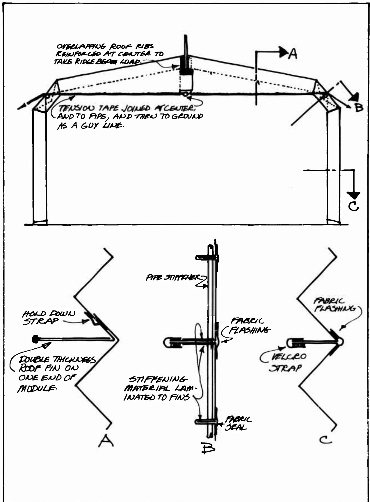
Figure 24. LES Joints and Reinforcement
