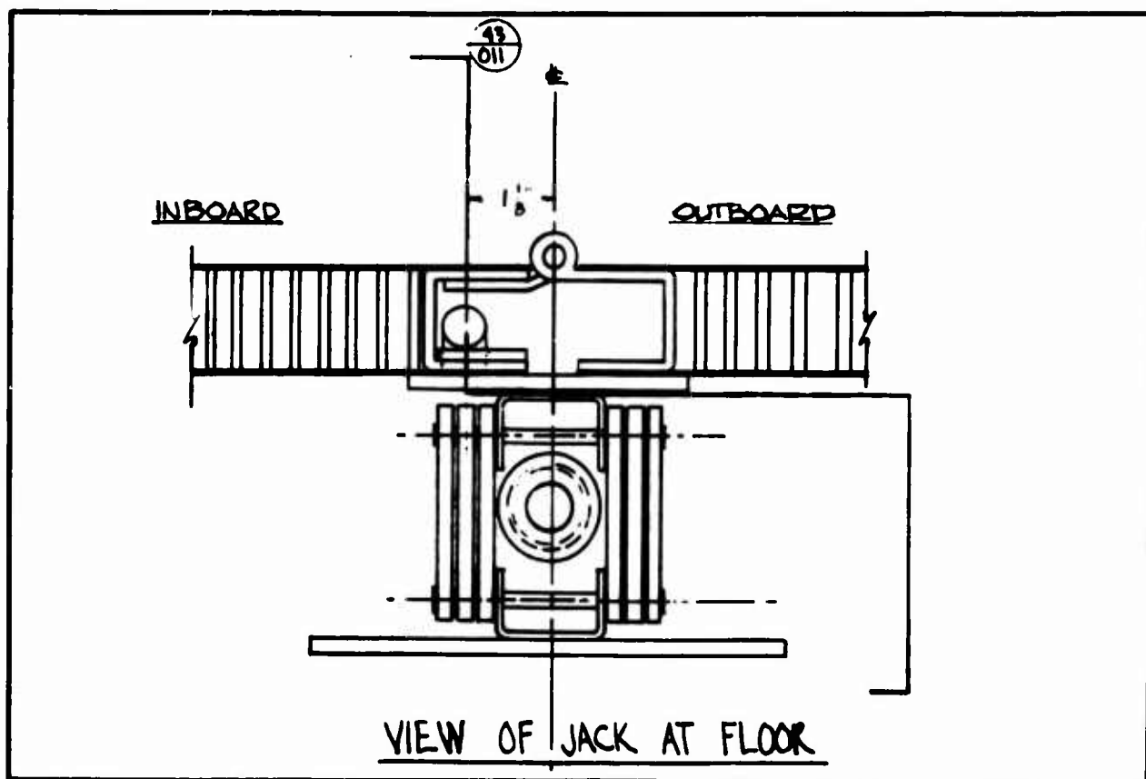
Figure 78. Support Jacks between Floor Segments
