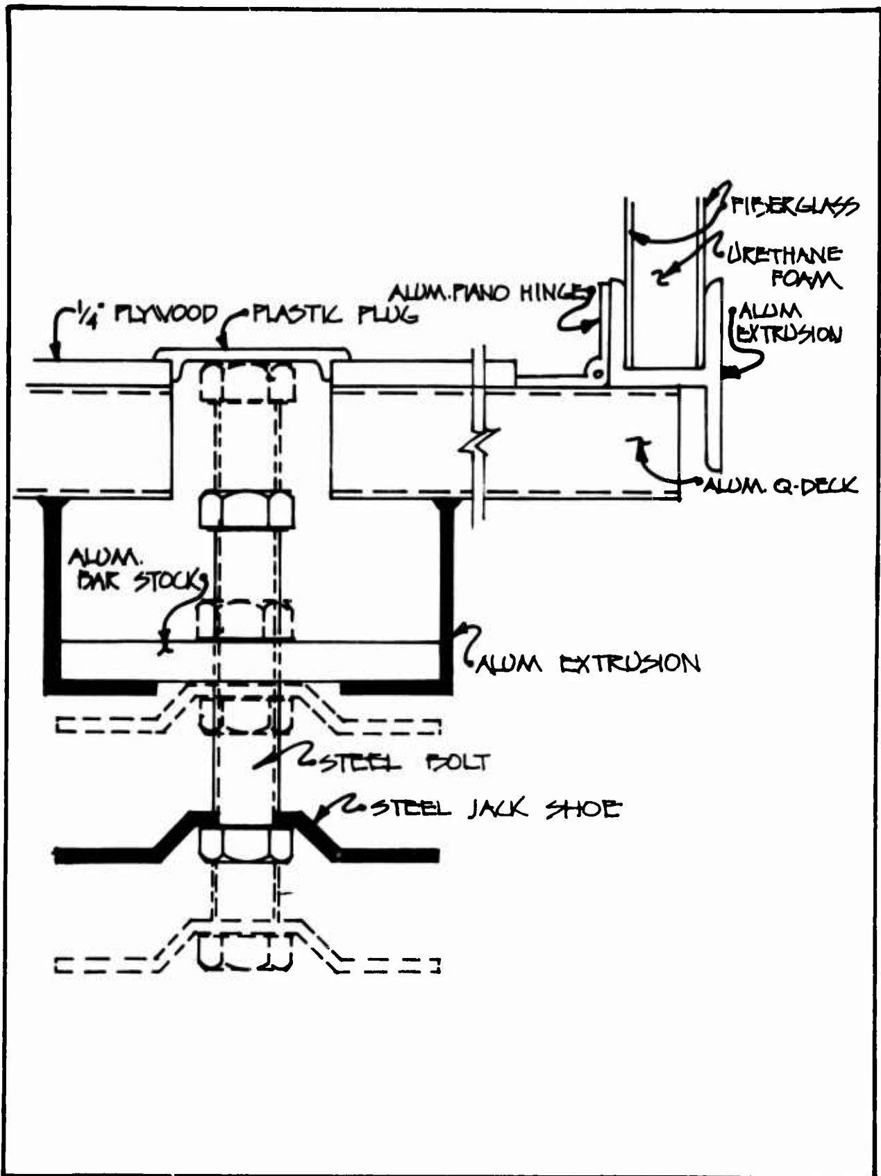
Figure 49. Floor Leveling Jack at Endwall
