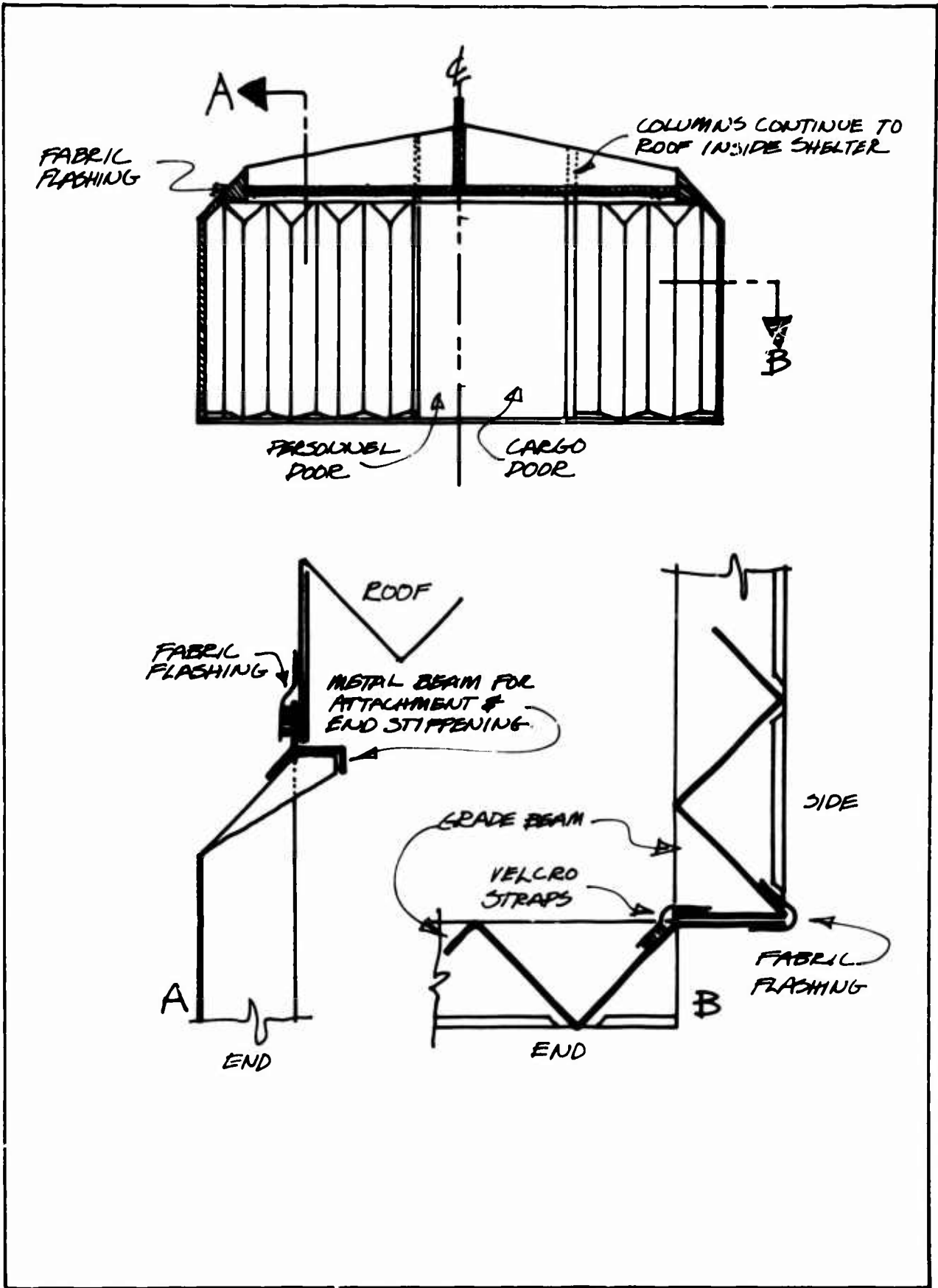
Figure 23. LES Alternate Endwall Details
