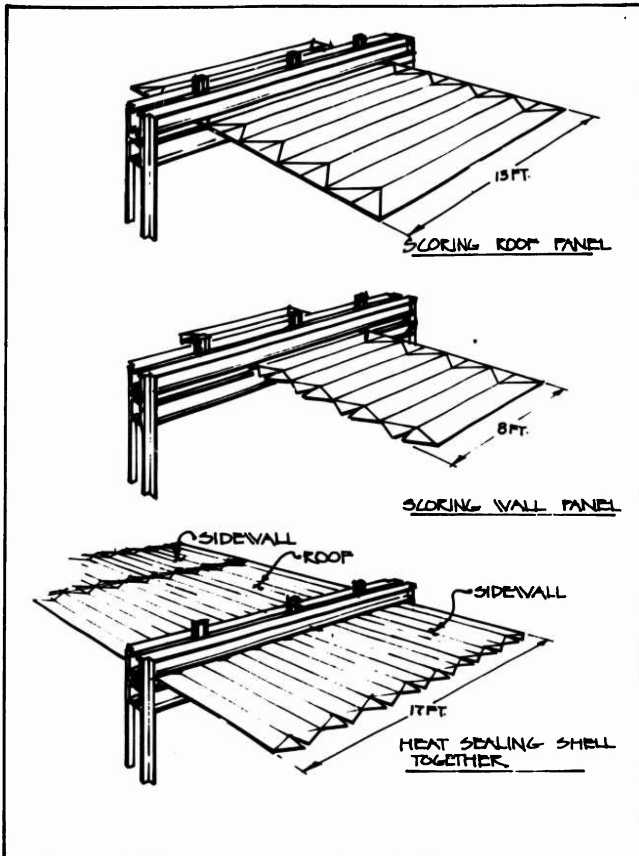
Figure 43. Manufacturing Stages in Foamboard Shell Production
