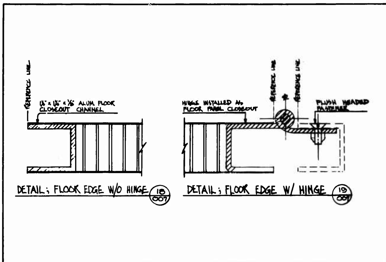
Figure 82. Floor Edge at Hinge Lines
