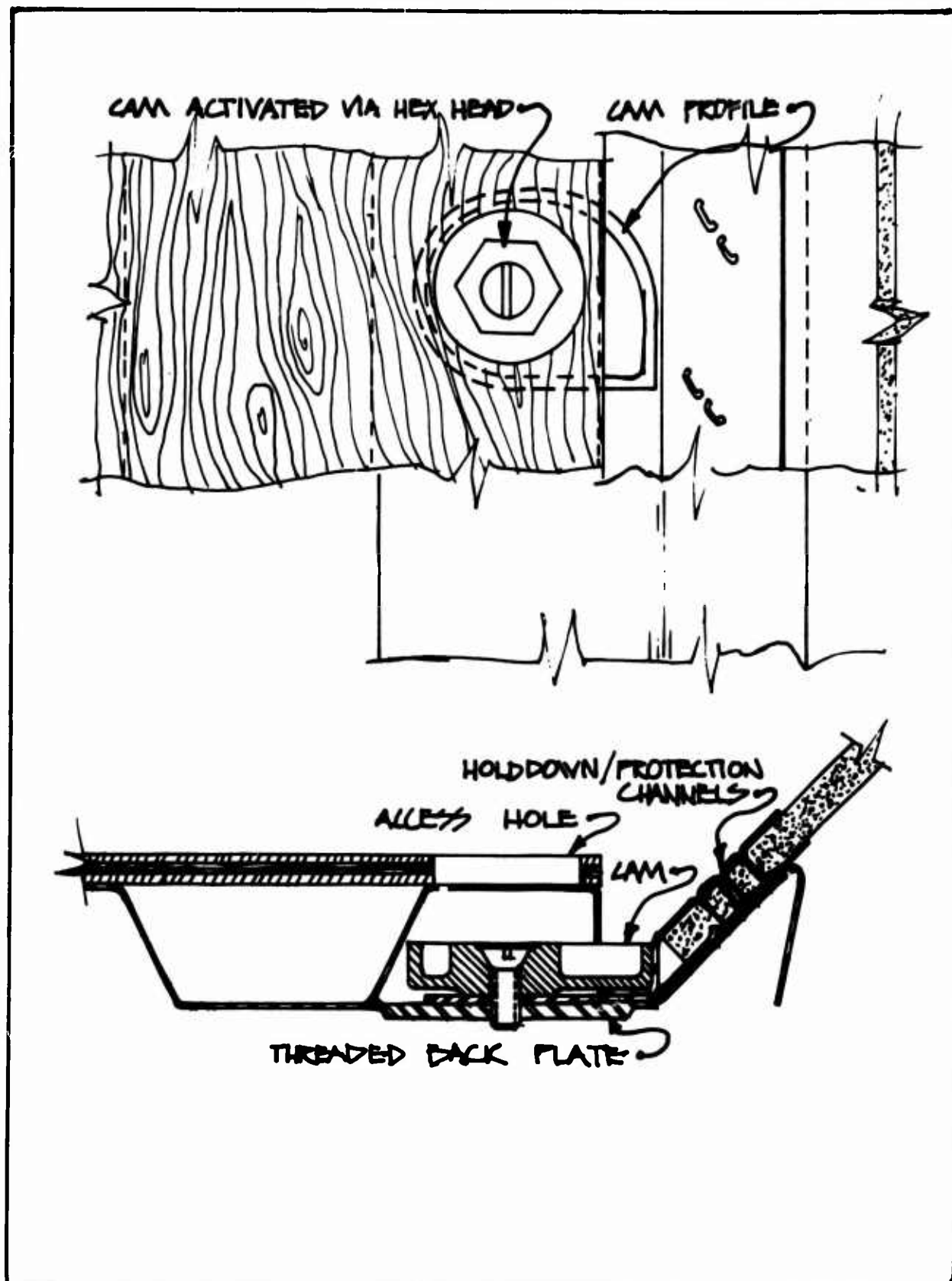
Figure 48. Foamboard Shell to Floor Connection
