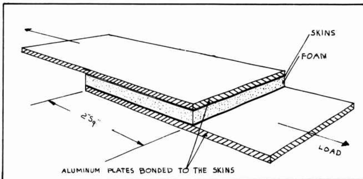
Figure 154. Typical Bond Test Specimen
