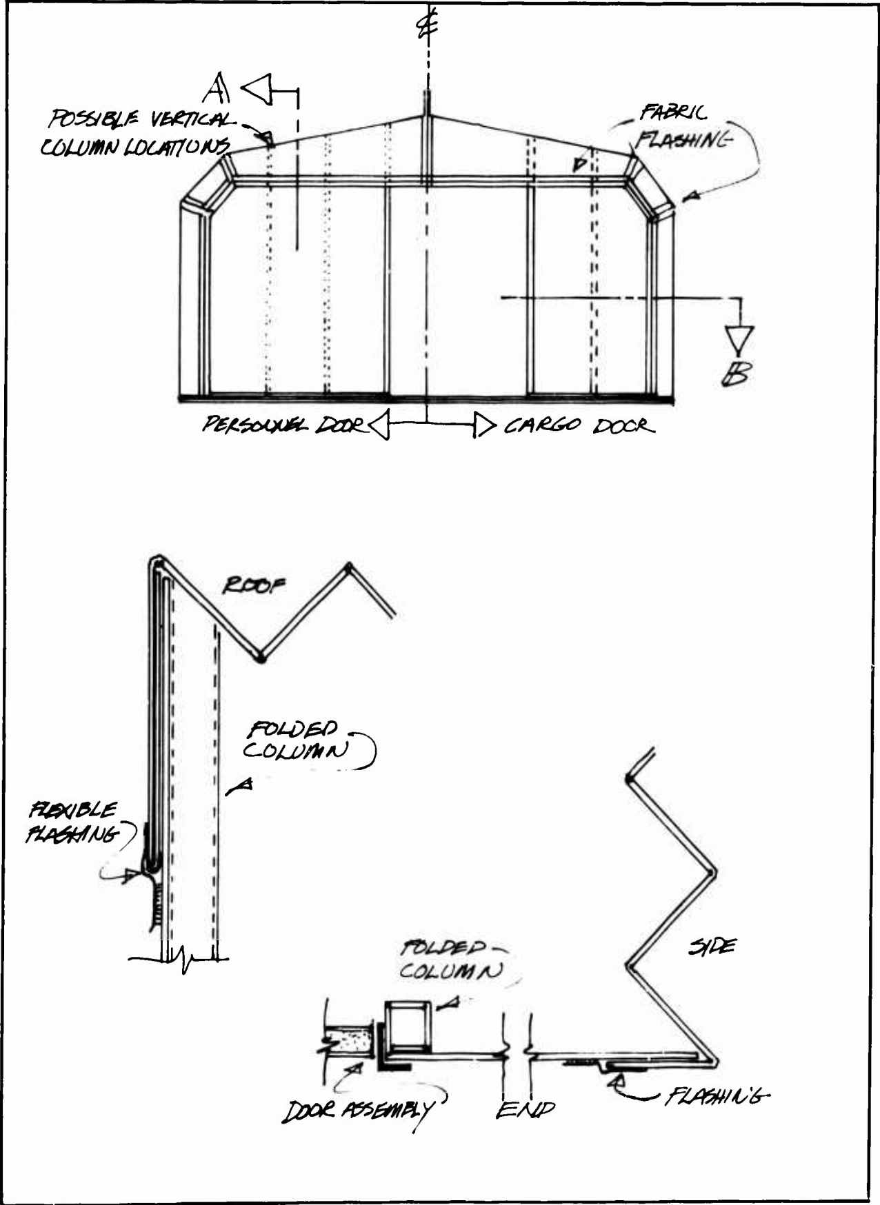
Figure 22. LES Endwall Framing Details
