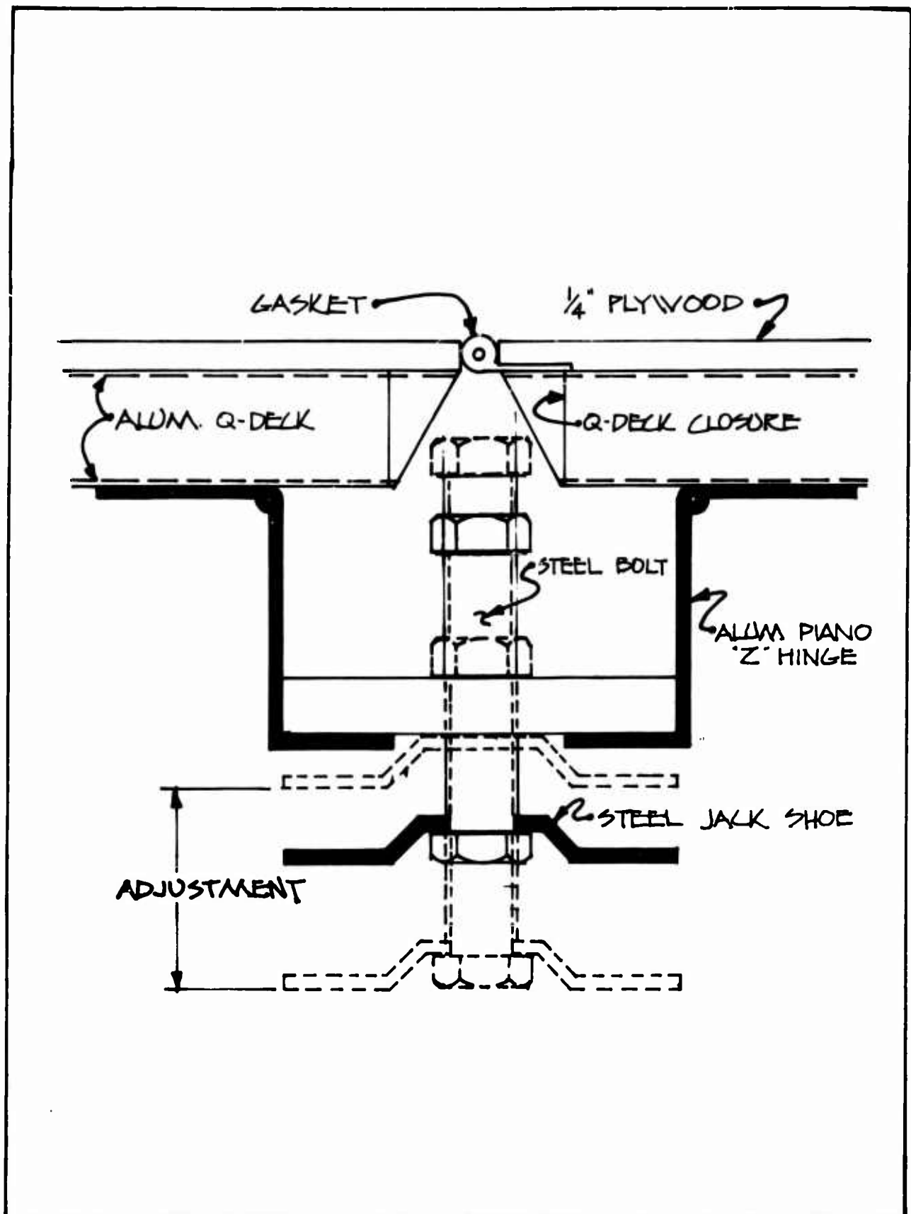
Figure 50. Floor Leveling Jack Between Floor Segments
