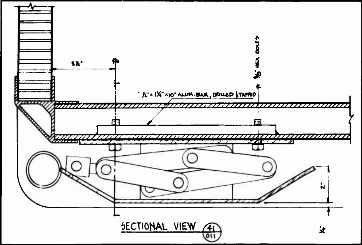
Figure 81. Support Jack at Center Section
