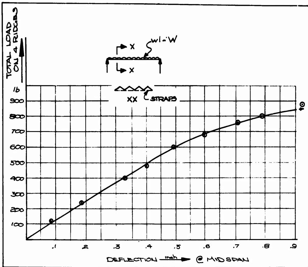
Figure 119. Load-Deflection Curve for 74' Span (Strapped)
