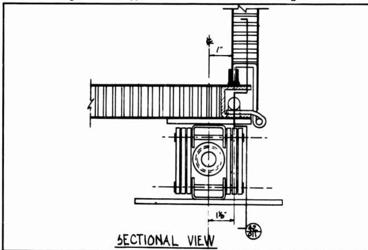
Figure 79. Support Jacks at Endwalls
