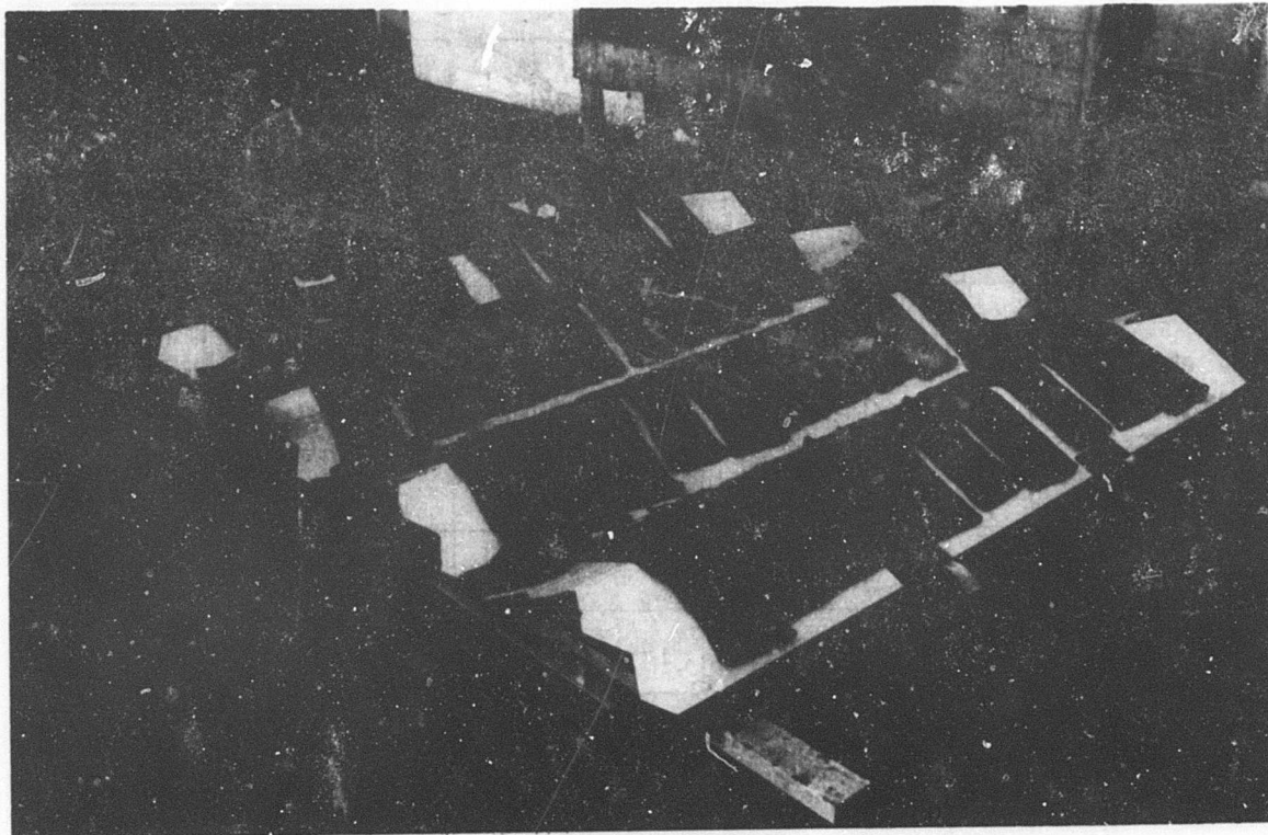
Figure 115. View of Static Test Setup
