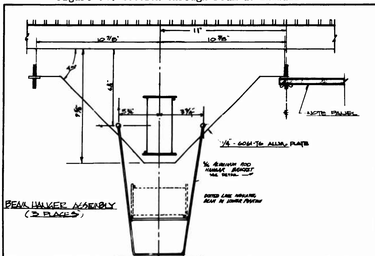
Figure 85. Beam Hanger Assembly
