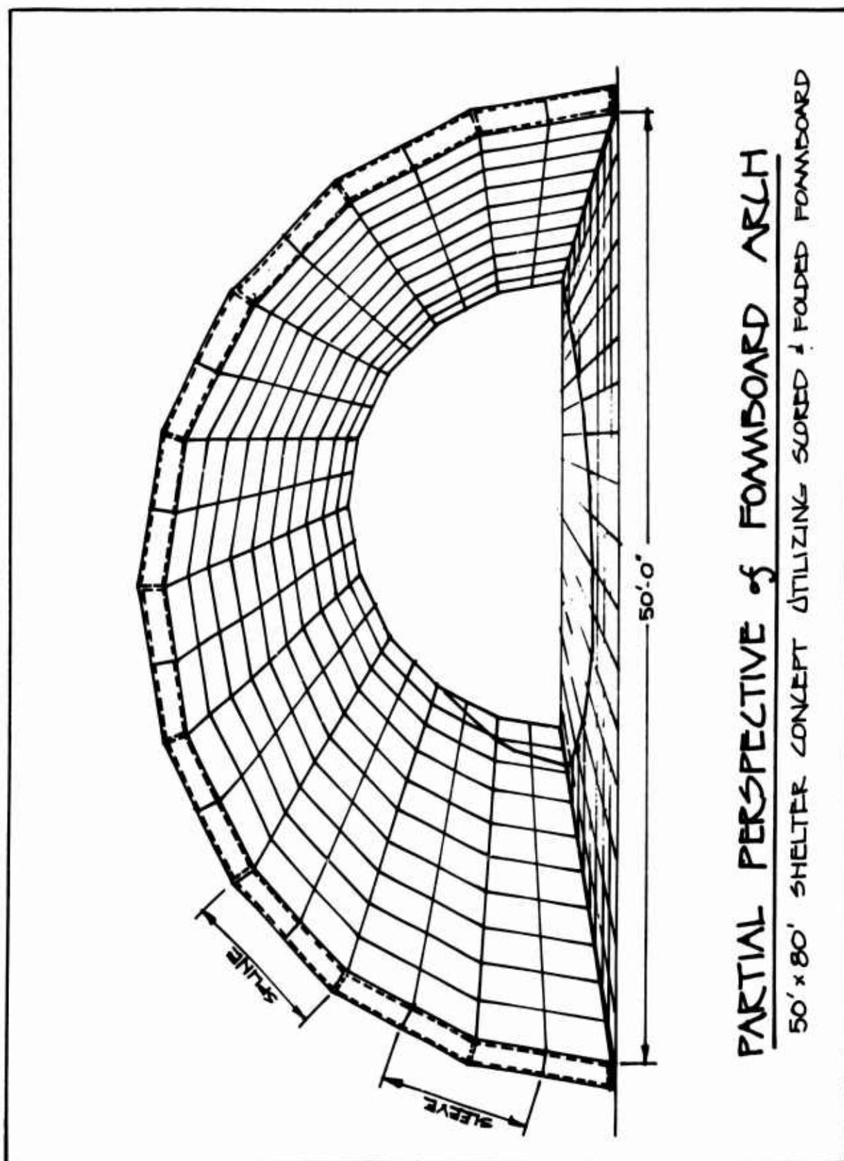
Figure 14. Partial Perspective of Foamboard Arch (50' span)
