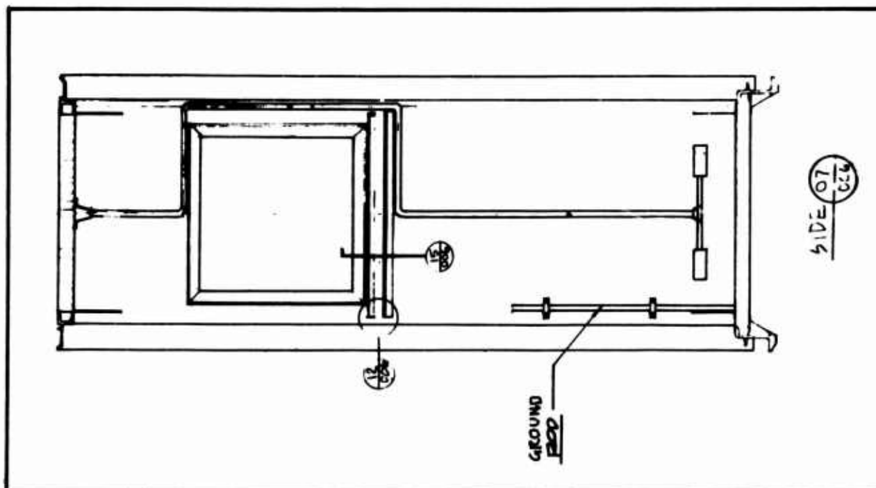
Figure 86. Container Interior (Utility Opening End)
