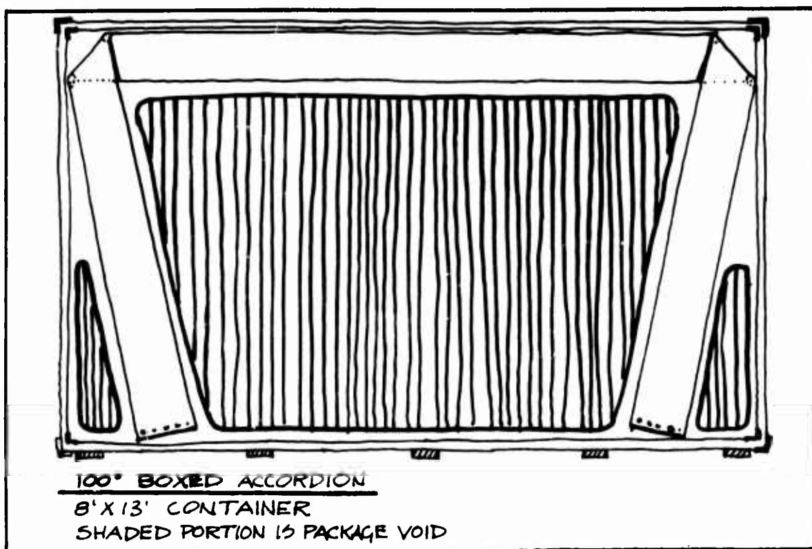
Figure 3. Shelter Folding Configuration (100°)
