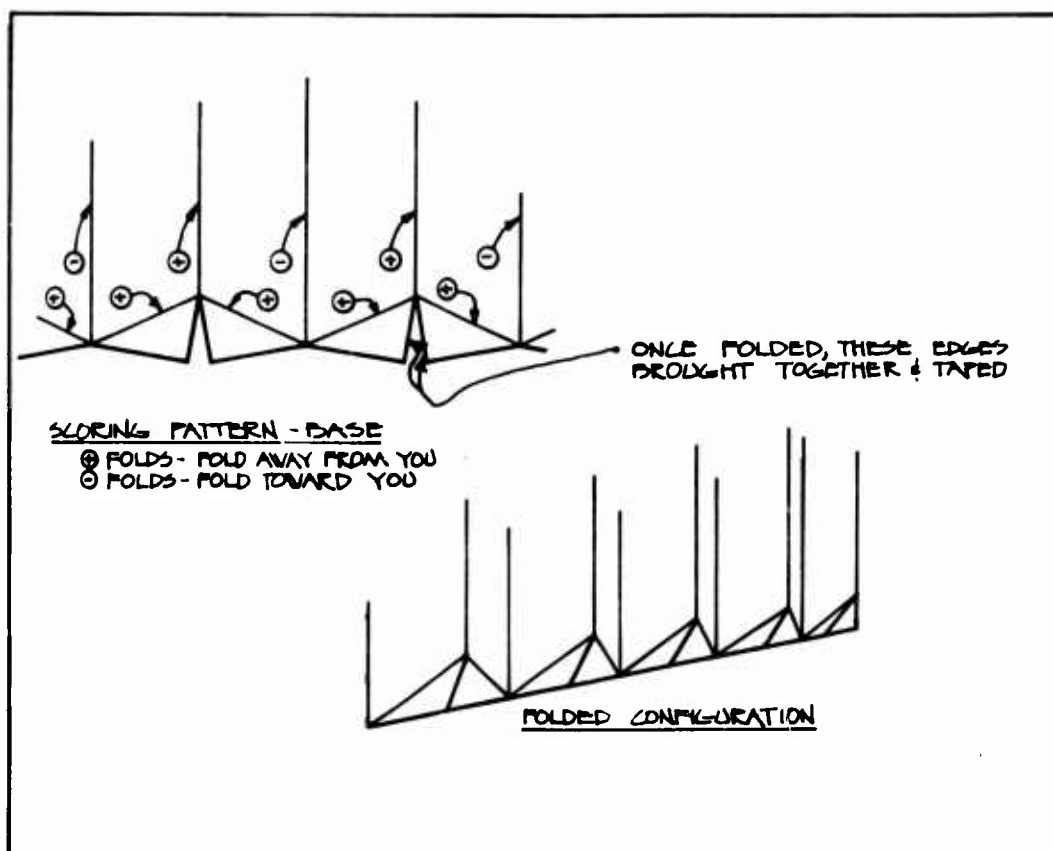
Figure 31. Foamboard Shell Base - Scoring and Folding
