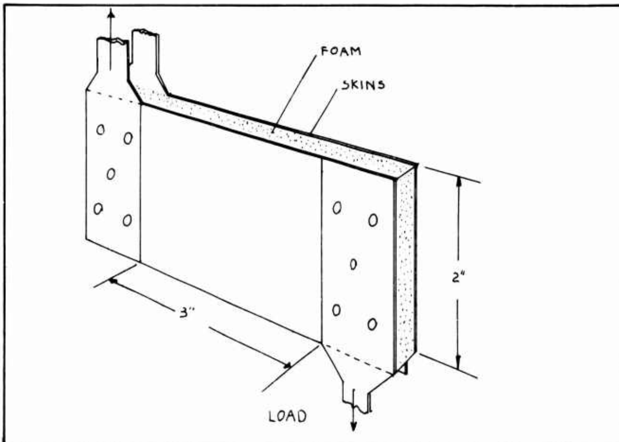
Figure 153. Typical Shear Test Specimen
