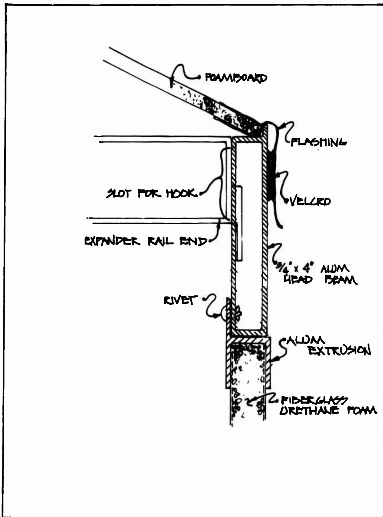
Figure 47. Foamboard Shell to Endwall Connection
