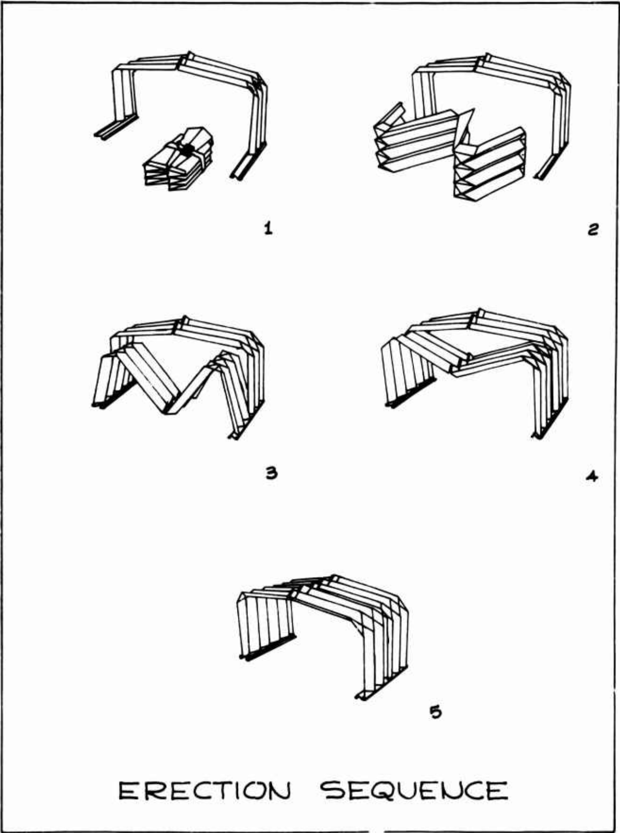
Figure 21. LES Erection Sequence
