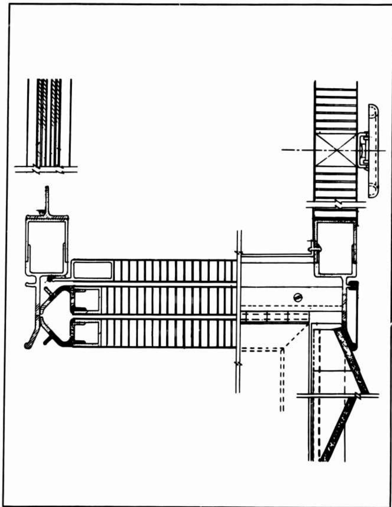
Figure 76. Horizontal Section Through Container
