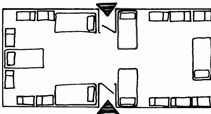
16'x35' SIDE ENTRANCE PERSONNEL SHELTER 12 MEN (TWO SCHEMES SHOWN)
