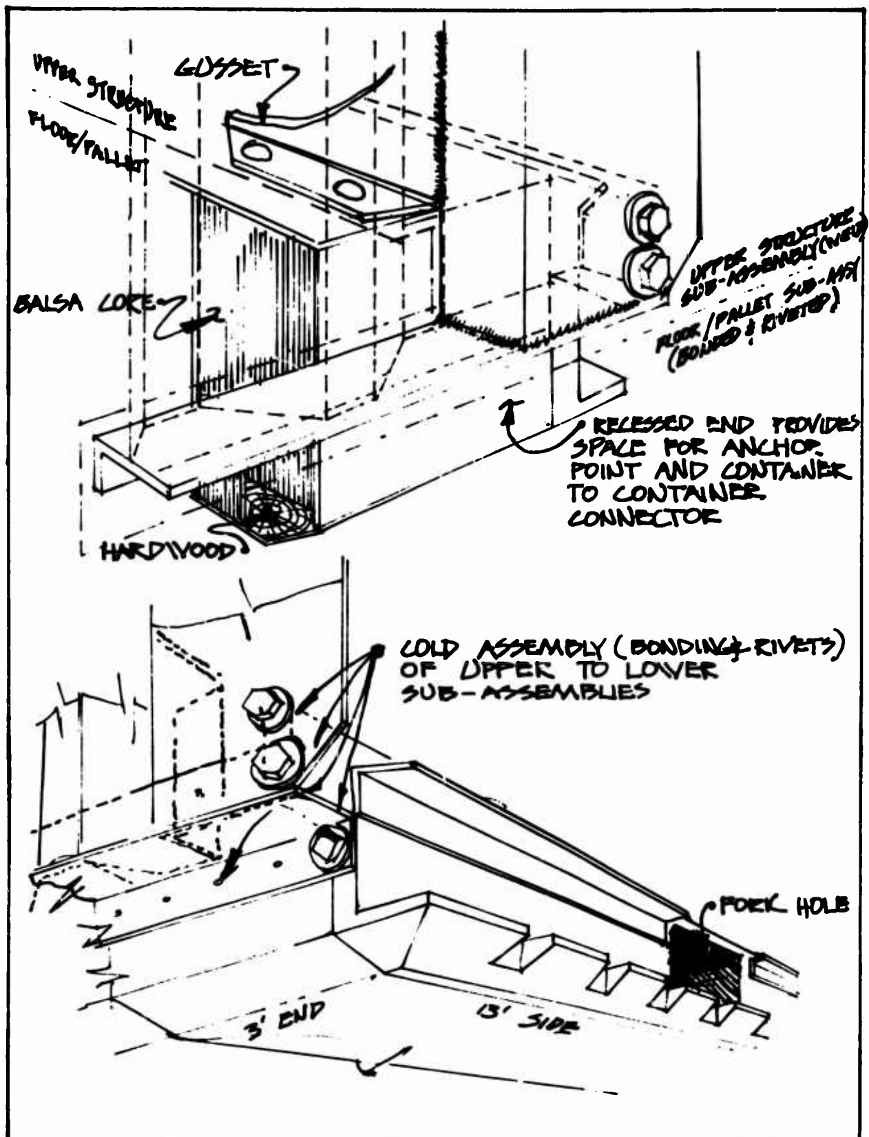
Figure 45. Center-Section Corner Assembly Details
