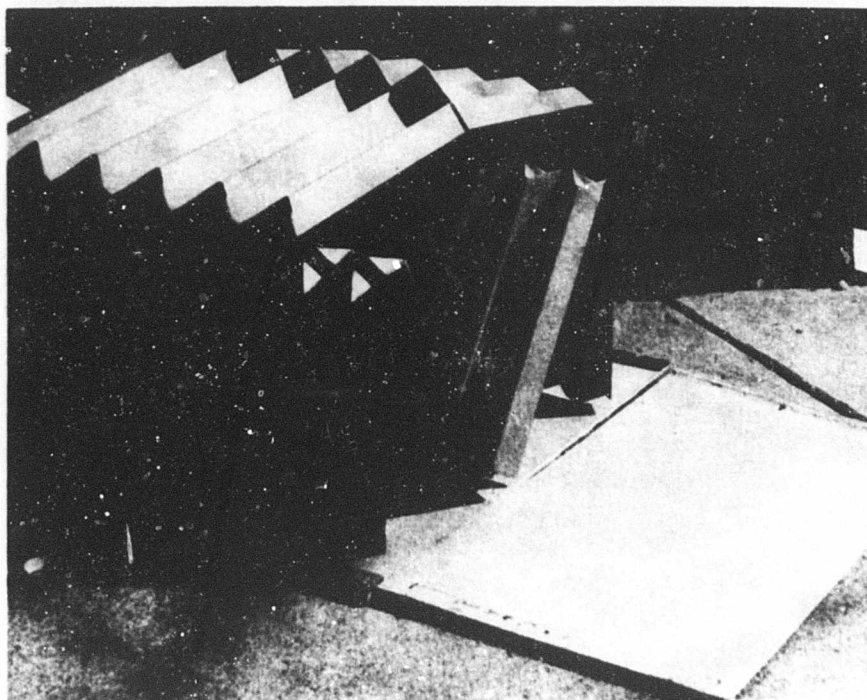
Figure 18. Partially Erected LES Concept
