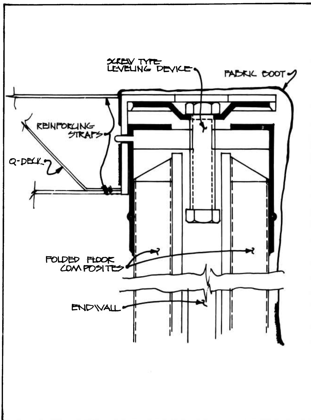
Figure 51. Folded Floors in Container Mode
