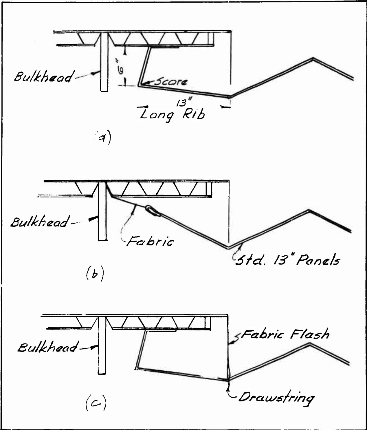
Figure 38. Foamboard Shell-to-Container Bulkhead; Attachment Variations
