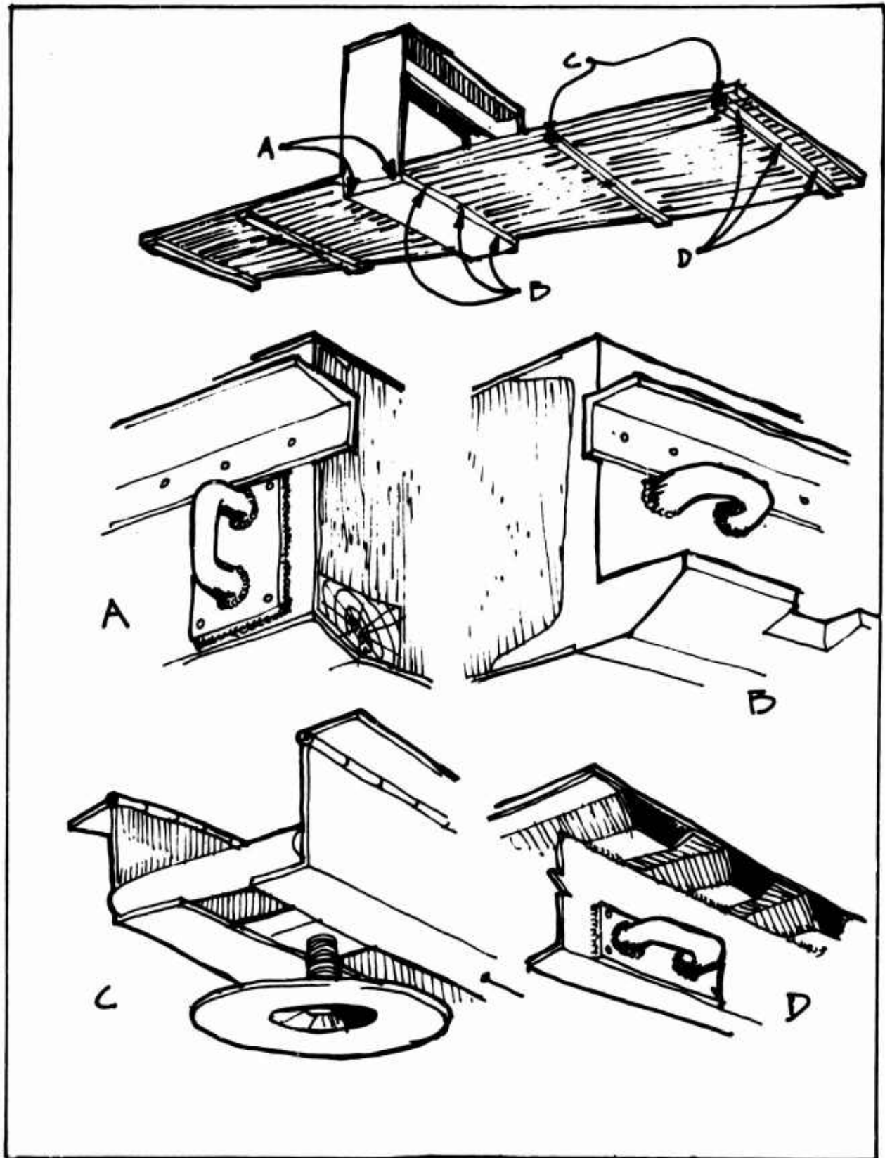
Figure 46. Shelter Anchoring Locations and Ties
