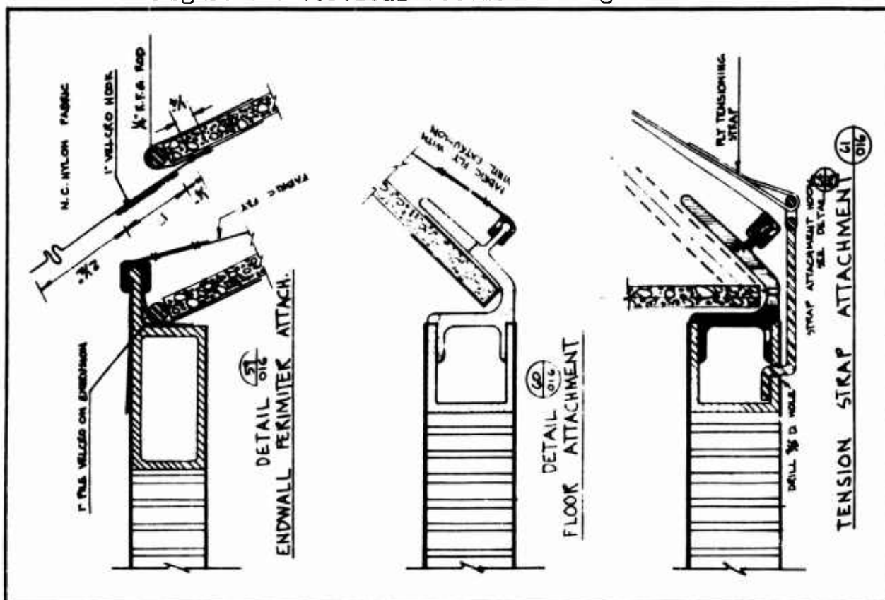
Figure 89. Attachment Details for Auxiliary Fly Cover
