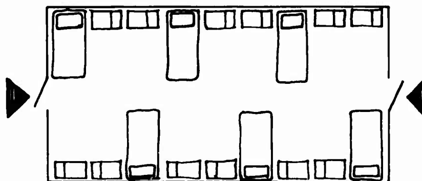
16'x32' PERSONNEL SHELTER 12 MEN.
