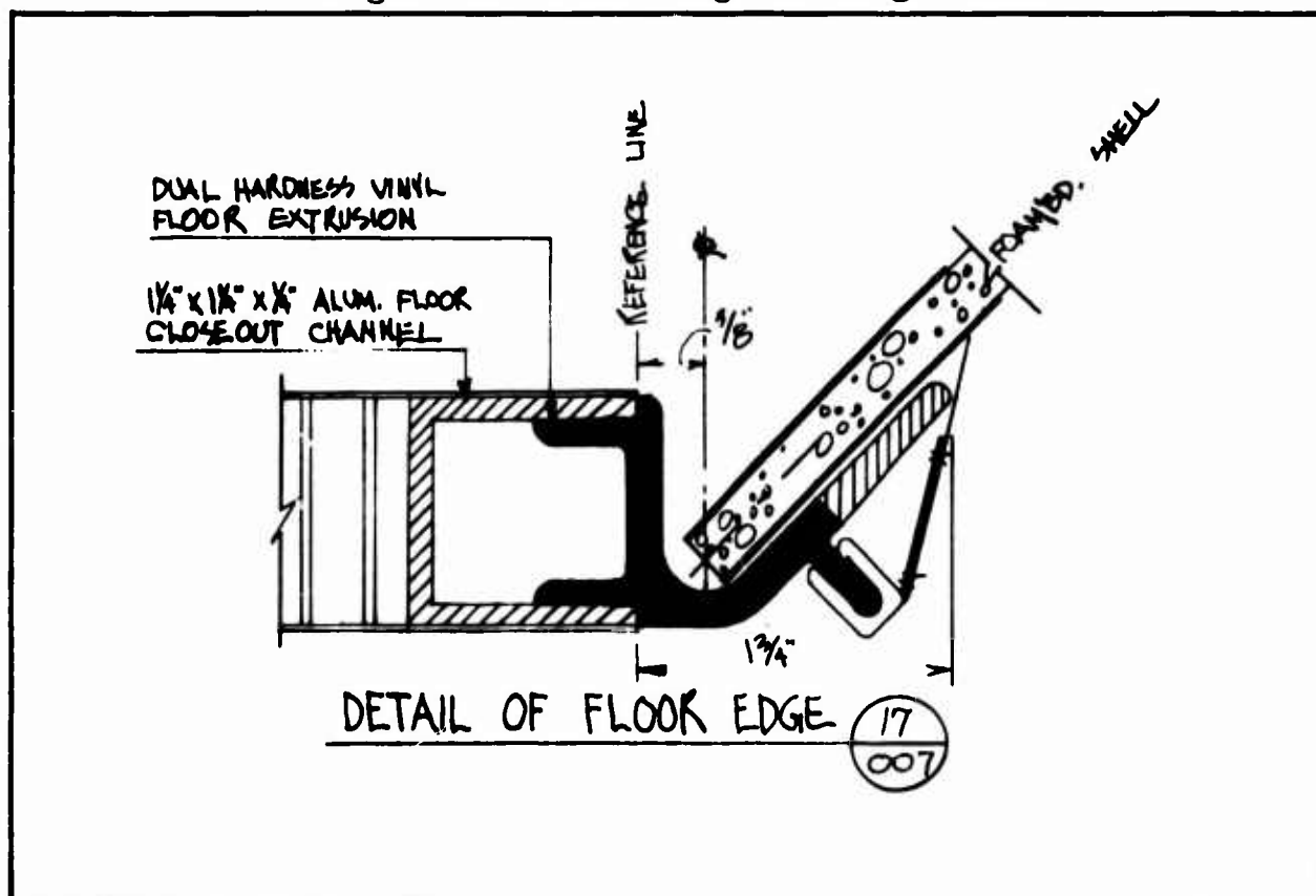
Figure 83. Floor Edge to Foamboard Sidewall Joint
