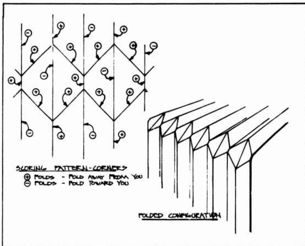
Figure 30. Foamboard Shell Knee Joint - Scoring and Folding
