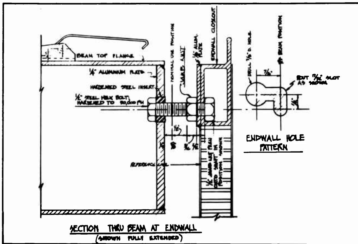
Figure 84. Section through Beam at Endwall
