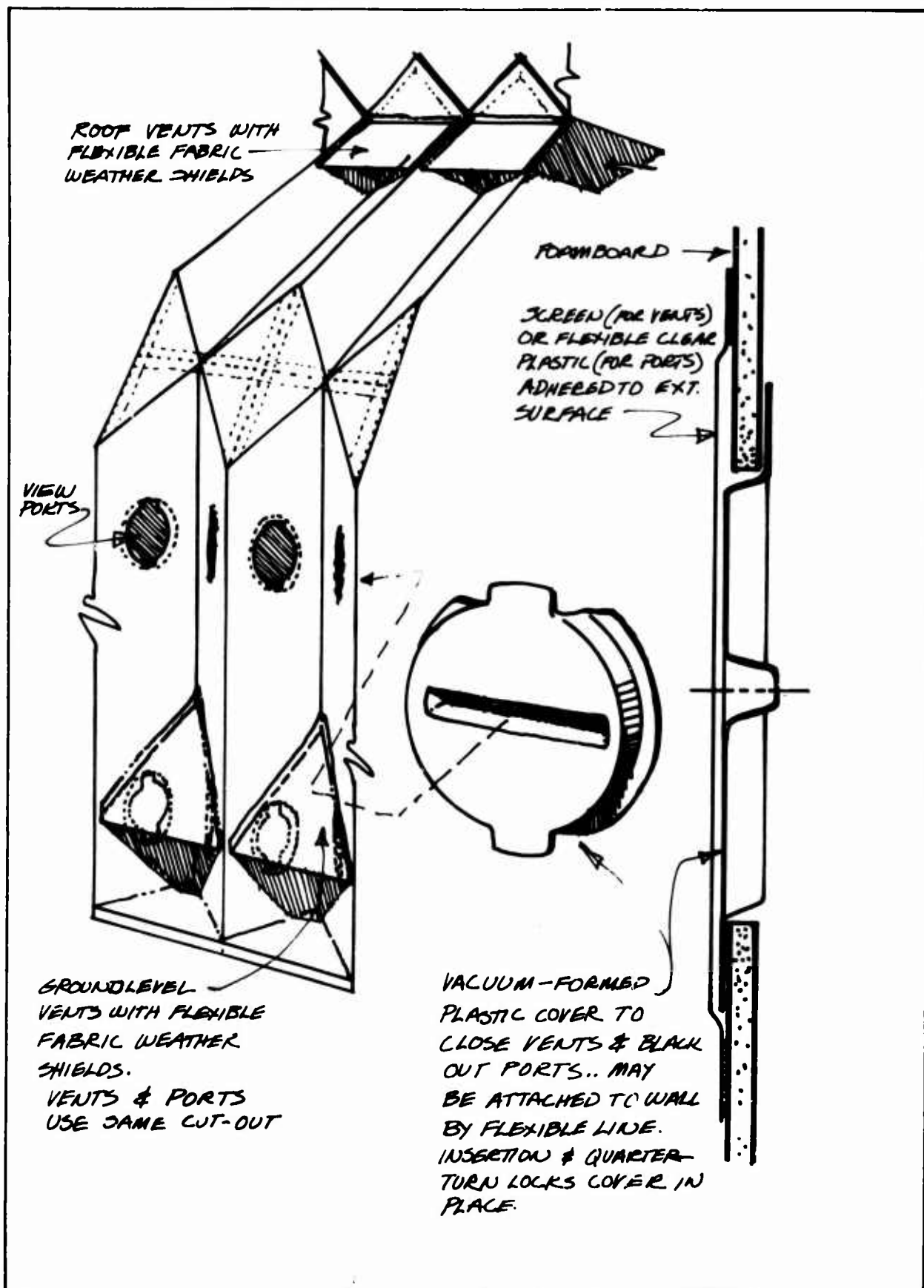
Figure 27. Vent and Window Concepts - LES and ES/C
