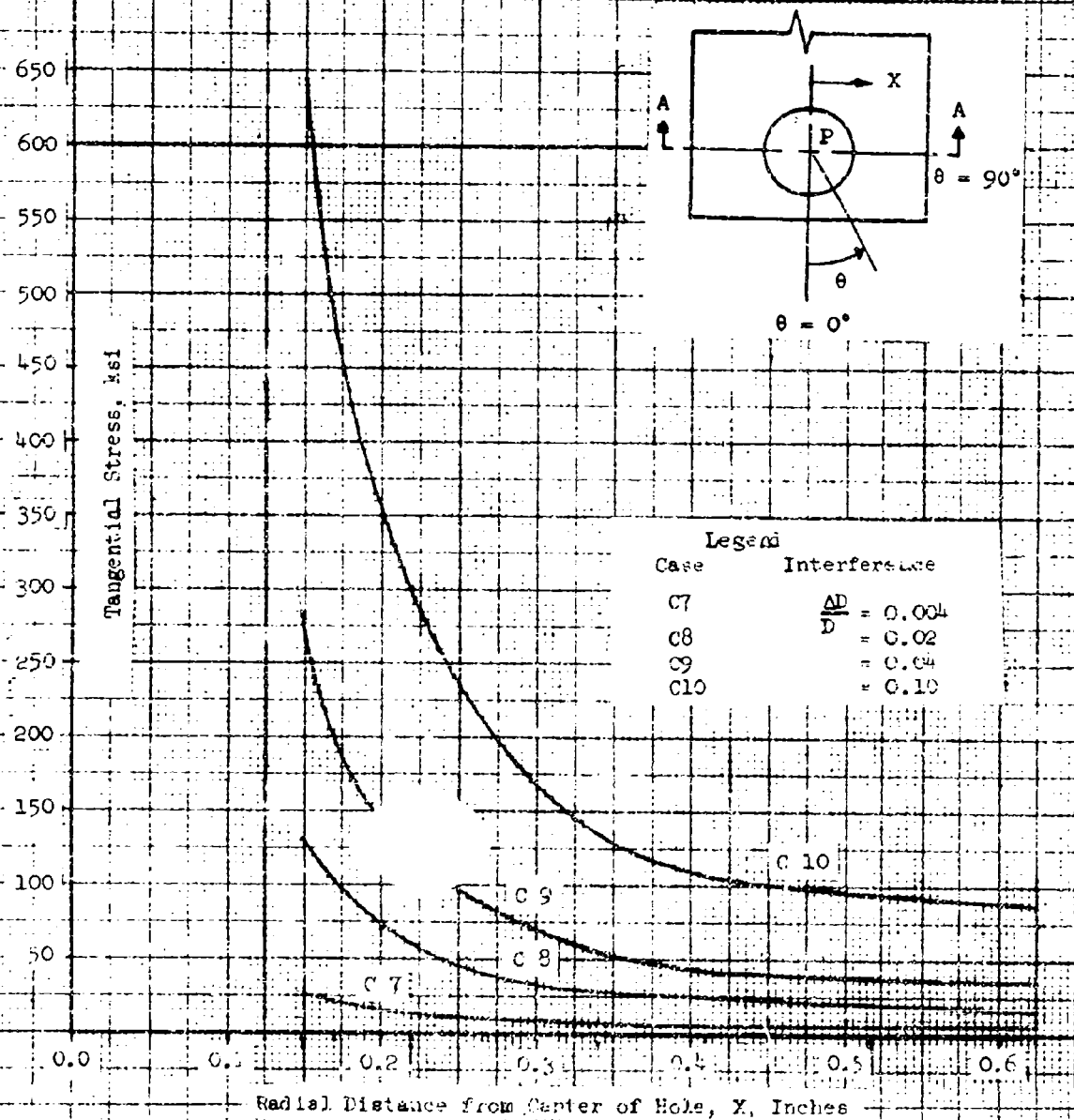
Fig. 31 Maximum Tangential Stress Variation for Different Interference Fits.
