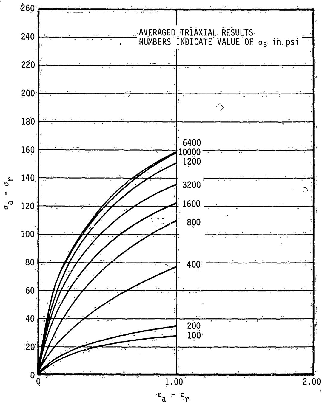
Figure 33. Watchling Hill Clay; Triaxial Test Results; ( \sigma_a - \sigma_r ) vs ( \epsilon_a - \epsilon_r ); Expanded Scale
