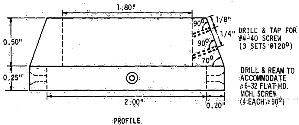
Figure 6. Lateral Deformeter
