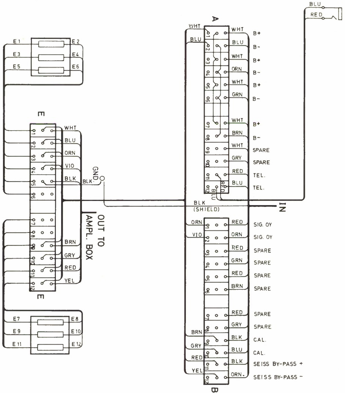
Figure A1.4 Junction box, wiring diagram; type 10Y(1)
