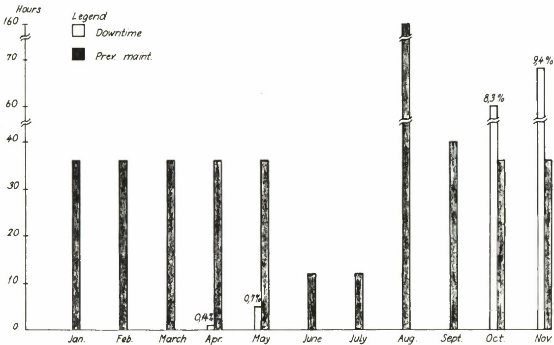
Figure A6. 43 Oyer - Vehicles - Downtime and preventive maintenance
