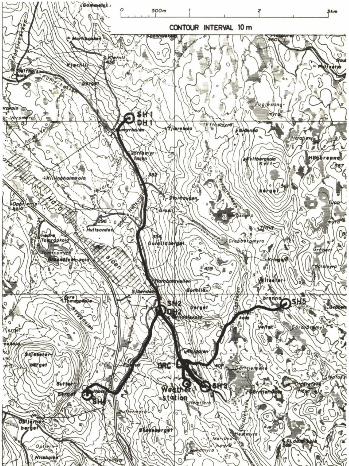
Figure 2.46 Noise study array configuration — = Cable route SH = Shallow hole DH = Deep hole
