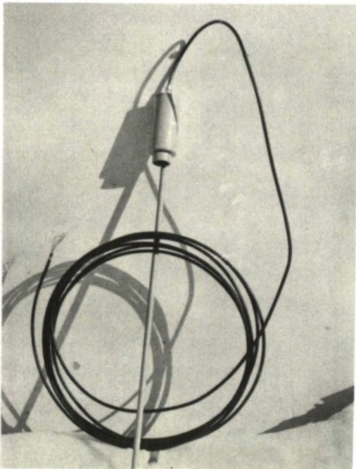
Figure 2.15 SP seismometer on stilt (Model Hall-Sears HS-10-1/ ARPA)
