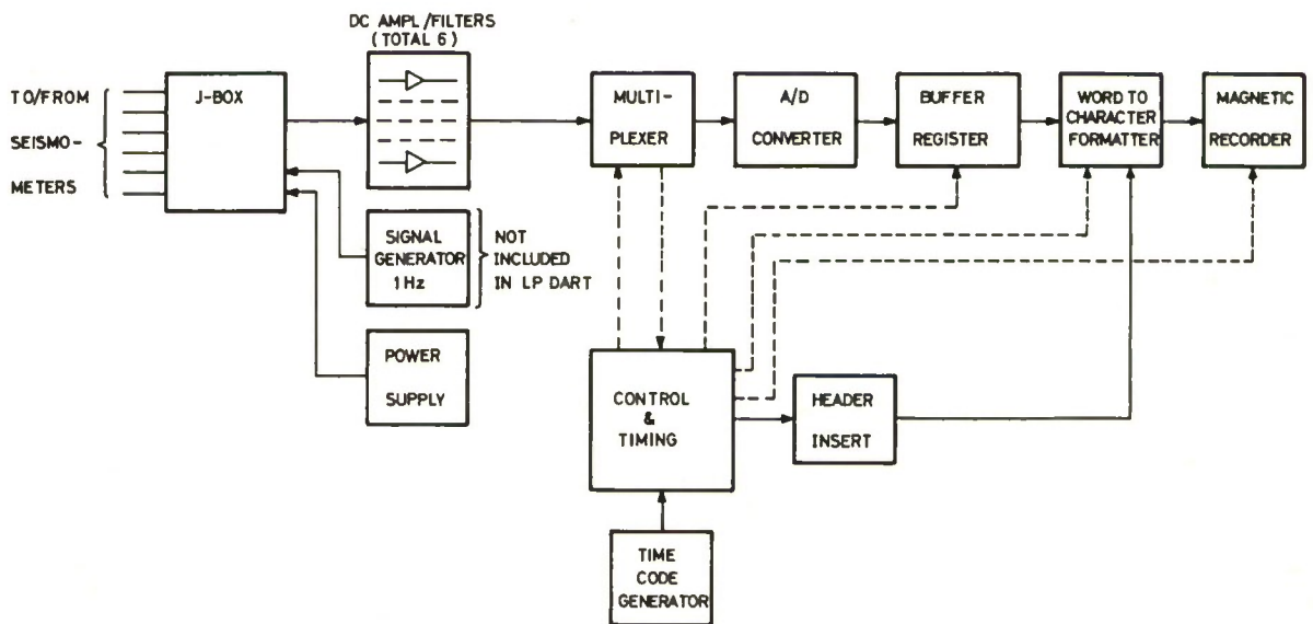
Figure 2.31 Block diagram of the DART system
