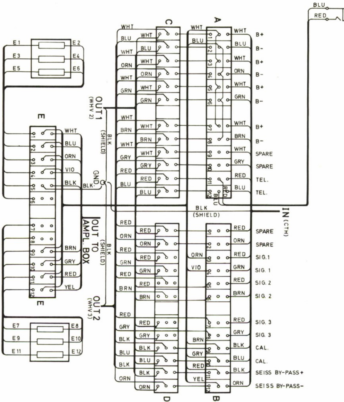
Figure A1.5 Junction box, wiring diagram; type branching point inner hexagon
