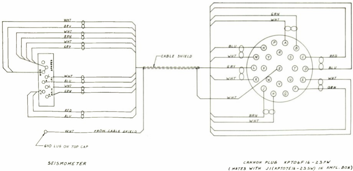
Figure A1.2 SP seismometer to amplifier box connections
