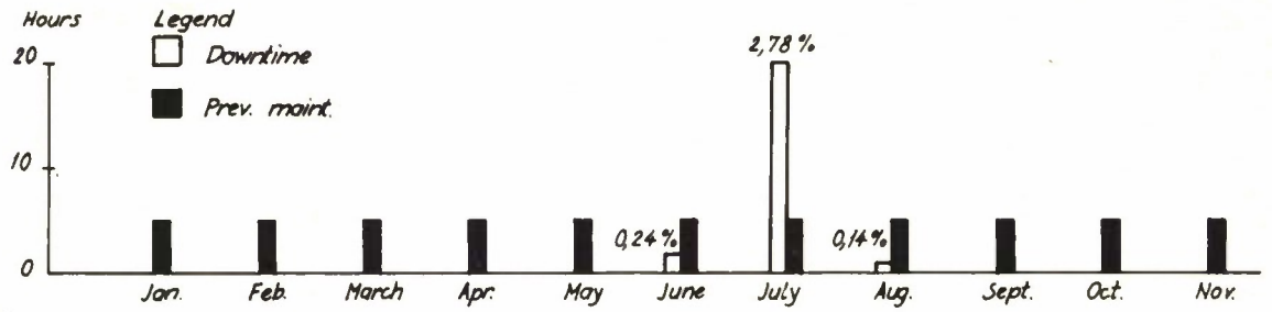
Figure A6.17 Falldalen - SP DART, clock - Downtime and preventive maintenance
