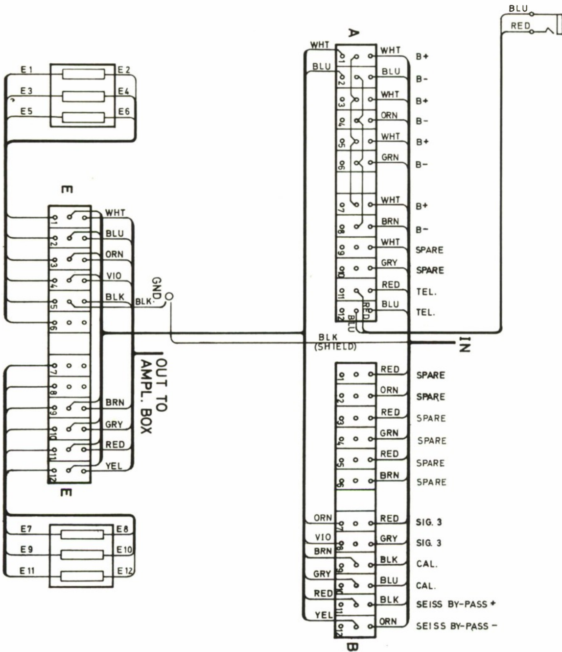
Figure A1.7 Junction box wiring diagram; type outer hexagon, right branch
