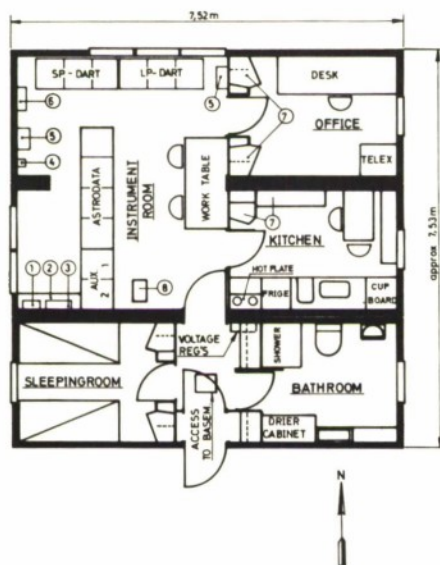
Figure 2.6 Arrangement of Øyer DRC
