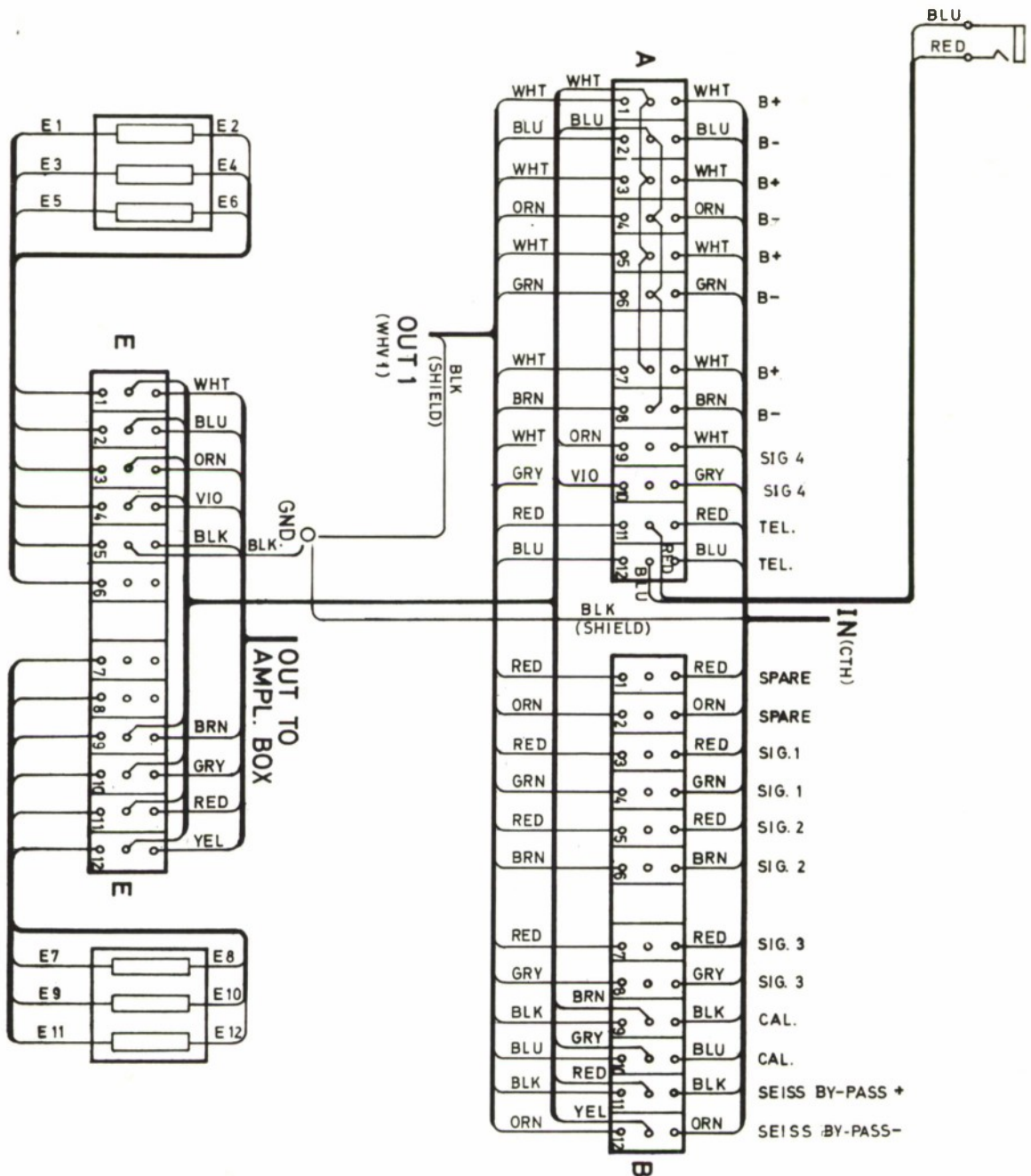
Figure A1.8 Junction box wiring diagram; type 1F4(20)
