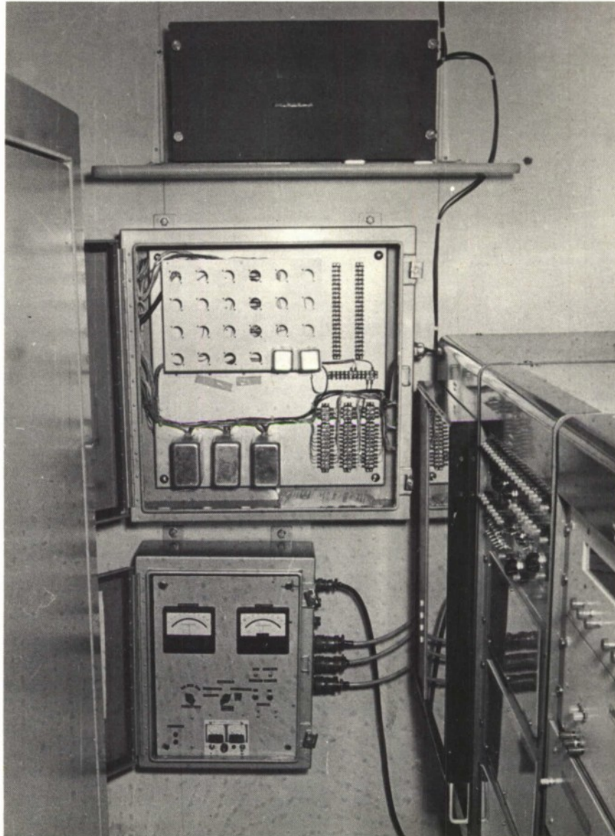
Figure 2.44 Cable/DART interfacing equipment in DRC Top: three-channel Geotech amplifier Middle: DRC junction box Bottom: monitor control unit
