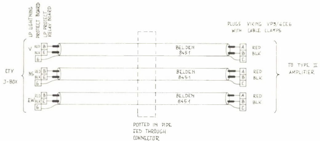
Figure A2.4 LPV cable connection
