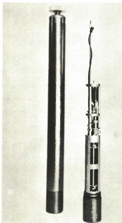
Figure 2.47 SP seismometer used in deep holes (Model Geotech 20171A - with and without cover).
