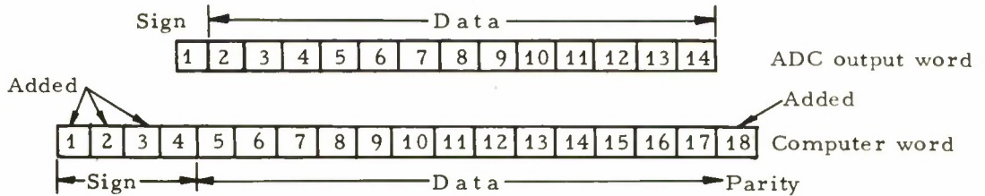
Figure 2.29 Astrodata word configuration
