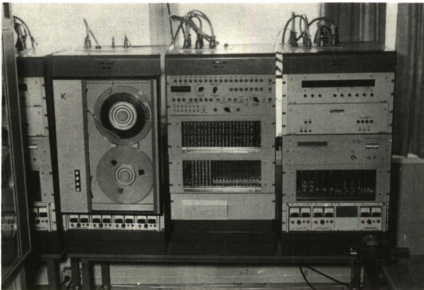
Figure 2.30 The DART recording system
