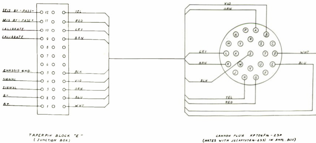
Figure A1.3 Amplifier box to junction box connections
