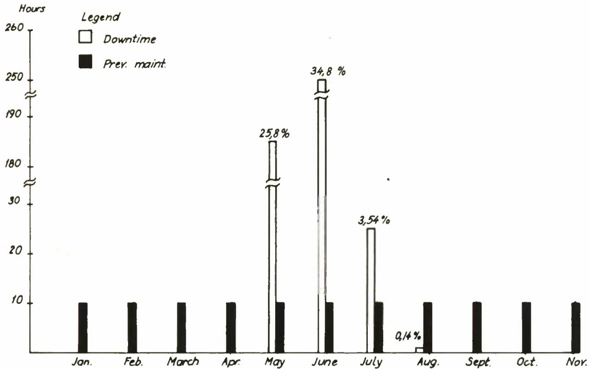
Figure A6.15 Falldalen - SP DART - Downtime and preventive maintenance (Total)
