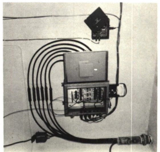
Figure 2.42 Seismometer/cable interfacing equipment in LPVs Left: Junction assembly Right: LPV junction box.
