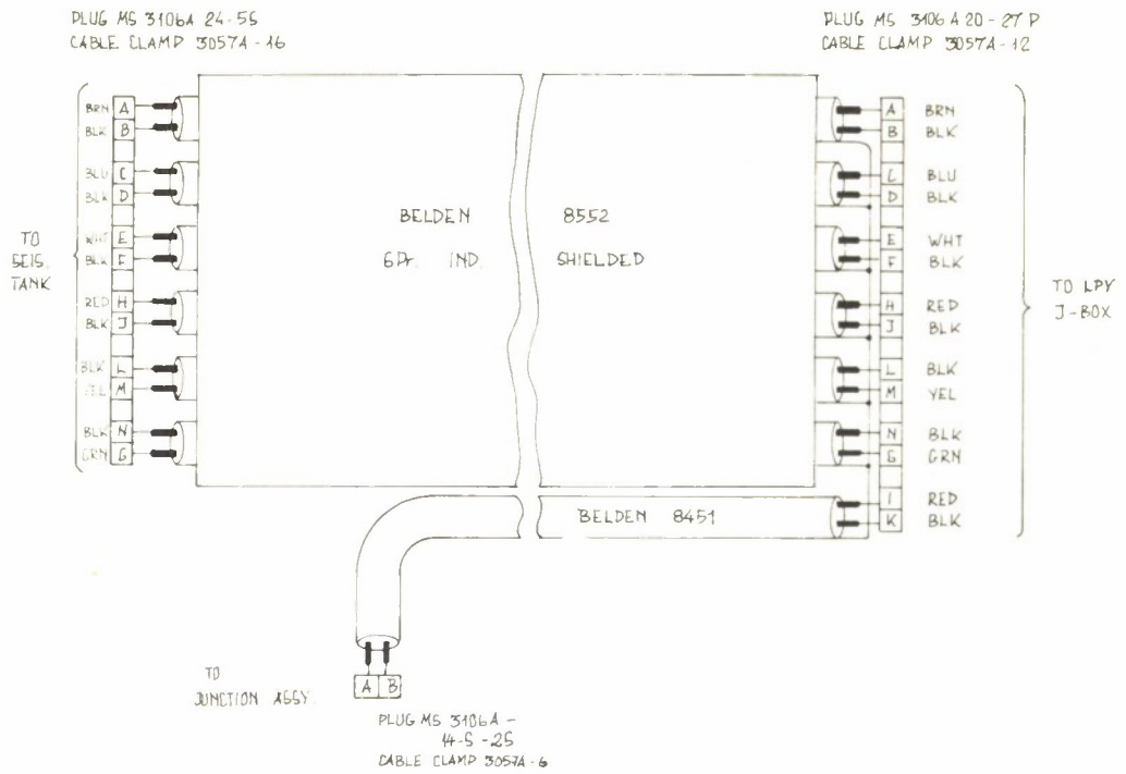
Figure A2.4 LPV cable connection
