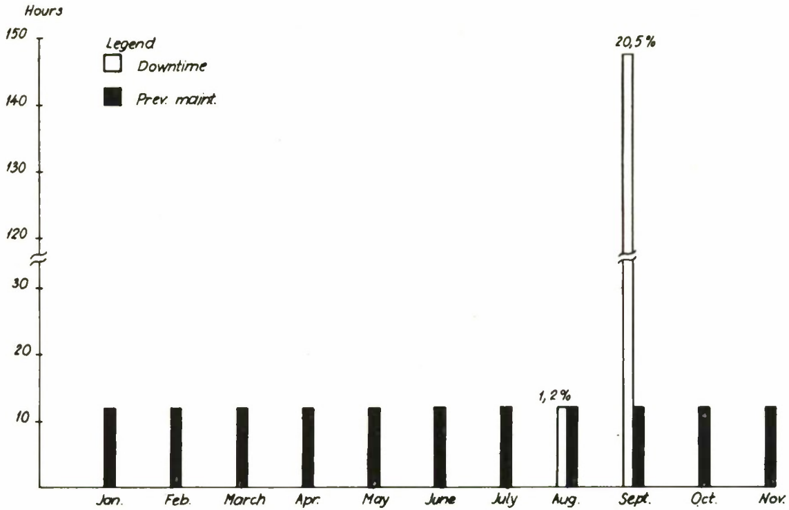
Figure A6. 36 Øyer - LP Front End - Downtime and preventive maintenance (Total)
