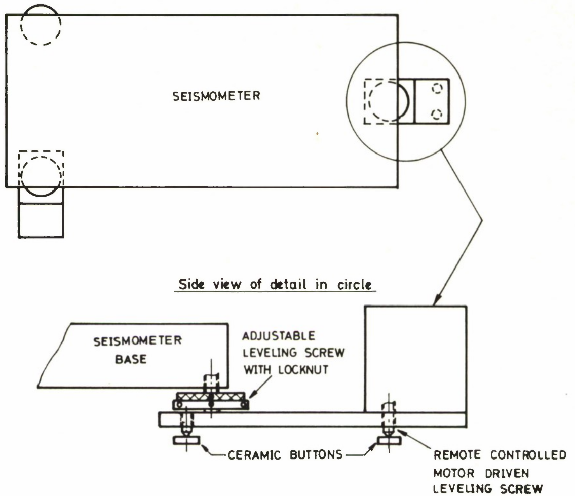
Figure 2.40 Mounting of LP seismometers with levelling devices
