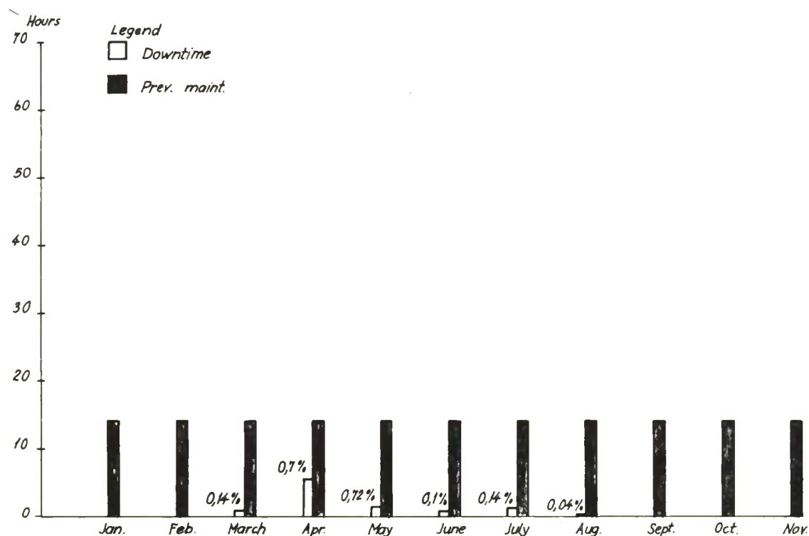
Figure A6.23 Falldalen - LP DART - Downtime and preventive maintenance (Total)
