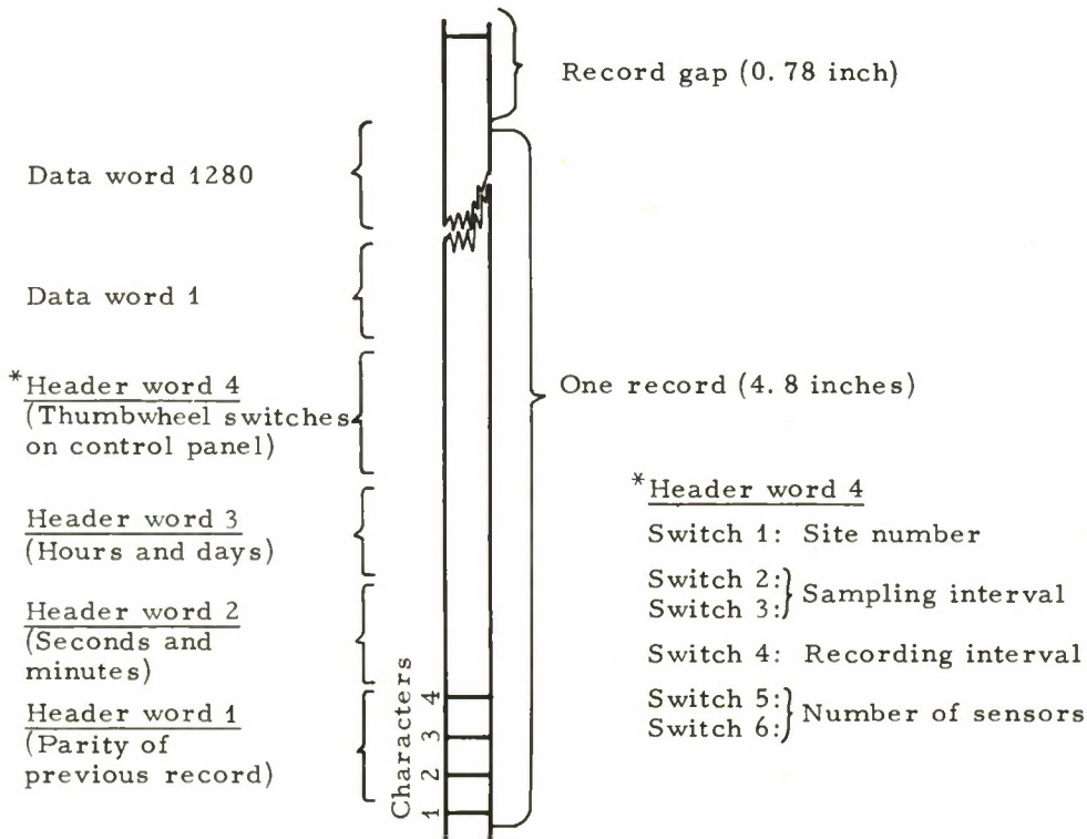
Figure 2.32 Astrodata tape format
