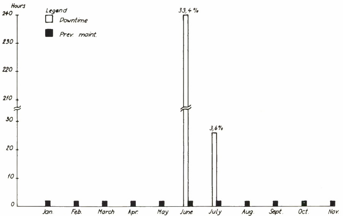
Figure A6.35 Falldalen - SP Front End, WHV amplifiers - Downtime and preventive maintenance
