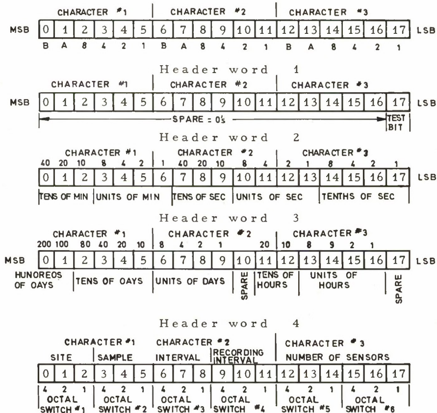
Figure 2.33 DART data and header words
