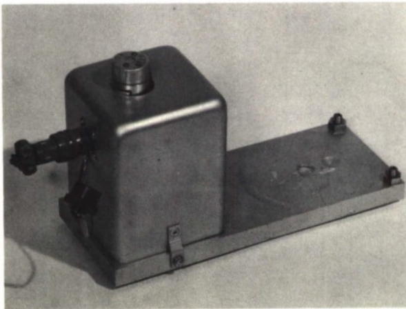
Figure 2.41 Remote levelling device for LP seismometers
