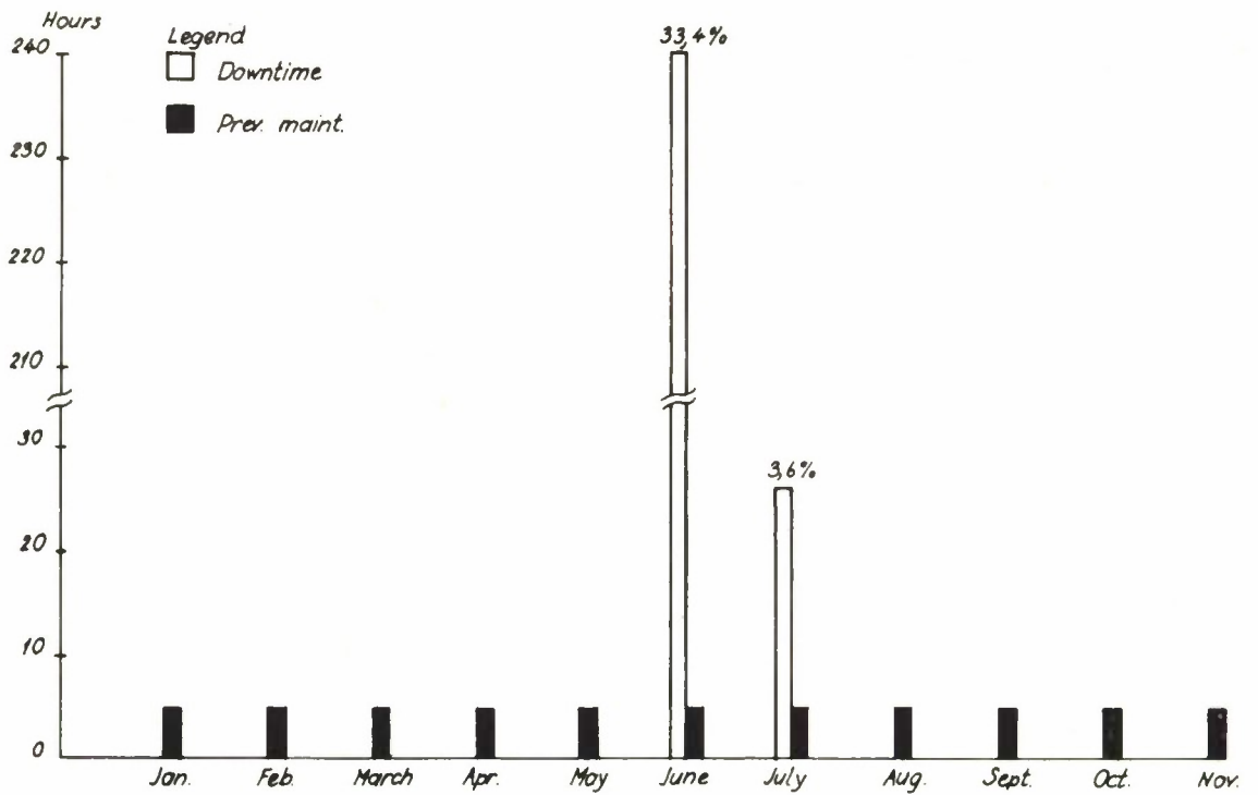
Figure A6.34 Falldalen - SP Front End - Downtime and preventive maintenance (Total)
