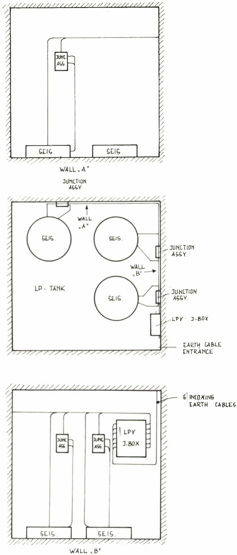
Figure 2.43 Physical layout in LPV
