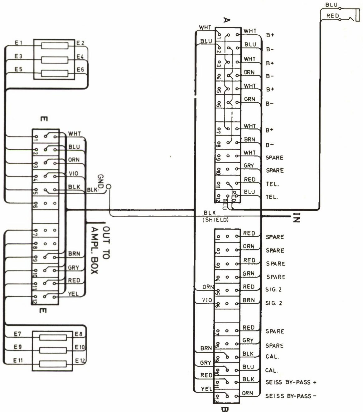
Figure A1.6 Junction box, wiring diagram; type outer hexagon, left branch
