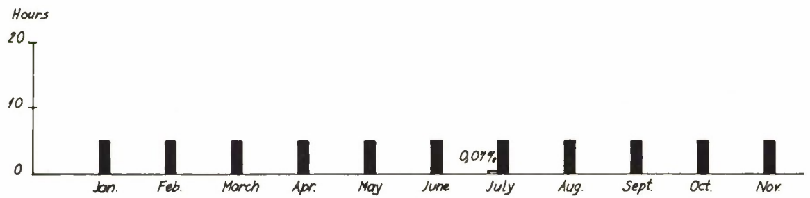
Figure A6.18 Falldalen - SP DART, recorder - Downtime and preventive maintenance
