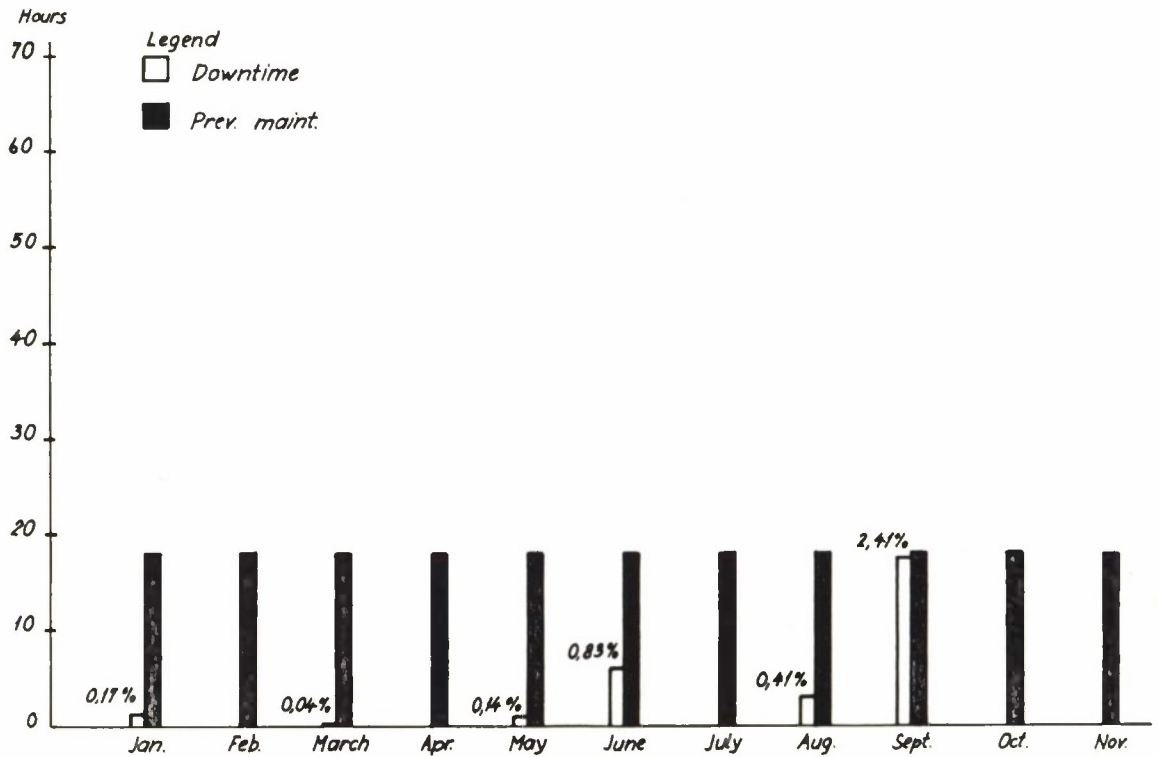
Figure A6.19 Øyer - LP DART - Downtime and preventive maintenance (Total)
