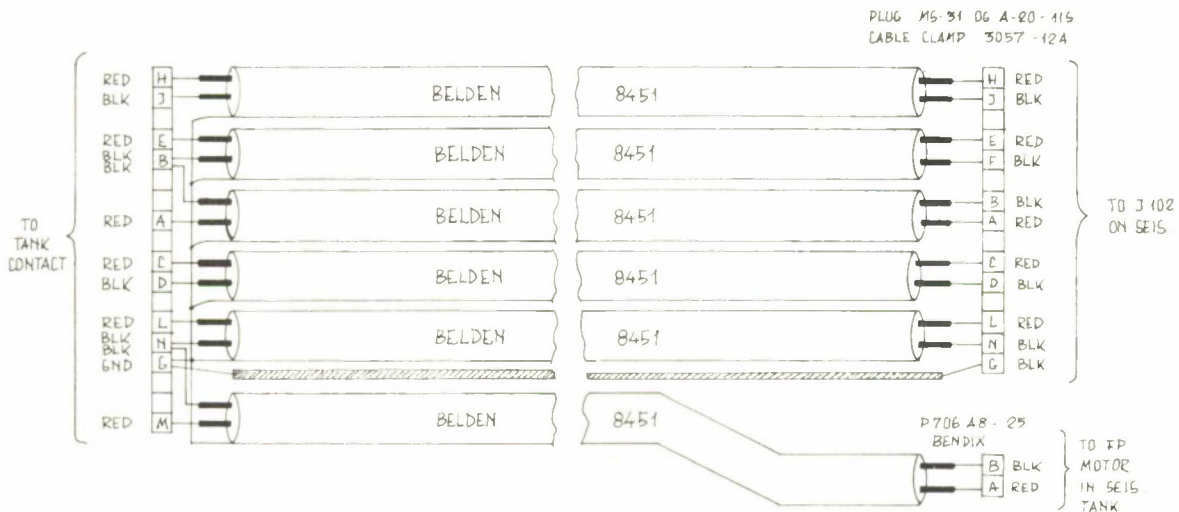
Figure A2.2 Internal LP tank connections, vertical seismometer
