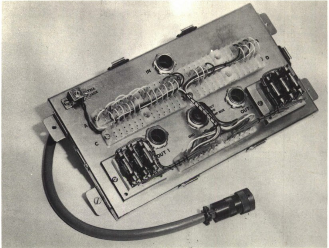
Figure 2.24 Junction Box, branching type
