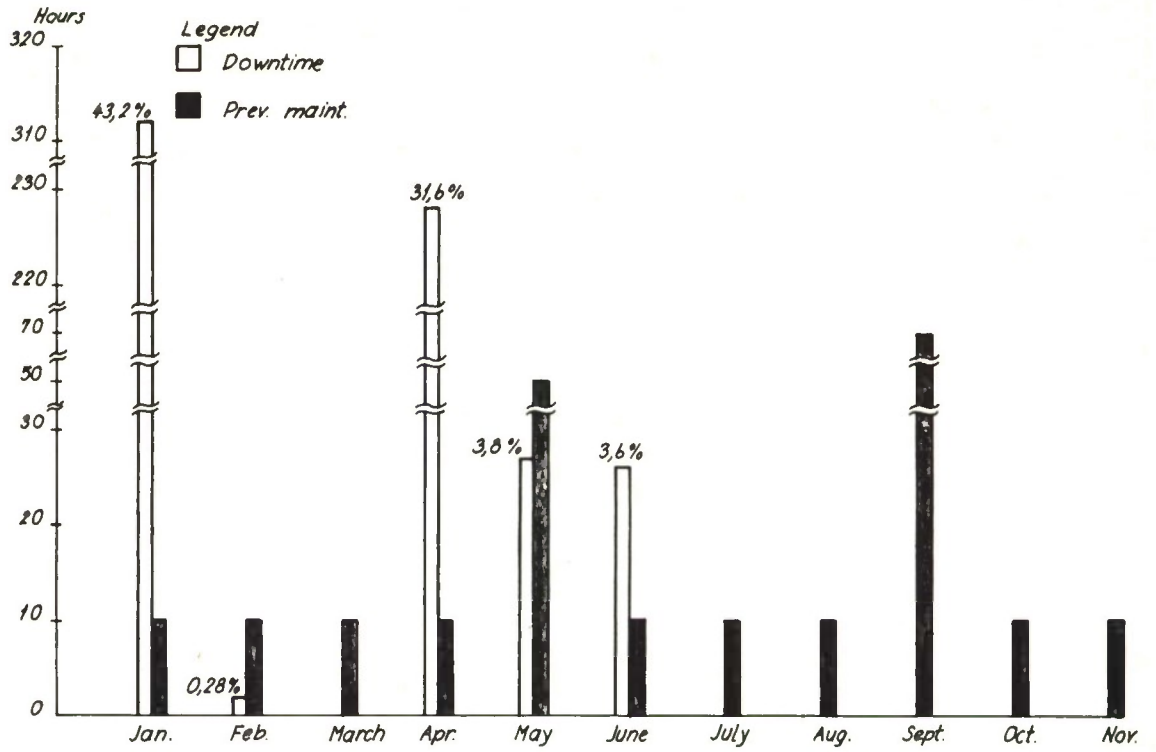
Figure A6.30 Oyer - SP Front End - Downtime and preventive maintenance (Total)
