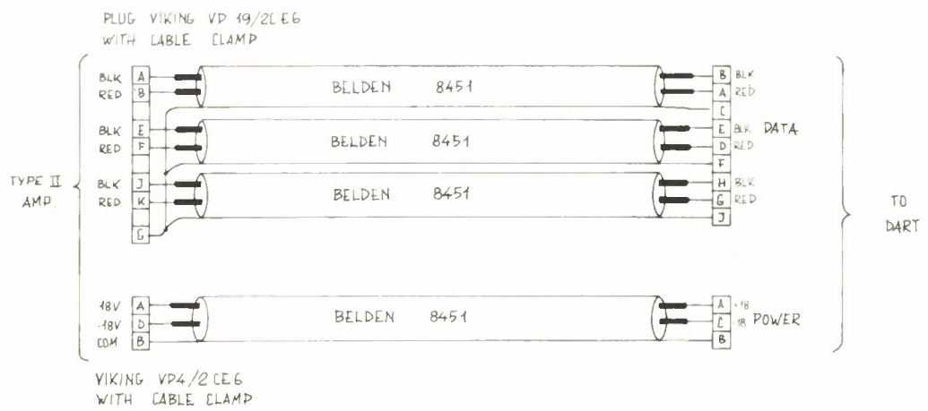
Figure A2.6 Data and power cable amplifier to LP recorder (DART) in DRC
