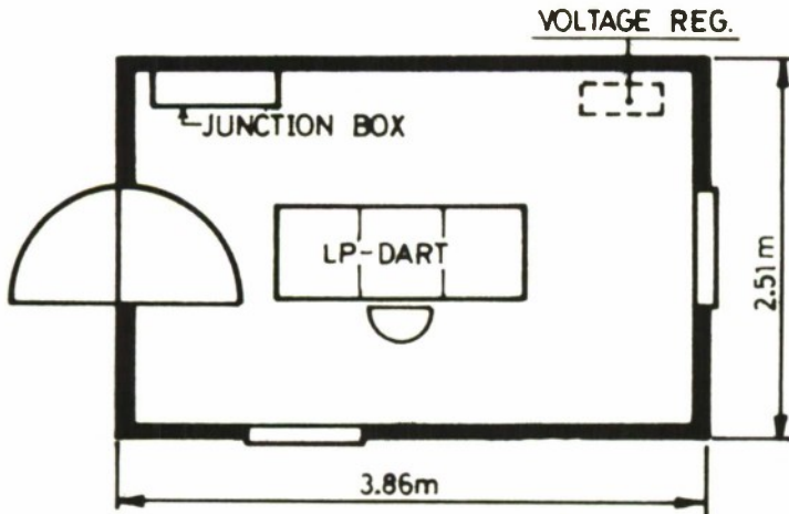
Figure 2.13 Arrangement of Trysil DRC
