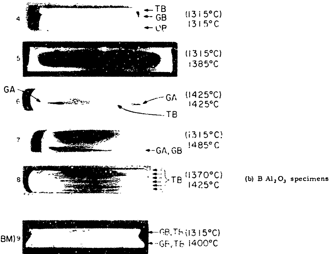
Fig. 7 - Cross sections of \text{Al}_2\text{O}_3 vacuum hot-pressed without additives. Figures at the right refer to the temperatures of starting pressure and hot pressing. Cross sections are all 1.2 to 1.5 in. in diameter. Note rounding of edges due to shrinkage from the die. GA and GB refer to green areas and green bands, and OB and TB refer to opaque and translucent bands. Other coloration was as seen in the photos. Samples 4 through 6 were pressed with 10,000 psi for 90, 60, and 5 minutes, respectively. Sample 4 was nearer the bottom of the die. Samples 7 and 8 were pressed with 5000 psi for 15 minutes. Note the black areas in Samples 5 and 7 and many fine bands in Sample 8 that had a gray-orange appearance in transmission. BM \text{Al}_2\text{O}_3 was hot-pressed with 5000 psi for 30 minutes. Note that the bands are made up of light green translucent patches and irregular edges due to shrinking away from the die.
