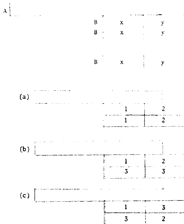
FIGURE 4 A Logical Data Structure and Specific Instances
