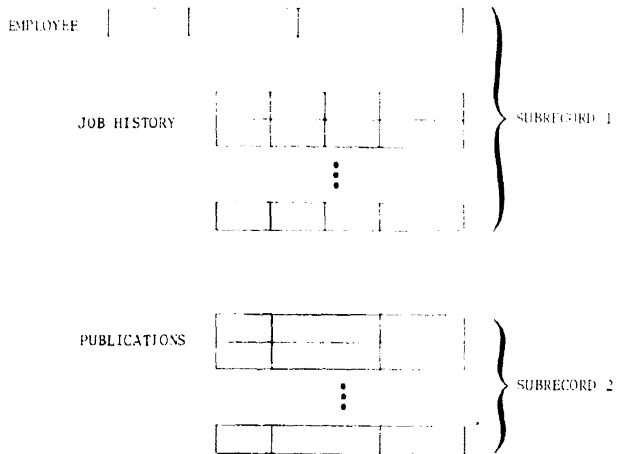
FIGURE 2 Partitioning of Logical Records into Logical Subrecords
