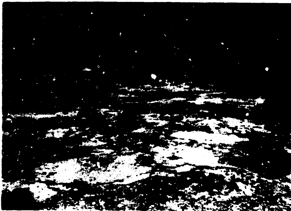
Figure 4. Travertine-Crust Zone in northern part of playa.
