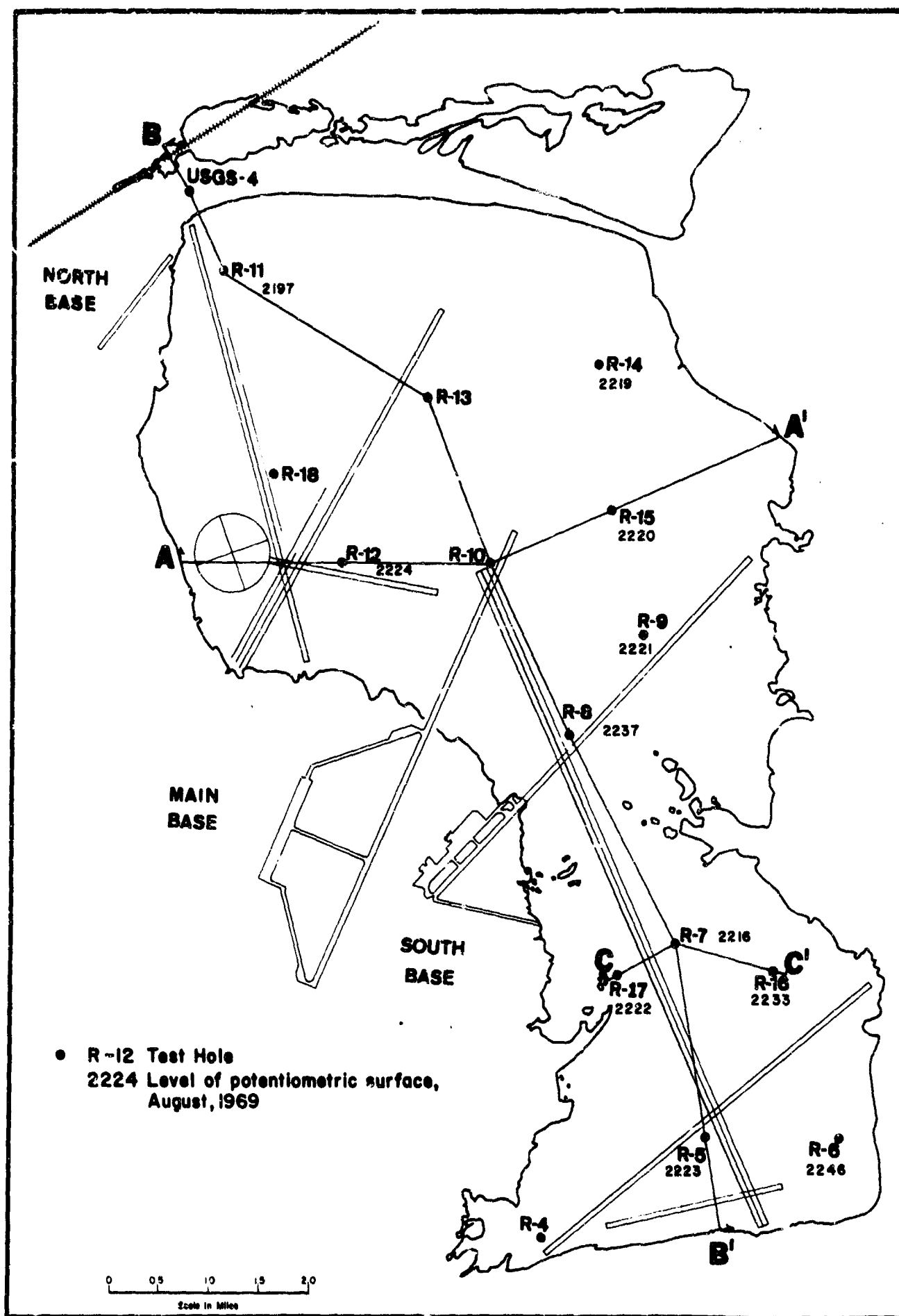
Figure 16. Map of Rogers Playa showing lines of cross sections and elevations of potentiometric surfaces in test wells.
