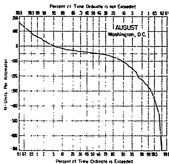
Figure A9. Cumulative probability distribution of dN/dh for a ground-based 50-m layer (Washington, D.C.).
