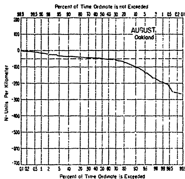
Figure A2. Cumulative probability distribution of dN/dh for a ground-based 50-m layer (Oakland, Calif.).
