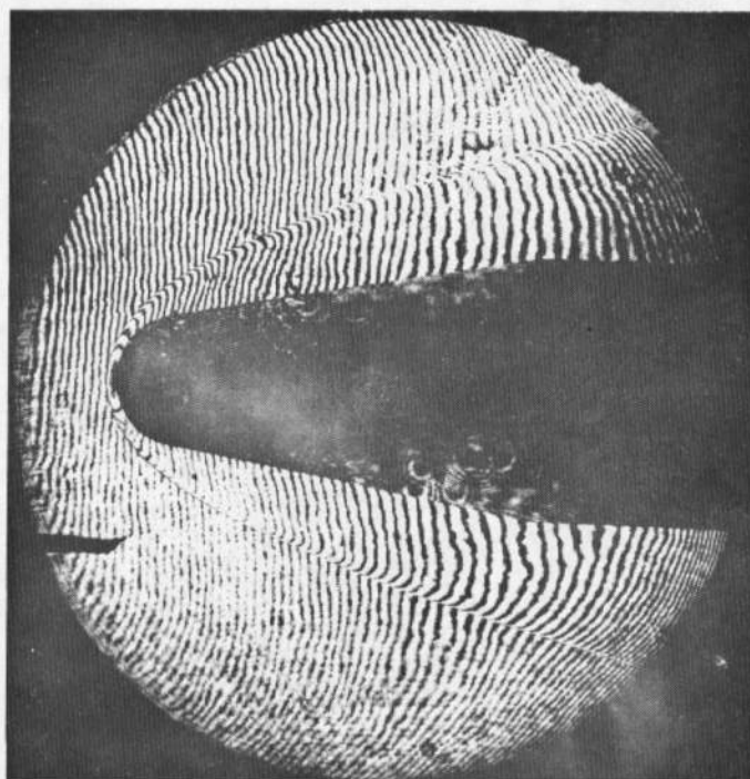
Fig. 25 Interferogram Reconstructions
