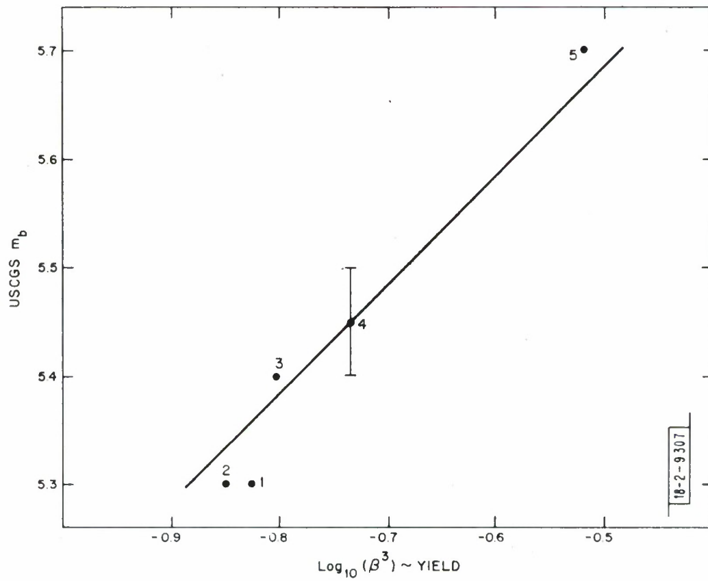
Fig. 12. USCGS m_b plotted vs \text{log}_{10}(\beta^3) using \beta determined in the simultaneous fit of all the spectra of each event. The straight line has a slope of 1.0.
