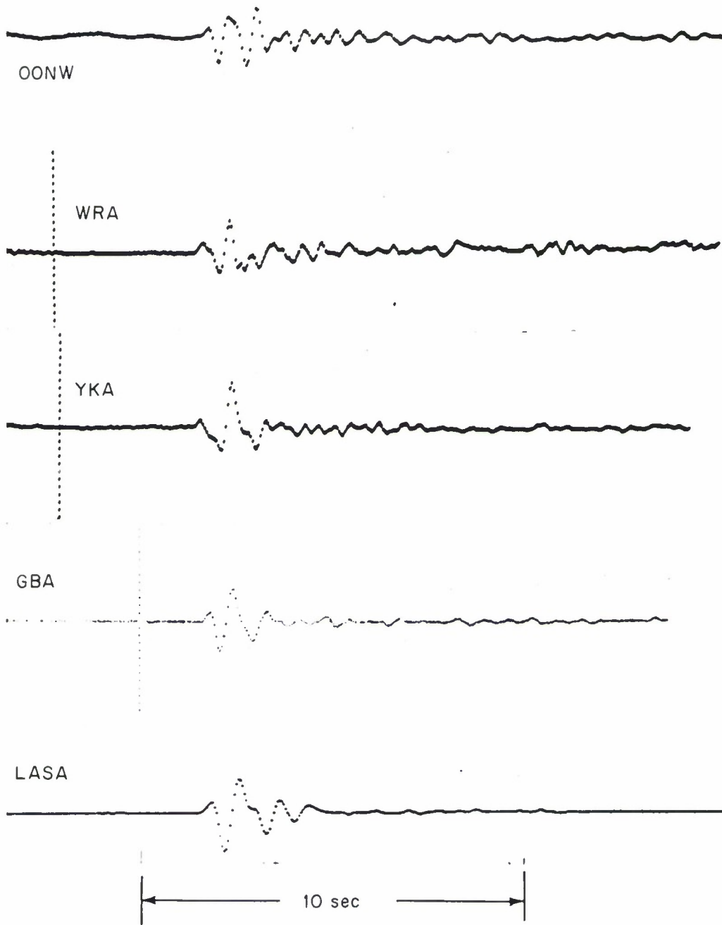
Fig. 6. The beams at the five arrays of event 1, m_b = 5.3 .
