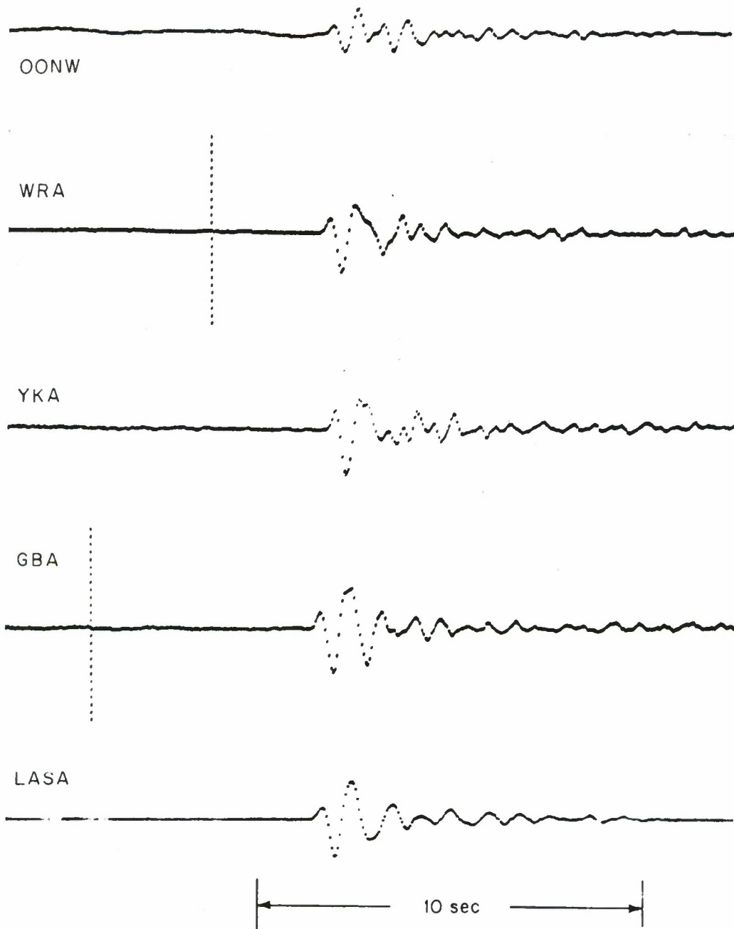
Fig. 7. The beams at the five arrays of event 5, m_b = 5.7 .
