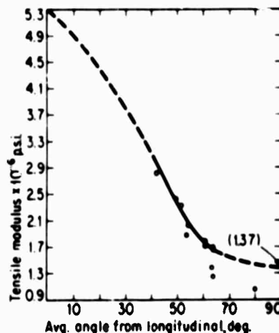
Fig. 7: Young's modulus versus longitudinal fiber orientation for 50% volume, 1/8-in. glass fiber in epoxy. Dashed line is extrapolation to limits predicted by Tsai-Halpin equations (see footnote 2 above).
