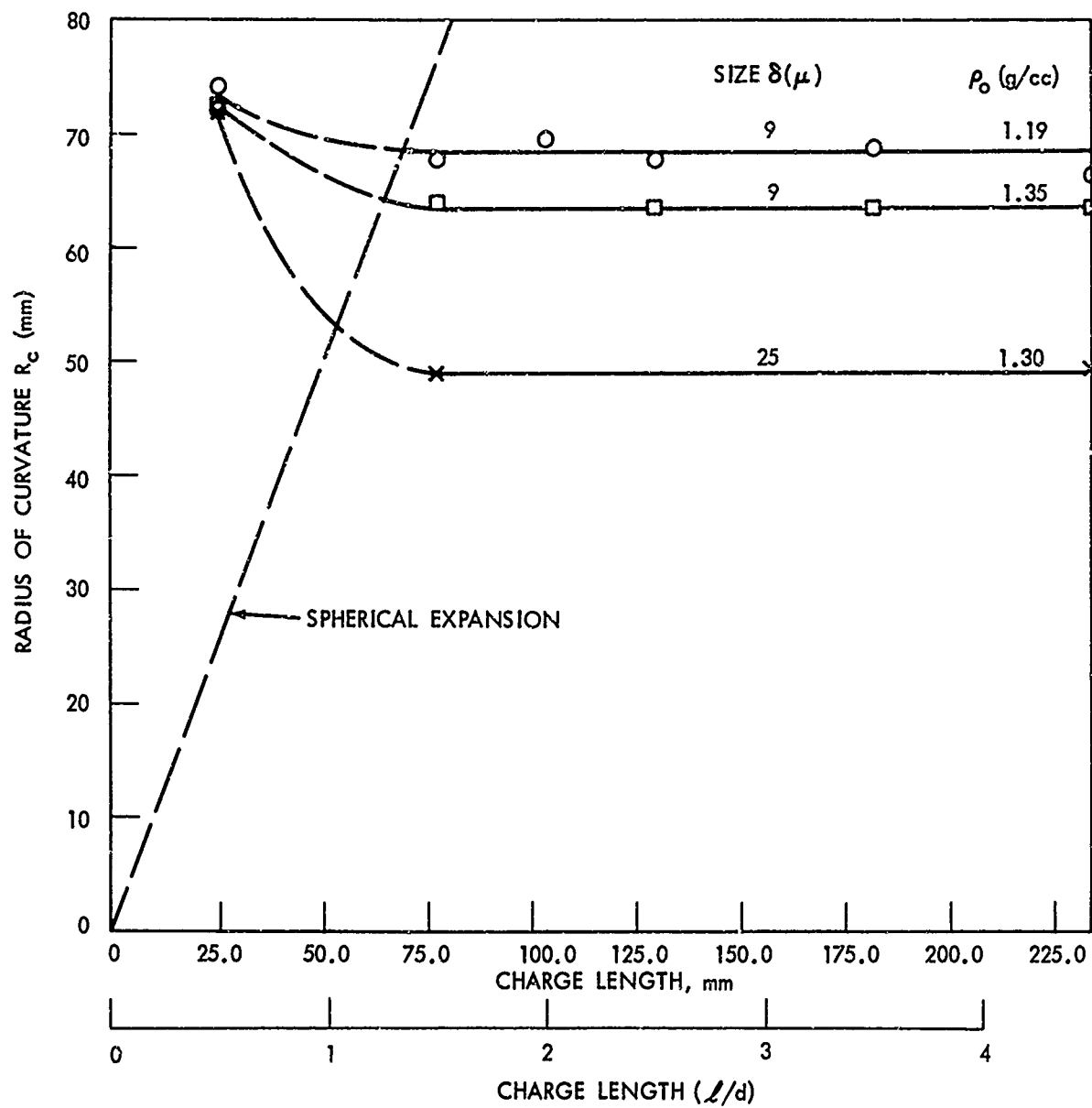
FIG. 7 RADIUS OF CURVATURE VS LENGTH OF AP CHARGES OF N-138 AND N-126, d = 50.8 mm
