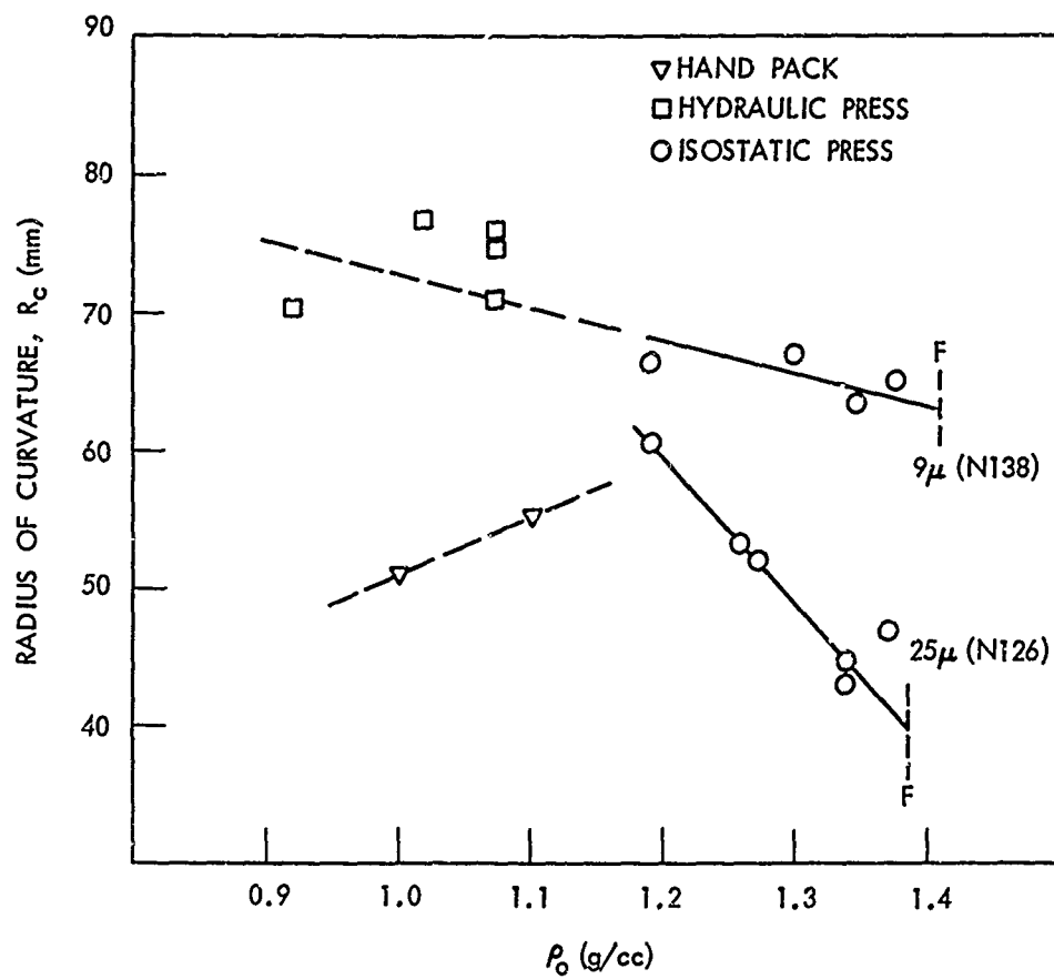
FIG. 6 R_c VS \rho_0 CURVES FOR 9 \mu AND 25 \mu AP AT d \sim 50 mm.
