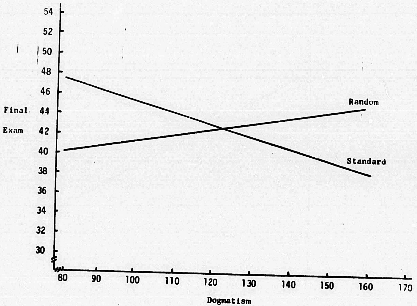
Figure 4 Regression of final examination score on Dogmatism
