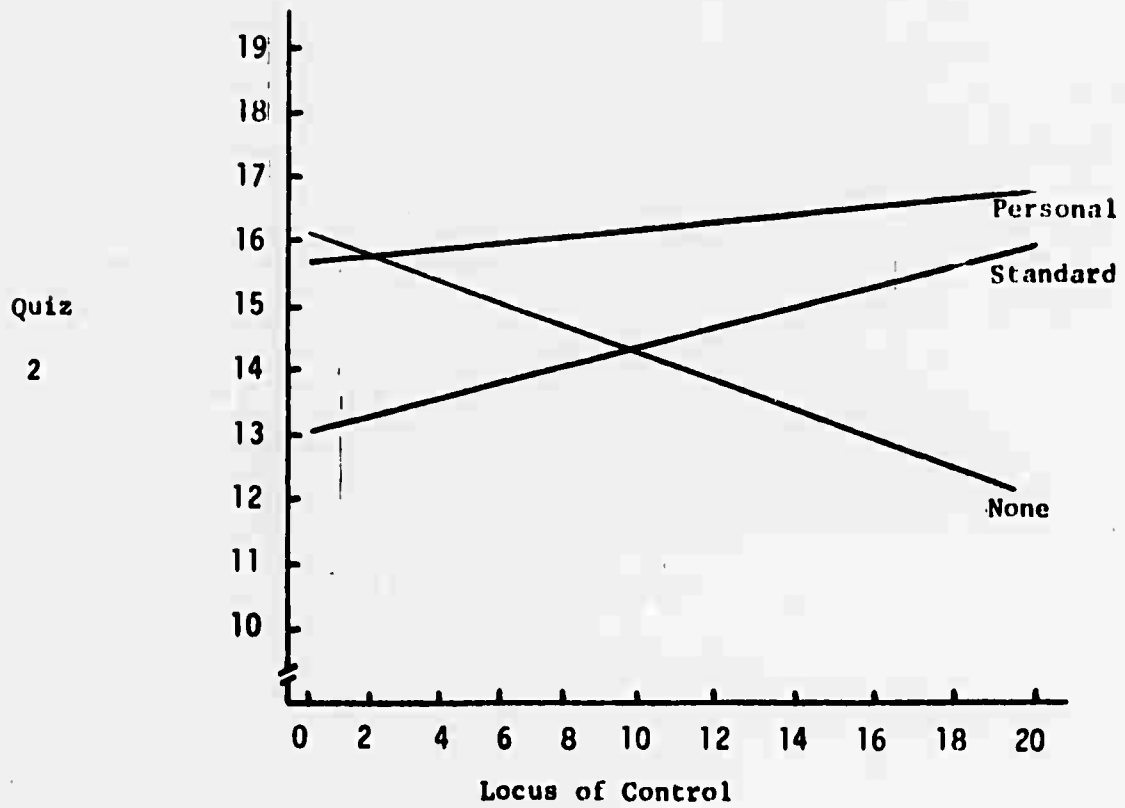
Figure 5 Regression of Quiz 2 Scores on Locus of Control
