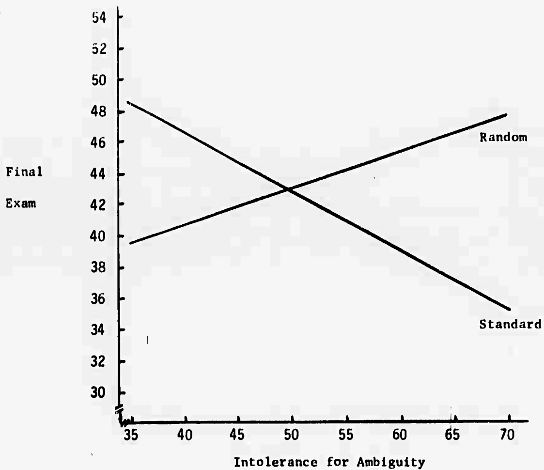
Figure 3 Regression of Final Exam Scores on Intolerance for Ambiguity
