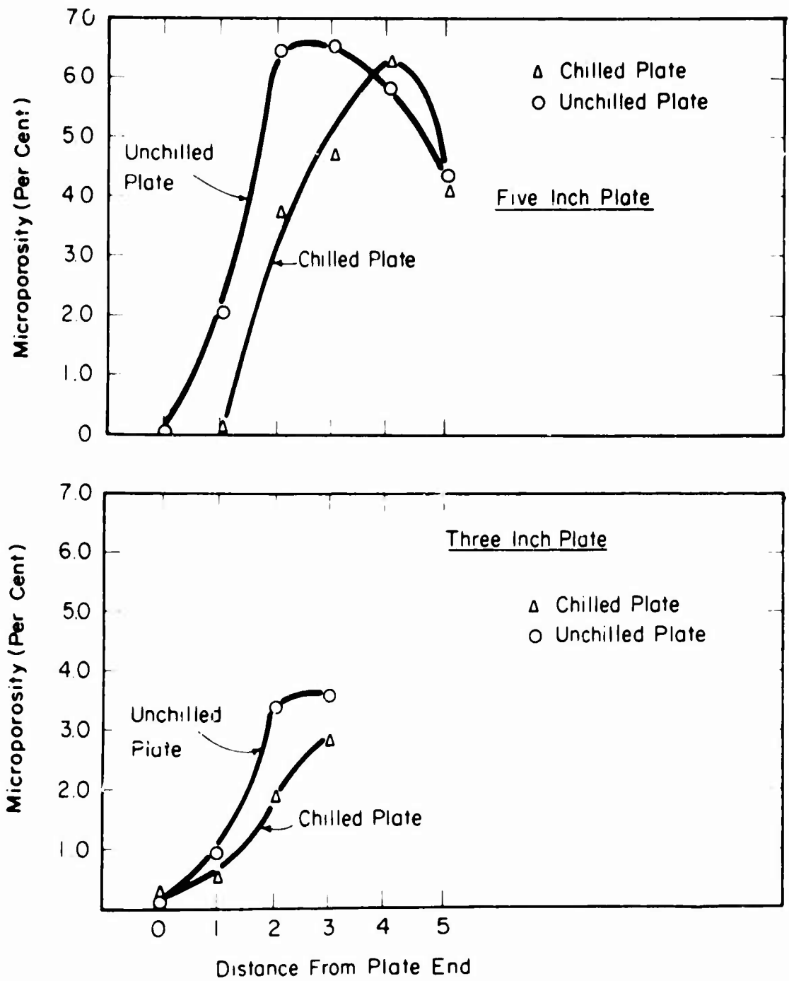
Figure 12 Microporosity Survey in Plate Castings (each point represents an average of data from two to four different castings)
