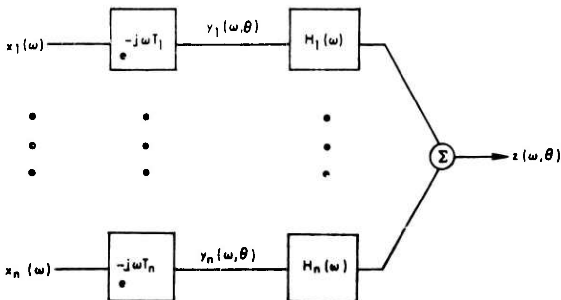
Fig. 1 - Conventional Beamformer
