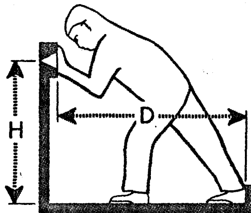
Figure 2. Forward leaning, push with both hands. Force plate adjusted to a height (H) of 70% and to a distance (D) of 80% of each subject's acromial height.
