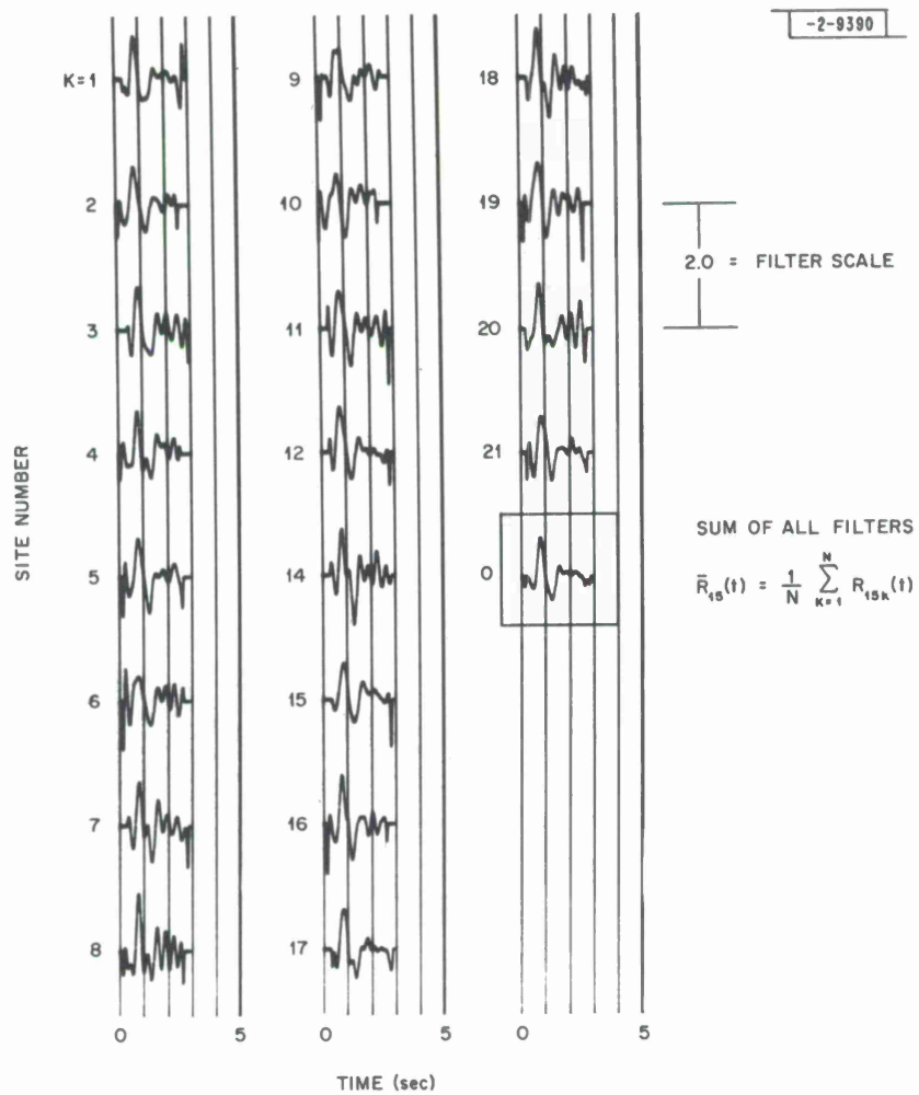
Fig. 1-2. Empirical transfer functions R_{15k}(t) to shape event 1 to event 5 at subarray site k . Average of all filters is shown in box.
