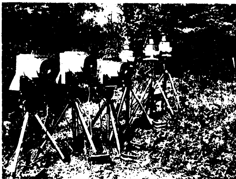
FIGURE 29. PHOTOGRAPH OF RADIOMETERS SET UP TO OBSERVE 81-mm MORTARS, 8/27/68. The narrow-field-of-view radiometers are on the left and the wide-field-of-view radiometers on the right.
