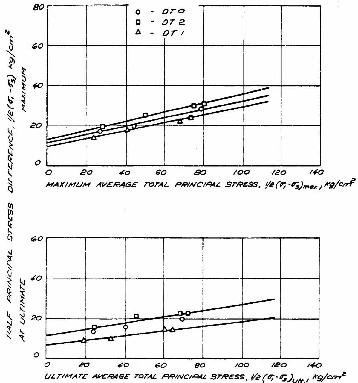
FIG. 4.9 INFLUENCE OF DELAY TIME OF COMPACT- TION ON THE TOTAL STRESS - STRENGTH BEHAVIOR OF M-21 + 5% CEMENT.
