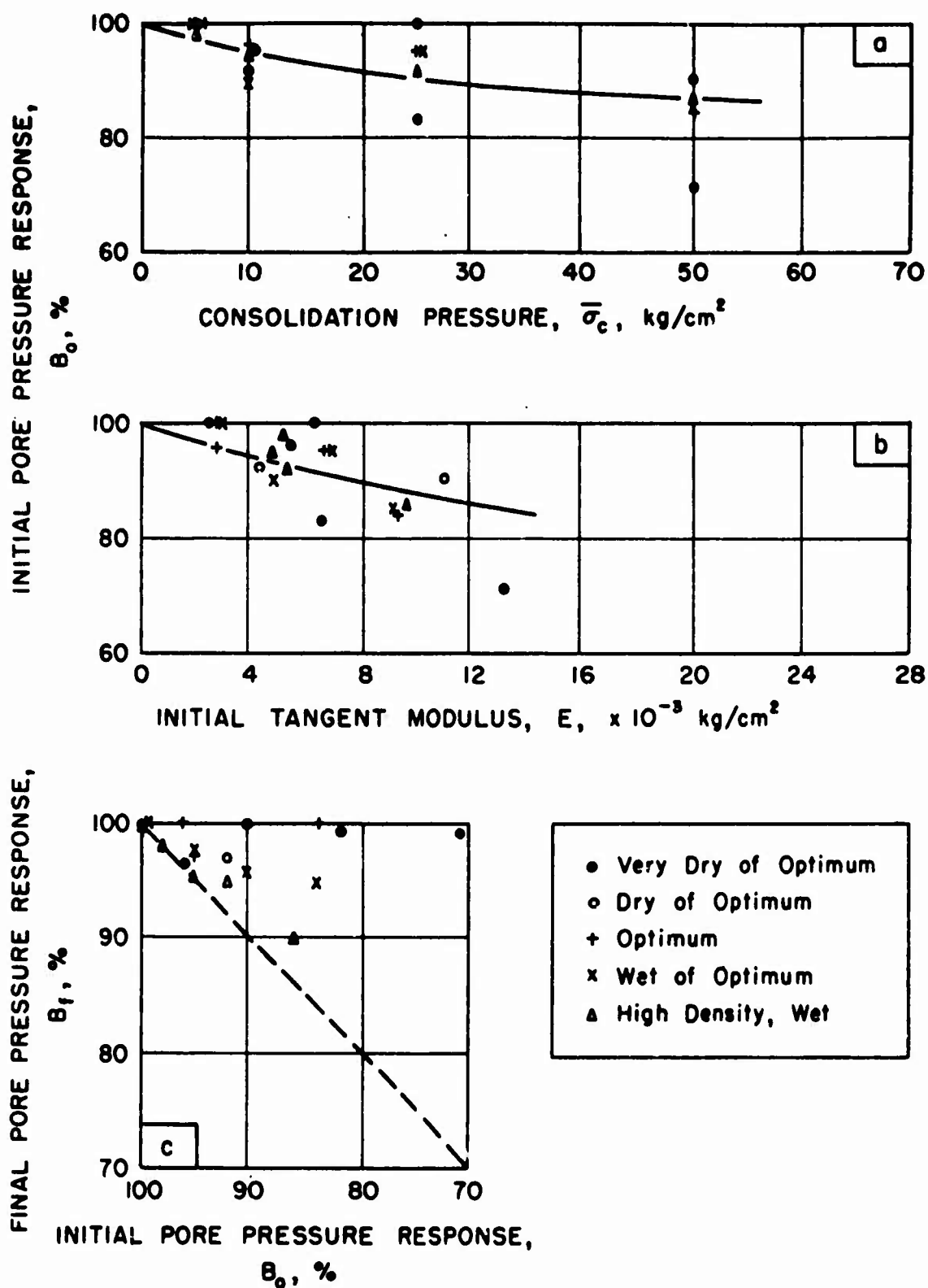
FIG.3.26 PORE PRESSURE RESPONSE OF UNTREATED MASSACHUSETTS CLAYEY SILT.
