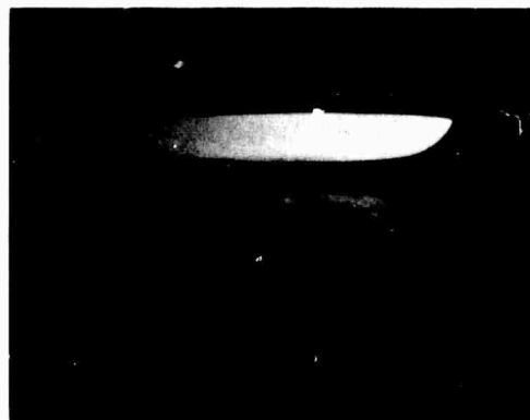
(b) Molybdenum Anode Glowing Red Hot (Note Reflection on Cathode)
