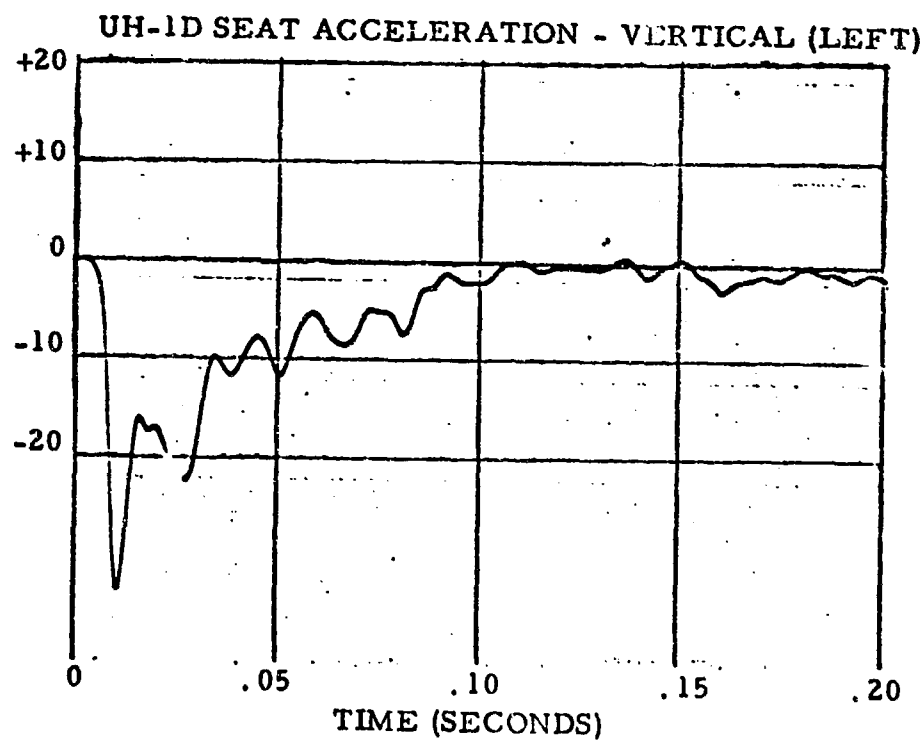
Figure B8. UH-1B/D SEAT TEST NO. 3.
