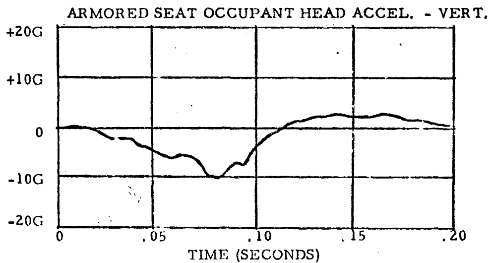
Figure A2. UH-1B/D ARMORED SEAT TEST NO. 1
