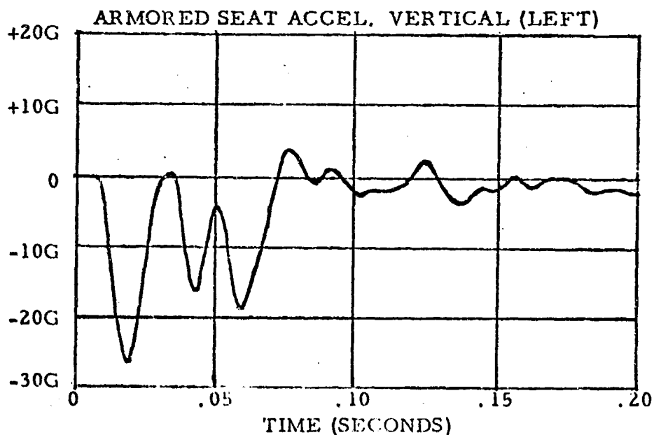
Figure A3. UH-1B/D ARMORED SEAT TEST NO. 2.
