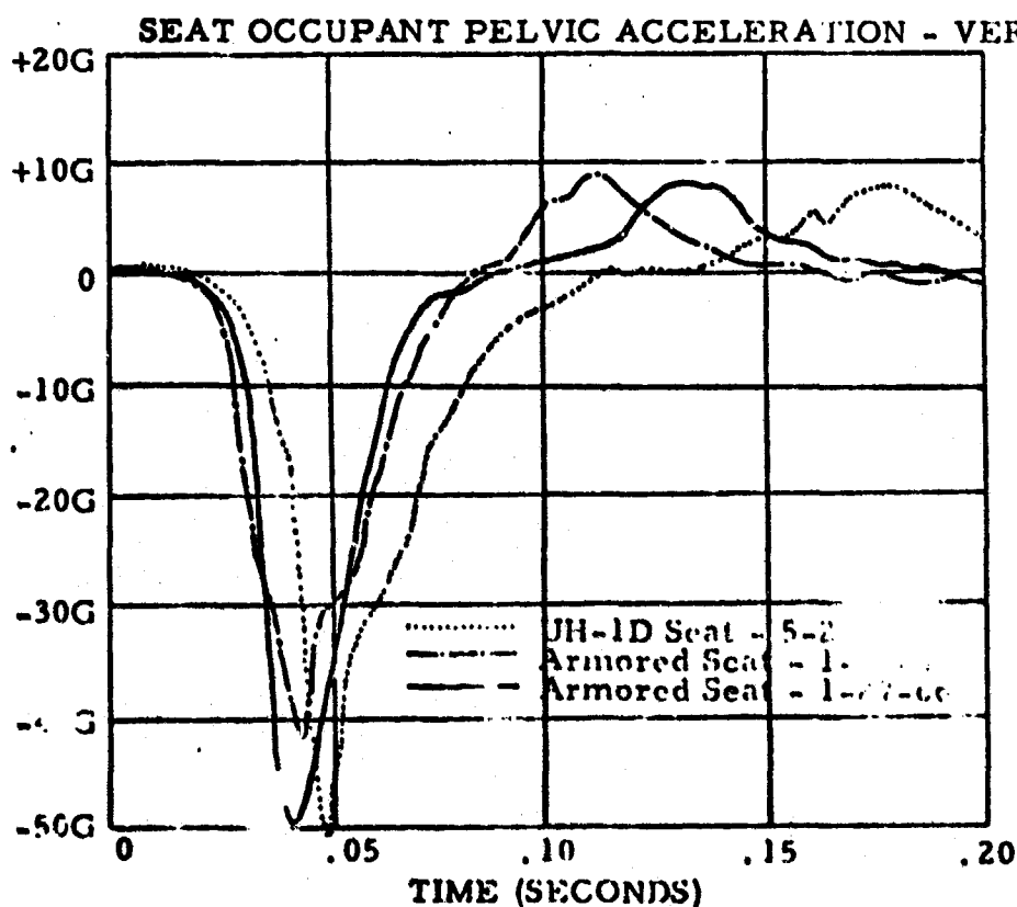
Figure 7. UH-1B/D Armored Seat Test No. 1 With Results of May 1965 and January 11, 1966 Tests Superimposed.
