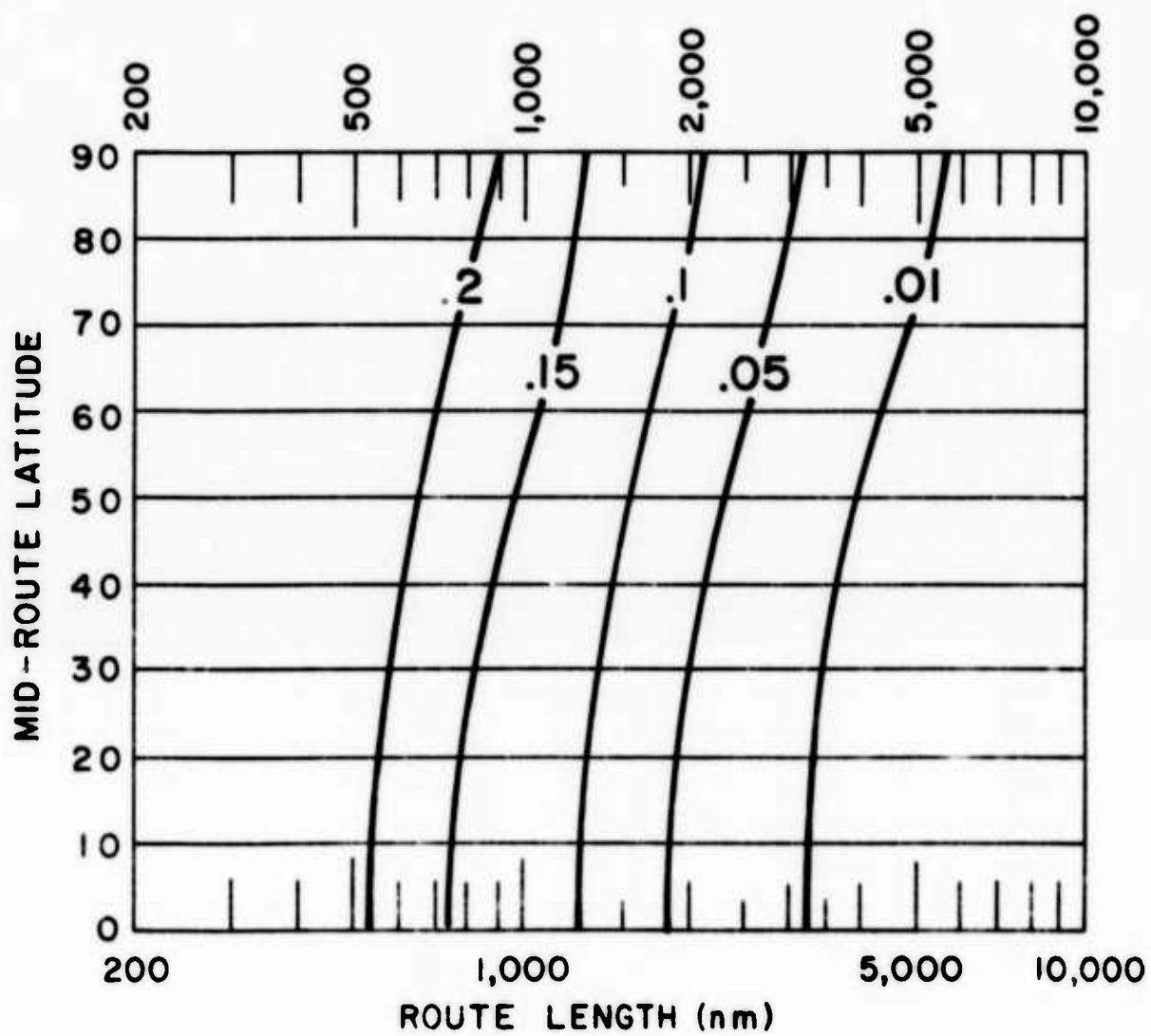
Graph 26. Probability of the Enroute Temperatures Exceeding the Temperatures on the Map, Opposite Page
