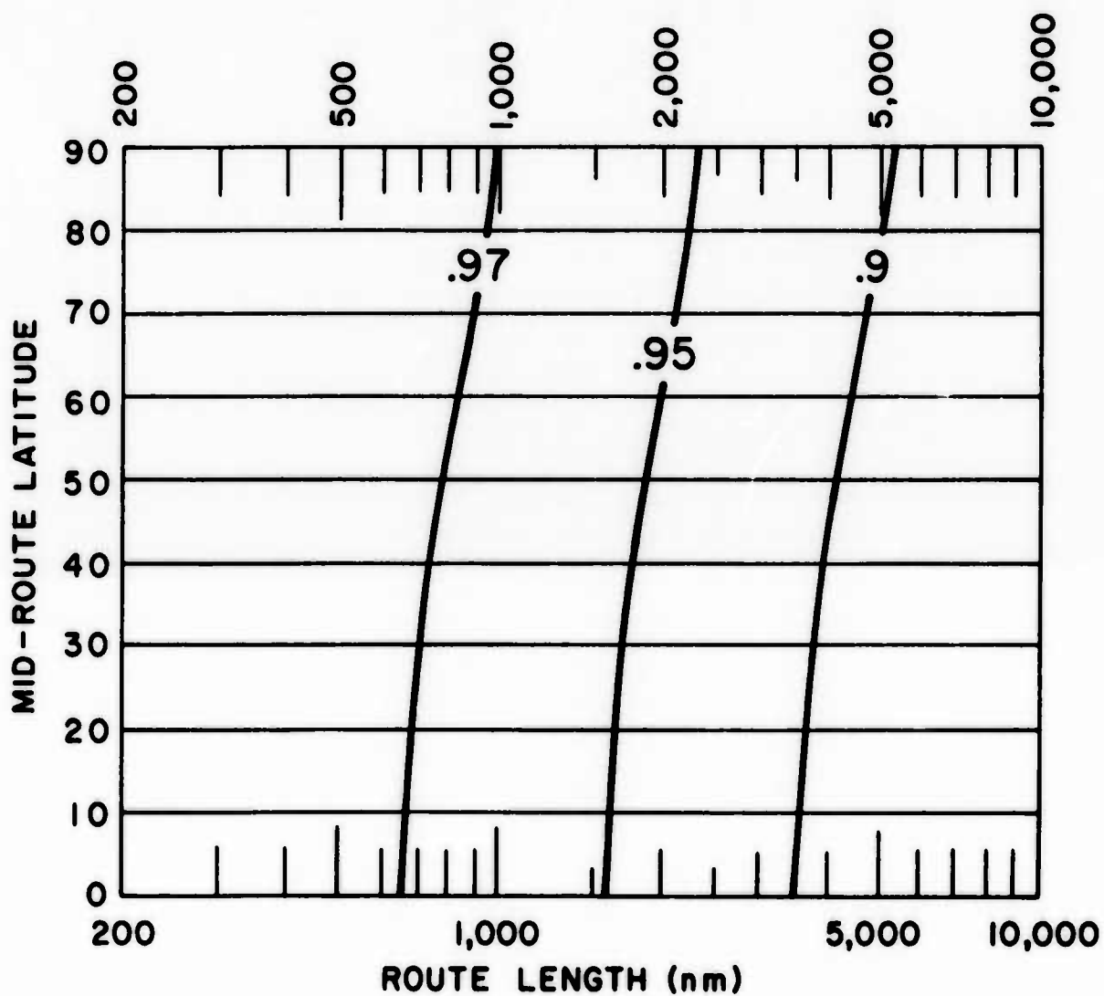
Graph 43. Probability of the Enroute Temperatures Exceeding the Temperatures on the Map, Opposite Page
