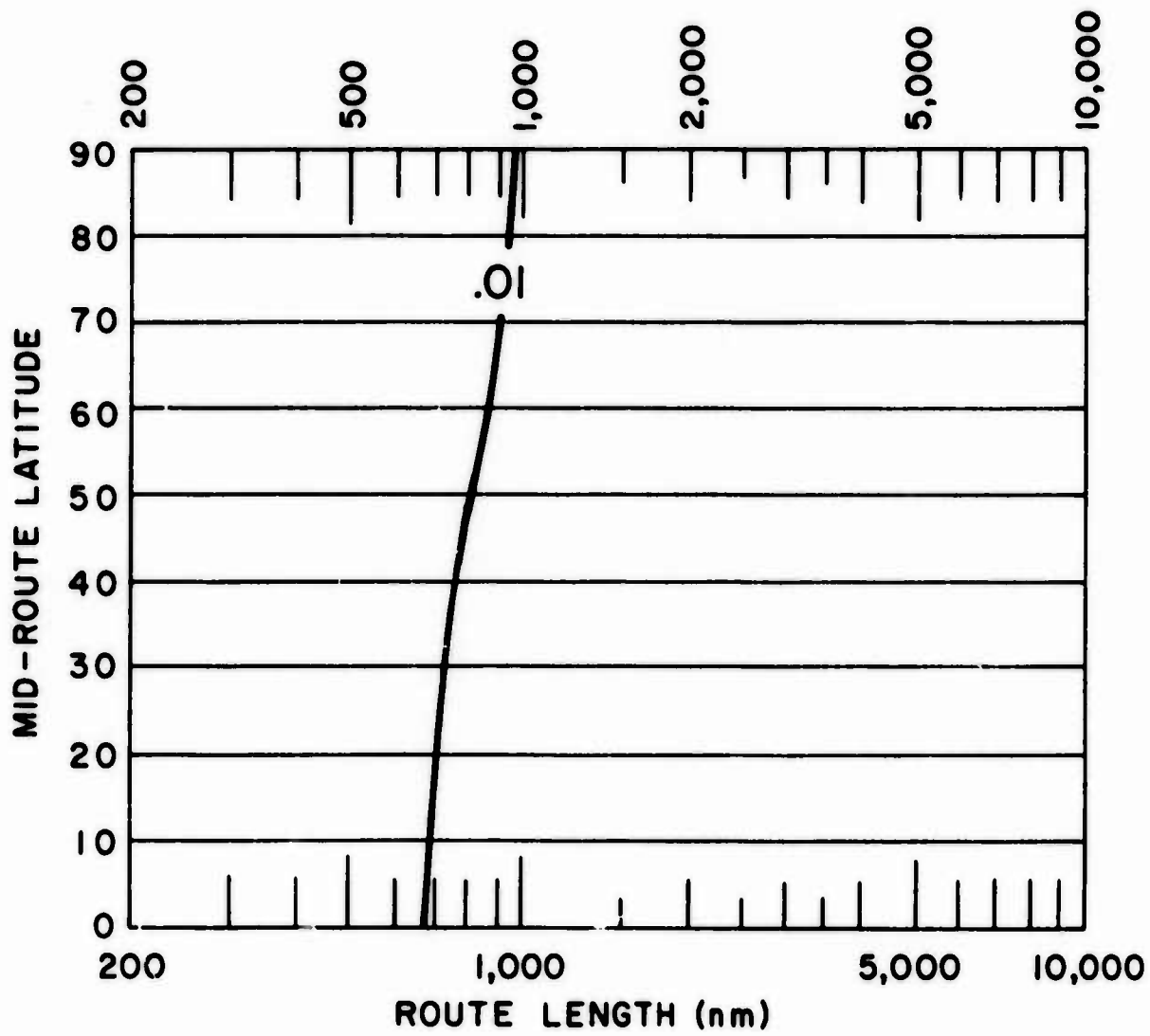
Graph 49. Probability of the Enroute Temperatures Exceeding the Temperatures on the Map, Opposite Page
