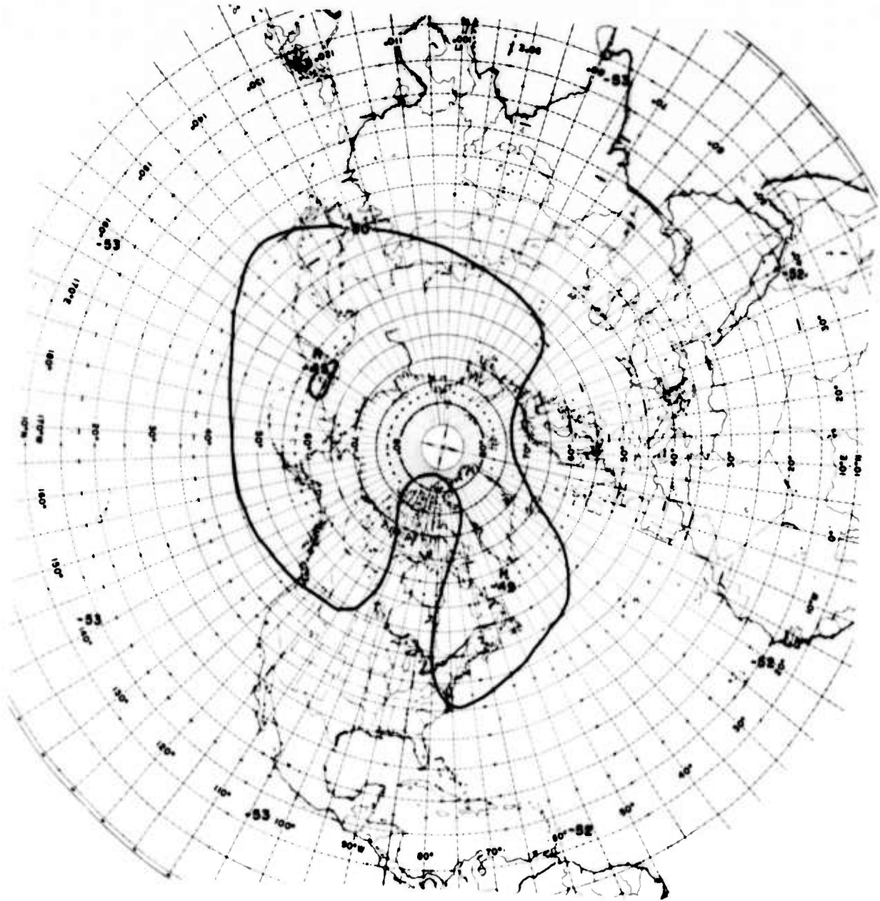
Plate 83. Temperature at 30 mb, in September, October, November, 90 Percentile
