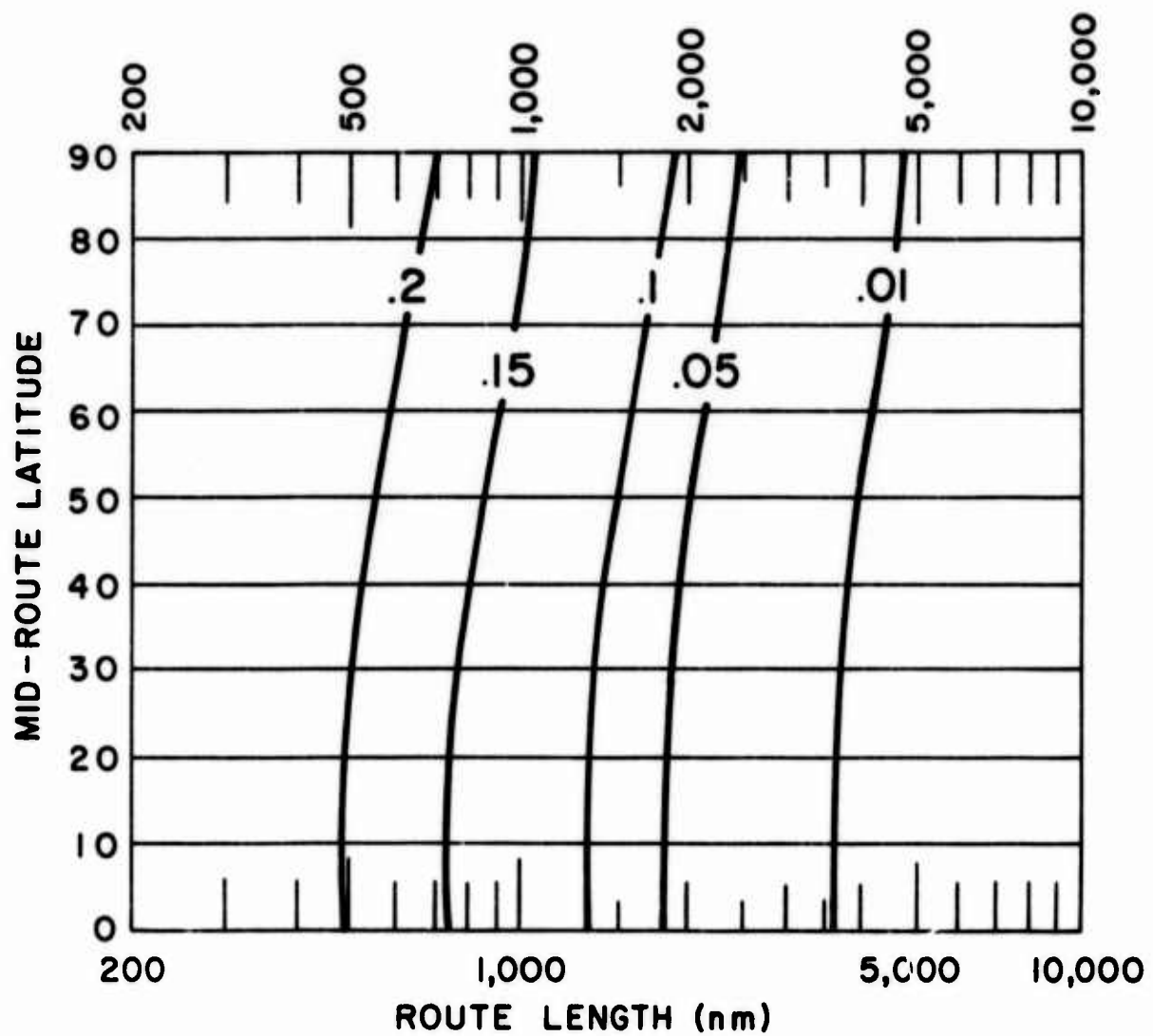
Graph 12. Probability of the Enroute Temperatures Exceeding the Temperatures on the Map, Opposite Page
