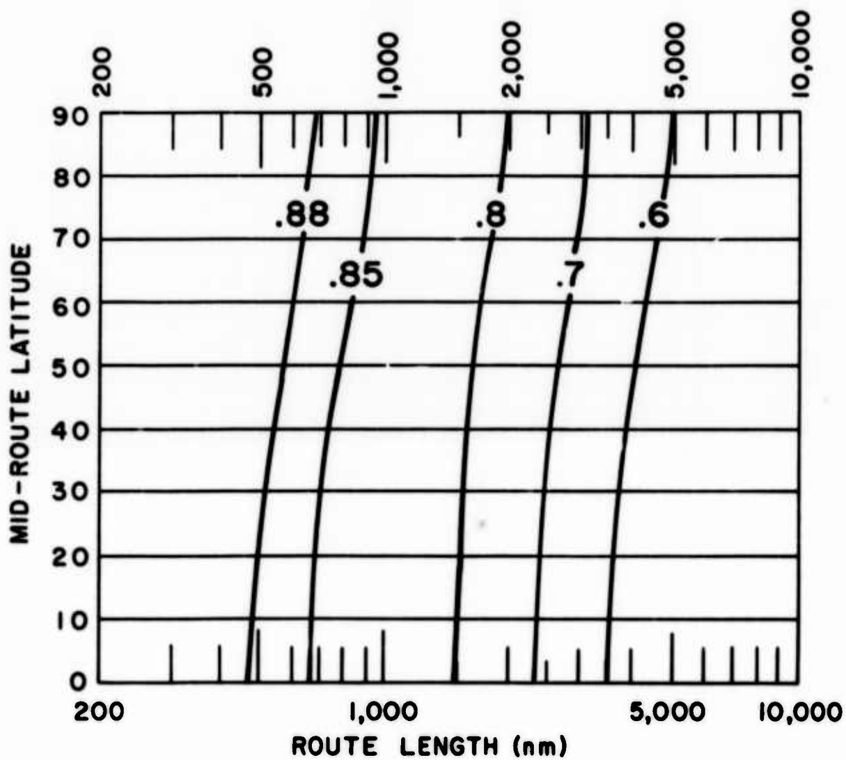
Graph 23. Probability of the Enroute Temperatures Exceeding the Temperatures on the Map, Opposite Page
