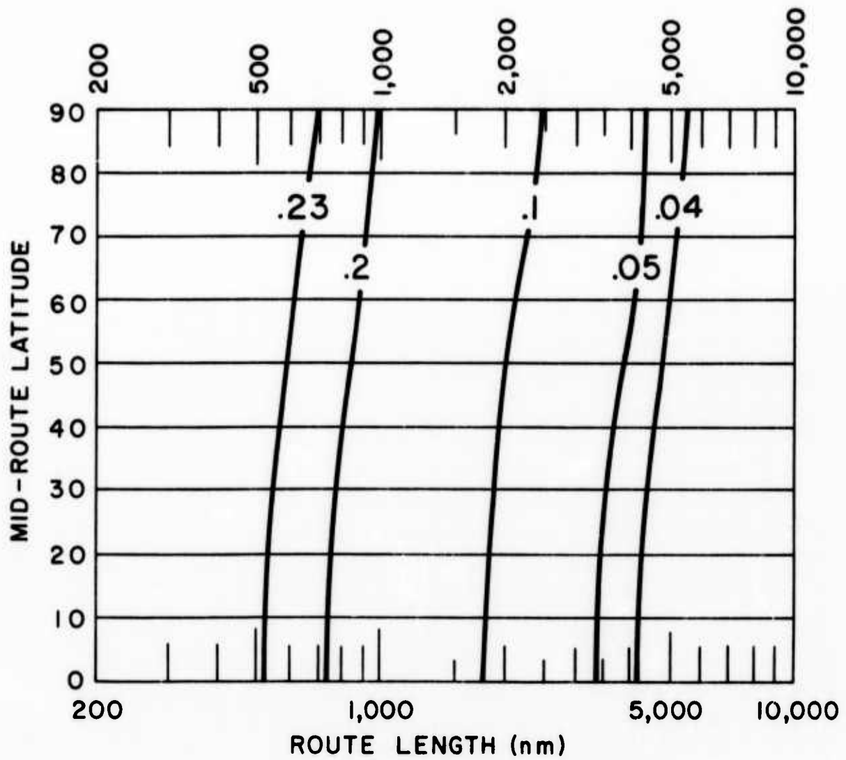
Graph 54. Probability of the Enroute Temperatures Exceeding the Temperatures on the Map, Opposite Page
