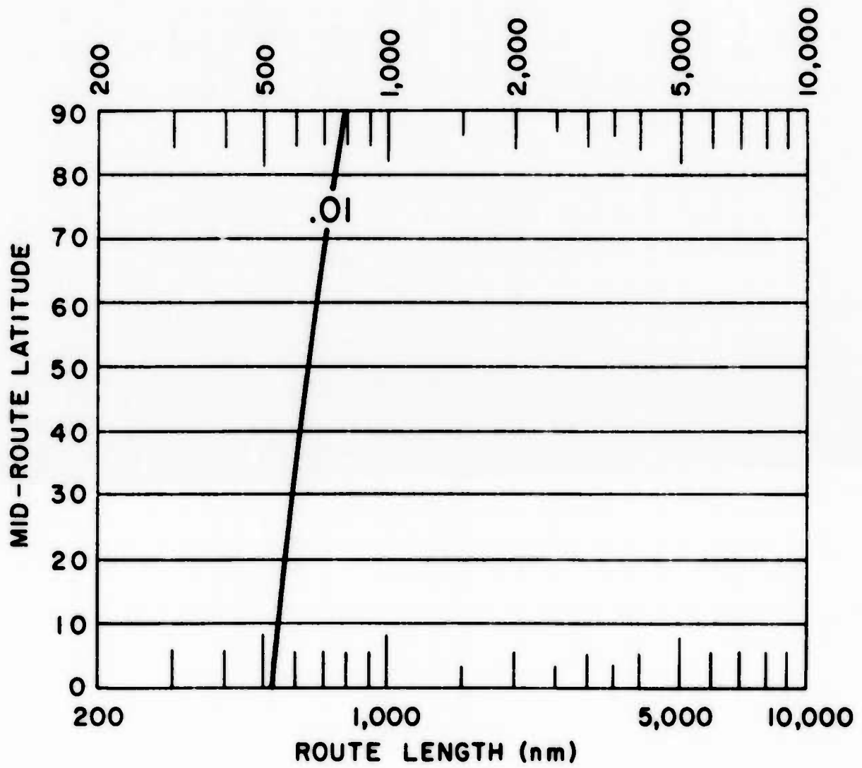
Graph 28. Probability of the Enroute Temperatures Exceeding the Temperatures on the Map, Opposite Page
