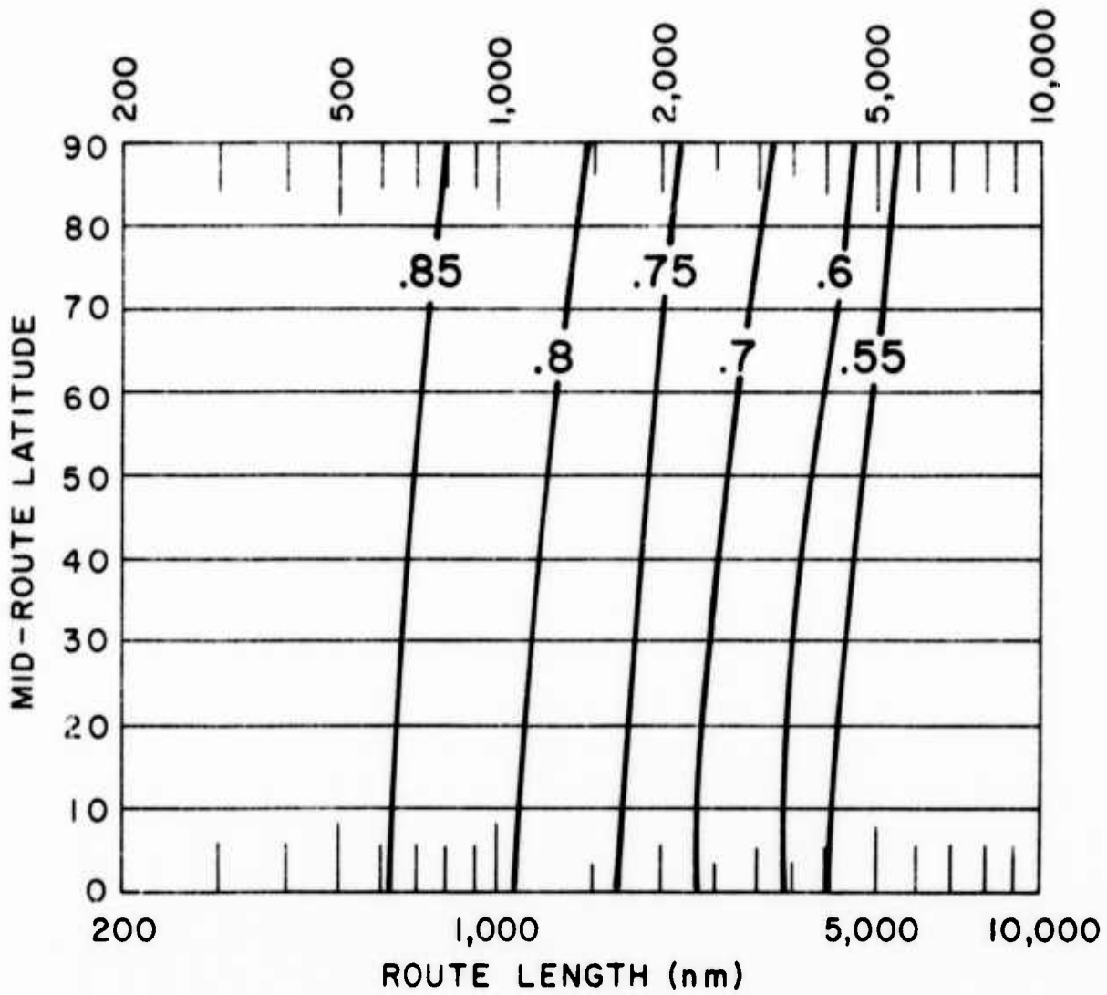
Graph 16. Probability of the Enroute Temperatures Exceeding the Temperatures on the Map, Opposite Page
