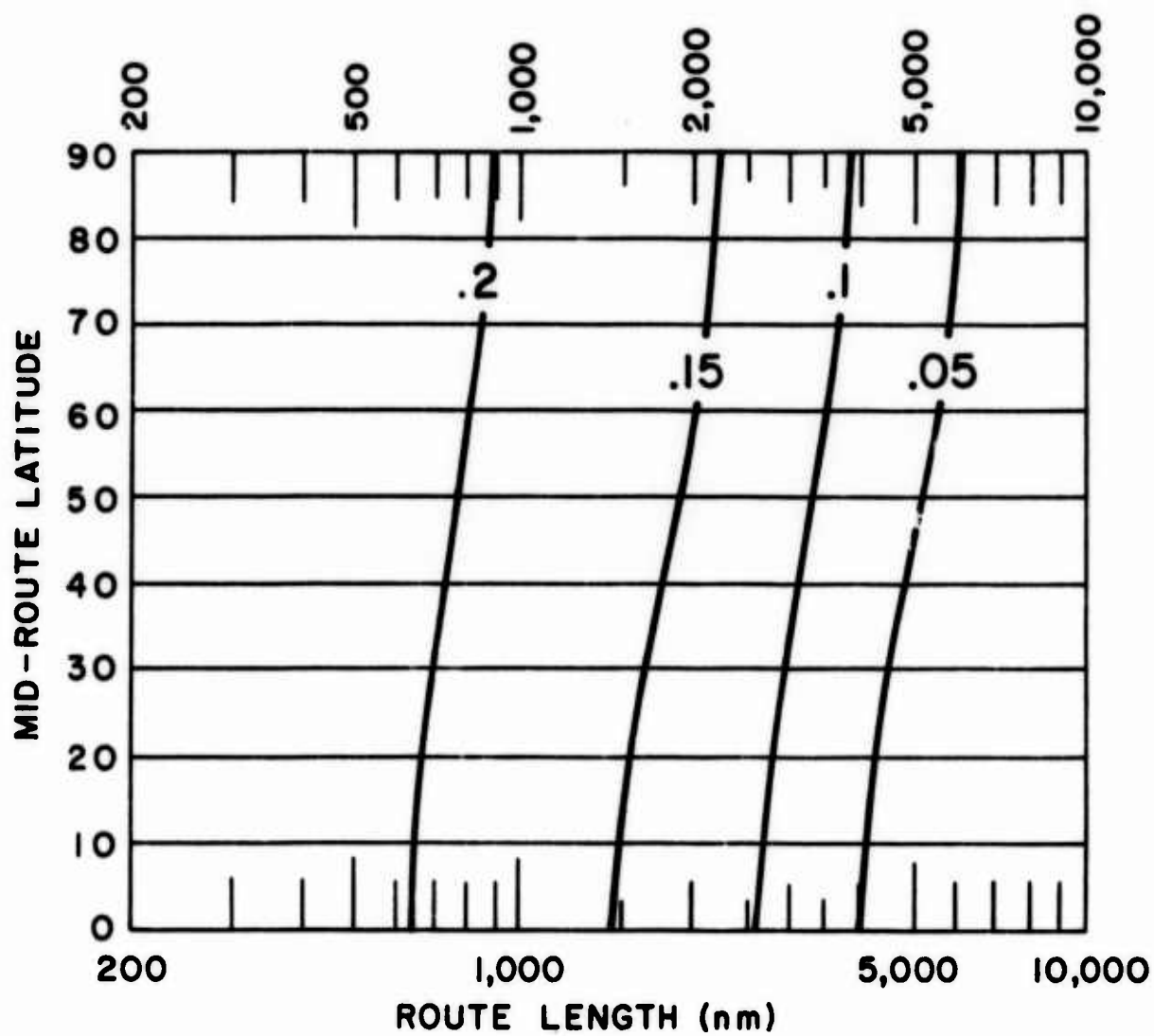
Graph 82. Probability of the Enroute Temperatures Exceeding the Temperatures on the Map, Opposite Page
