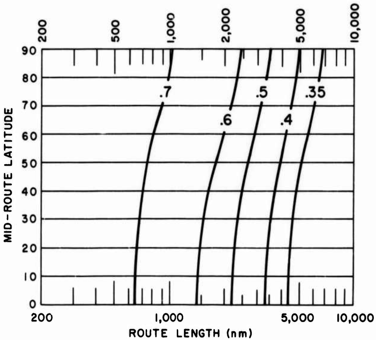
Graph 45. Probability of the Enroute Temperatures Exceeding the Temperatures on the Map, Opposite Page
