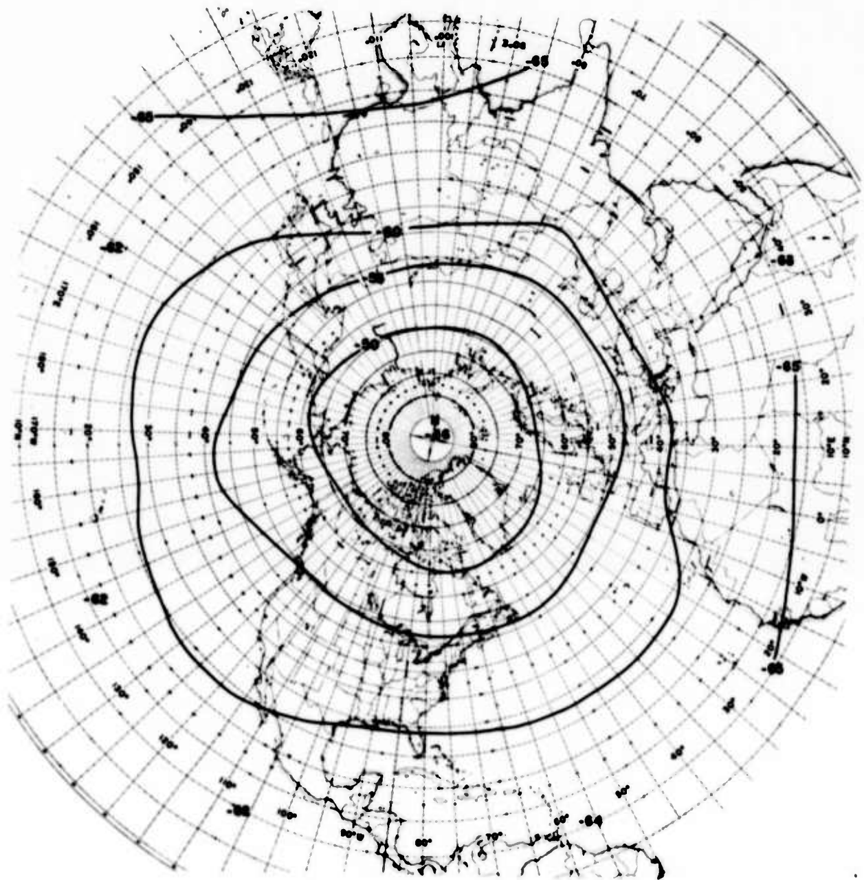
Plate 43. Temperature at 50 mb, in June, July, August, 2 Percentile
