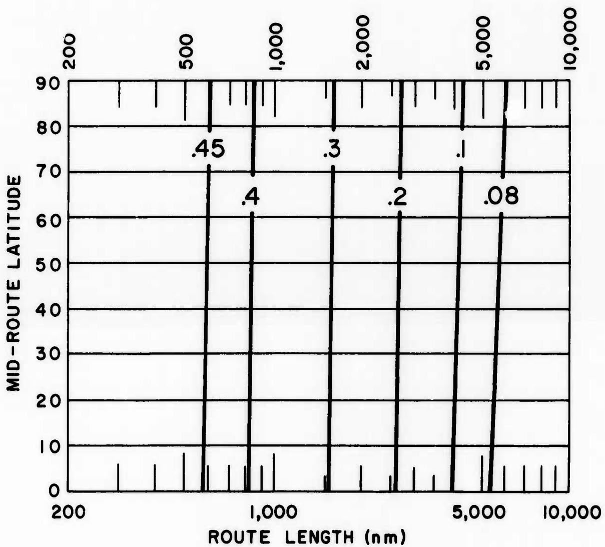
Graph 60. Probability of the Enroute Temperatures Exceeding the Temperatures on the Map, Opposite Page
