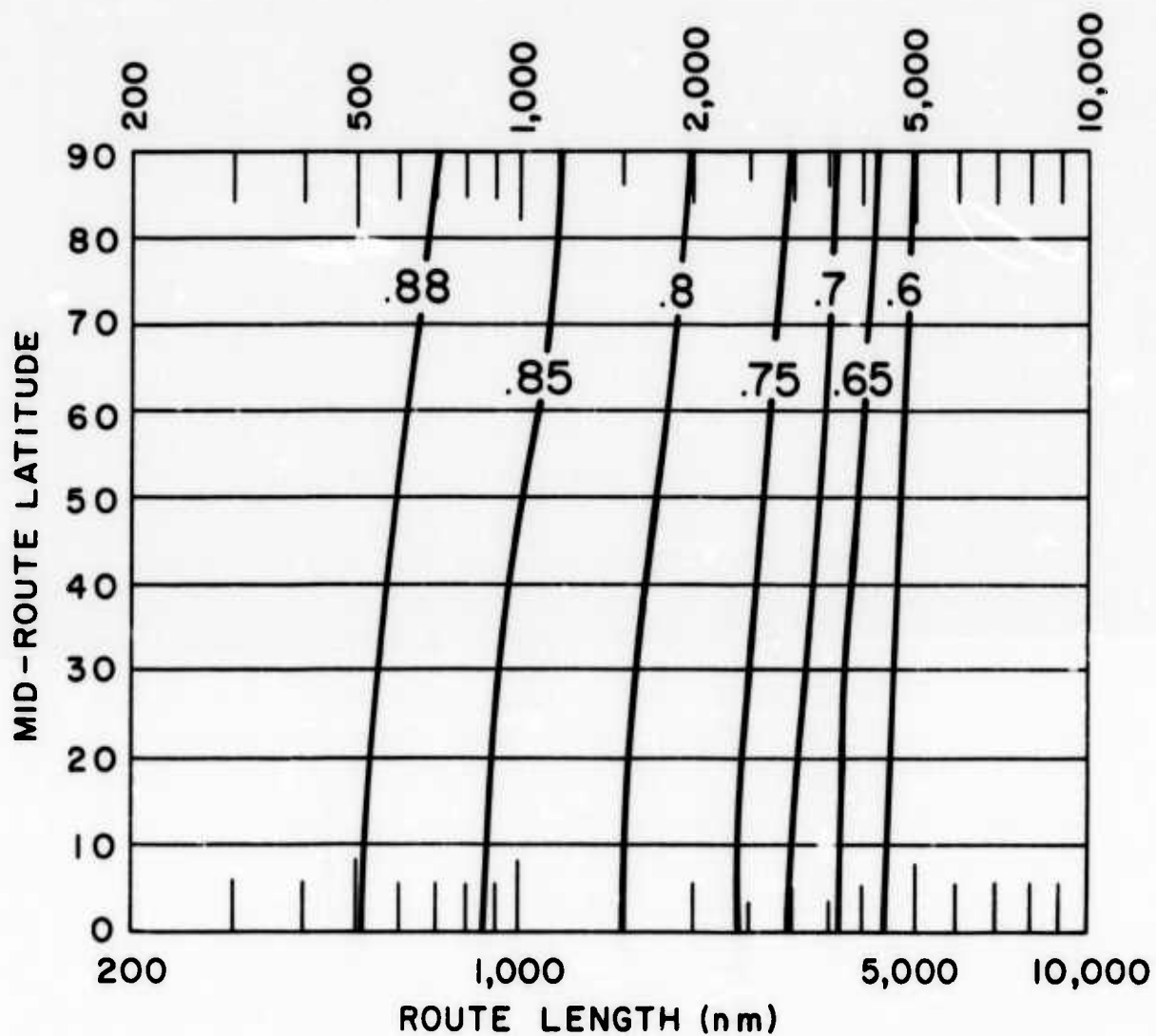
Graph 2. Probability of the Enroute Temperatures Exceeding the Temperatures on the Map, Opposite Page
