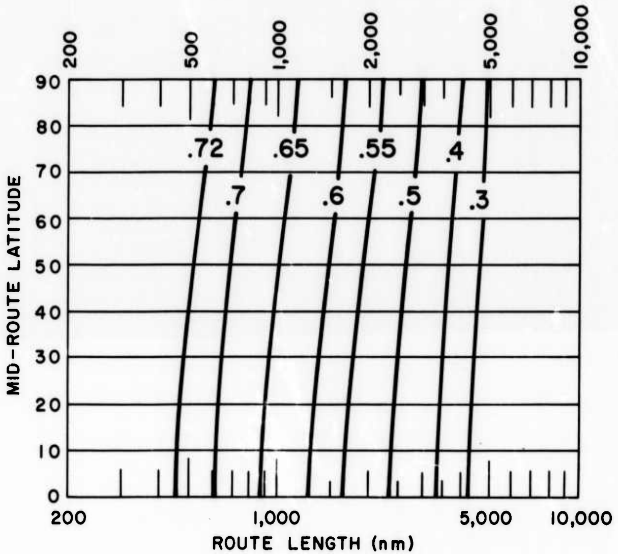
Graph 31. Probability of the Enroute Temperatures Exceeding the Temperatures on the Map, Opposite Page
