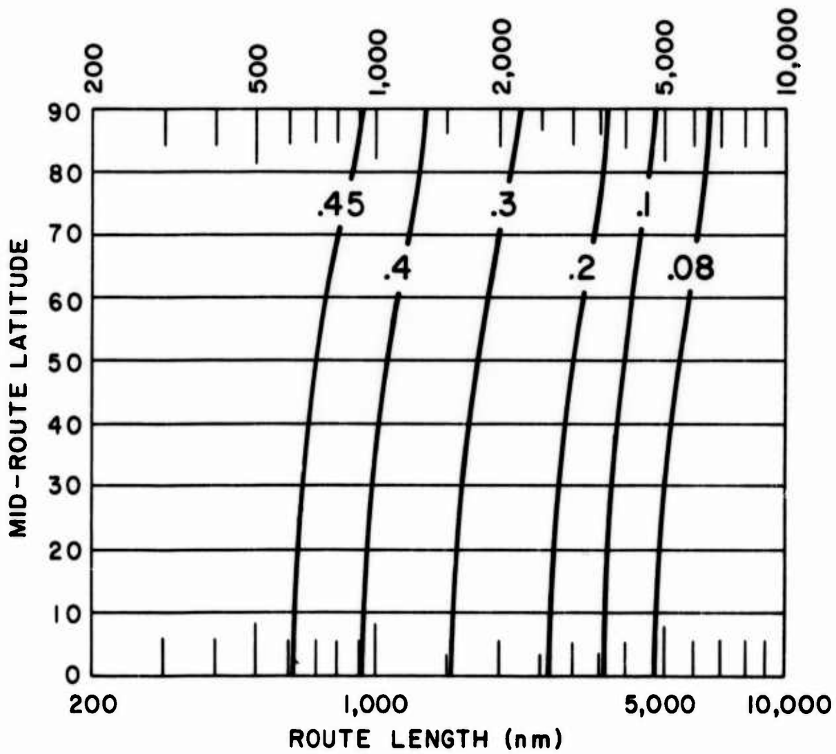
Graph 46. Probability of the Enroute Temperatures Exceeding the Temperatures on the Map, Opposite Page
