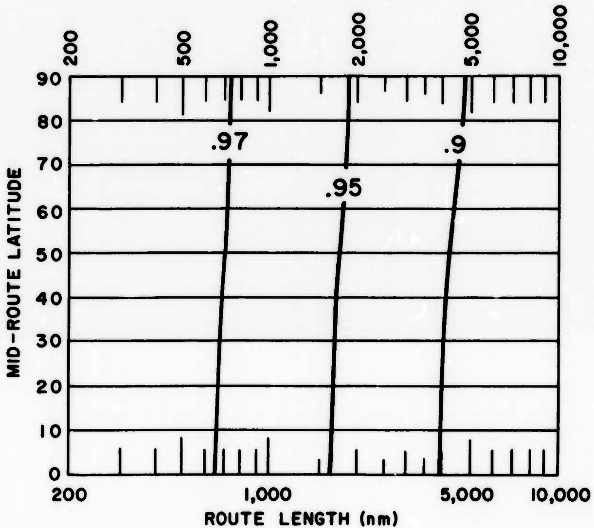
Graph 71. Probability of the Enroute Temperatures Exceeding the Temperatures on the Map, Opposite Page
