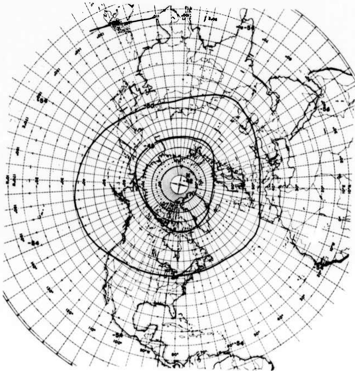
Plate 73. Temperature at 30 mb, in June, July, August, 25 Percentile
