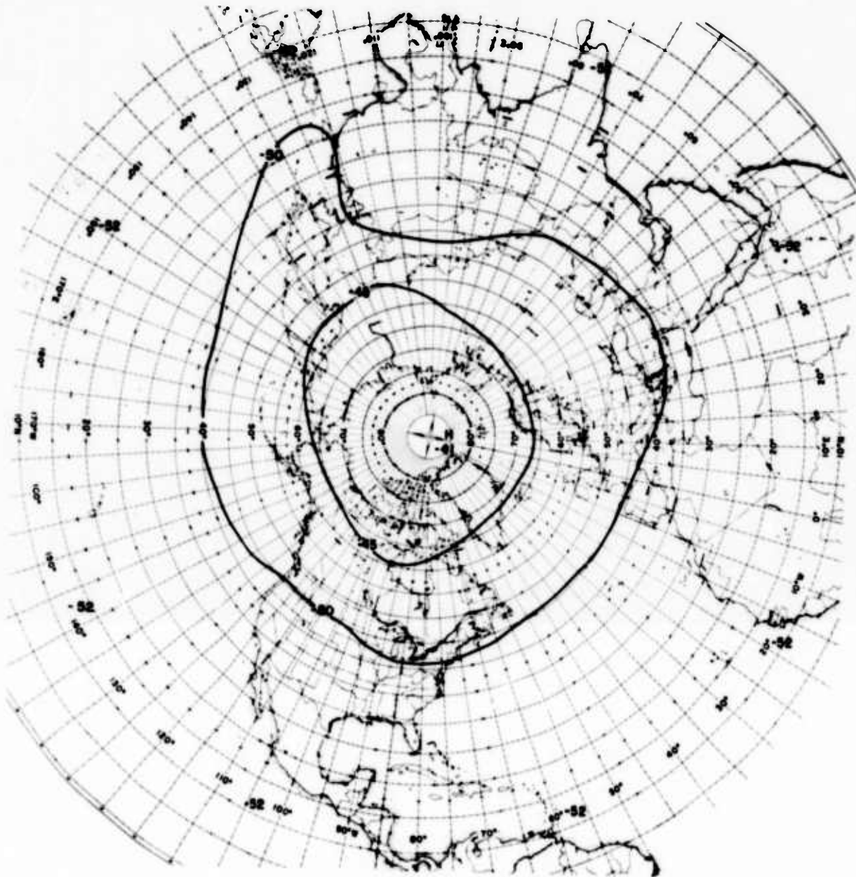
Plate 69. Temperature at 30 mb, in March, April, May, 90 Percentile
