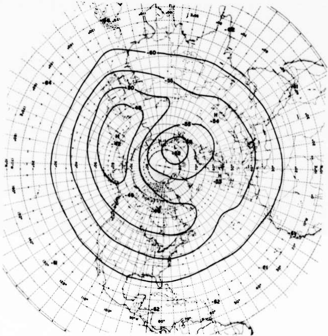
Plate 34. Temperature at 50 mb, in December, January, February, 90 Percentile
