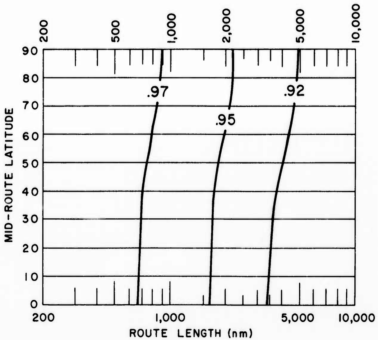
Graph 50. Probability of the Enroute Temperatures Exceeding the Temperatures on the Map, Opposite Page
