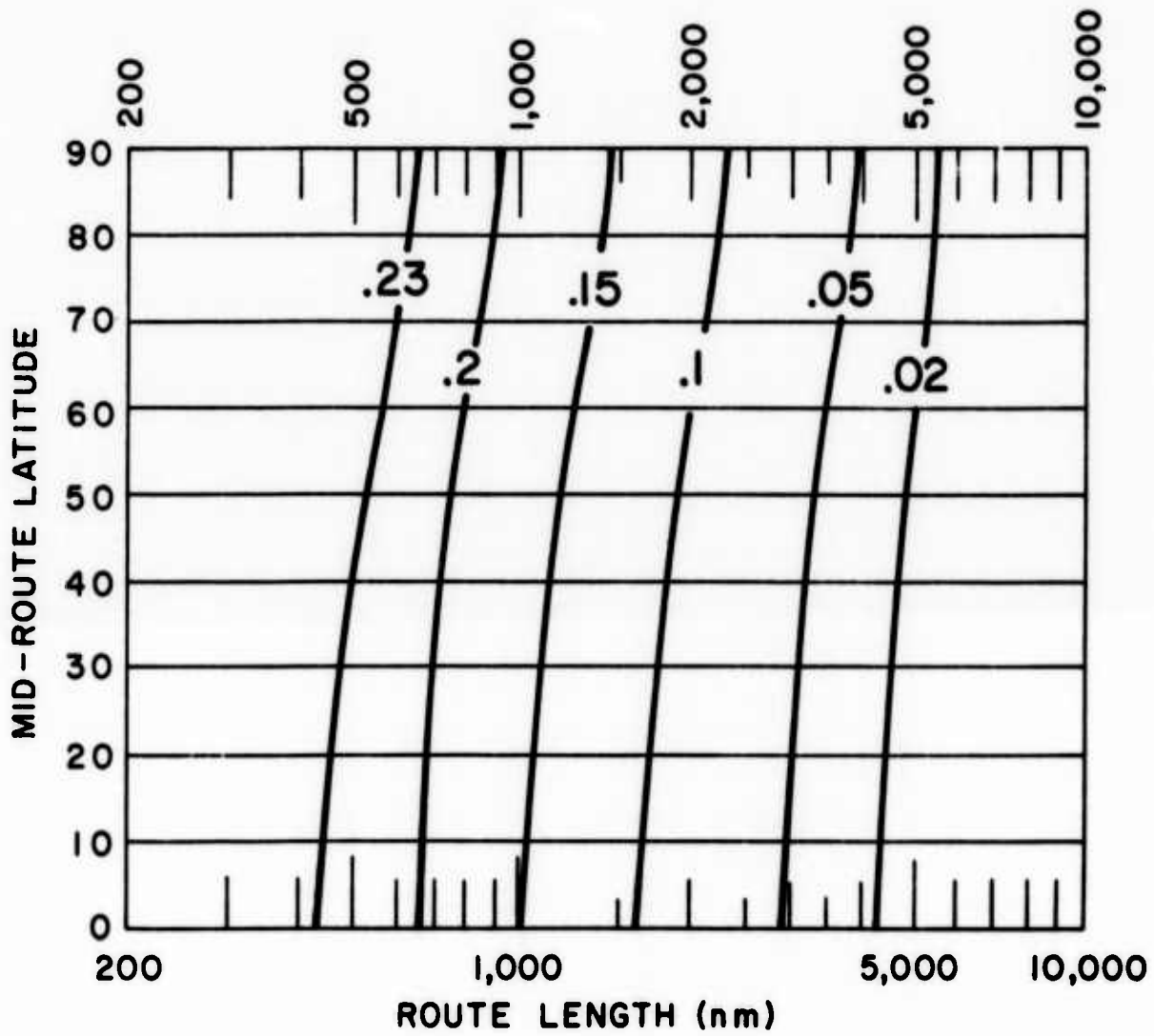
Graph 40. Probability of the Enroute Temperatures Exceeding the Temperatures on the Map, Opposite Page
