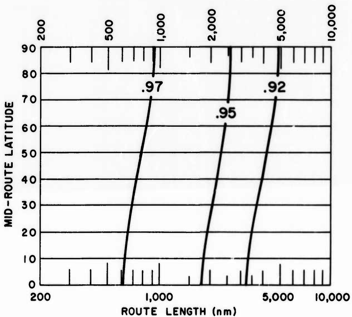
Graph 78. Probability of the Enroute Temperatures Exceeding the Temperatures on the Map, Opposite Page
