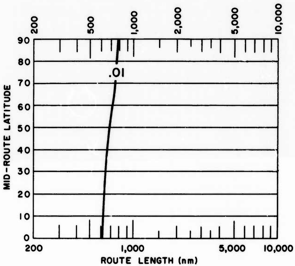
Graph 77. Probability of the Enroute Temperatures Exceeding the Temperatures on the Map, Opposite Page
