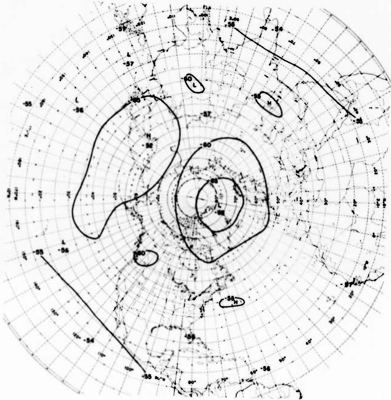
Plate 65. Temperature at 30 mb, in March, April, May, 10 Percentile
