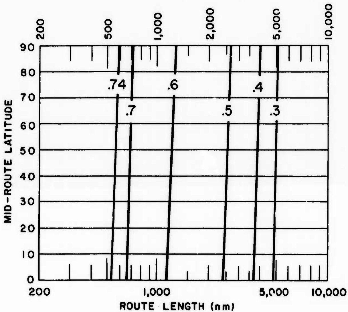
Graph 59. Probability of the Enroute Temperatures Exceeding the Temperatures on the Map, Opposite Page
