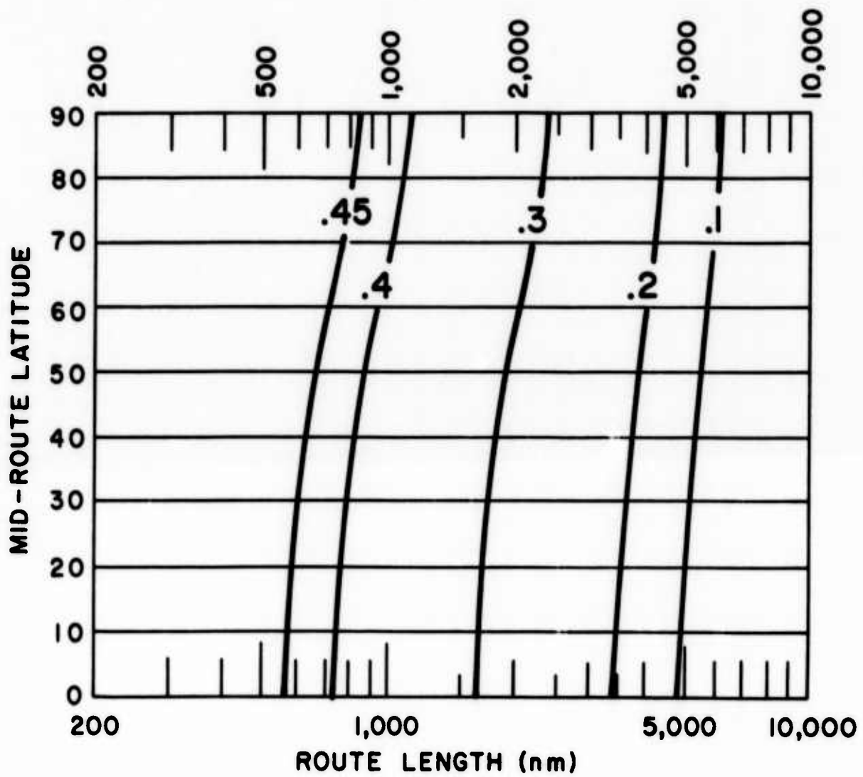
Graph 39. Probability of the Enroute Temperatures Exceeding the Temperatures on the Map, Opposite Page
