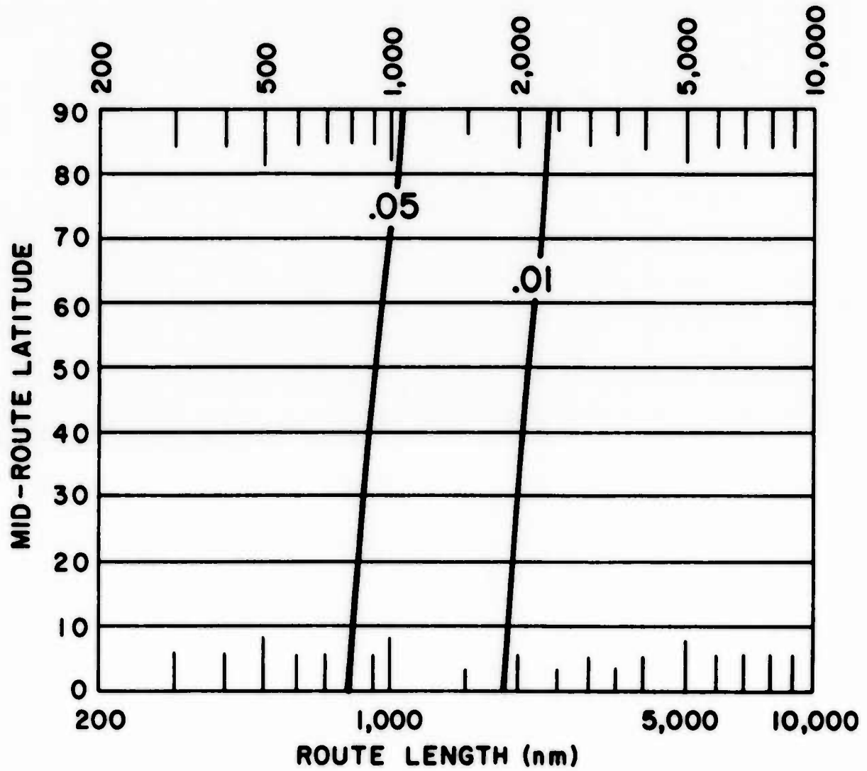
Graph 41. Probability of the Enroute Temperatures Exceeding the Temperatures on the Map, Opposite Page
