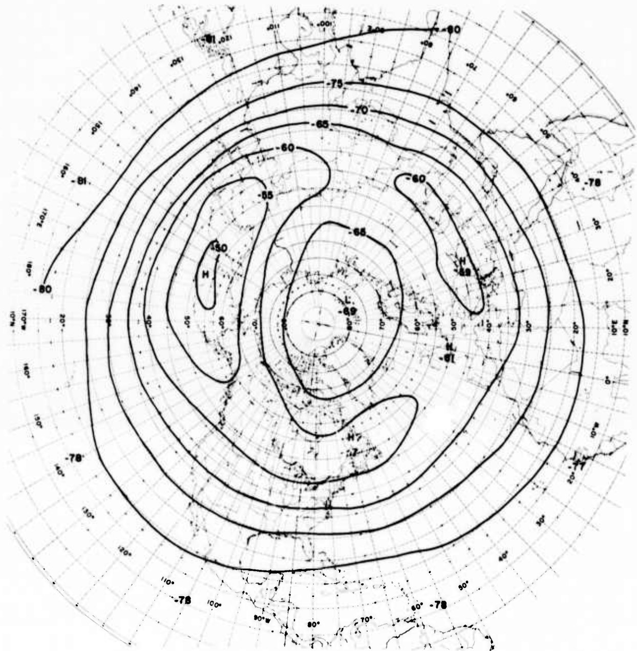
Plate 3. Temperature at 100 mb, in December, January, and February, 25 Percentile
