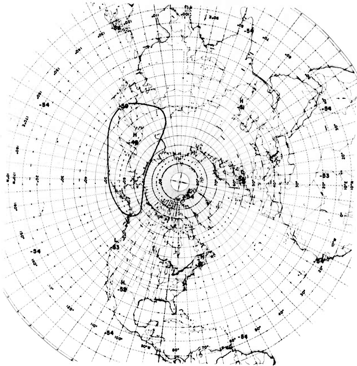
Plate 82. Temperature at 30 mb, in September, October, November, 75 Percentile
