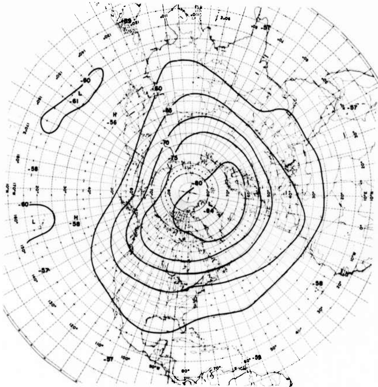
Plate 57. Temperature at 30 mb, in December, January, February, 2 Percentile
