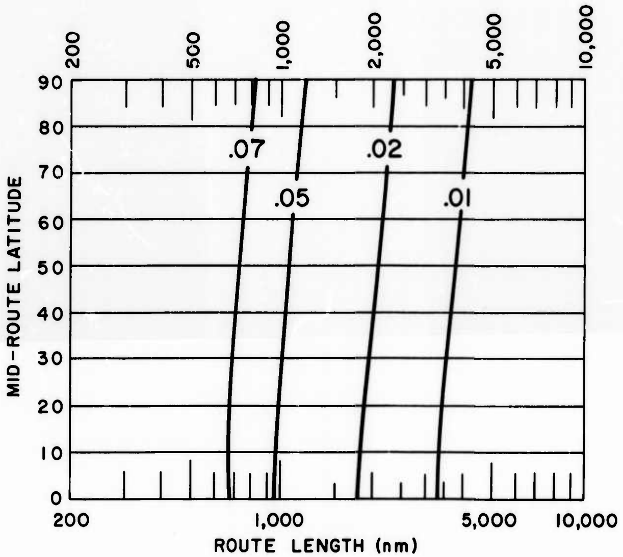
Graph 55. Probability of the Enroute Temperatures Exceeding the Temperatures on the Map, Opposite Page
