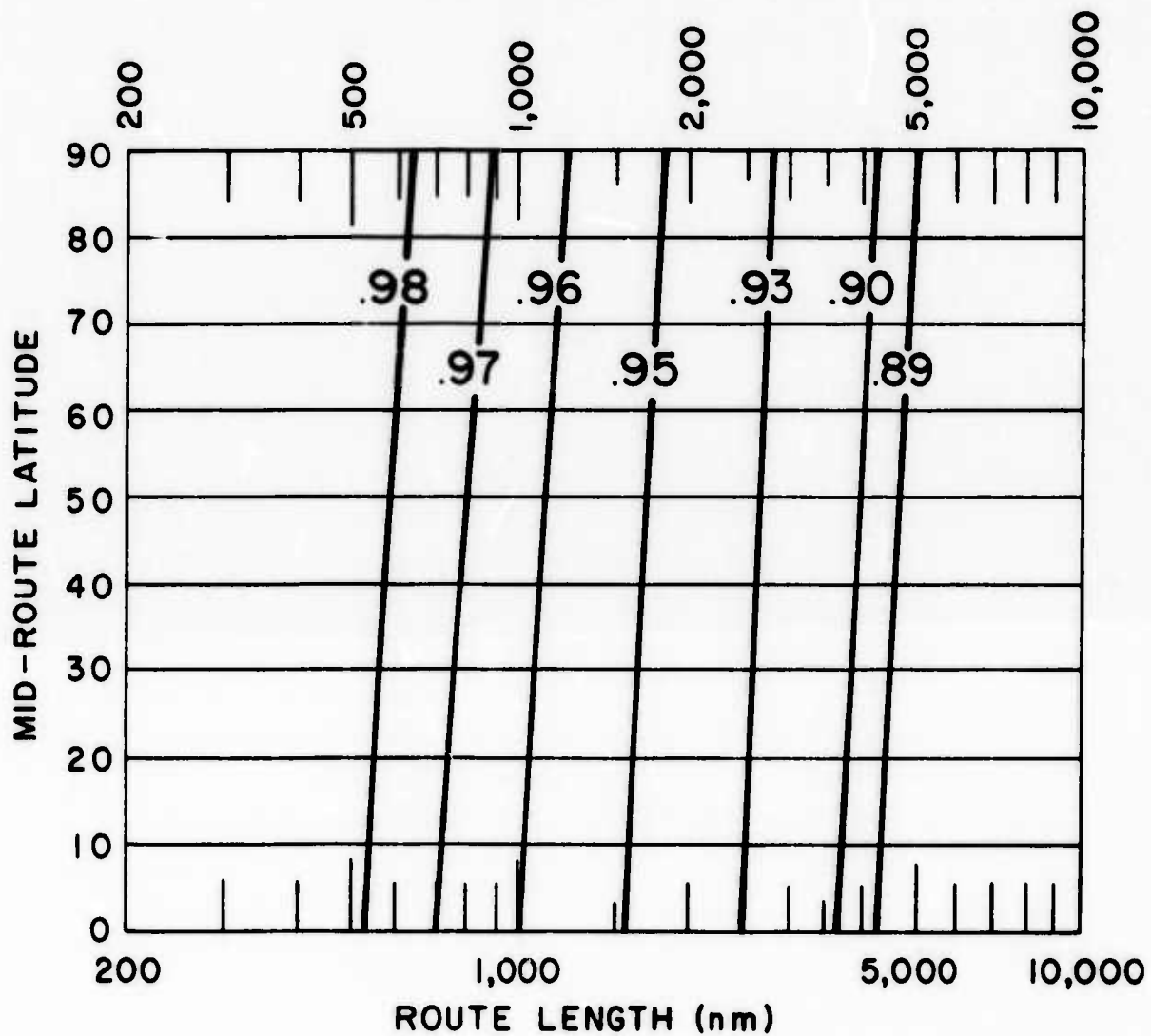
Graph 1. Probability of the Enroute Temperatures Exceeding the Temperatures on the Map, Opposite Page
