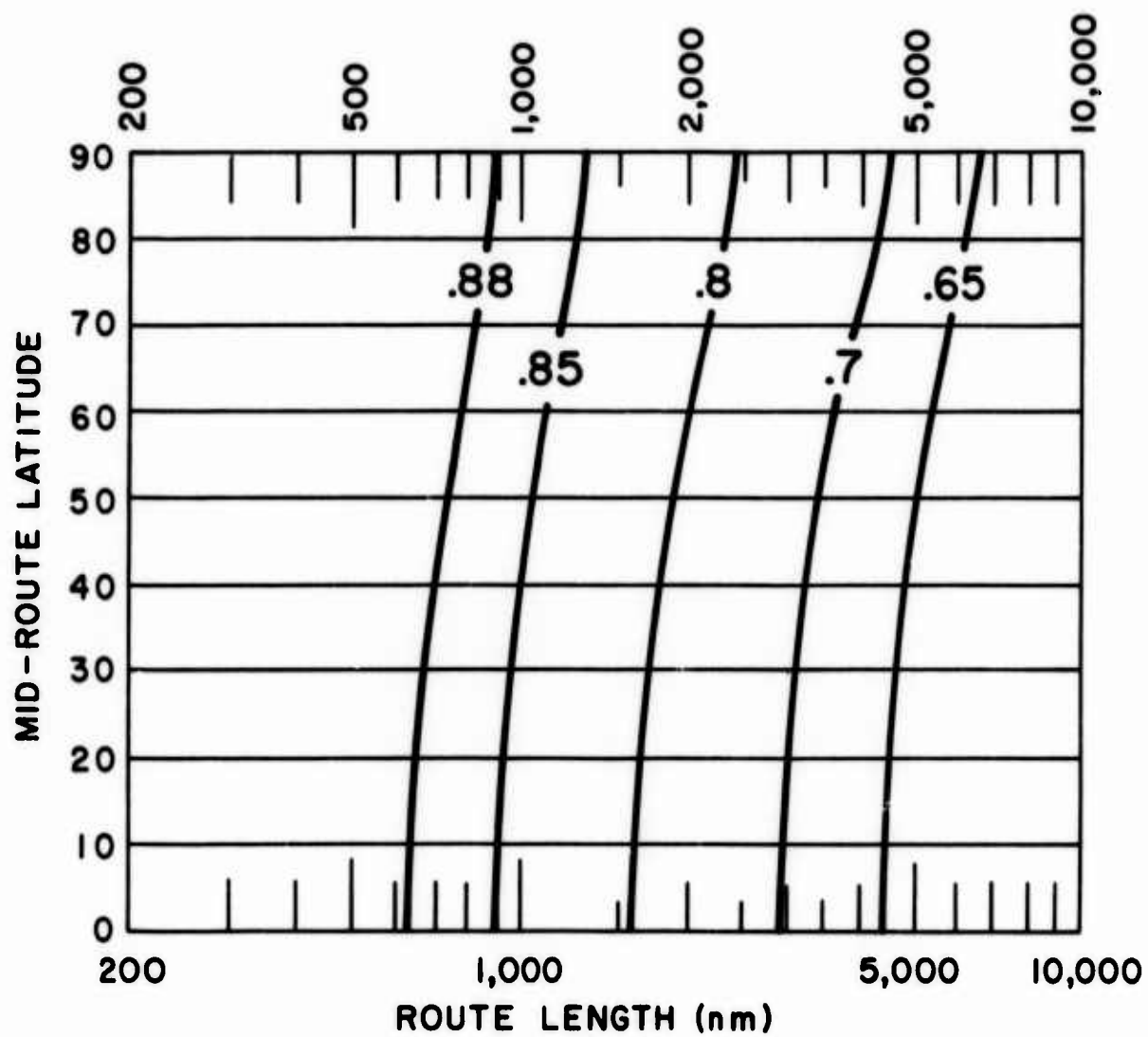
Graph 44. Probability of the Enroute Temperatures Exceeding the Temperatures on the Map, Opposite Page
