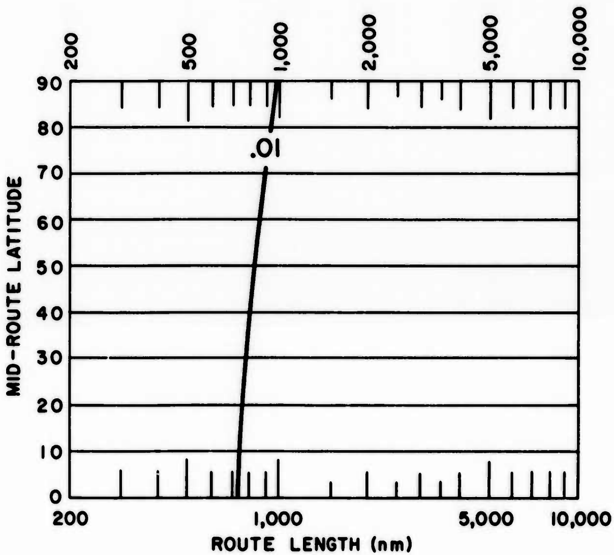
Graph 42. Probability of the Enroute Temperatures Exceeding the Temperatures on the Map, Opposite Page
