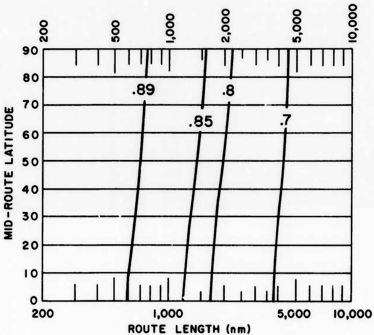
Graph 65. Probability of the Enroute Temperatures Exceeding the Temperatures on the Map, Opposite Page
