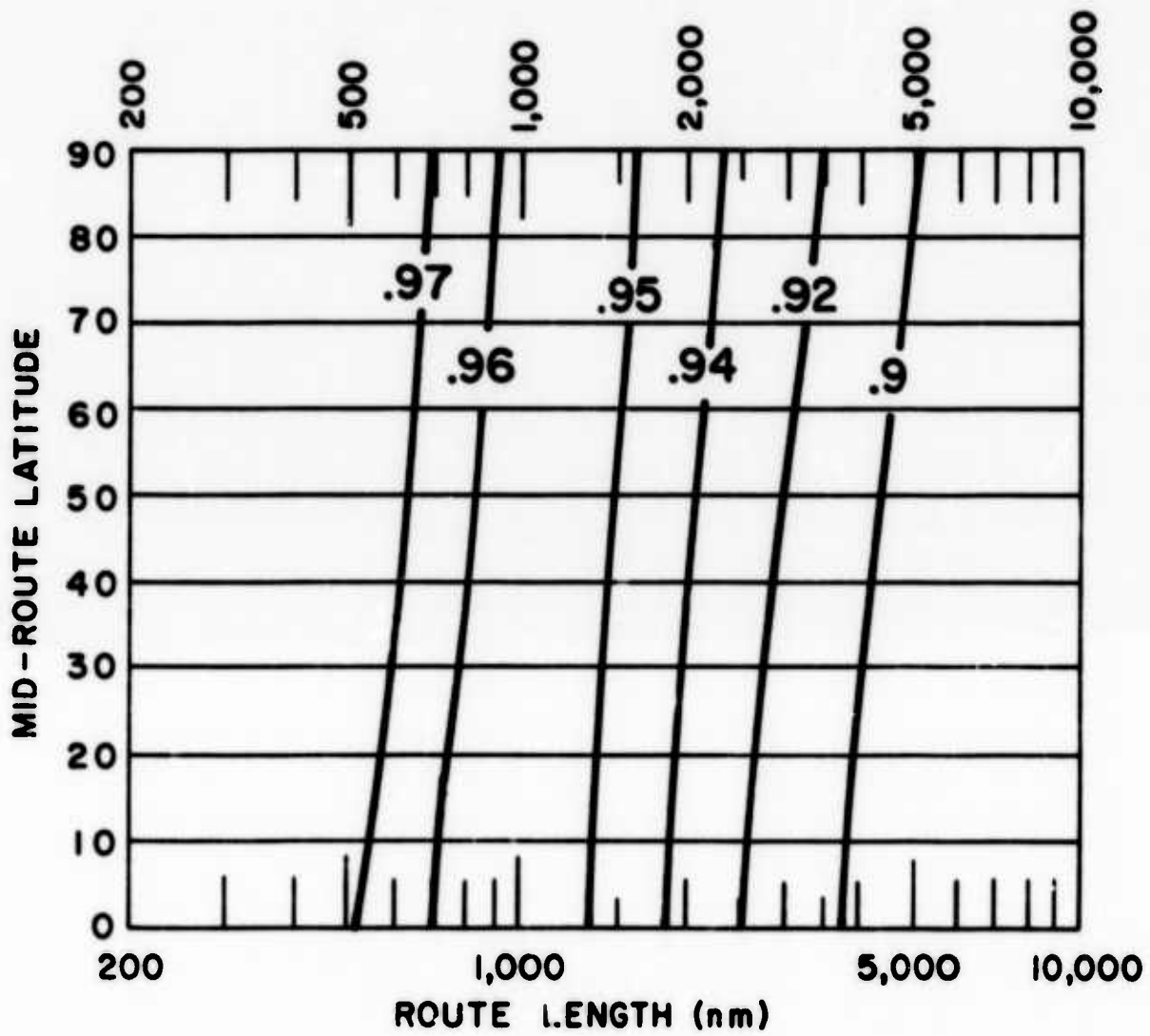
Graph 36. Probability of the Enroute Temperatures Exceeding the Temperatures on the Map, Opposite Page
