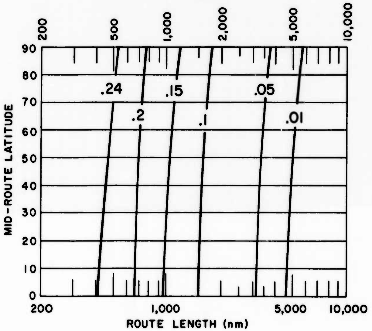
Graph 33. Probability of the Enroute Temperatures Exceeding the Temperatures on the Map, Opposite Page
