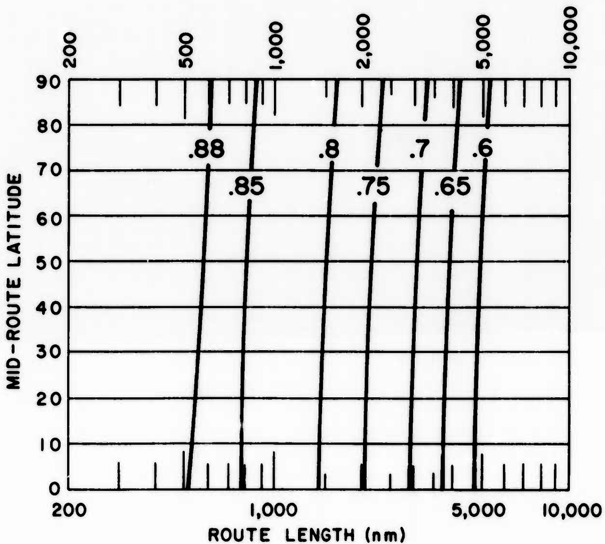
Graph 30. Probability of the Enroute Temperatures Exceeding the Temperatures on the Map, Opposite Page
