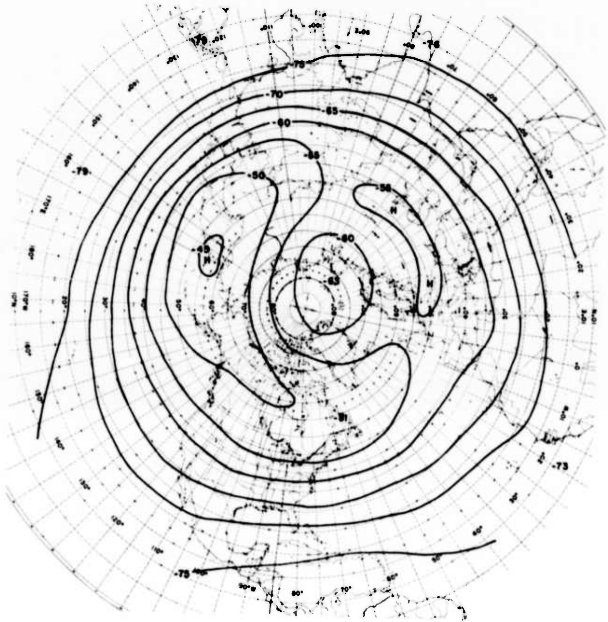
Plate 5. Temperature at 100 mb, in December, January, and February, 75 Percentile
