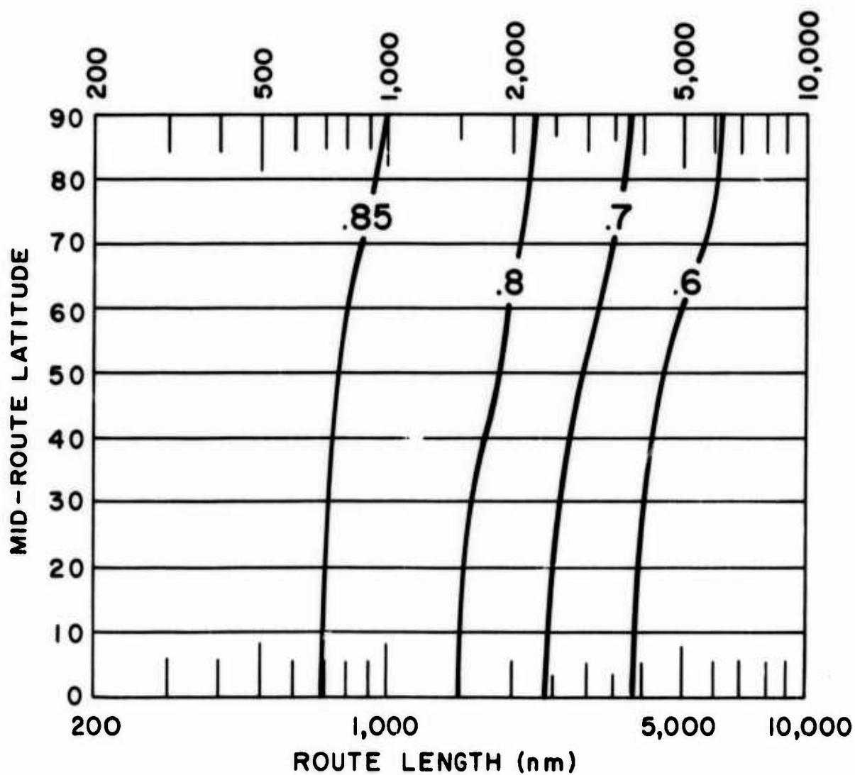
Graph 9. Probability of the Enroute Temperatures Exceeding the Temperatures on the Map, Opposite Page
