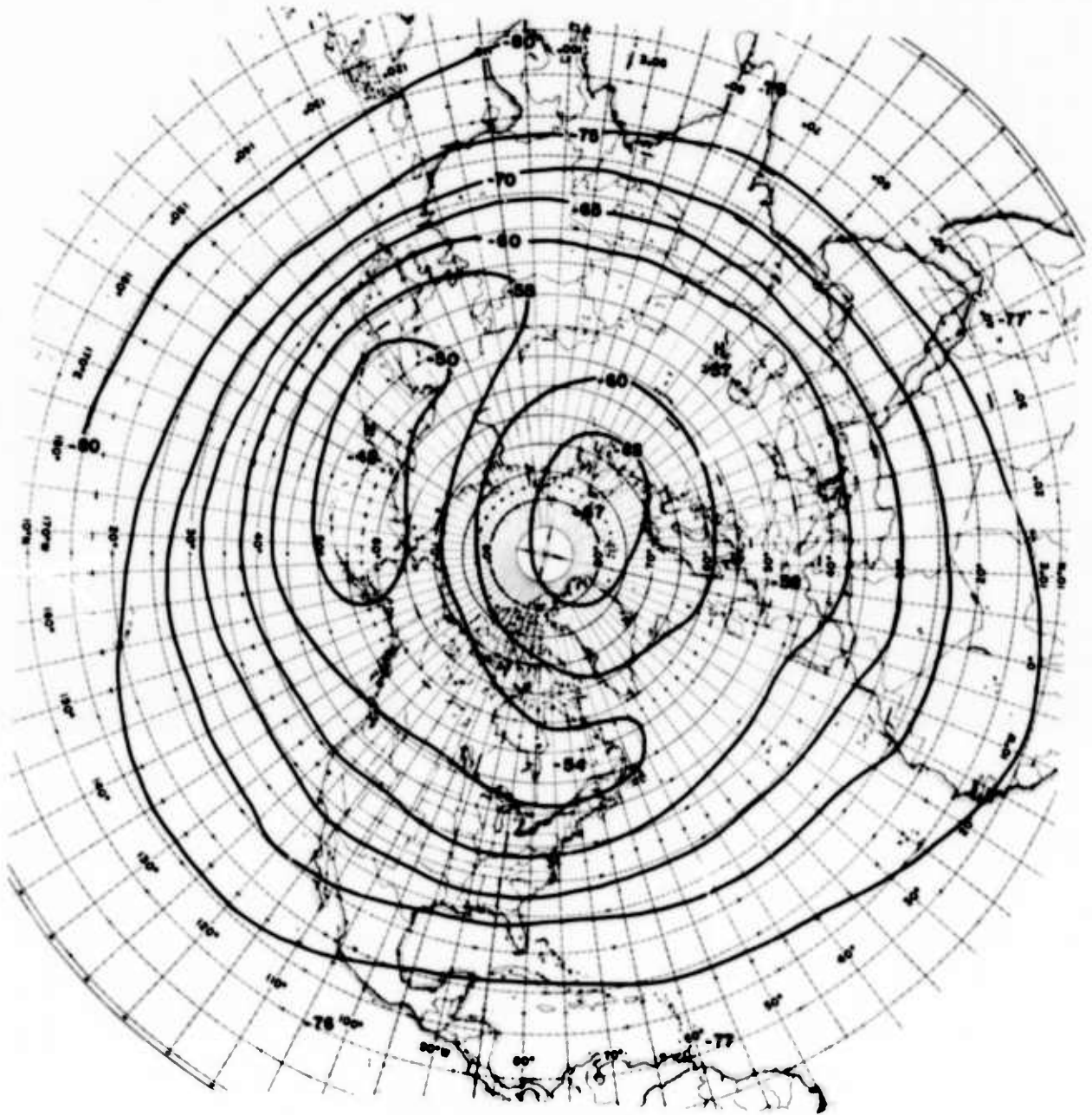
Plate 4. Temperature at 100 mb, in December, January, and February, 50 Percentile
