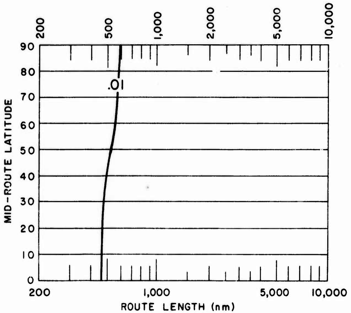
Graph 14. Probability of the Enroute Temperatures Exceeding the Temperatures on the Map, Opposite Page
