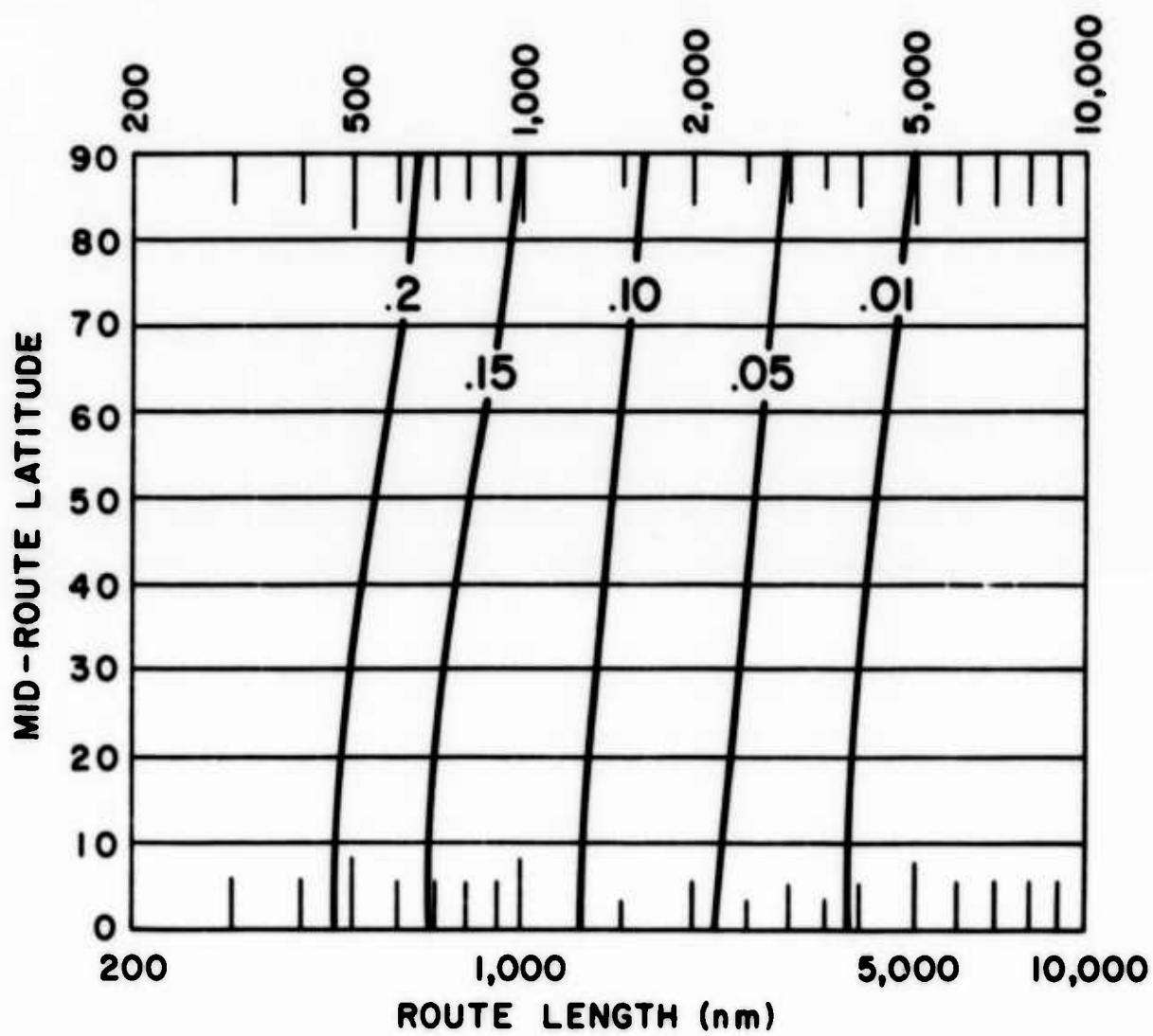
Graph 5. Probability of the Enroute Temperatures Exceeding the Temperatures on the Map, Opposite Page
