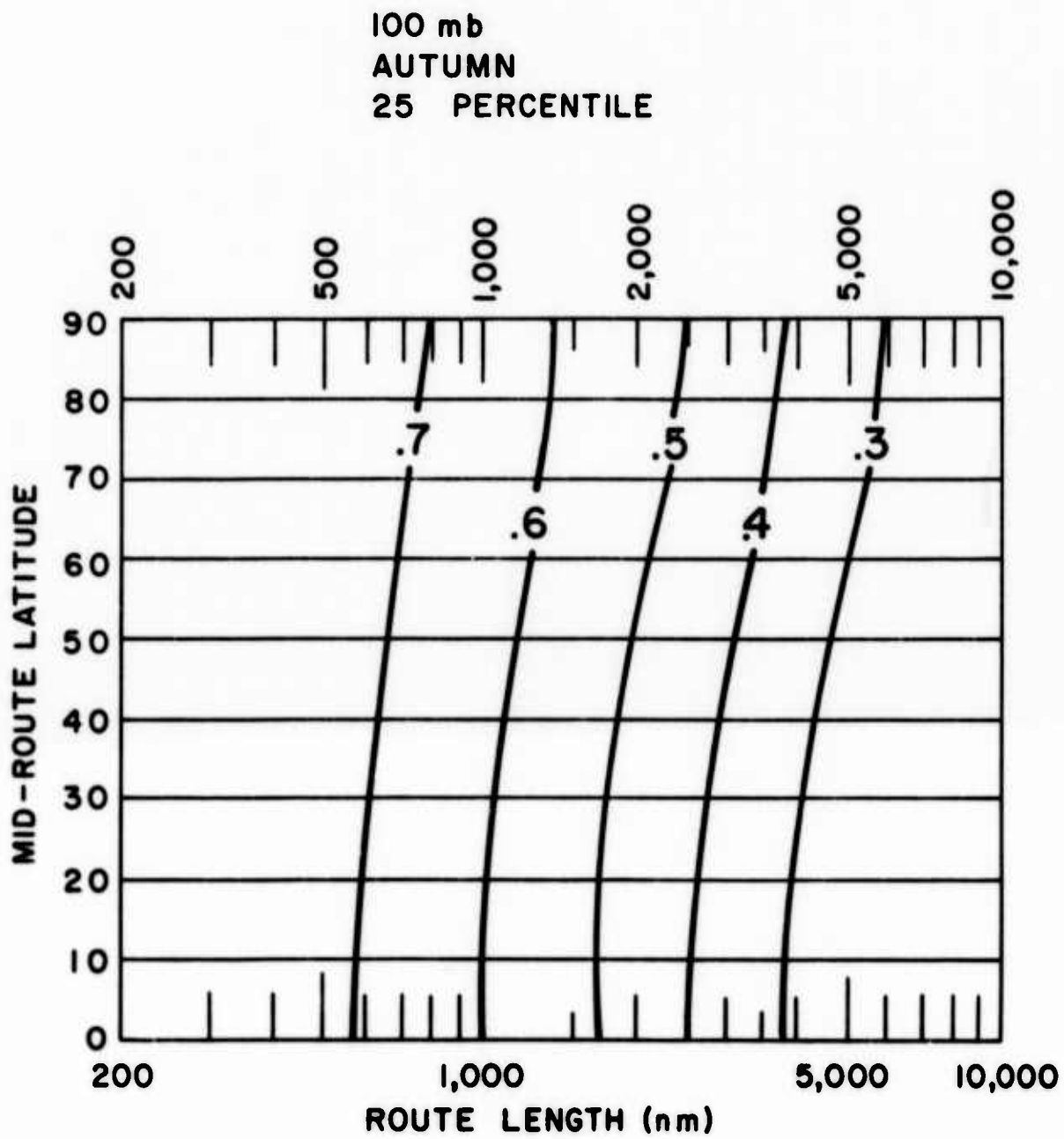
Graph 24. Probability of the Enroute Temperatures Exceeding the Temperatures on the Map, Opposite Page
