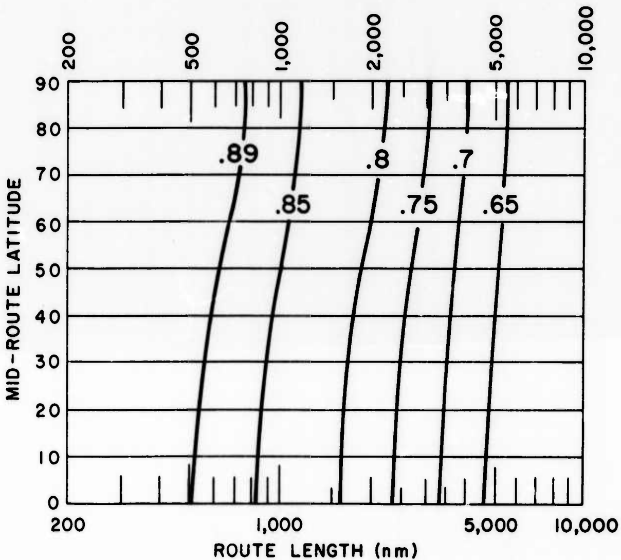
Graph 37. Probability of the Enroute Temperatures Exceeding the Temperatures on the Map, Opposite Page
