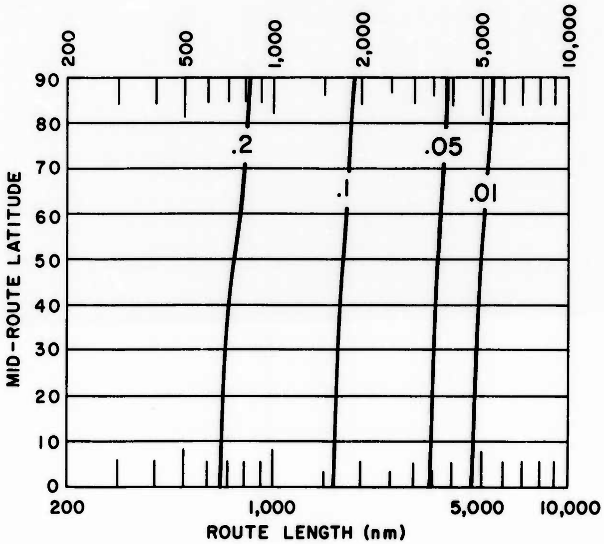
Graph 75. Probability of the Enroute Temperatures Exceeding the Temperatures on the Map, Opposite Page
