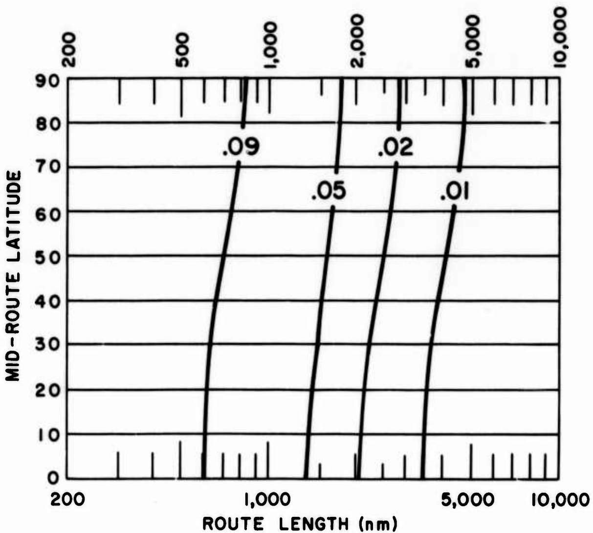
Graph 83. Probability of the Enroute Temperatures Exceeding the Temperatures on the Map, Opposite Page
