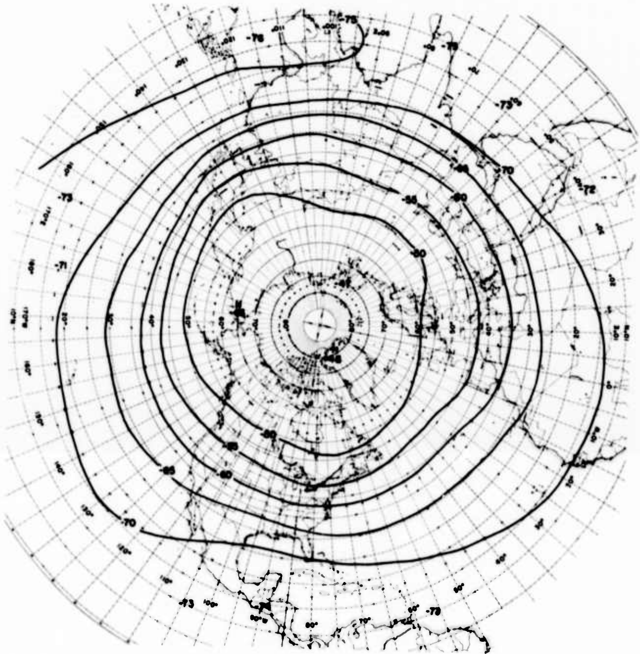
Plate 27. Temperature at 100 mb, in September, October, November, 90 Percentile
