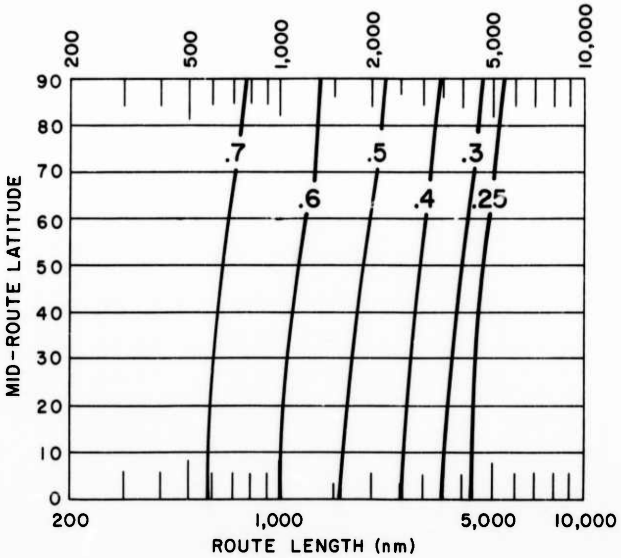
Graph 17. Probability of the Enroute Temperatures Exceeding the Temperatures on the Map, Opposite Page
