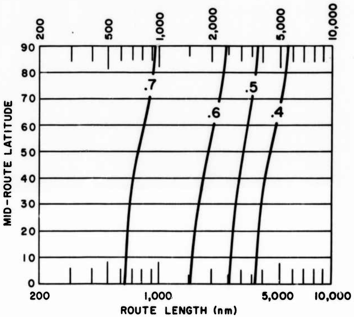
Graph 73. Probability of the Enroute Temperatures Exceeding the Temperatures on the Map, Opposite Page
