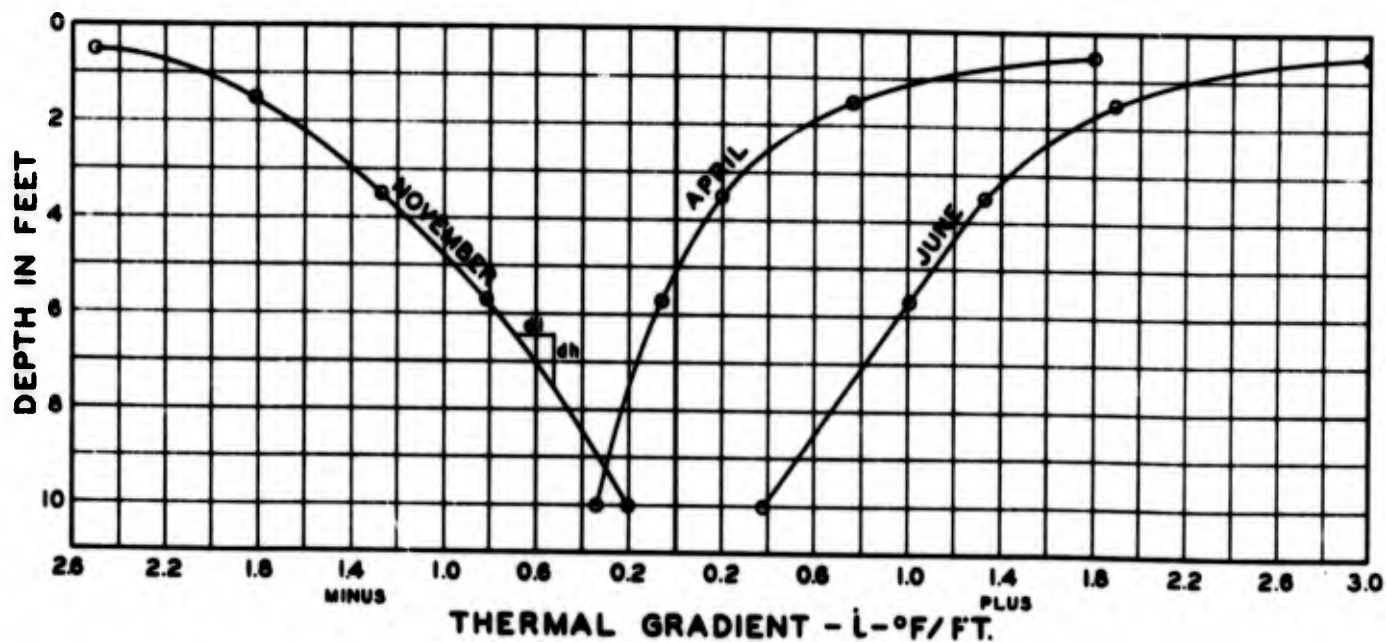
THERMAL GRADIENTS FOR MONTHS OF APRIL, JUNE AND NOVEMBER
