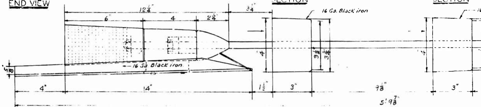
TAIL ASSEMBLY ALTERNATE
