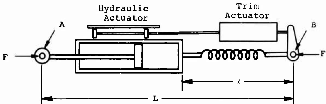
Figure 2. Schematic of Constant Force Actuator.
