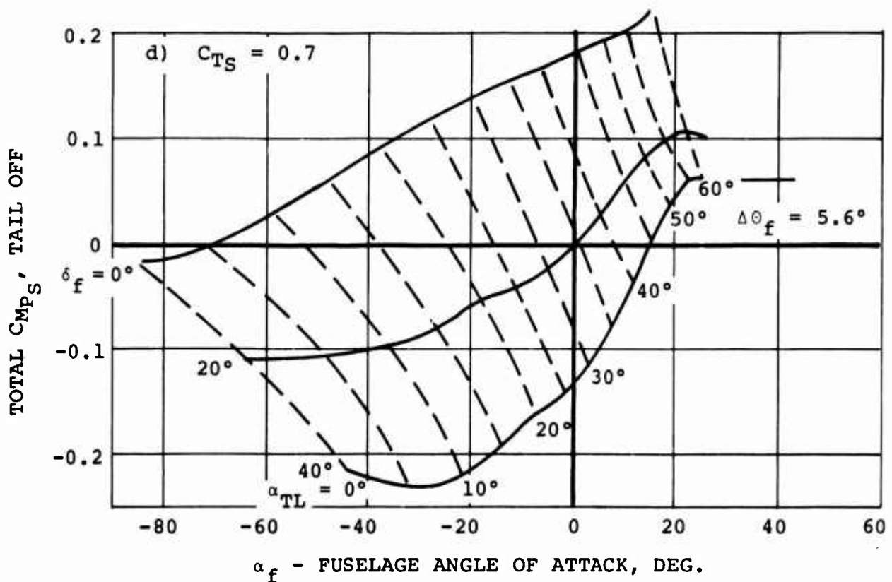
Figure 9. Variation of Total Moment with Fuselage Angle of Attack. (2 of 3)
