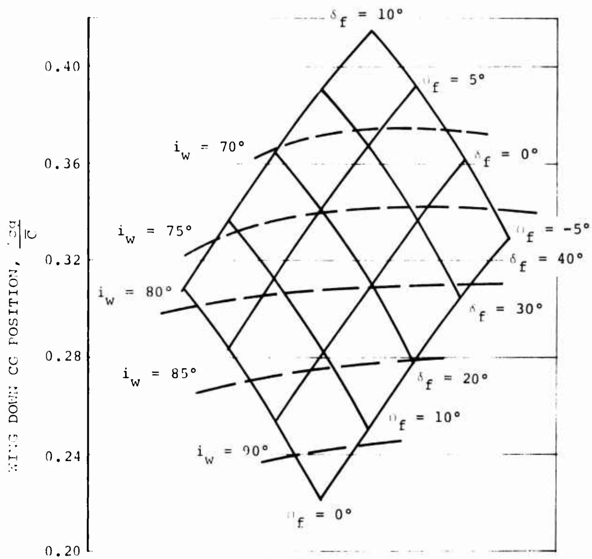
Figure 17. Flap Trim with Geared Flap.
