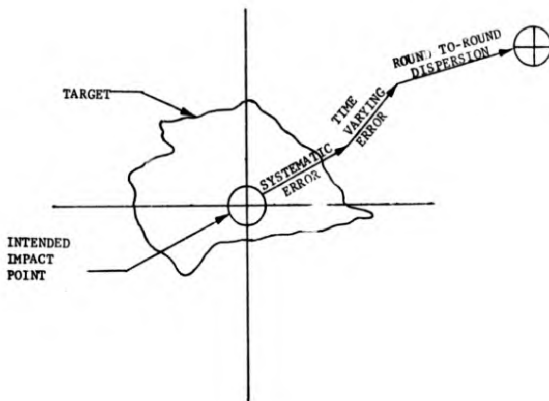
Impact Point Error Geometry [Ref. 10]
