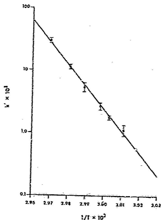
Fig. 2. Plot of the logarithm of the inactivation constant of intracellular \beta -galactosidase as a function of the reciprocal of the absolute temperature.
