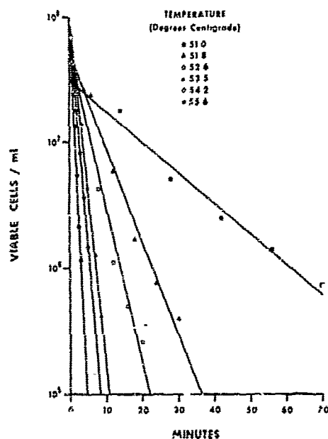
Fig. 3. Thermal inactivation of E. coli K12/37 at temperatures ranging from 51.0°C to 55.6°C. The logarithm of the number of viable cells is plotted as a function of time of exposure for each temperature.
