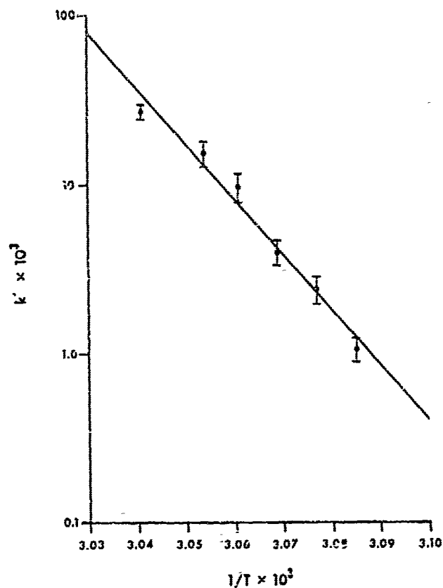
Fig. 4. Plot of the logarithm of the inactivation constant of E. coli K12/37 as a function of the reciprocal of the absolute temperature.
