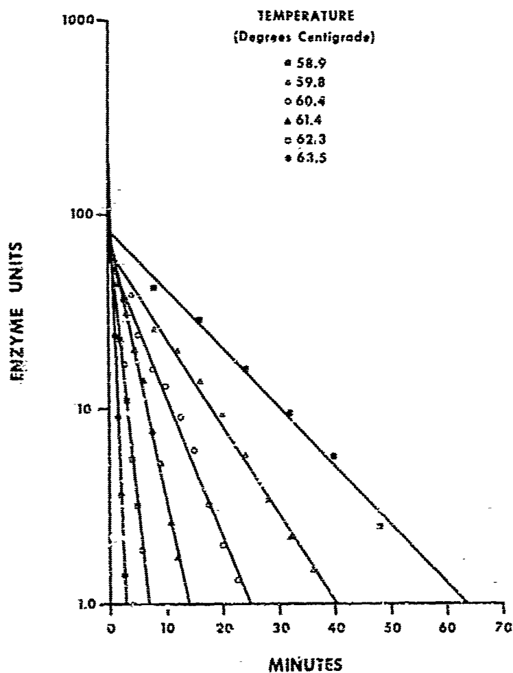
Fig. 1. Thermal inactivation of intracellular \beta -galactosidase at temperatures ranging from 58.9°C to 63.5°C. The logarithm of the enzyme activity is plotted as a function of time of exposure for each temperature.
