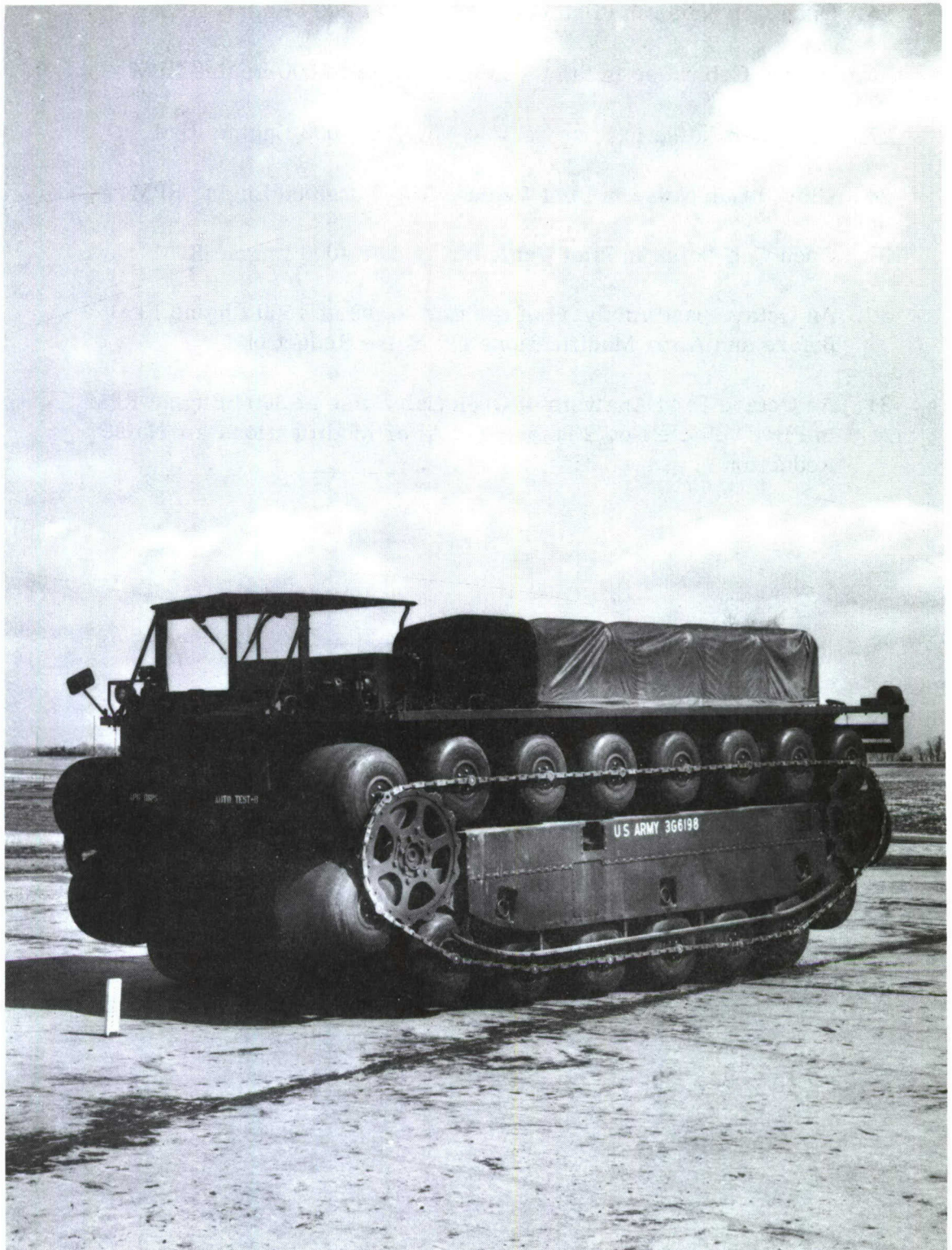
Fig. 1. THE XM759 CARGO CARRIER (MARGINAL TERRAIN VEHICLE) PILOT VEHICLE NO. 3
