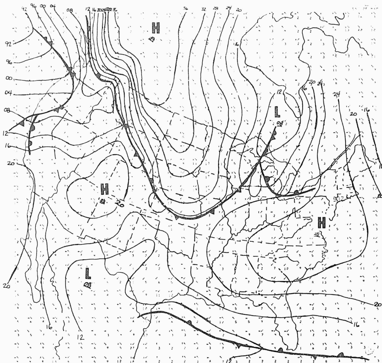
SURFACE ANALYSIS SUPERIMPOSED; WIND SPEEDS IN METERS PER SECOND
