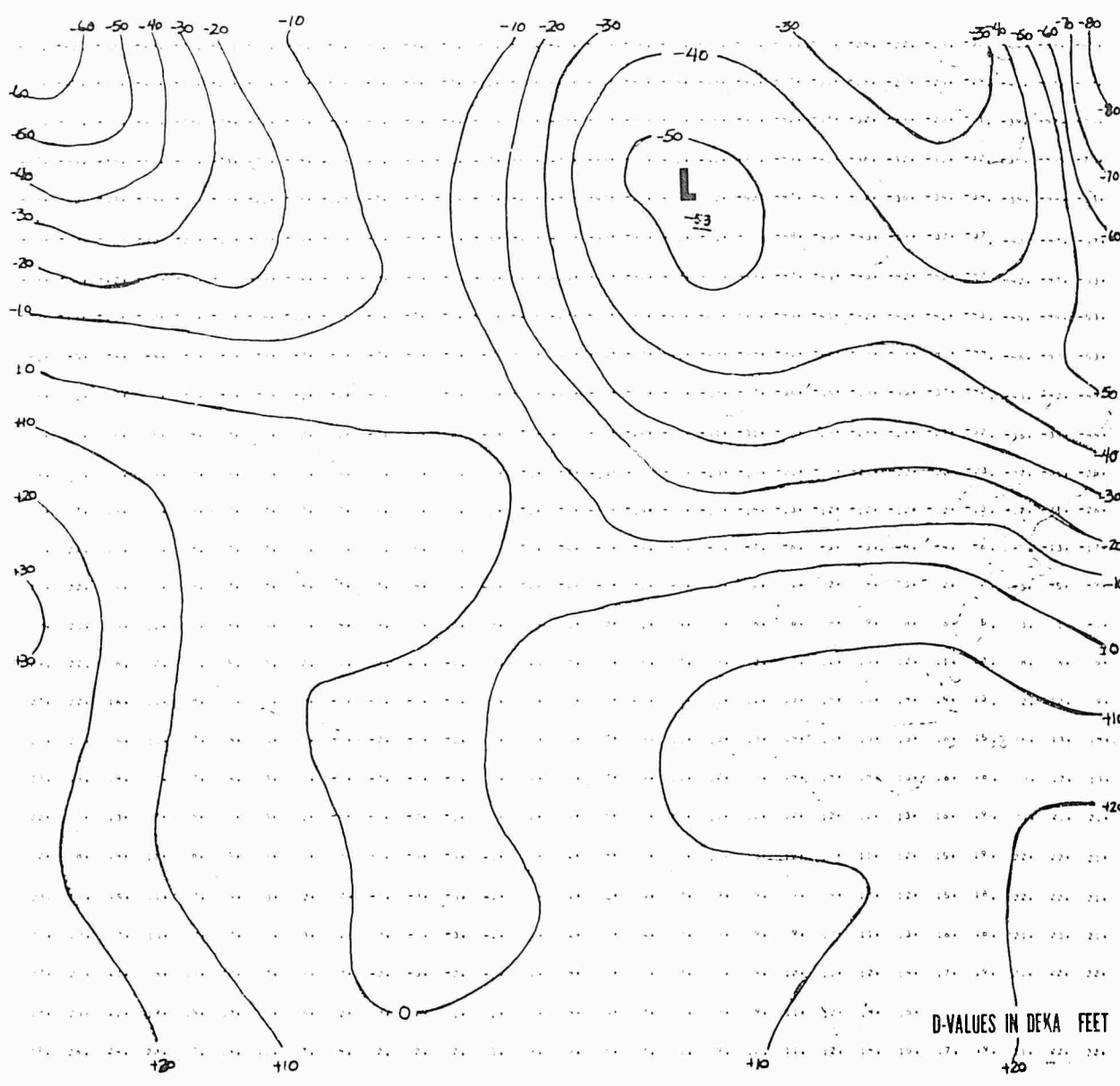
FIG. 23 12 HOUR 1600m O-VALUE FORECAST VALID AT 1200Z 16 JANUARY 1970
