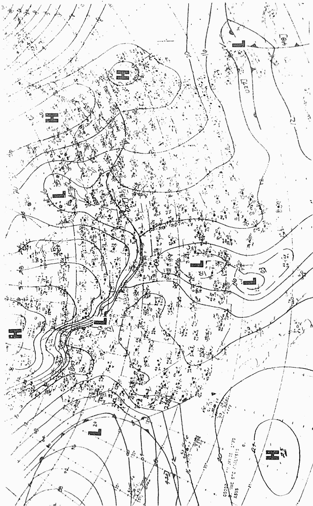
FIG. 4 SURFACE ANALYSIS FOR 0000Z 16 JANUARY 1970
