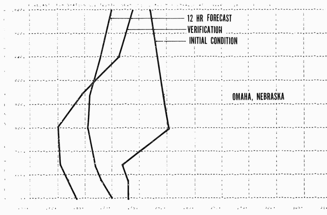
FIG. 25 TEMPERATURE SOUNDINGS FOR ALBANY, NEW YORK AND OMAHA, NEBRASKA
