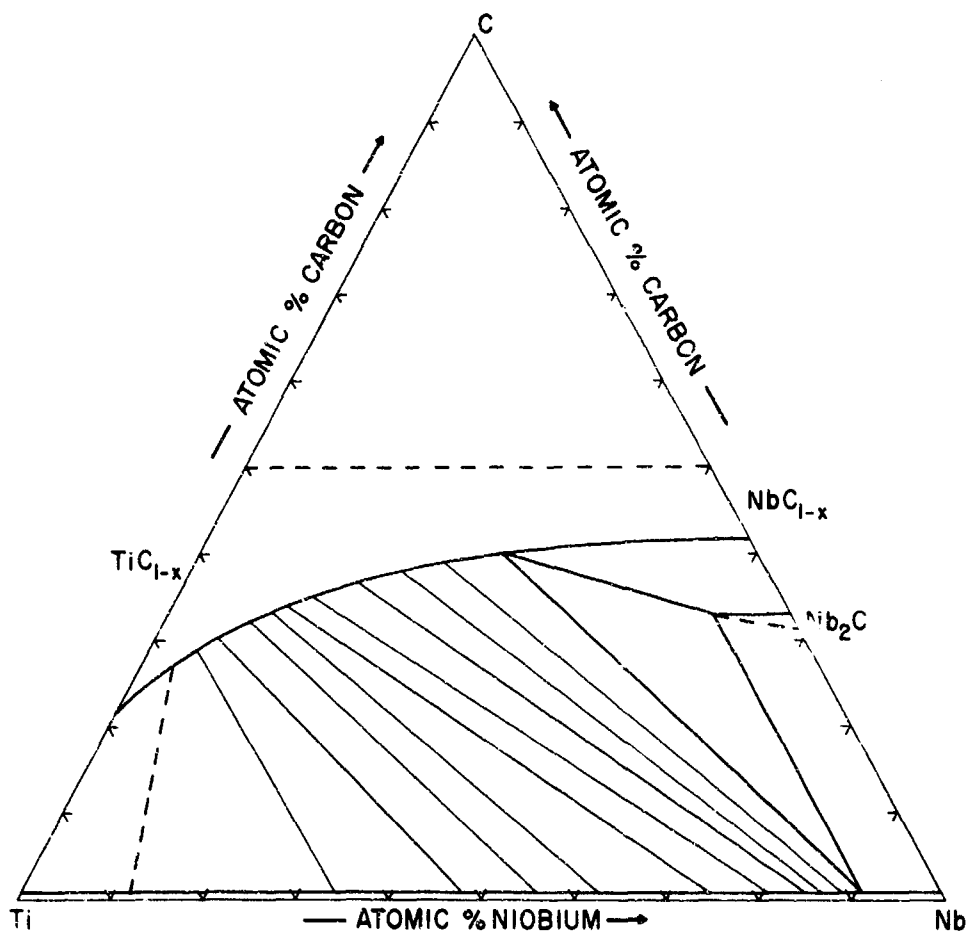
Figure 15. Isothermal Section of the Ti-Nb-C System at 1600°C. (After P. Stecher et al., 1964)
