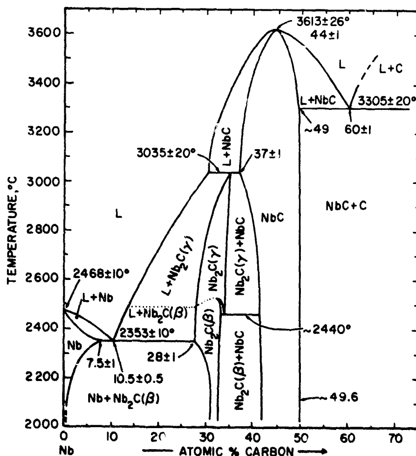
Figure 12. Phase Diagram of the Nb-C System.
