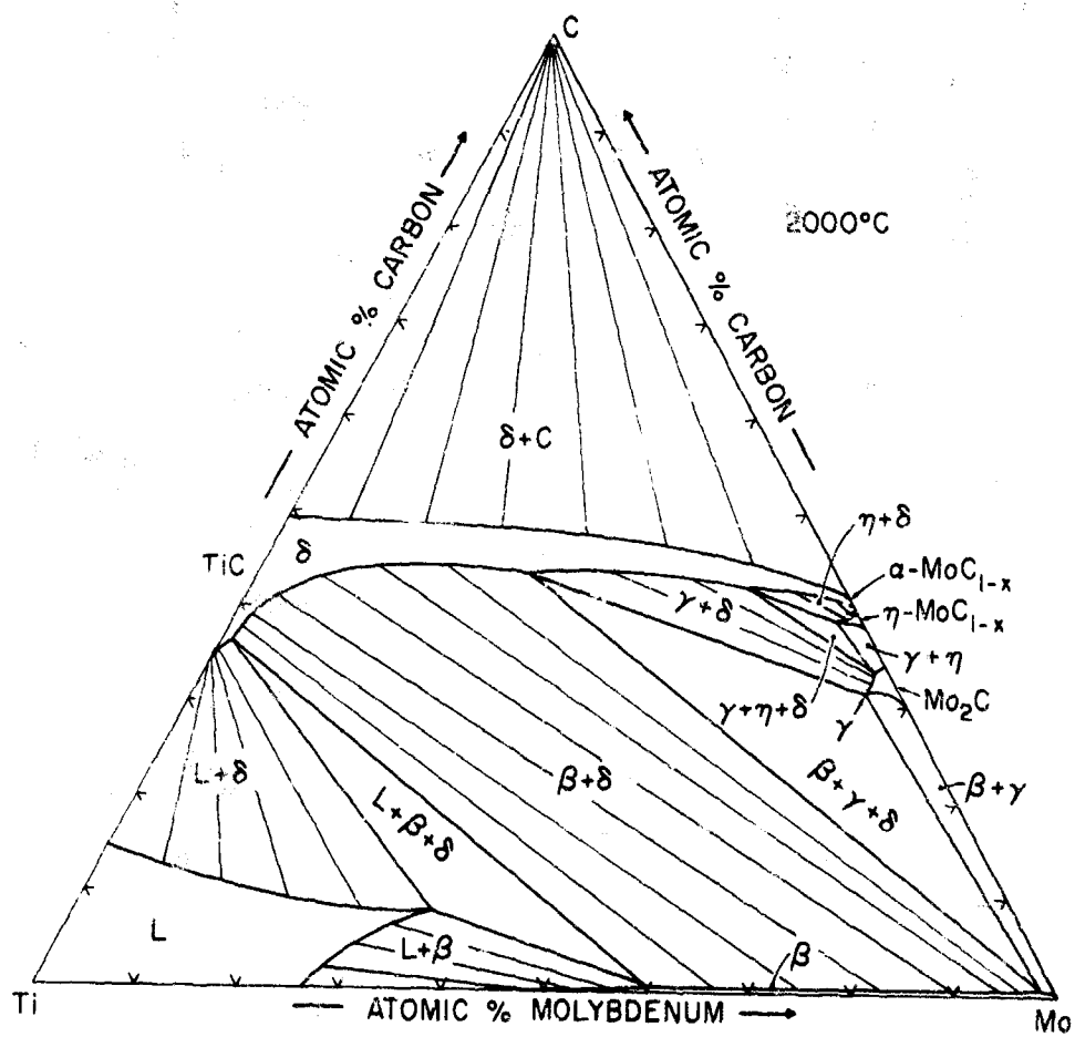
Figure 107. Isothermal Section of the Ti-Mo-C System at 2000° C.
