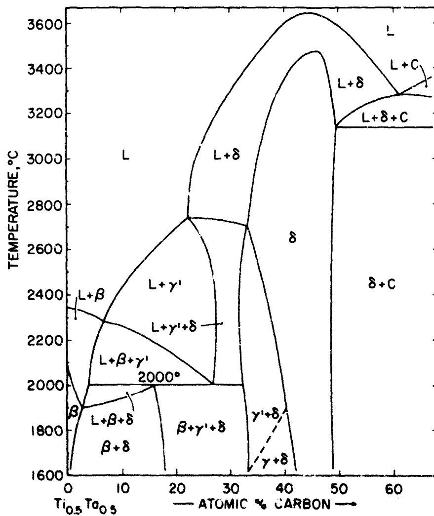
Figure 76. Isopleth \text{Ti}_{0.5}\text{Ta}_{0.5}\text{-C} .
