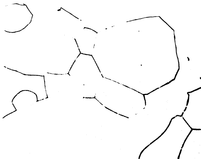
Figure 40. Ti-Nb-C (5-47-48 At.%), Melted, Reequilibrated X190 for 1 Minute at 3300°C, and Cooled.
