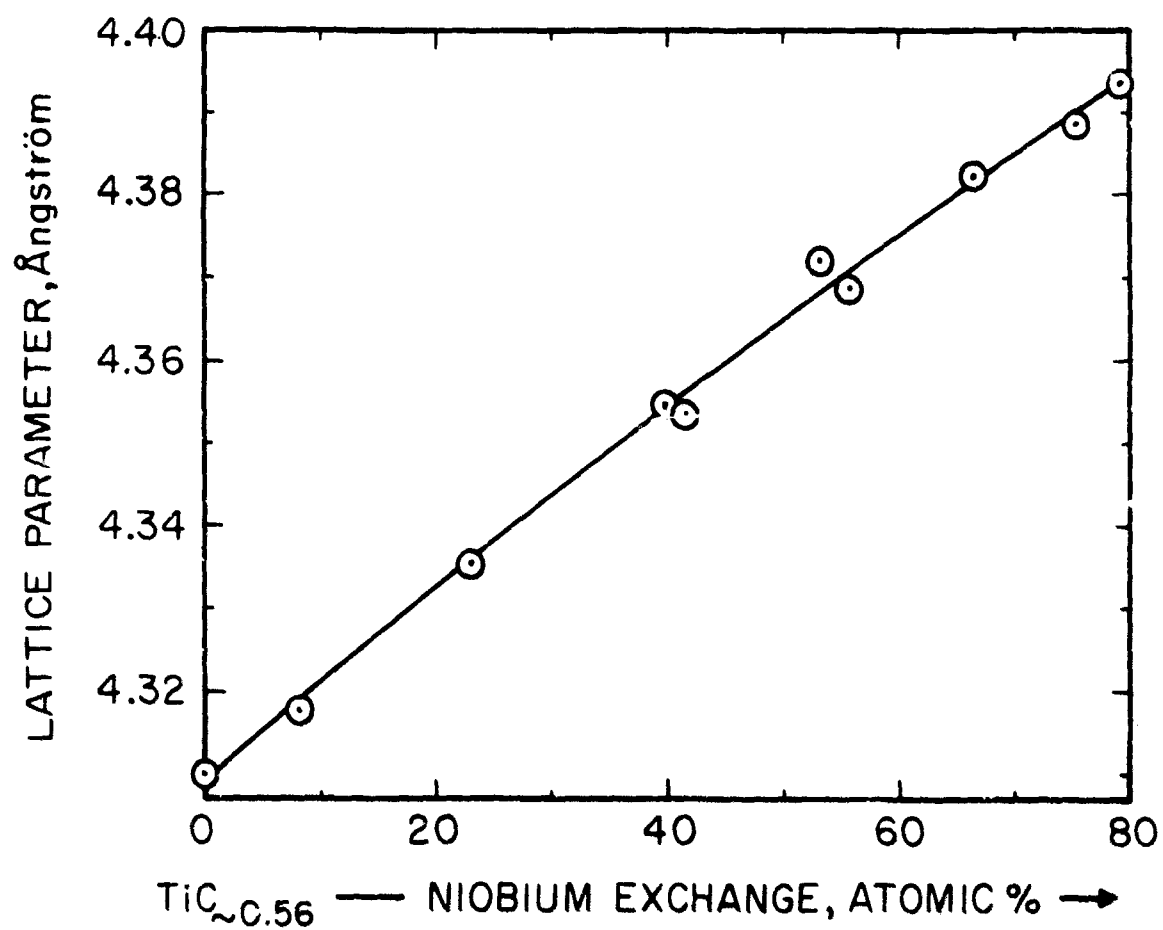
Figure 29. Lattice Parameters of the Monocarbide Phase Containing Between 35 and 38 At. % Carbon.
