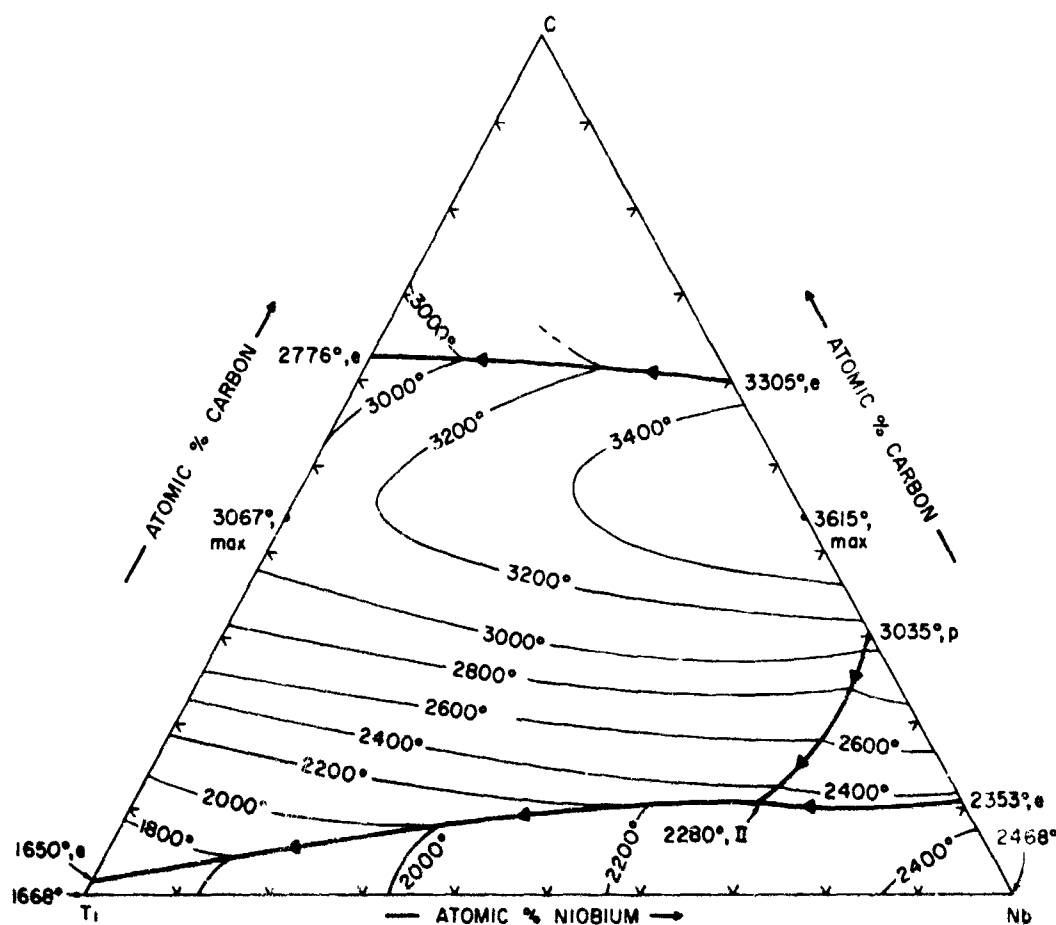
Figure 3. Liquidus Projections in the Ti-Nb-C System.
