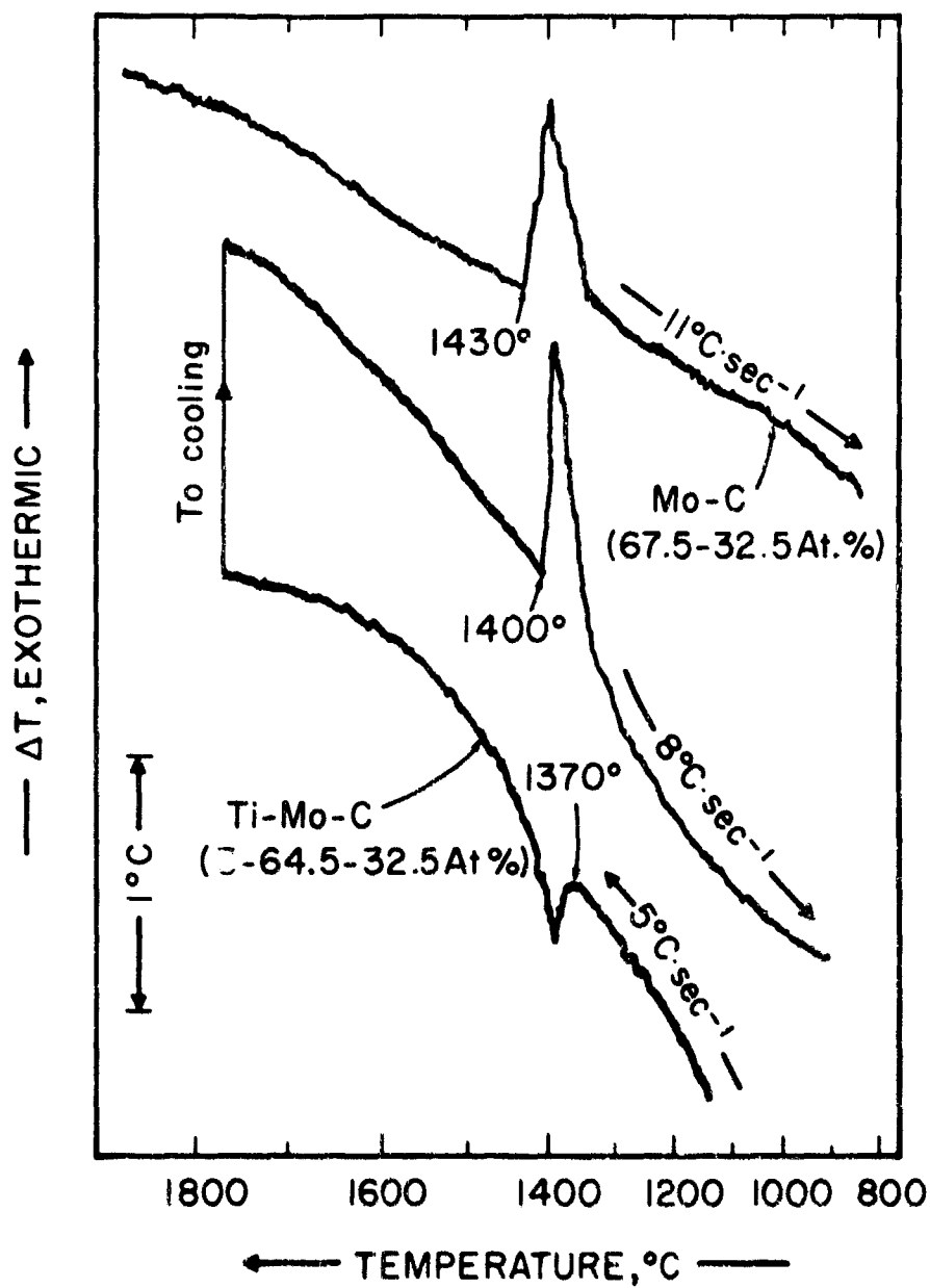
Figure 81. DTA-Thermograms Showing the Order-Disorder Transition in Binary \text{Mo}_2\text{C} and a Ternary Subcarbide Alloy Containing 3 At. % Titanium.
