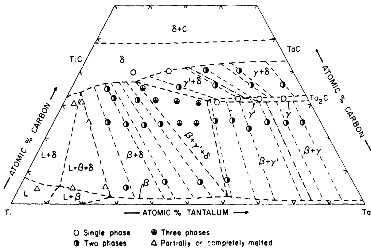
Figure 53. Sample Location and Qualitative Phase Evaluation of the Alloy Series Equilibrated at 1800°C.
