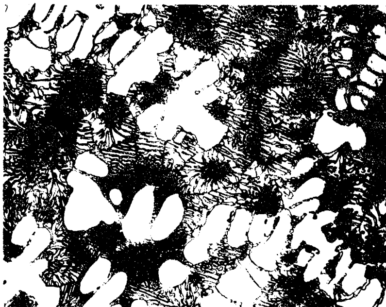
Figure 92. Ti-Mo-C (20-68-12 At.%), Melted and Rapidly Cooled.
