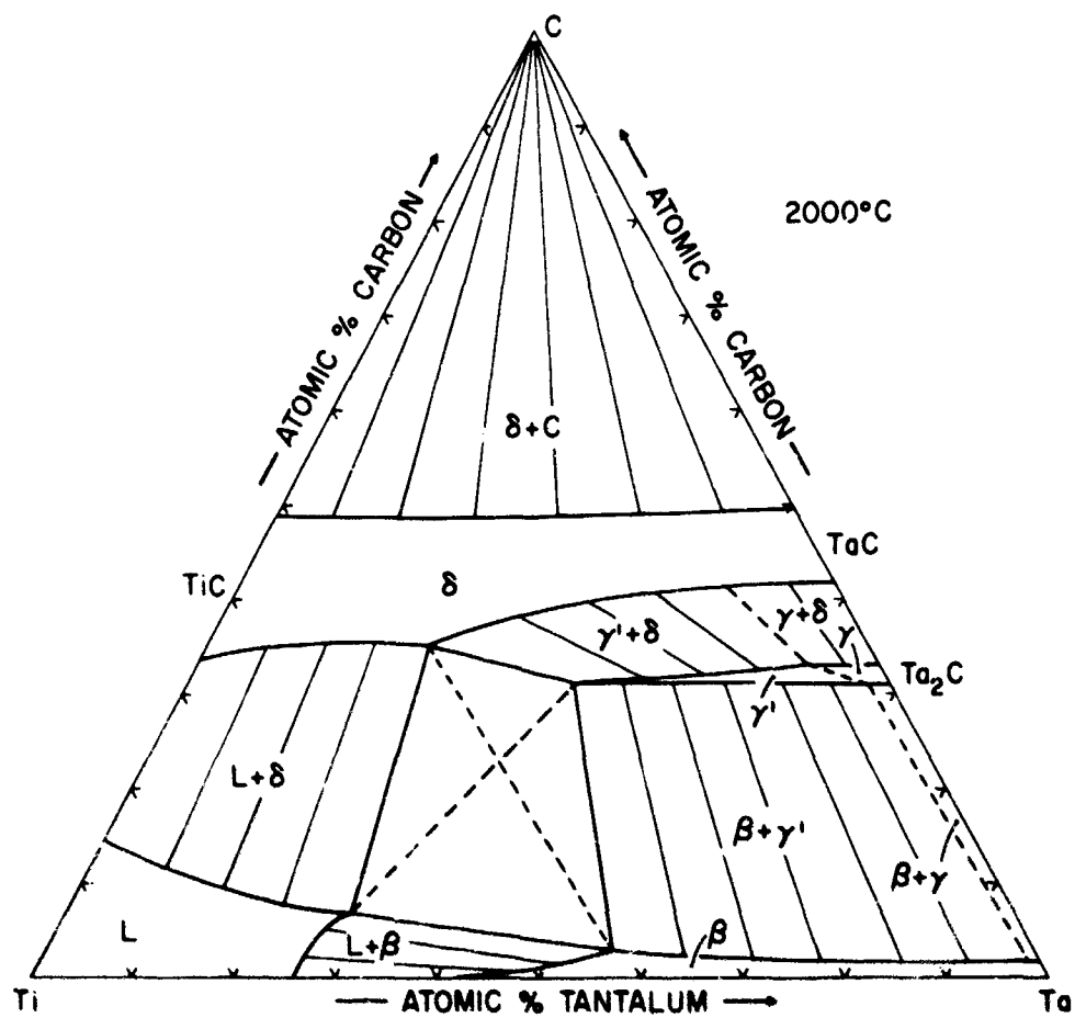
Figure 71. Isothermal Section of the Ti-Ta-C System at 2000° C.
