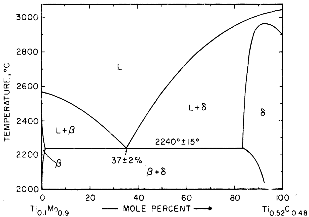
Figure 111. Isopleth at the Pseudobinary Section \text{Ti}_{0.1}\text{Mo}_{0.9}\text{Ti}_{0.52}\text{C}_{0.48} .
