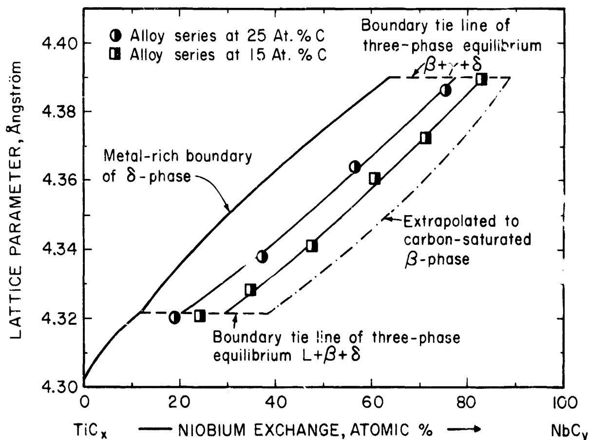
Figure 28. Determination of the Tie Line Distribution in the Two-Phase Field \beta + \delta by the Lattice Parameters of the Monocarbide Phase in Two-Phased, Metal + Monocarbide, Alloys.
