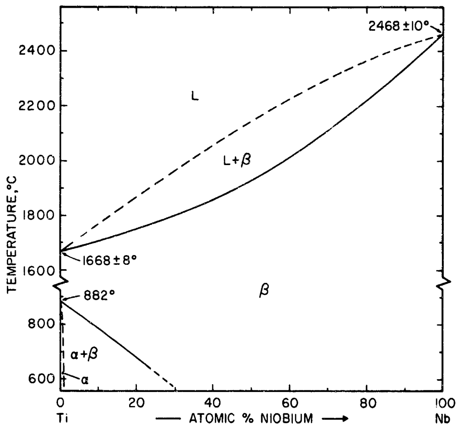
Figure 24. Phase Diagram of the Ti-Nb System
