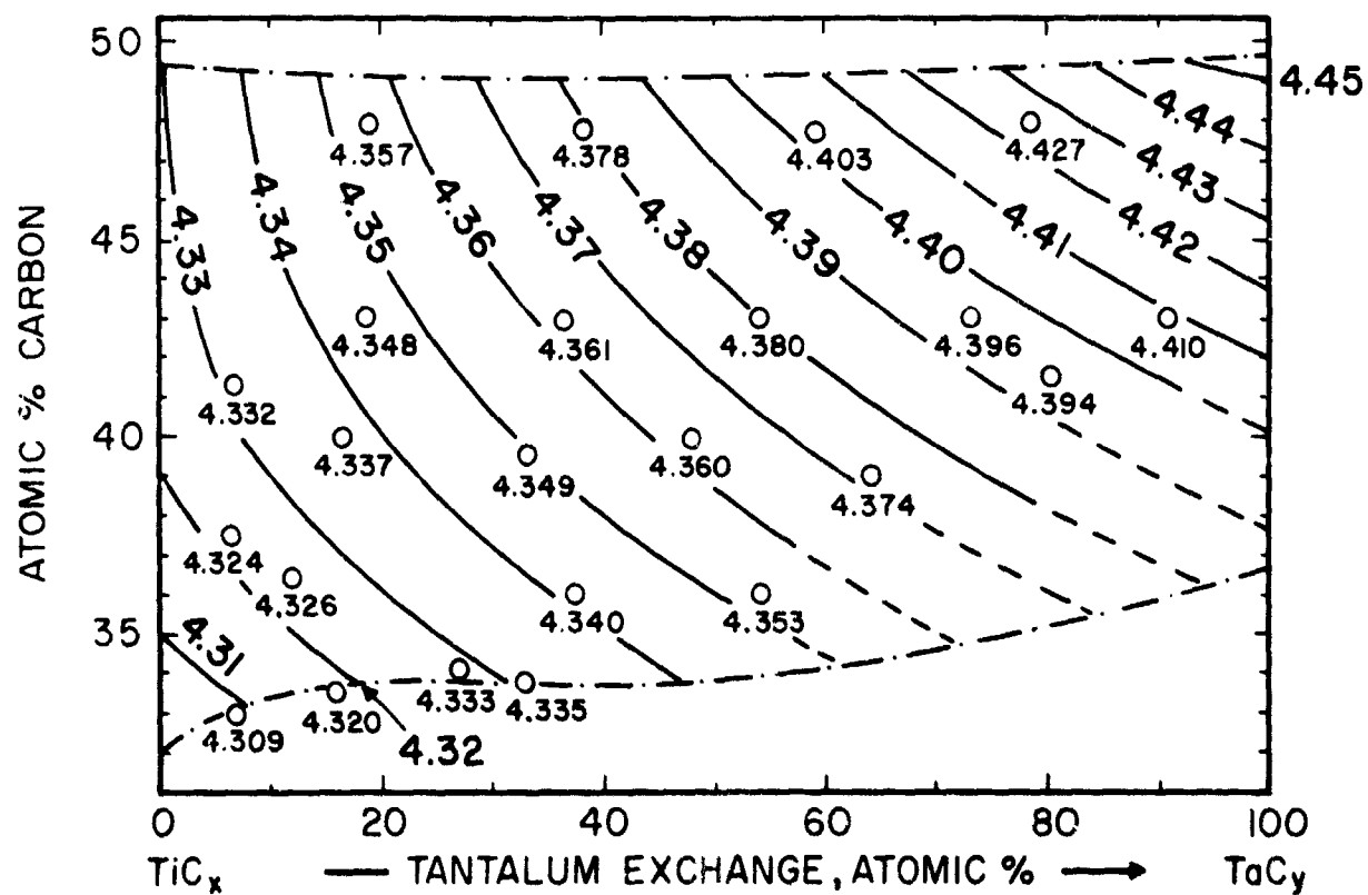
Figure 60. Measured Lattice Parameters and Isoparametric Lines for the (Ti, Ta)C_{1-x} Solid Solution.
