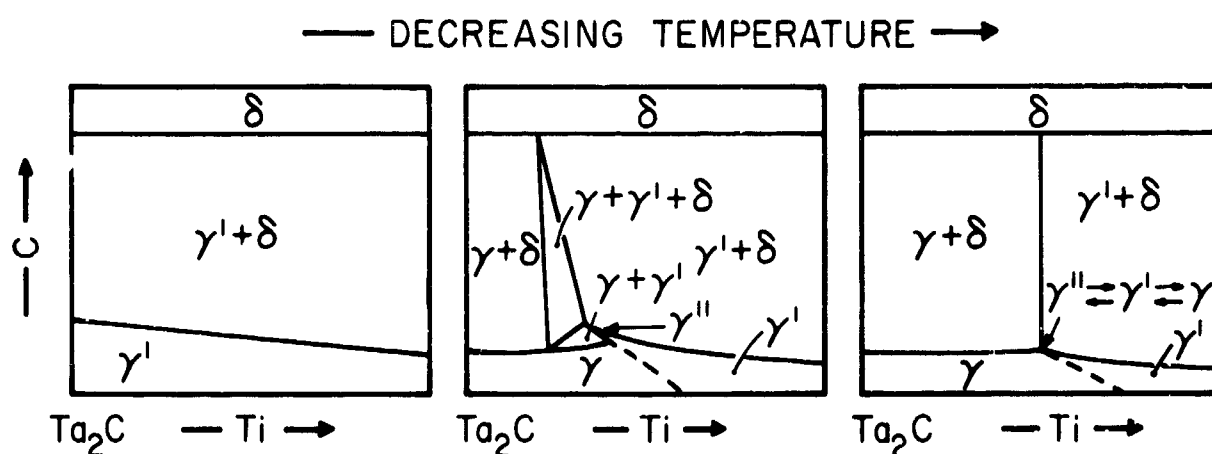
Figure 59. Ti-Ta-C: Diagrammatic Presentation of the Continuation of the Heterogeneous \alpha - \beta -Ta 2 C Phase Transition into the Ternary.
