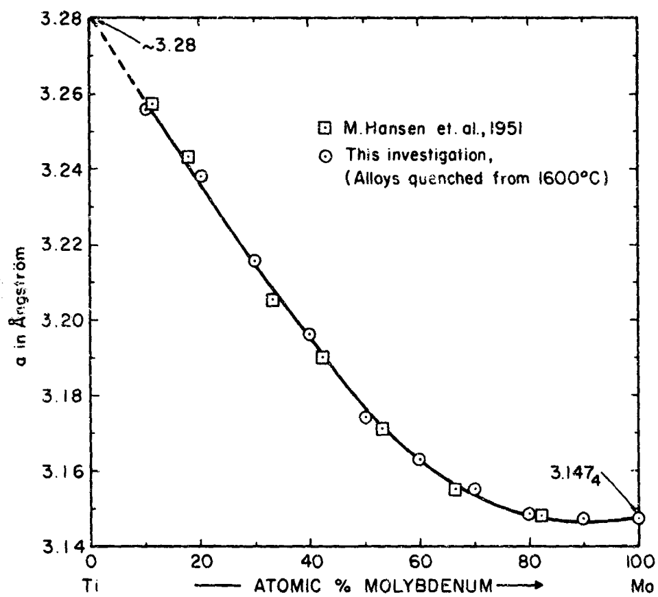
Figure 23. Lattice Parameters of the Cubic (Ti,Mo)-Solid Solution.
