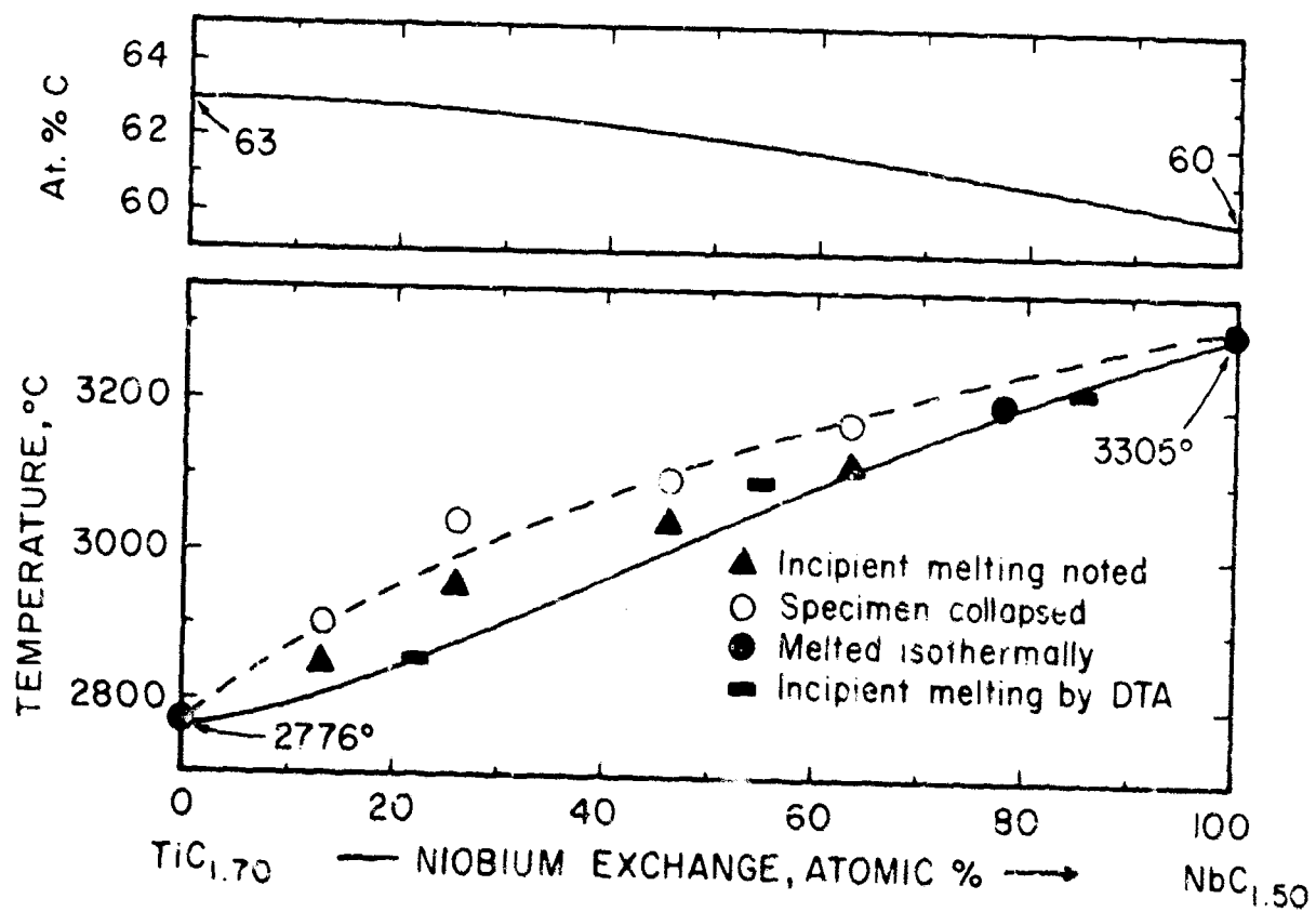
Figure 41. Melting Temperatures of Ti-Nb-C Alloys Located Along the Monocarbide + Graphite Eutectic Trough.
