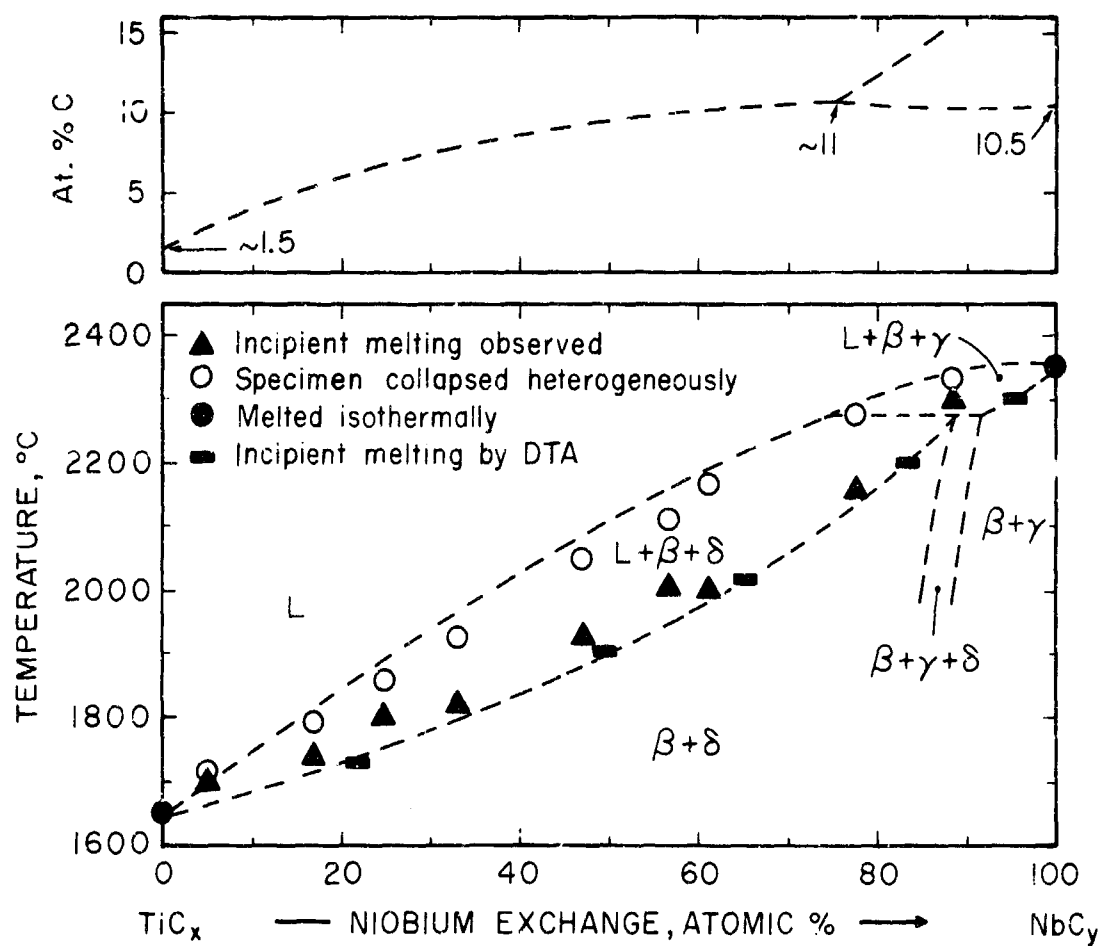
Figure 33. Measured Melting Temperatures of Alloys Located Along the Metal-Rich Eutectic Trough.
