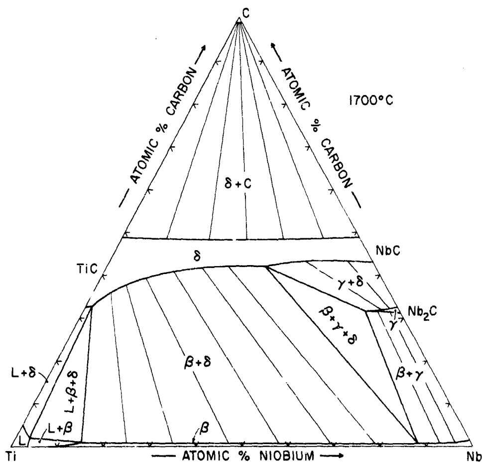
Figure 45. Isothermal Section of the Ti-Nb-C System at 1700°C.
