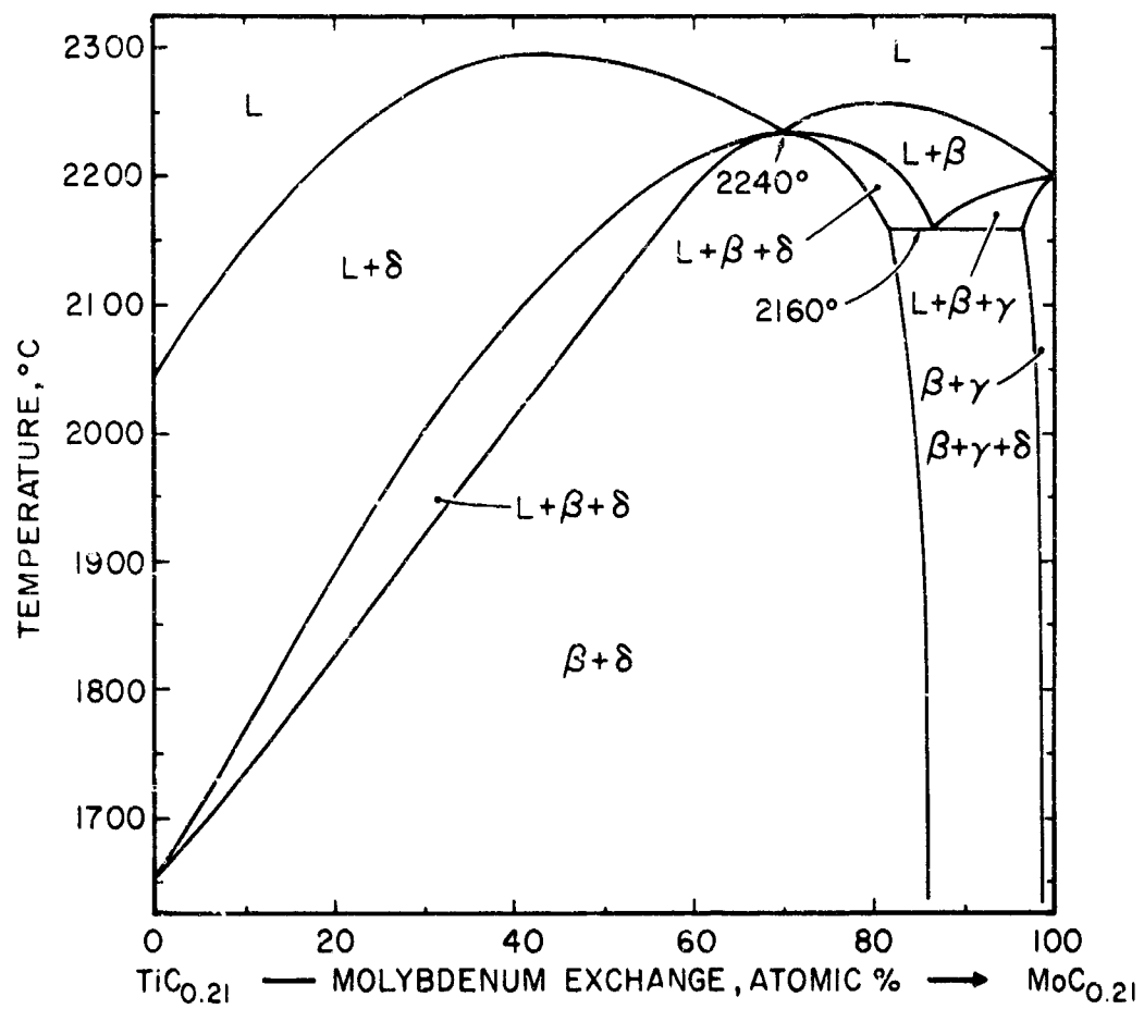
Figure 113. Isopleth \text{TiC}_{0.21} - \text{MoC}_{0.21} .
