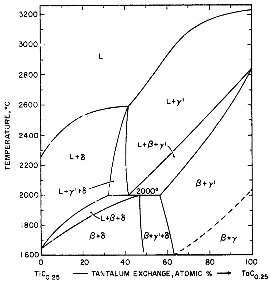
Figure 77. Isopleth \text{TiC}_{0.25} - \text{TaC}_{0.25}
