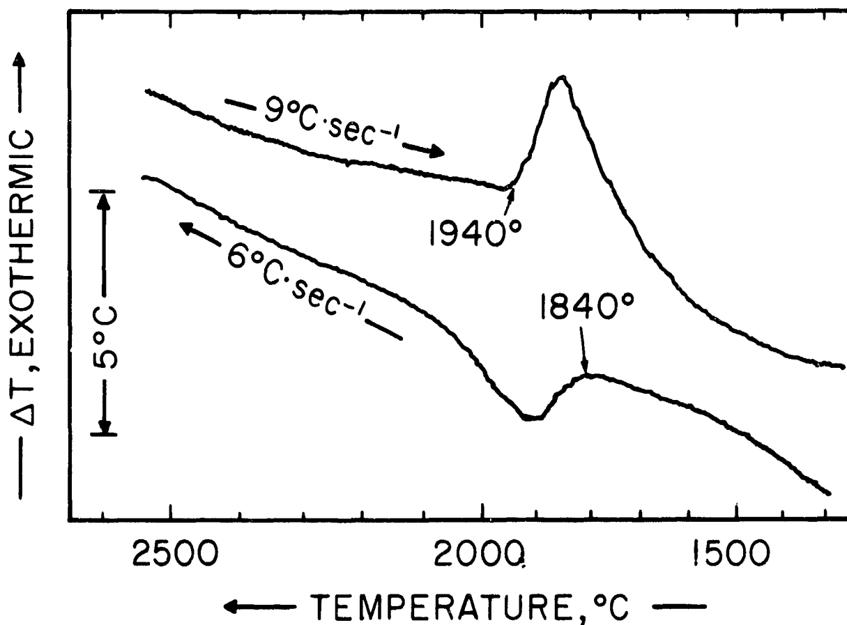
Figure 57. DTA-Thermogram of a Ti-Ta-C (9-63-28 At.%) Alloy, Showing the Order-Disorder Transition in the Substoichiometric (\text{Ti, Ta})_2\text{C} Phase.
