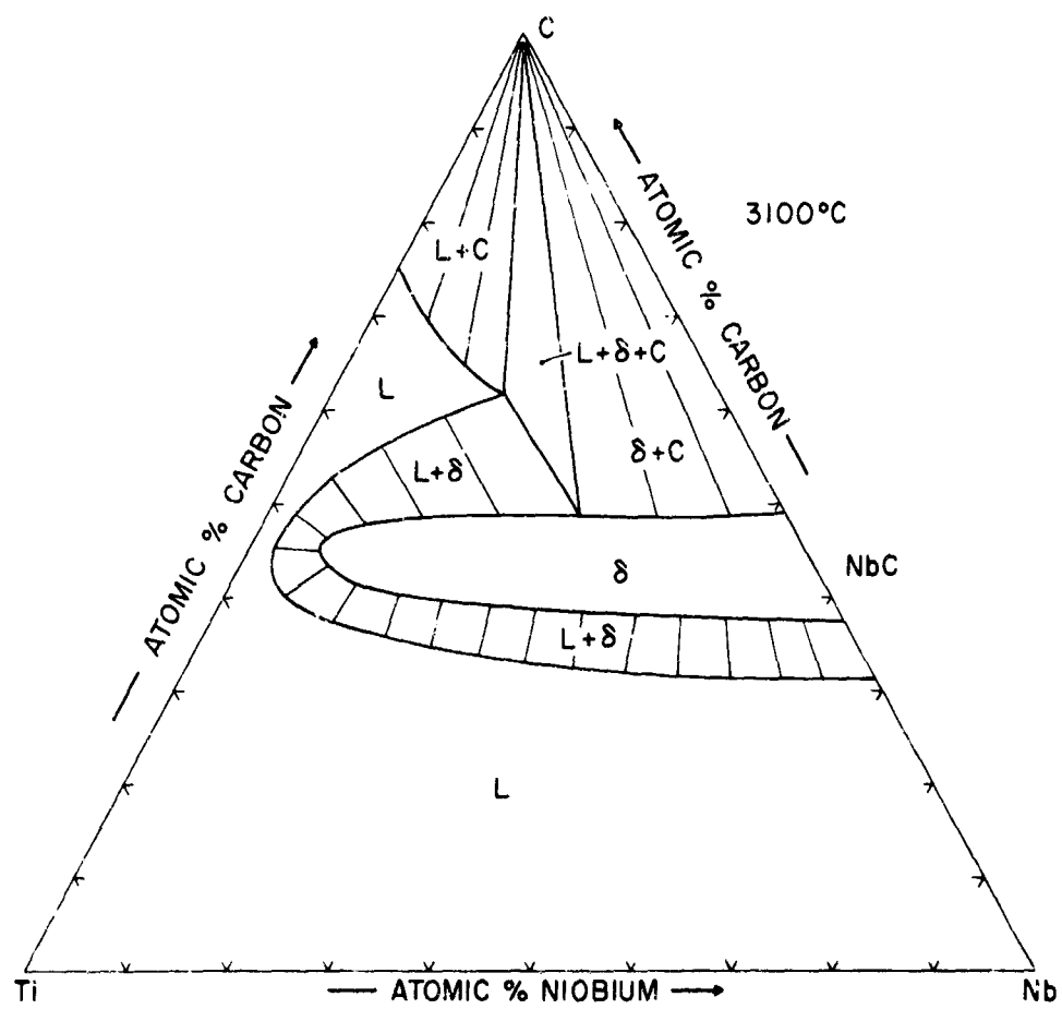
Figure 49. Isothermal Section of the Ti-Nb-C System at 3100°C.
