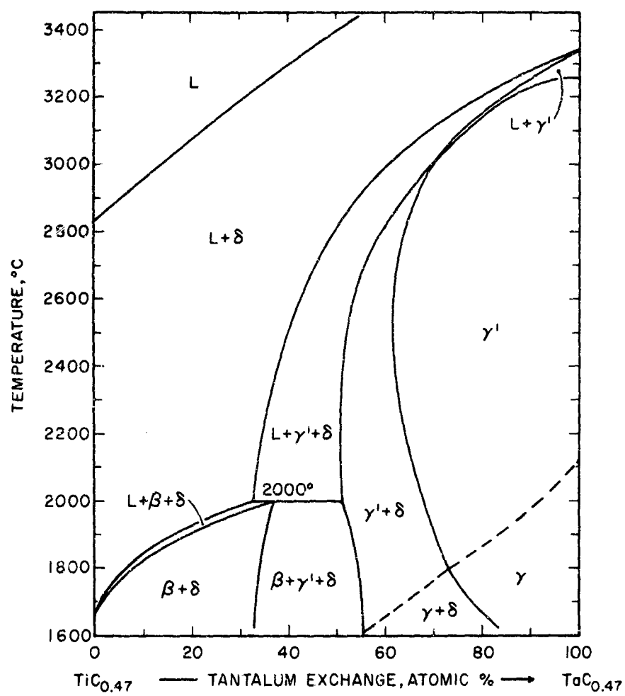
Figure 78. Isopleth \text{TiC}_{0.47} - \text{TaC}_{0.47} .
