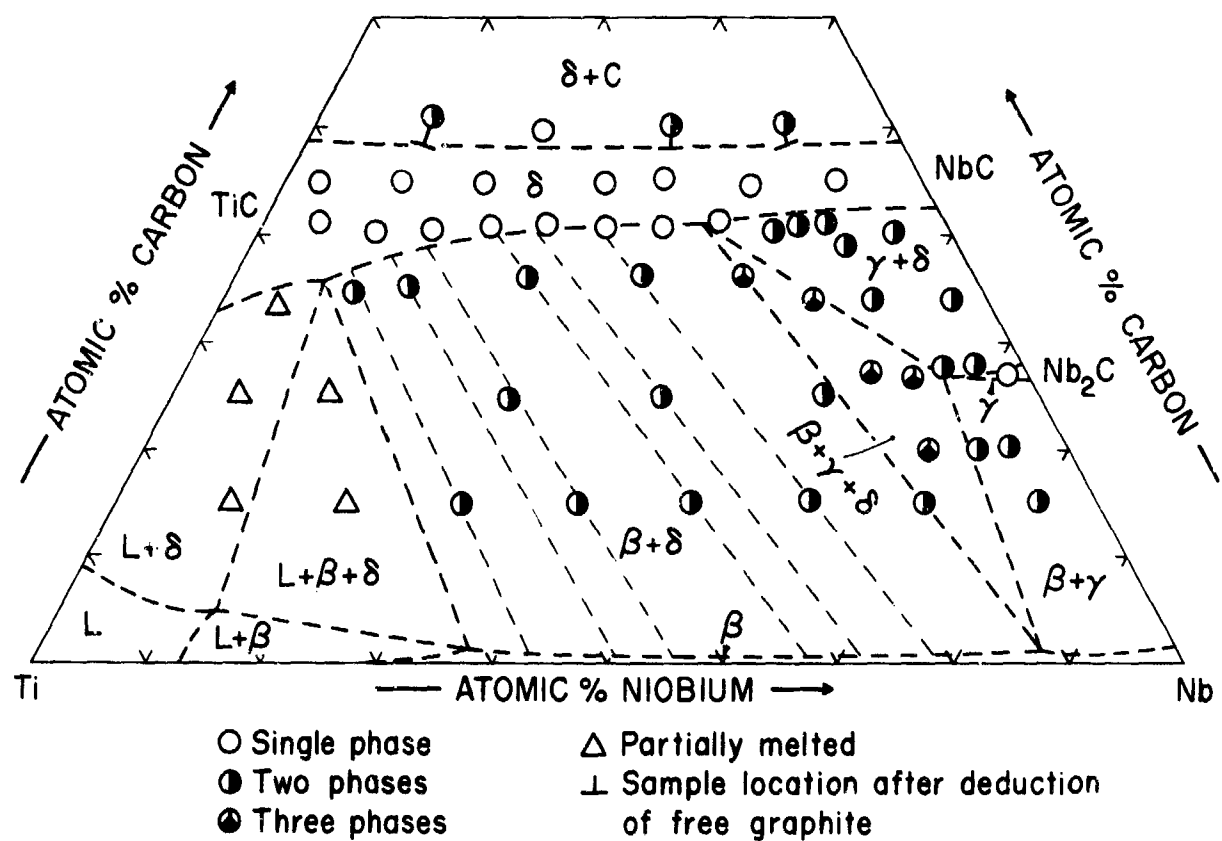
Figure 27. Qualitative Phase Evaluation of Ti-Nb-C Alloys Equilibrated at 1800°C.
