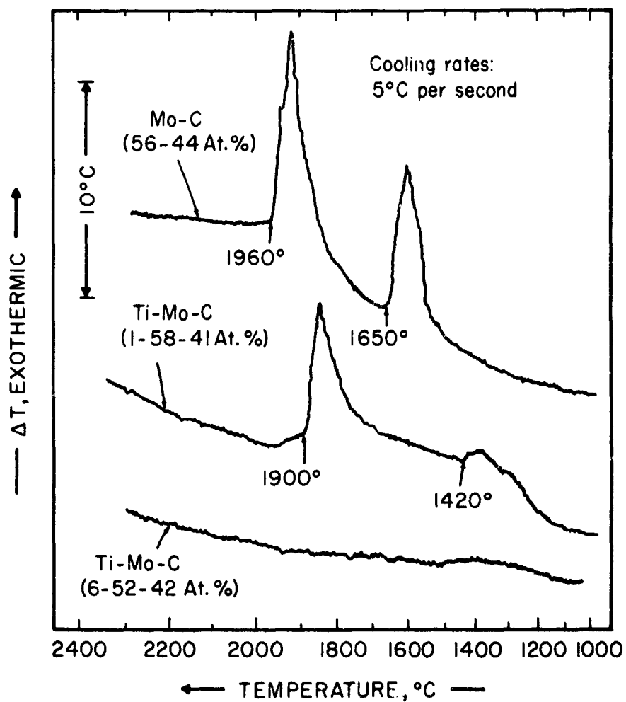
Figure 84. Decomposition of the \beta - \text{MoC}_{1-x} and \eta - \text{MoC}_{1-x} Phases Upon Cooling in Binary Mo-C and Ternary Ti-Mo-C Alloys.
