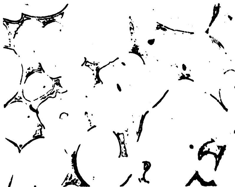
Figure 97. Ti-Mo-C (53-13-34 At.%), Equilibrated at 2200^\circ\text{C} and Quenched.
