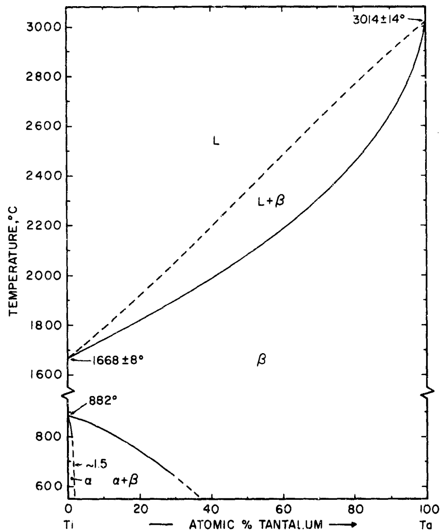
Figure 25. Phase Diagram of the Ti-Ta-System.
