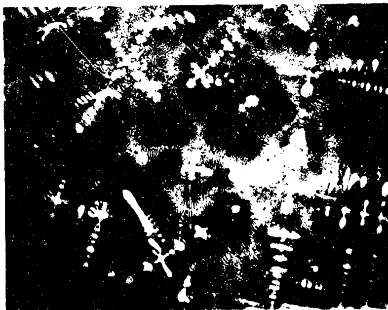
Figure 93. Ti-Mo-C (28-54-18 At.%) Small Amounts of Binary Monocarbide in a Pseudobinary \text{Me} + \text{MeC}_{1-x} Eutectic Matrix.
