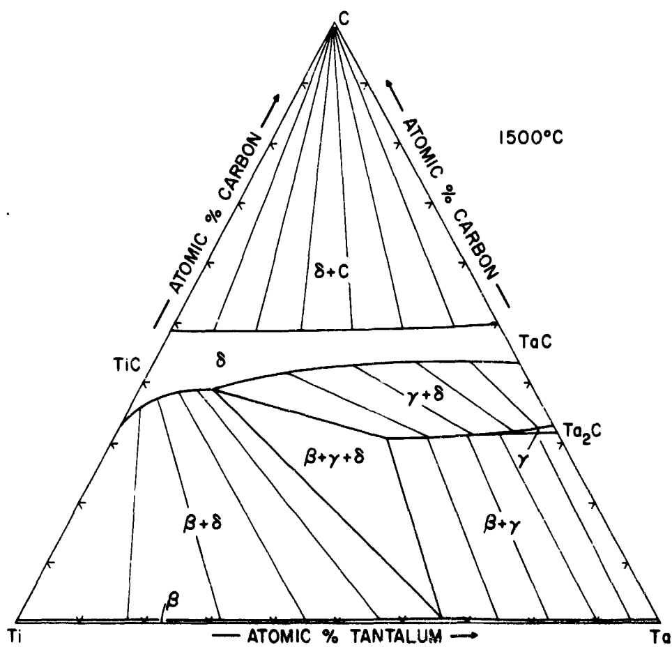
Figure 69. Isothermal Section of the Ti-Ta-C System at 1500°C.
