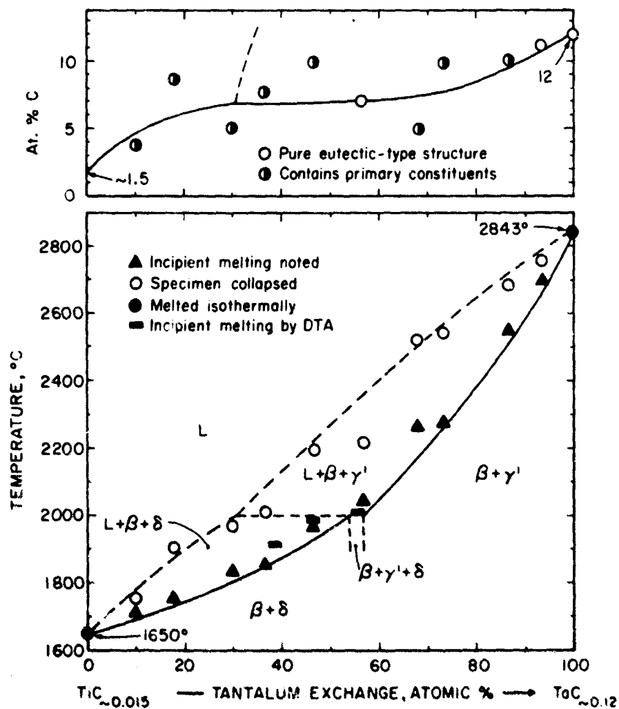
Figure 62. Ti-Ta-C: Melting Temperatures at the Metal-Rich Eutectic Trough and Metallographic Location of the Boundary Line.
