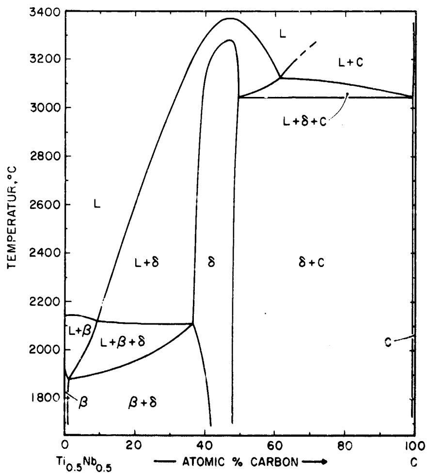
Figure 50. Isopleth \text{Ti}_{0.5}\text{Nb}_{0.5}\text{-C} .
