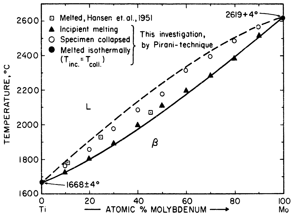
Figure 22. Melting Temperatures of Ti-Mo Alloys. (Temperature Error Figures Based on Reproducibility)
