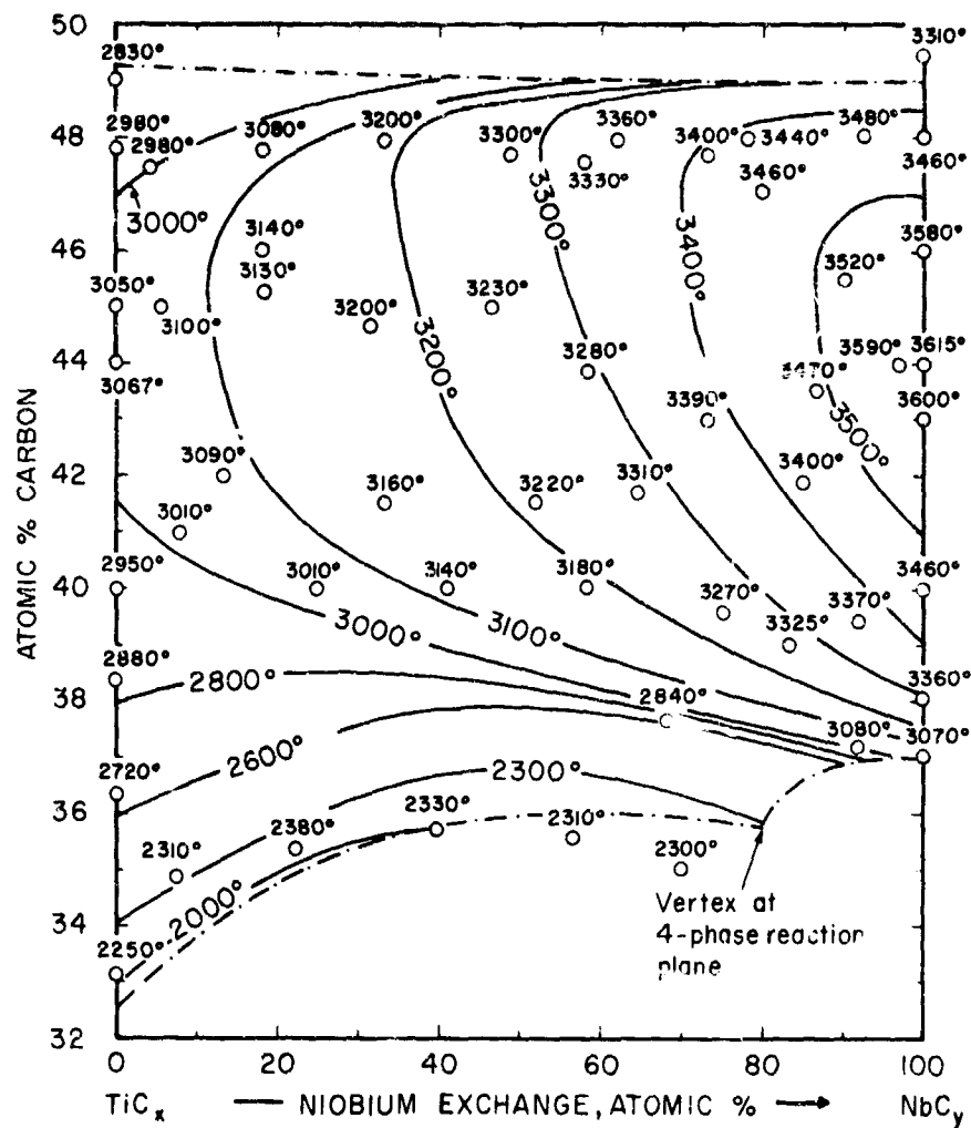
Figure 37. Solidus Temperatures of the Monocarbide (\text{Ti,Nb})\text{C}_{1-x} , Solid Solution.
