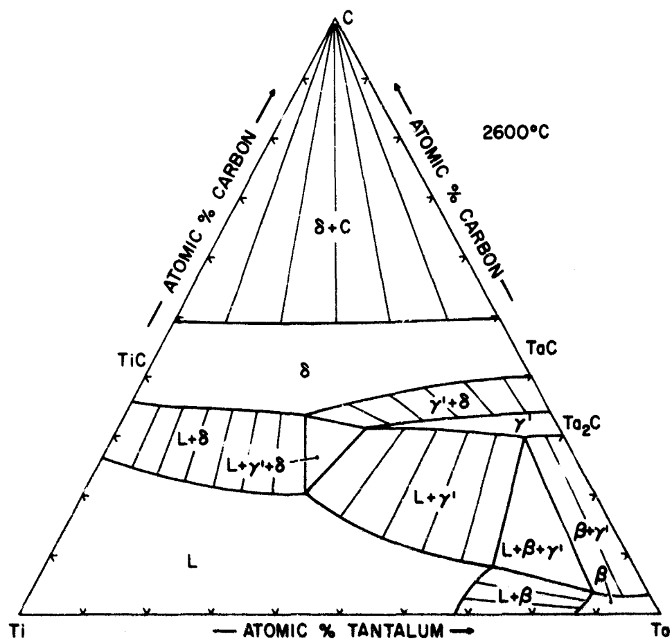
Figure 73. Isothermal Section of the Ti-Ta-C System at 2600°C.
