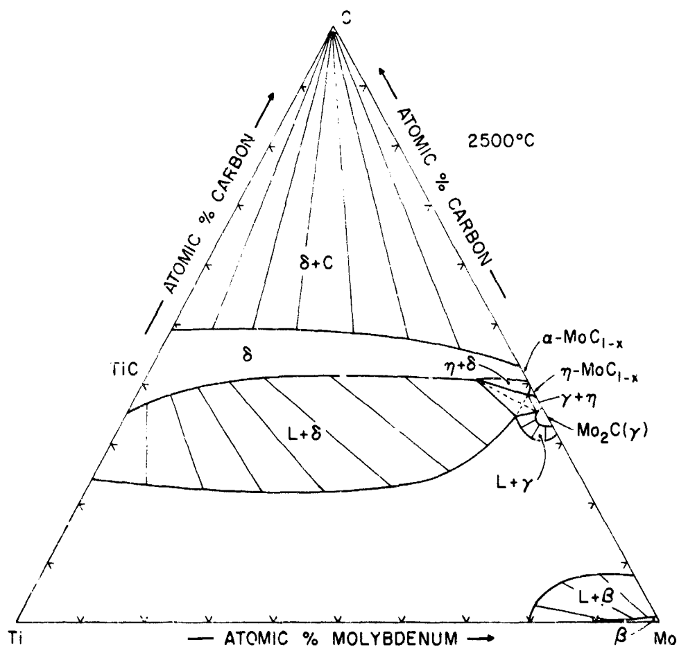
Figure 109. Isothermal Section of the Ti-Mo-C System at 2500°C.
