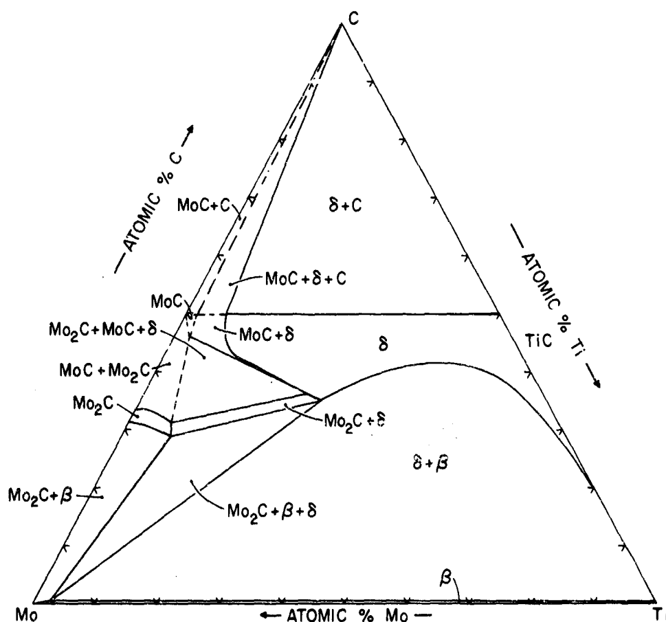
Figure 17. Isothermal Section of the Ti-Mo-C System at 1710°C.
