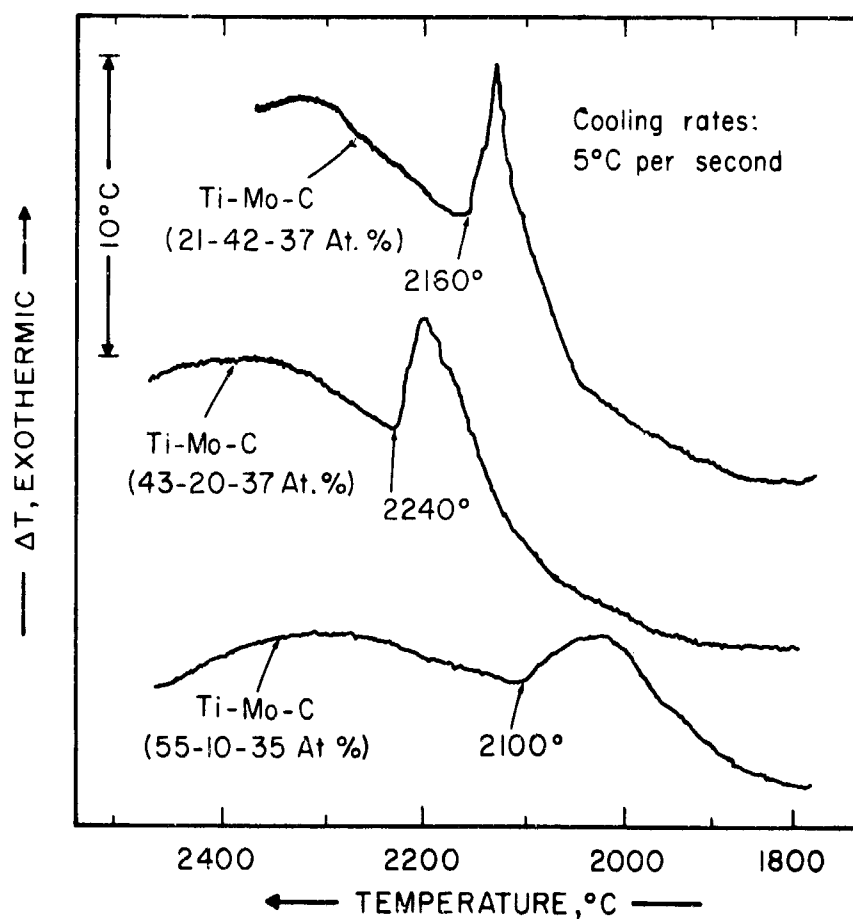
Figure 98. Ti-Mo-C Alloys Showing Solidification of Rest-Eutectic in Alloys Located Near the Monocarbide Phase Boundary.
