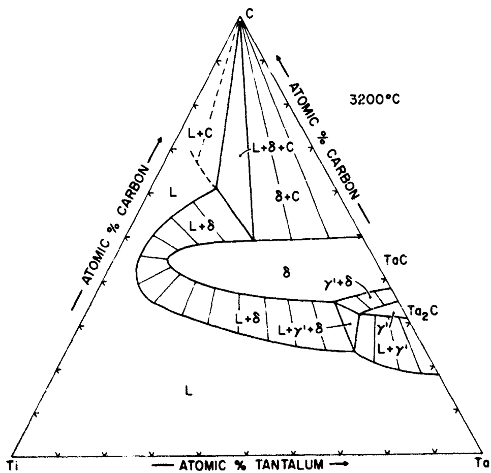
Figure 75. Isothermal Section of the Ti-Ta-C System at 3200° C.
