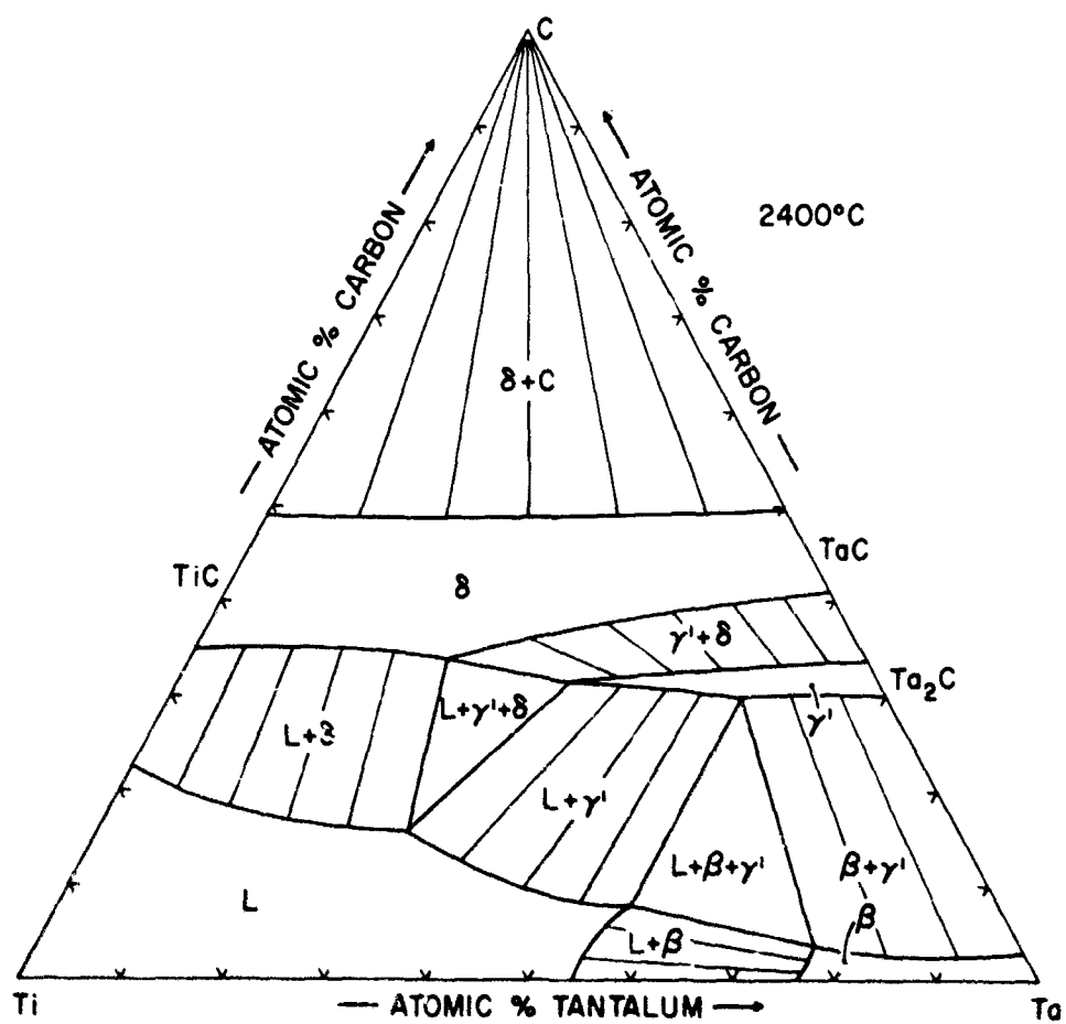
Figure 72. Isothermal Section of the Ti-Ta-C System at 2400°C.
