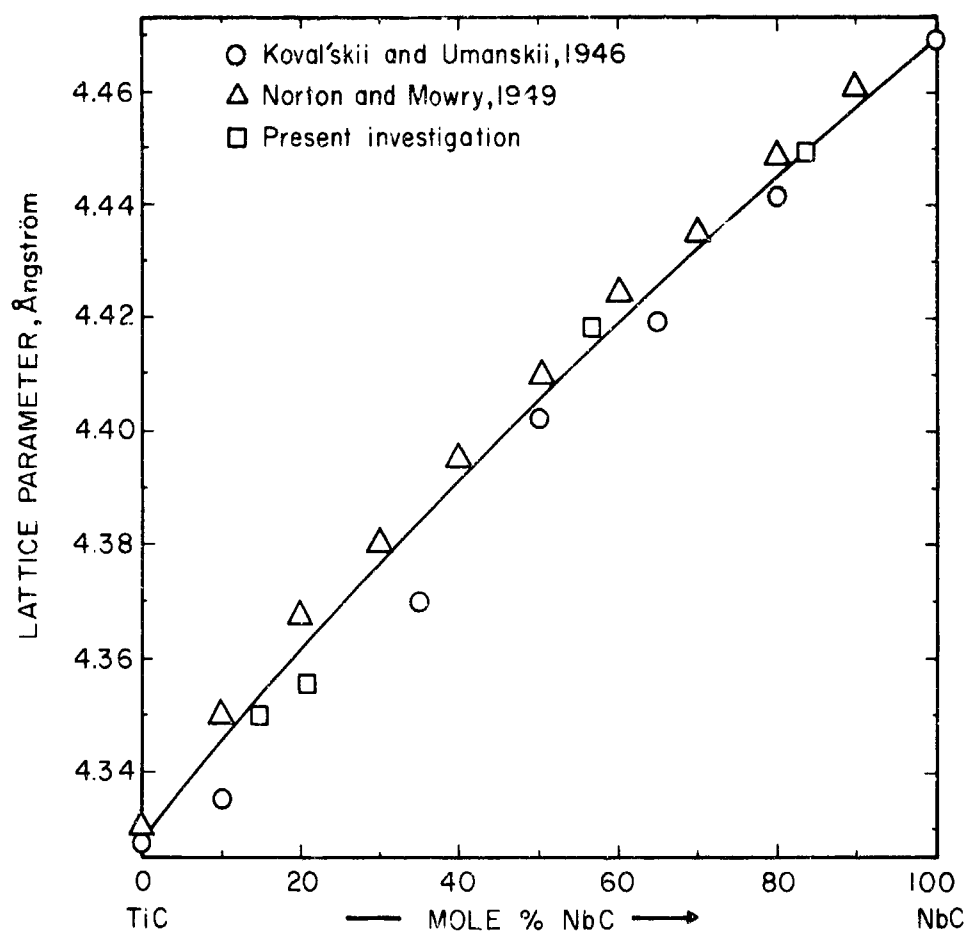
Figure 32. Lattice Parameters for the Carbon-Saturated Monocarbide Phase.
