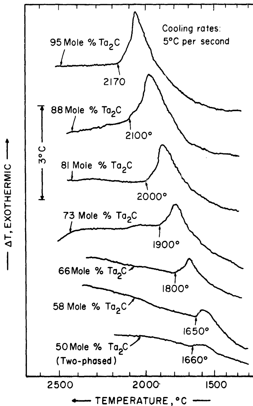
Figure 56. DTA-Thermograms (Cooling), Showing the Order-Disorder Transition in the Primary \text{Ta}_2\text{C} Phase and in the Ternary (\text{Ti}, \text{Ta})_2\text{C} Solid Solution. (32.5-33 At. % C).
