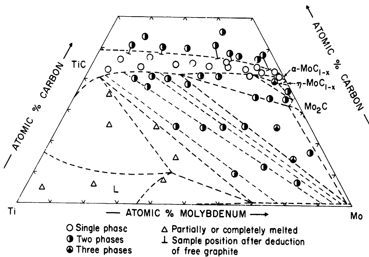
Figure 80. Sample Location and Qualitative Phase Evaluation of the Alloy Series Equilibrated at 2100°C.
