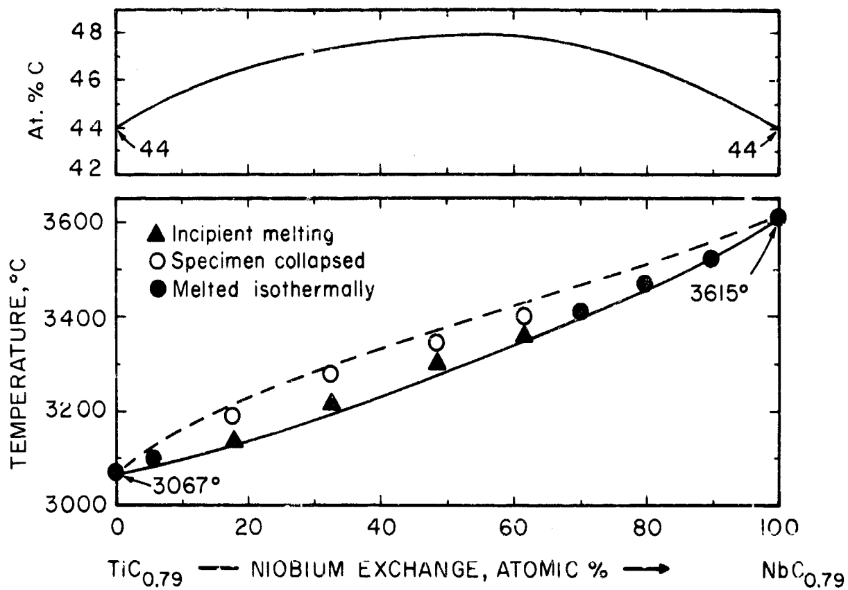
Figure 38. Maximum Solidus Temperatures of the (\text{Ti},\text{Nb})\text{C}_{1-x} Solid Solution.
