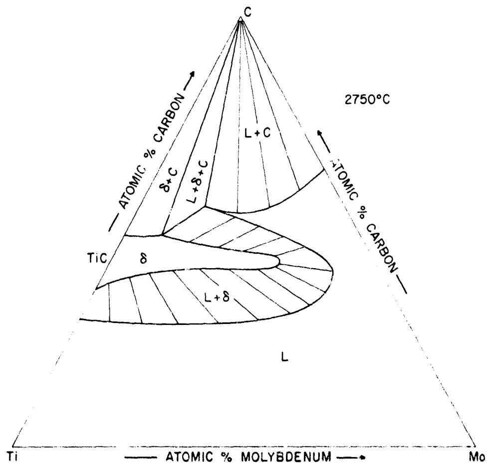
Figure 110. Isothermal Section of the Ti-Mo-C System at 2750°C.
