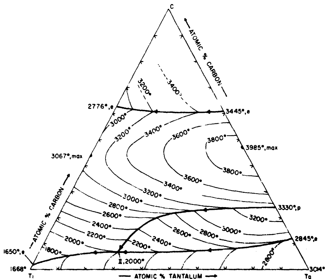
Figure 6. Liquidus Projections in the Ti-Ta-C System.
