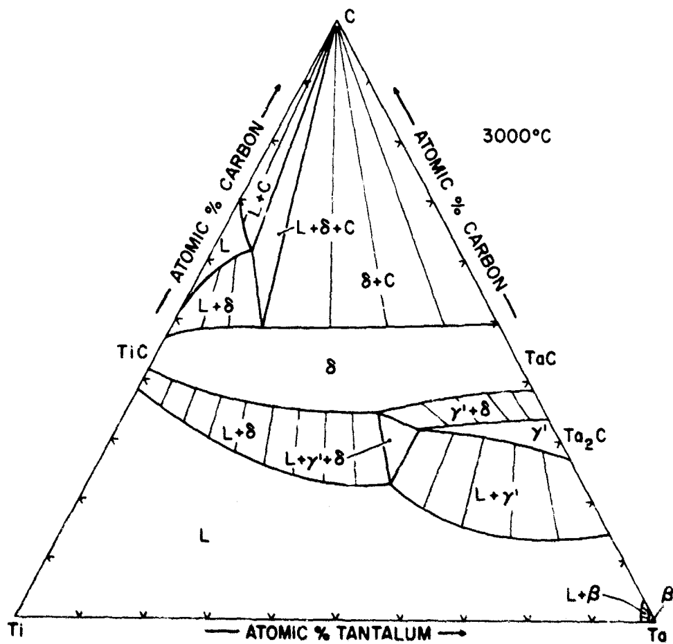
Figure 74. Isothermal Section of the Ti-Ta-C System at 3000°C.
