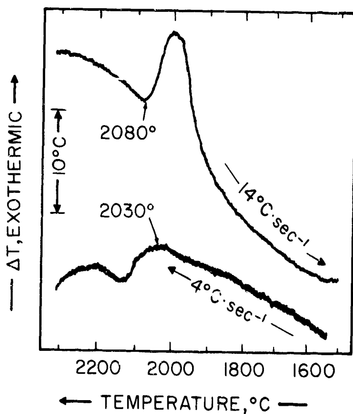
Figure 36. DTA-Thermogram of a Ti-Nb-C (28-47-25 At. %) Alloy Showing Bivariant Melting and Solidification of Metal-Rich Eutectic Alloys.
