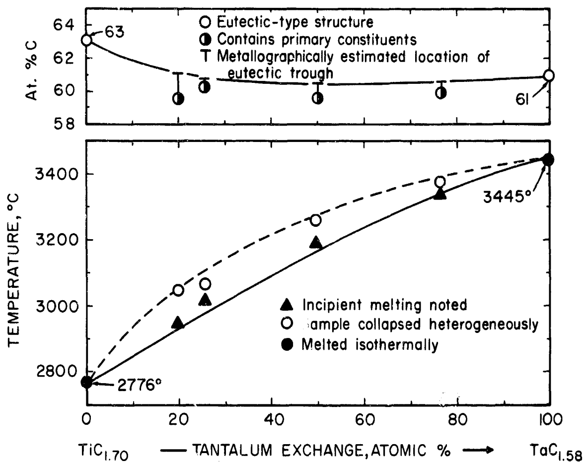
Figure 67. Melting Temperatures of Two-Phased, Monocarbide + Graphite Ti-Ta-C Alloys and Metallographic Location of Eutectic Trough.
