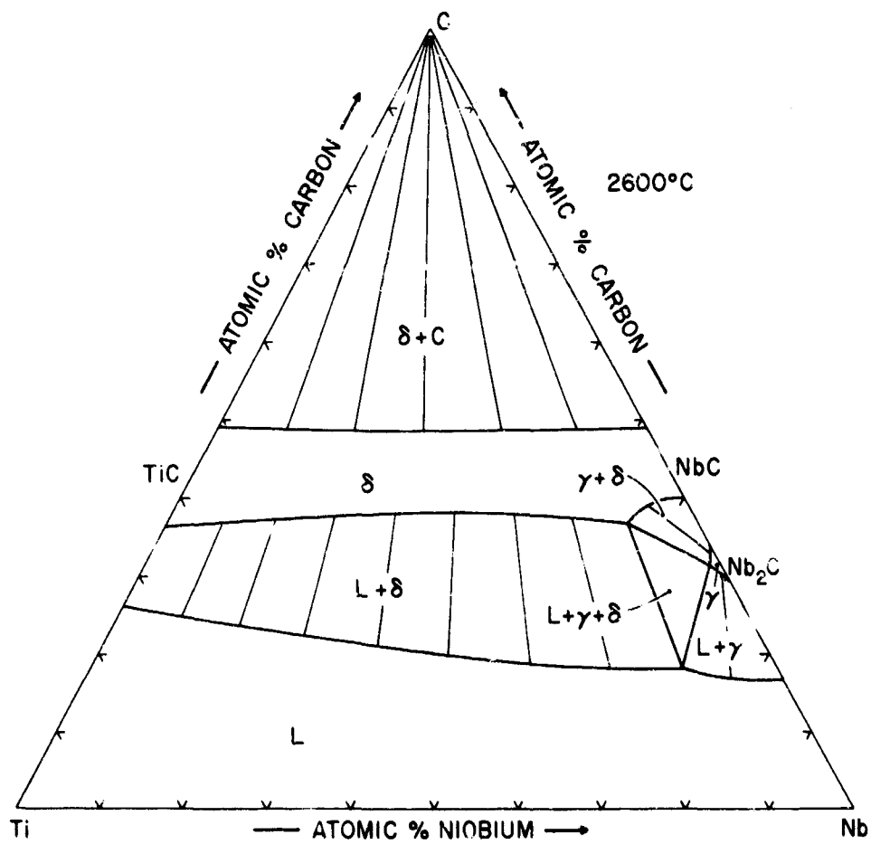
Figure 48. Isothermal Section of the Ti-Nb-C System at 2600°C.
