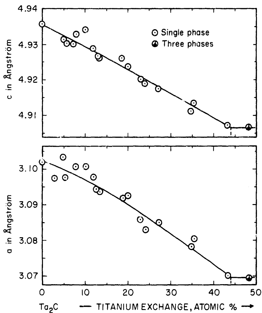
Figure 55. Lattice Parameters of the (Ti, Ta)_2C Solid Solution at 31 to 32 At.% Carbon. (Alloys Equilibrated at 2000° C)
