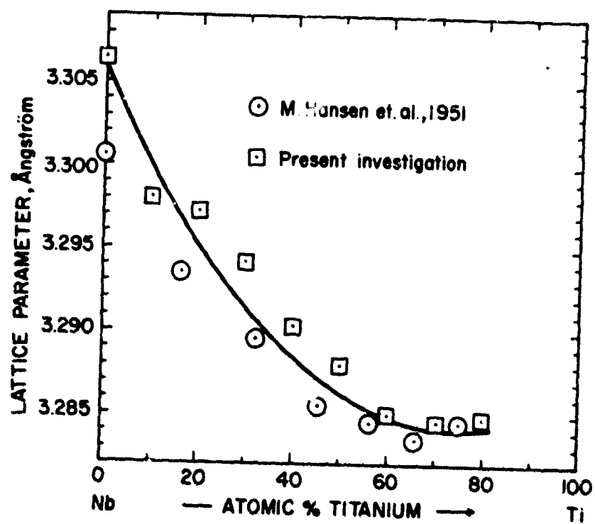
Figure 19. Lattice Parameters of the Cubic (Ti,Nb)-Solid Solution.
