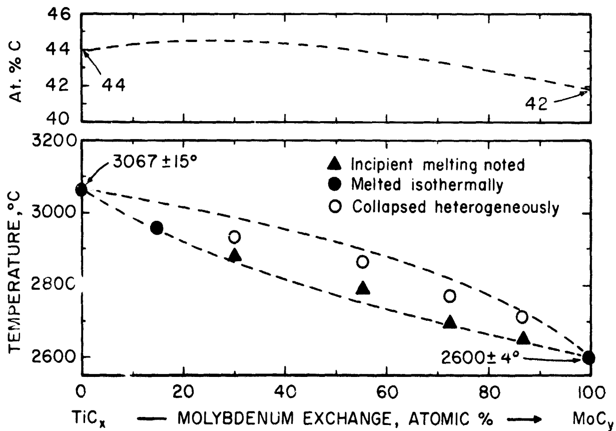
Figure 99. Maximum Solidus Temperatures of the (Ti,Mo)C 1-x Solid Solution.
