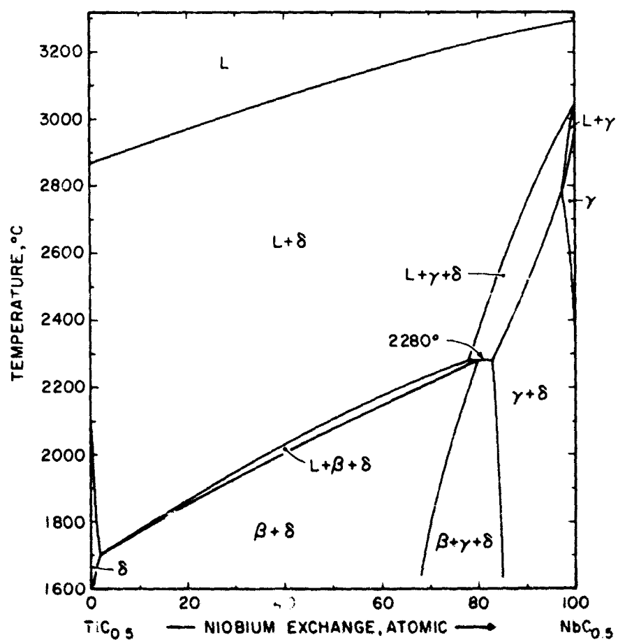
Figure 51. Isopleth \text{TiC}_{0.5} - \text{NbC}_{0.5}
