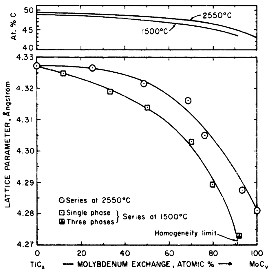
Figure 85. Lattice Parameters of the Carbon-Saturated Monocarbide Phase at 1500°C and 2550°C.
