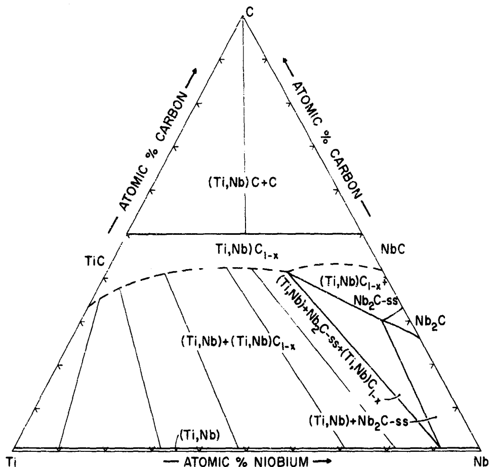
Figure 16. Isothermal Section of the Ti-Nb-C System at 1500°C.
