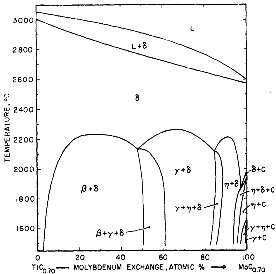
Figure 114. Isopleth \text{TiC}_{0.70} - \text{MoC}_{0.70}
