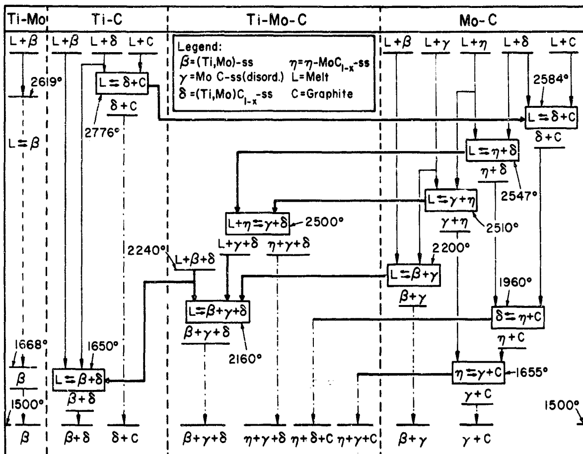
Figure 8. Reaction Diagram for the Ti-Mo-C System.
