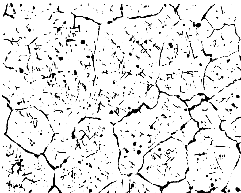
Figure 87. Ti-Mo-C (1-57-42 At.%), Equilibrated at 2350° C and X80 Cooled at 12° C per Second.
