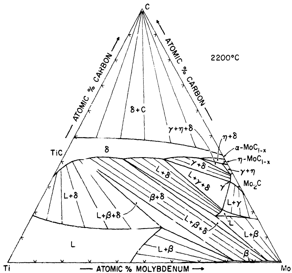
Figure 108. Isothermal Section of the Ti-Mo-C System at 2200° C.
