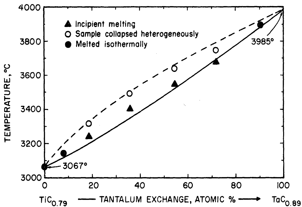
Figure 66. Maximum Solidus Temperatures of the (\text{Ti}, \text{Ta})\text{C}_{1-x} Solid Solution.
