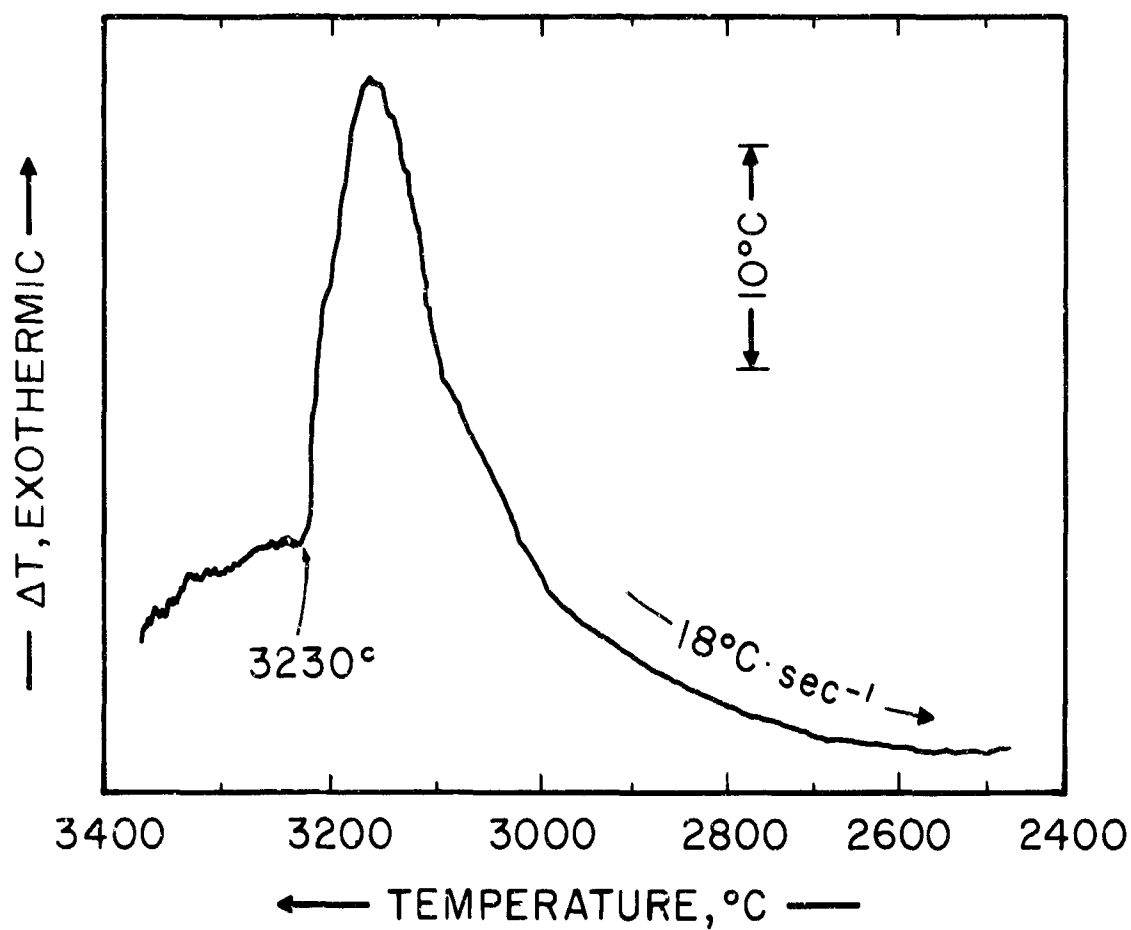
Figure 42. Solidification of the Bivariant (\text{Nb}, \text{Ti})\text{C} + \text{C} Eutectic in a Ti-Nb-C (7-38-55 At.%) Alloy.
