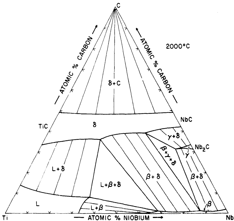
Figure 46. Isothermal Section of the Ti-Nb-C System at 2000° C.
