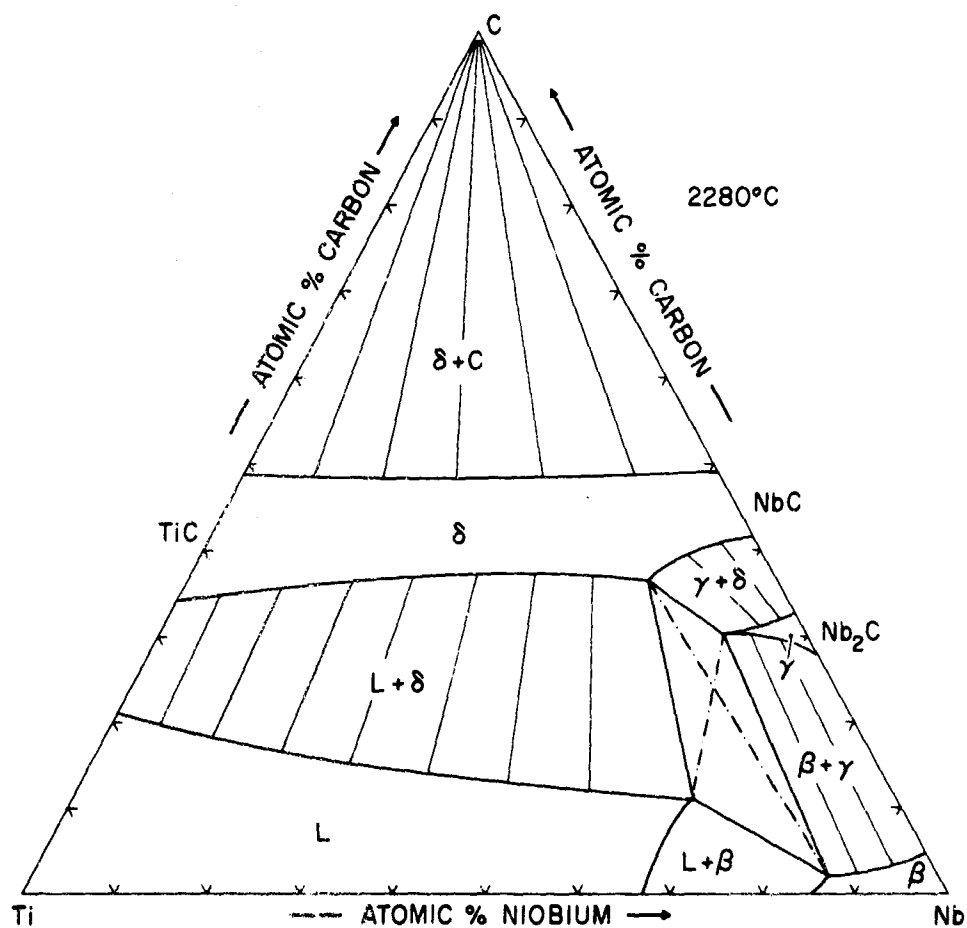
Figure 47. Isothermal Section of the Ti-Nb-C System at 2280°C.
