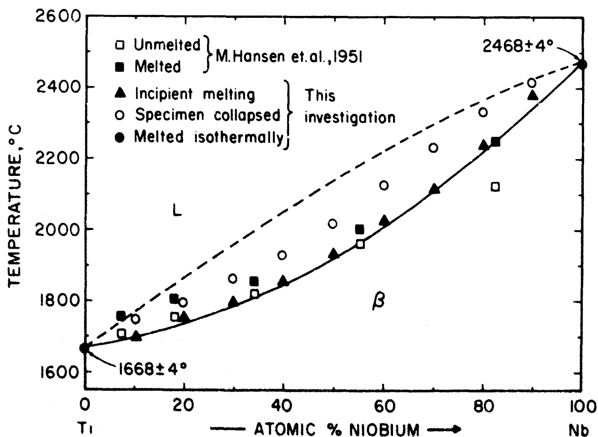
Figure 18. Melting Temperatures of Ti-Nb Alloys (Temperature error figures based on reproducibility)
