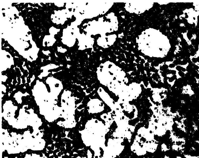
Figure 91. Ti-Mo-C (30-60-10 At. %), Melted and Rapidly Cooled.
