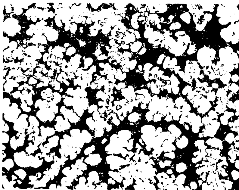
Figure 95. Ti-Mo-C (10-65-25 At.%), Melted and Quenched X350
