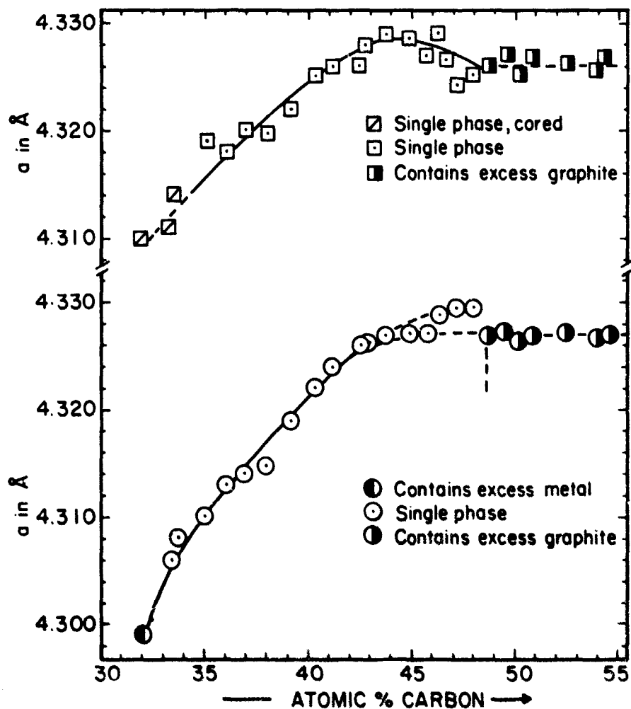
Figure 11. Lattice Parameters of the Carbon-Deficient Titanium Monocarbide.
