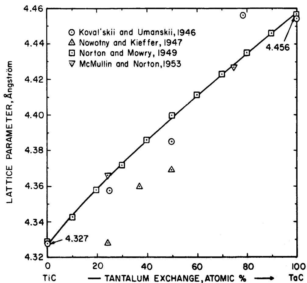
Figure 61. Lattice Parameters of the Cubic Monocarbide Solid Solution.
