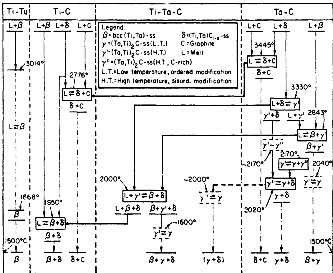
Figure 5. Reaction Diagram for Ti-Ta-C Alloys.
