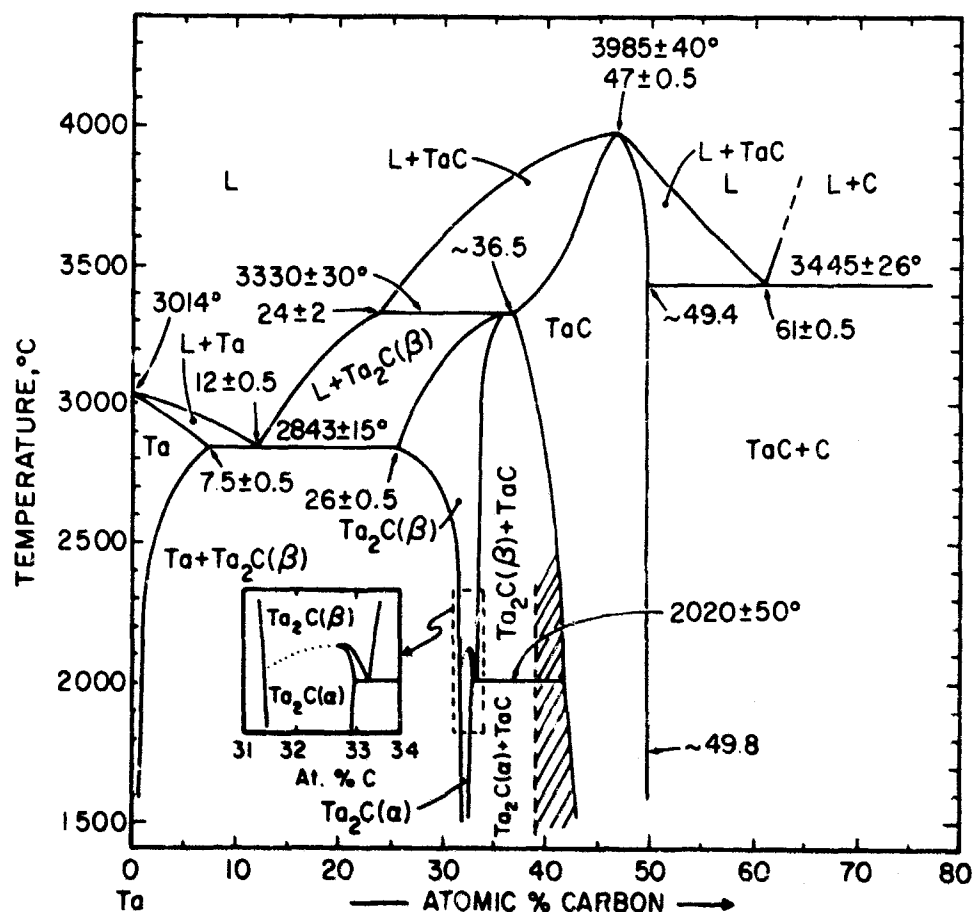
Figure 13. Phase Diagram of the Ta-C System. (After E. Rudy....., slightly revised).
