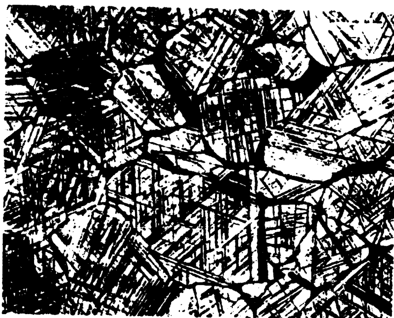
Figure 39. Ti-Nb-C (13-53-34 At.%), Equilibrated at 2600° C and Rapidly Cooled.
