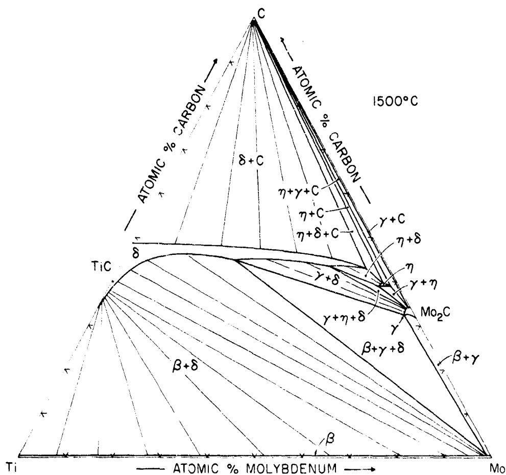
Figure 105. Isothermal Section of the Ti-Mo-C System at 1500°C.
