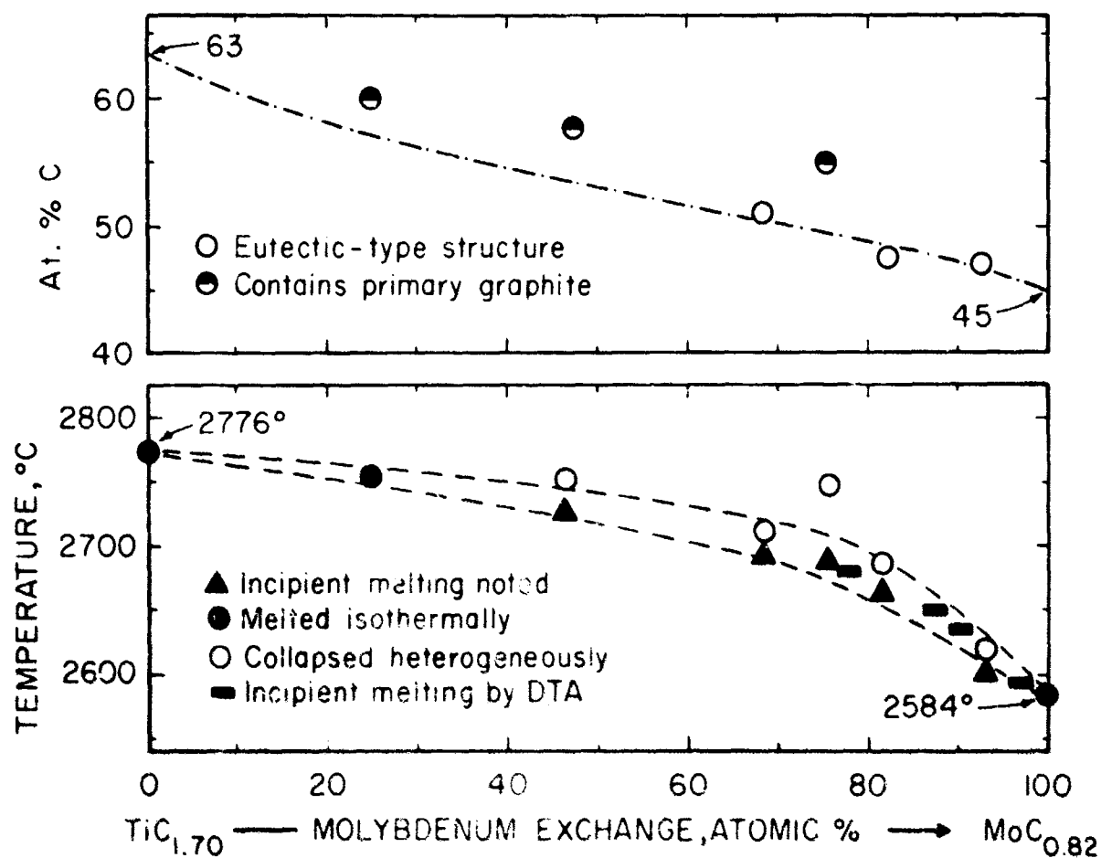
Figure 101. Melting Temperatures of Ti-Mo-C Alloys Located at, or Near, the Monocarbide + Graphite Eutectic Trough.
