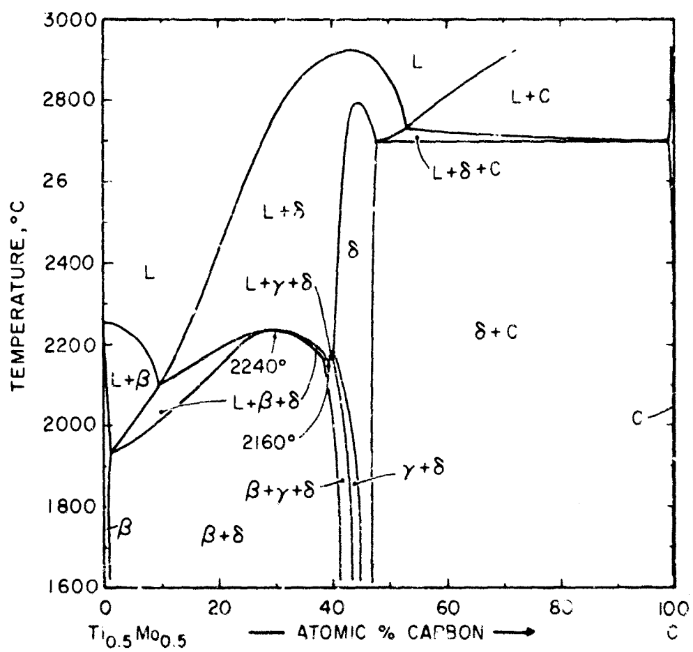
Figure 112. Isopleth \text{Ti}_{0.5}\text{Mo}_{0.5}\text{-C} .
