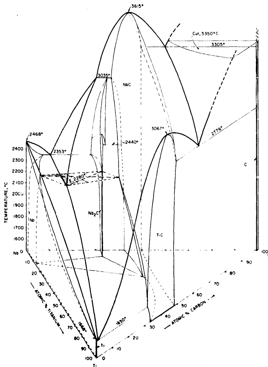
Figure 1. Isometric View of the Ti-Nb-C System.
