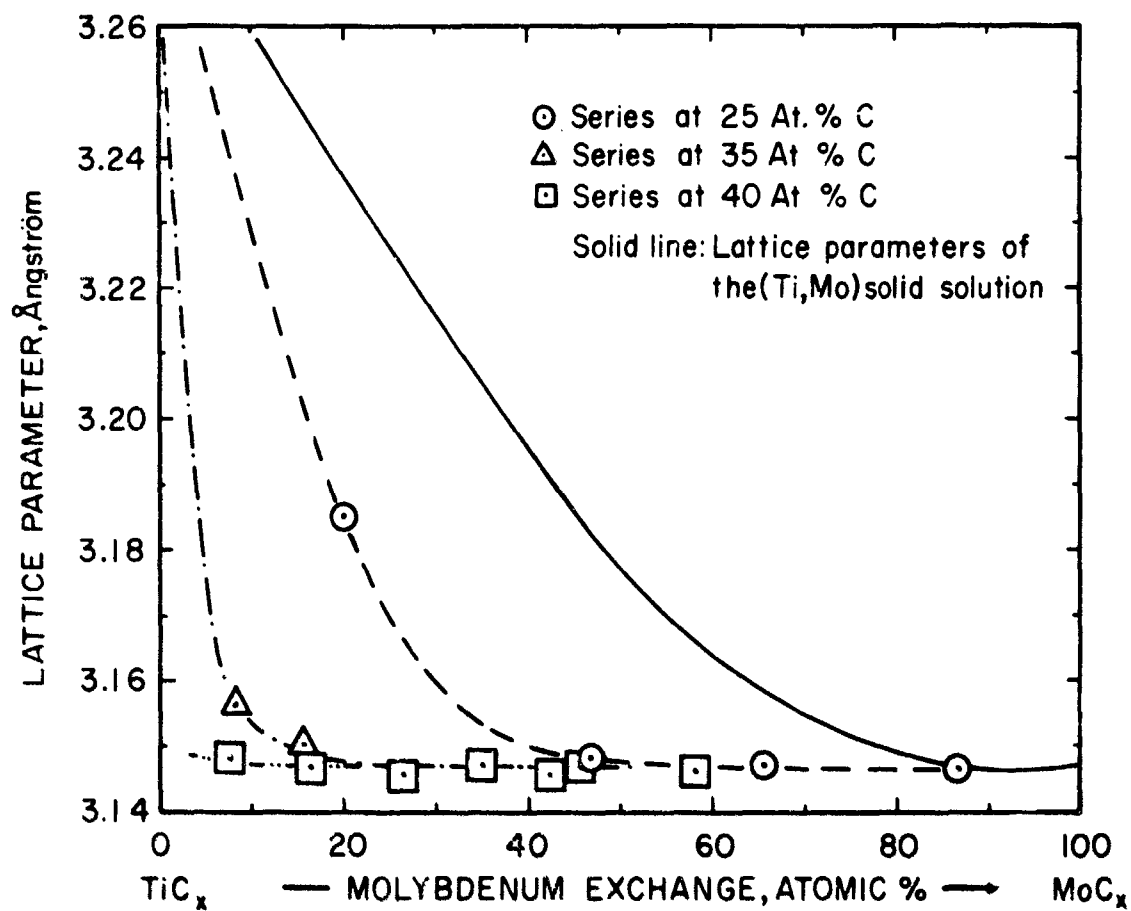
Figure 82. Lattice Parameters of the Cubic (A2) Metal Phase in Two-Phased, \beta + \delta , Alloys.
