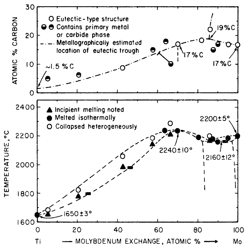
Figure 89. Ti-Mo-C: Melting Temperatures of Alloys Located Along the Metal-Rich Eutectic Trough and Metallographically Estimated Boundary Line.
