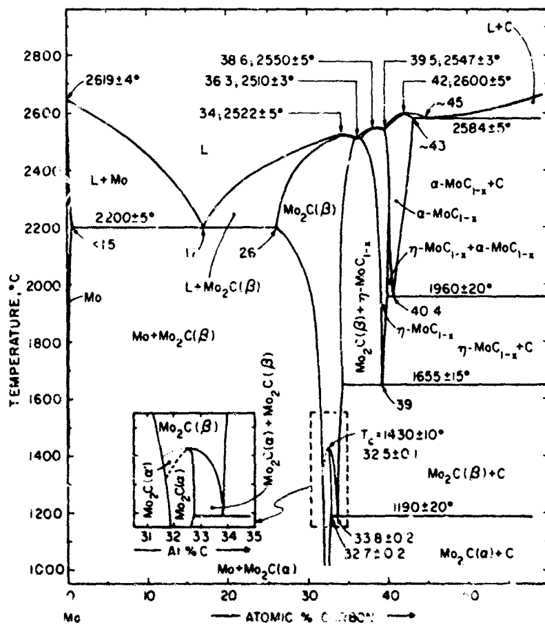
Figure 14. Phase Diagram of the Mo-C System (After E. Rudy et al., 1967).
