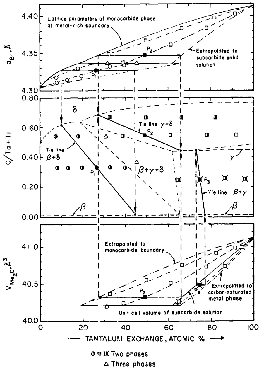
Figure 54. Measured Lattice Parameters for Two- and Three-Phased Ti-Ta-C, Graphical Smoothing of the Tie Lines, and Determination of the Tie Line Distribution in the Two-Phase Fields \beta + \delta , \beta + \gamma , and \gamma + \delta .
