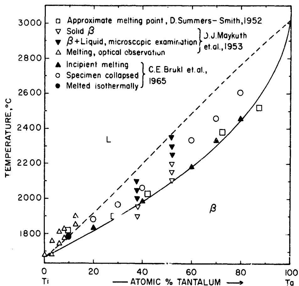
Figure 20. Melting Temperatures of Ti-Ta Alloys
