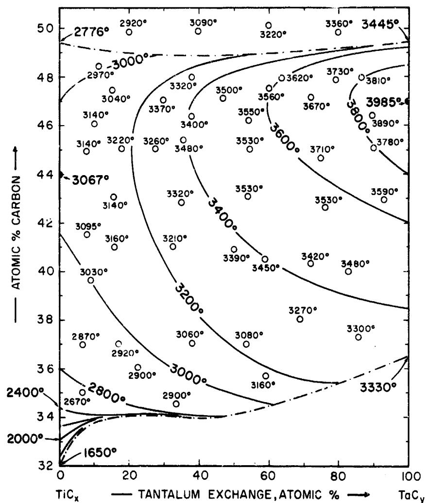
Figure 65. Experimental Solidus Surface and Derived Solidus Isotherms for the Monocarbide Solid Solution in the Ti-Ta-C System.
