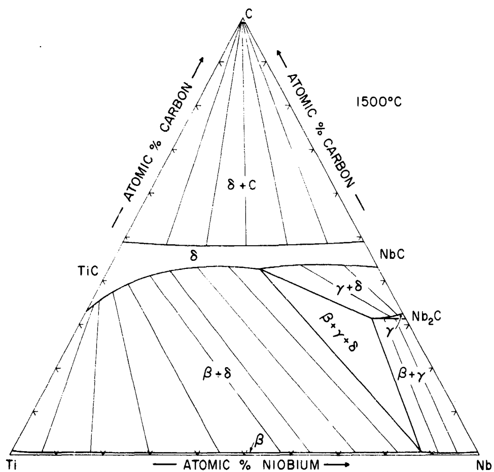
Figure 44. Isothermal Section of the Ti-Nb-C System at 1500°C.
