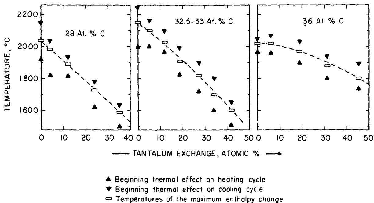
Figure 58. Experimental Order-Disorder Transition Temperatures of the (\text{Ta}, \text{Ti})_2\text{C} -Phase in Samples with Different Carbon Contents.
