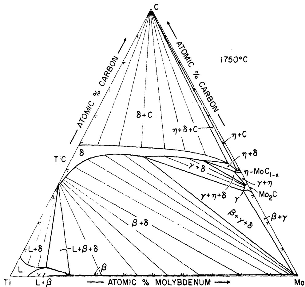
Figure 106. Isothermal Section of the Ti-Mo-C System at 1750°C.
